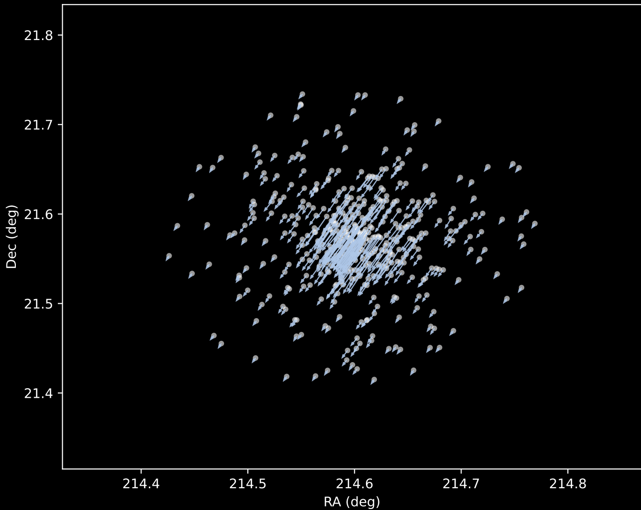
Gaia DR3 Cluster 1 Proper Motion Vectors (n=421)
