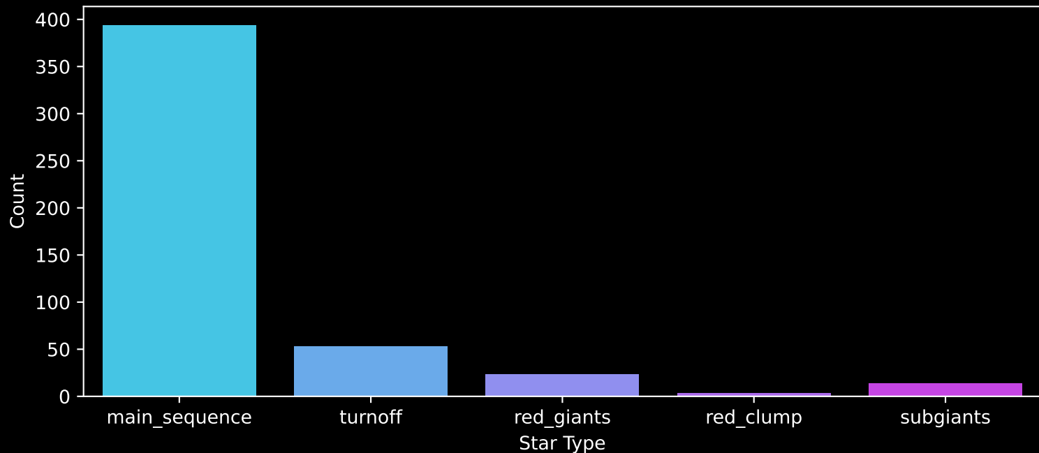
Gaia Cluster: [NGC_2420] Count plot of Star Type
