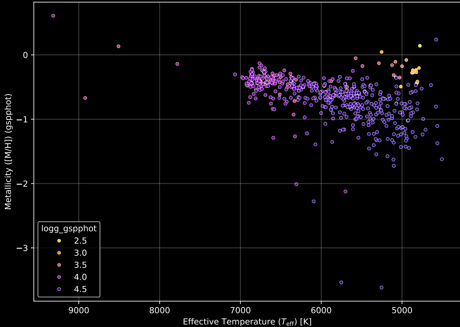
Gaia Cluster: [NGC_2420] Stellar Population Parameters (n= 487)
