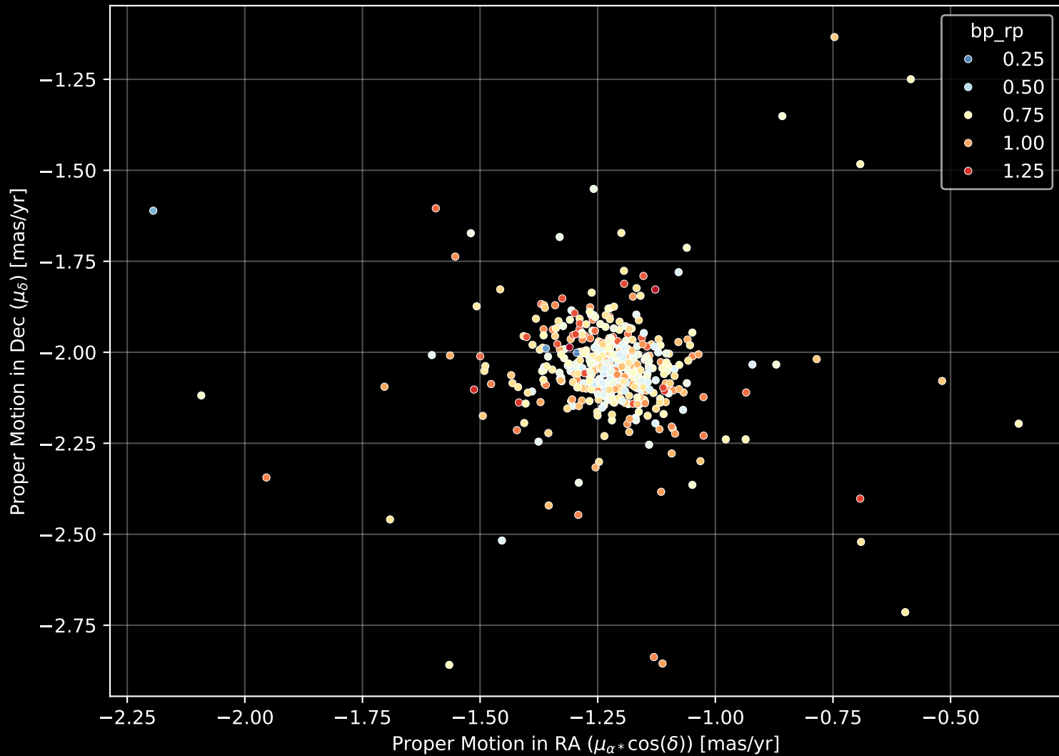
Gaia Cluster: [NGC_2420] Proper Motion Diagram (n= 487)
