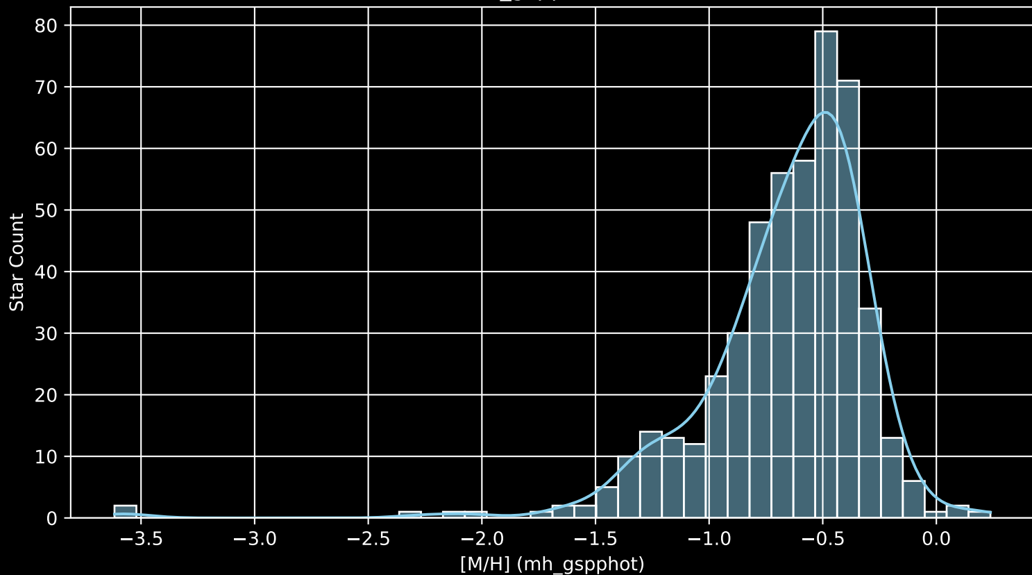
Gaia Cluster: [NGC_2420 [M/H] (mh_gspphot) (n= 486)
