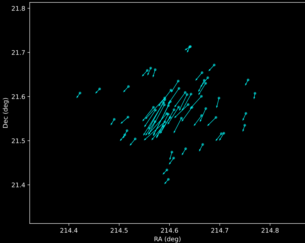
Gaia DR3 Noise Stream Proper Motion Vectors (n=60)
