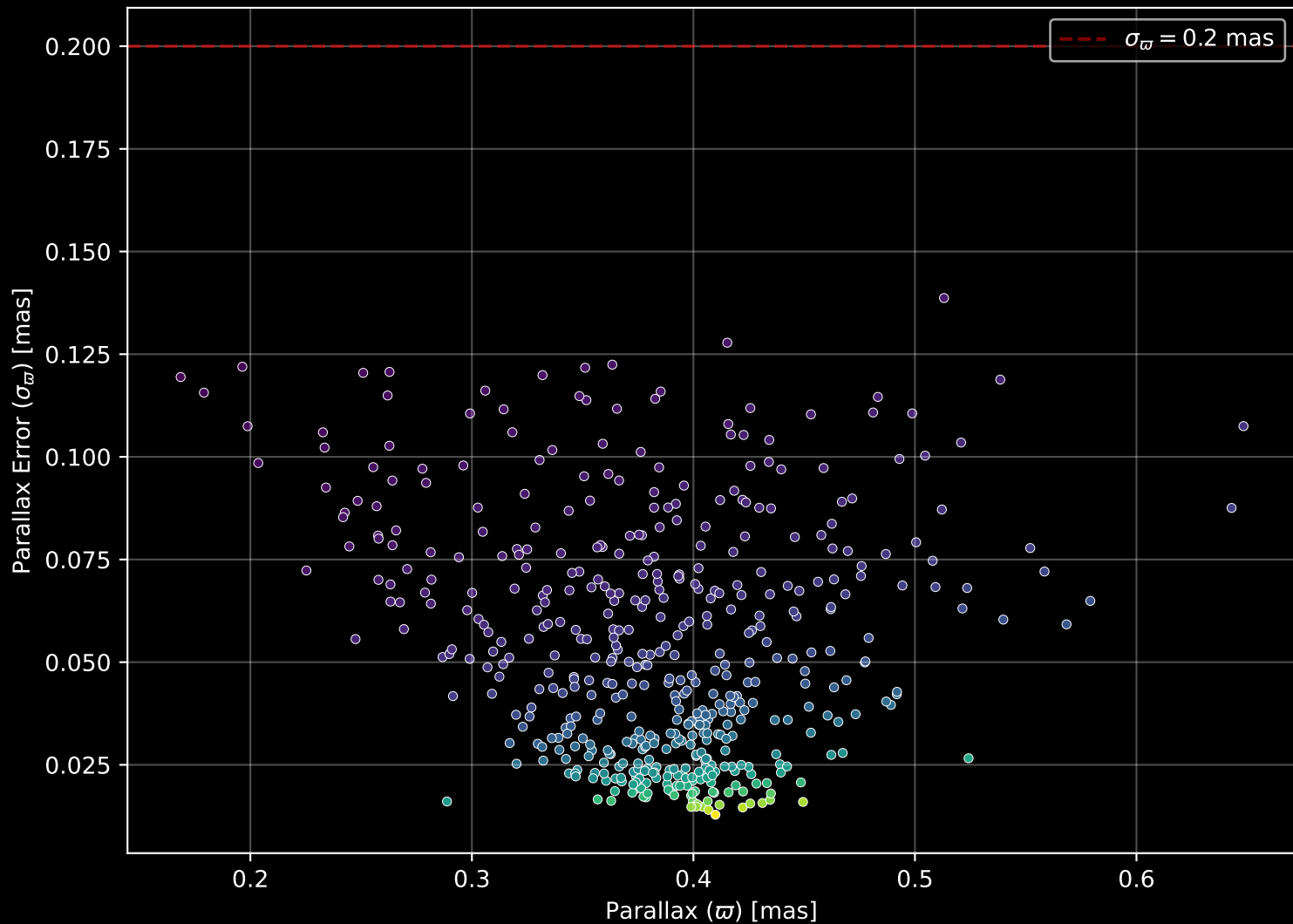
Gaia Cluster: [NGC_2420] Parallax Quality (n= 487)
