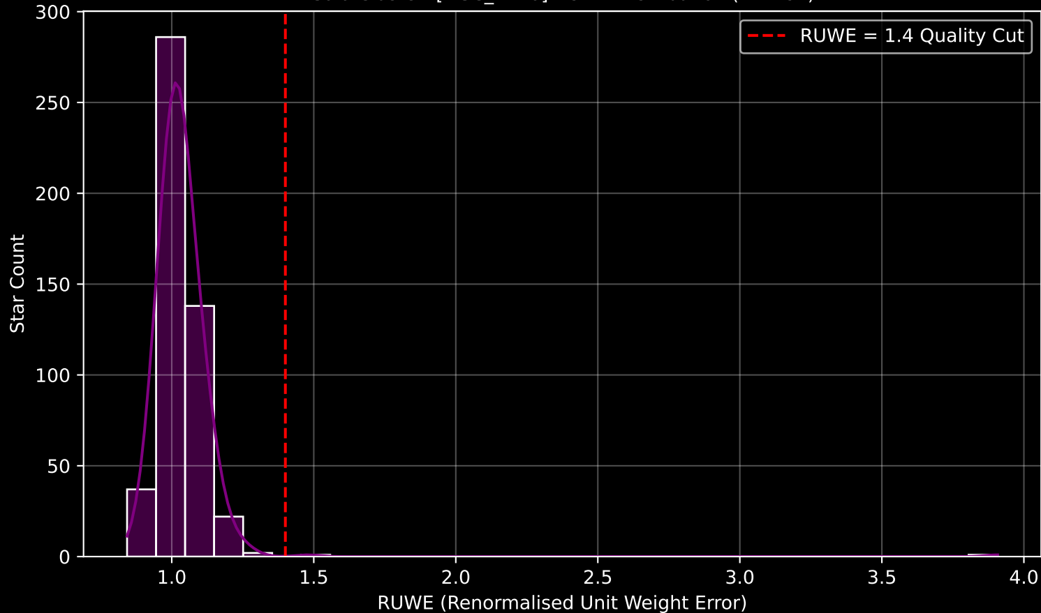
Gaia Cluster: [NGC_2420] RUWE Distribution (n= 487)
