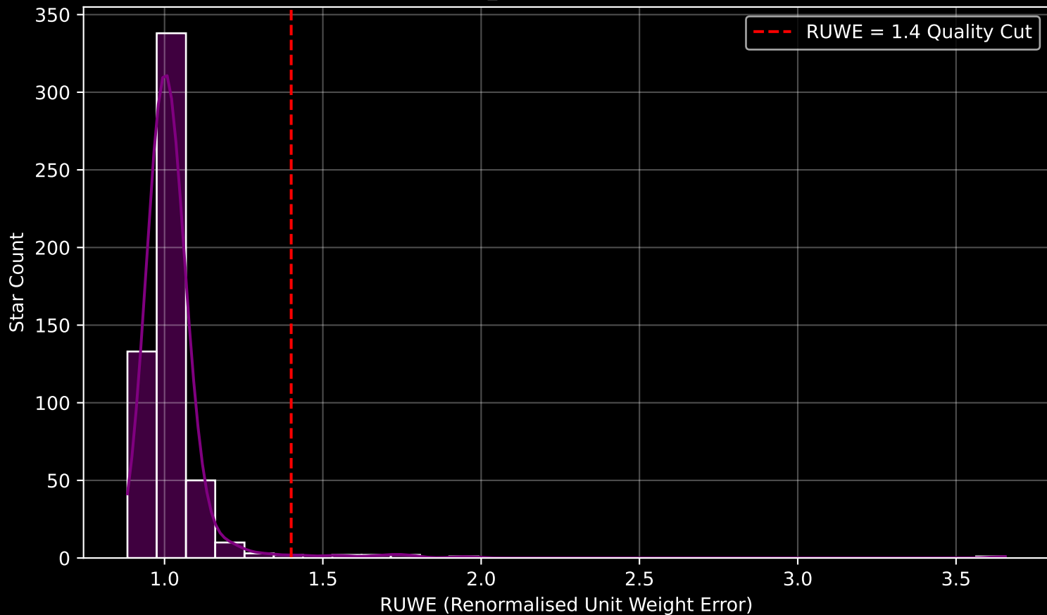
Gaia Cluster: [NGC_2421] RUWE Distribution (n= 544)
