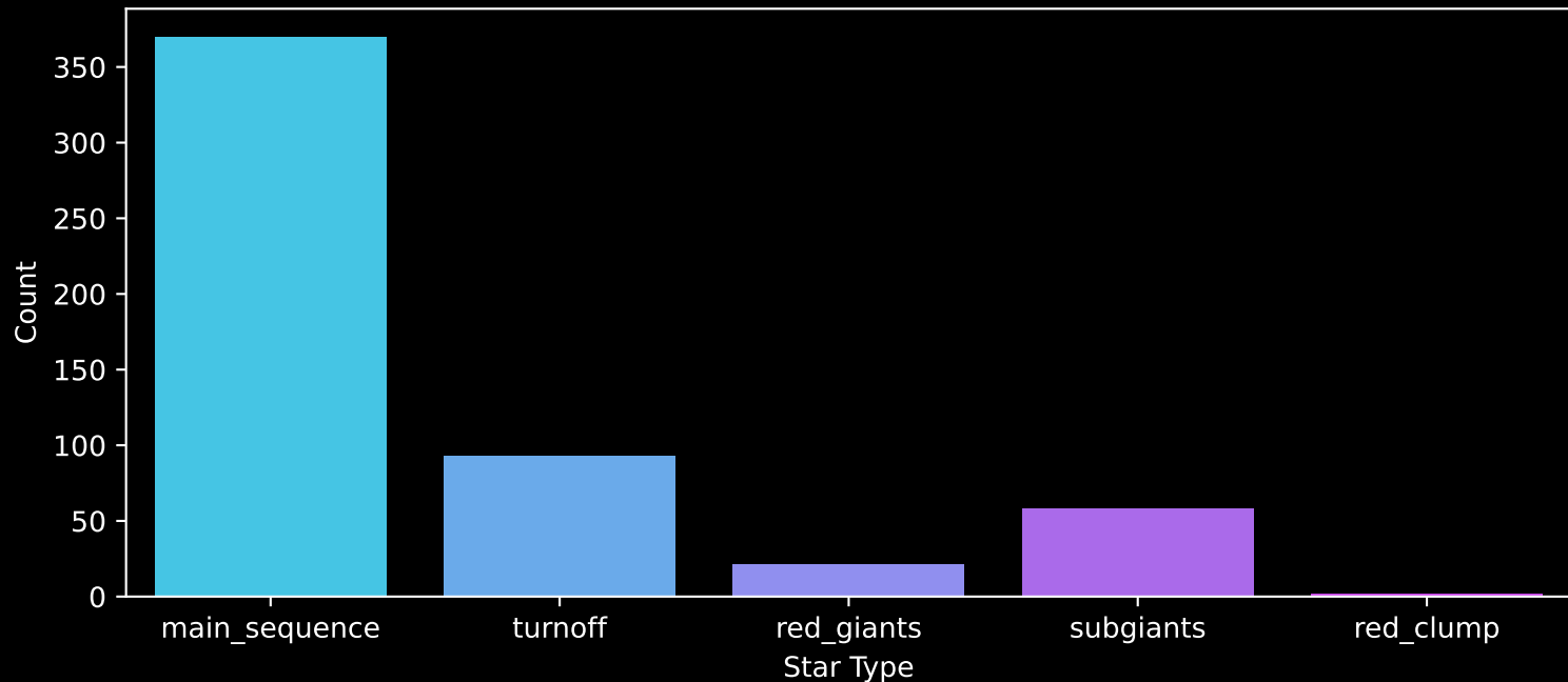
Gaia Cluster: [NGC_2421] Count plot of Star Type
