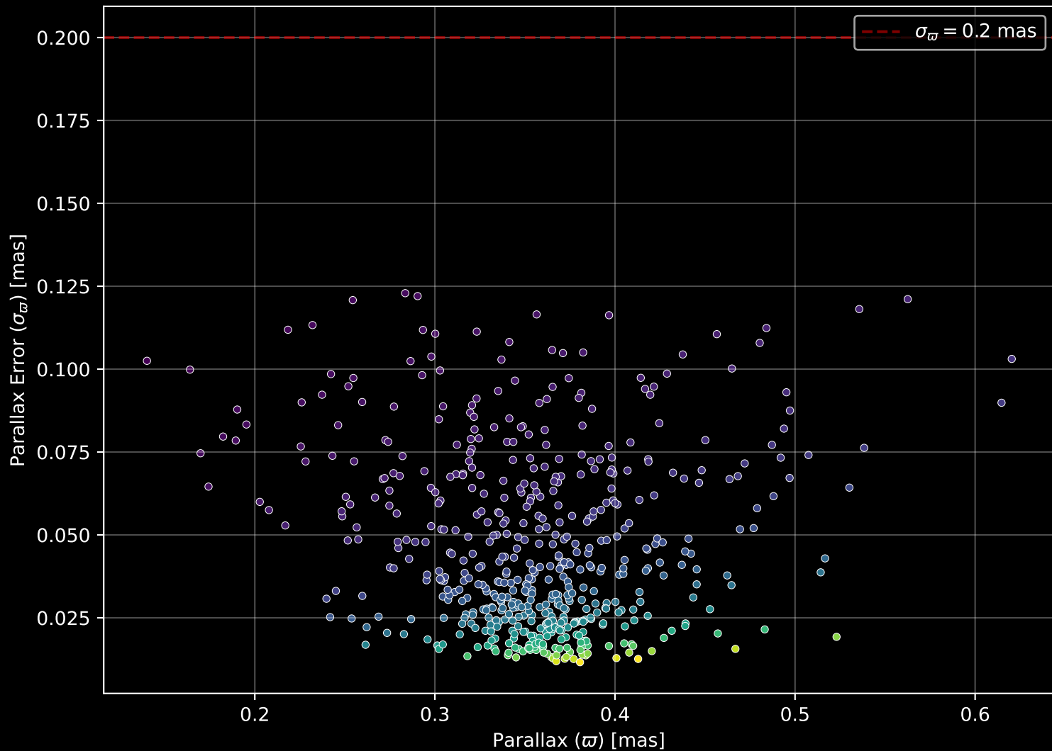
Gaia Cluster: [NGC_2421] Parallax Quality (n= 544)
