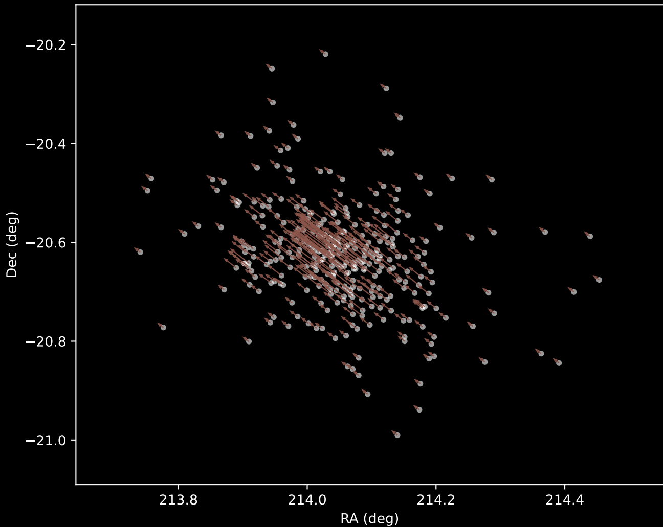
Gaia DR3 Cluster 10 Proper Motion Vectors (n=321)
