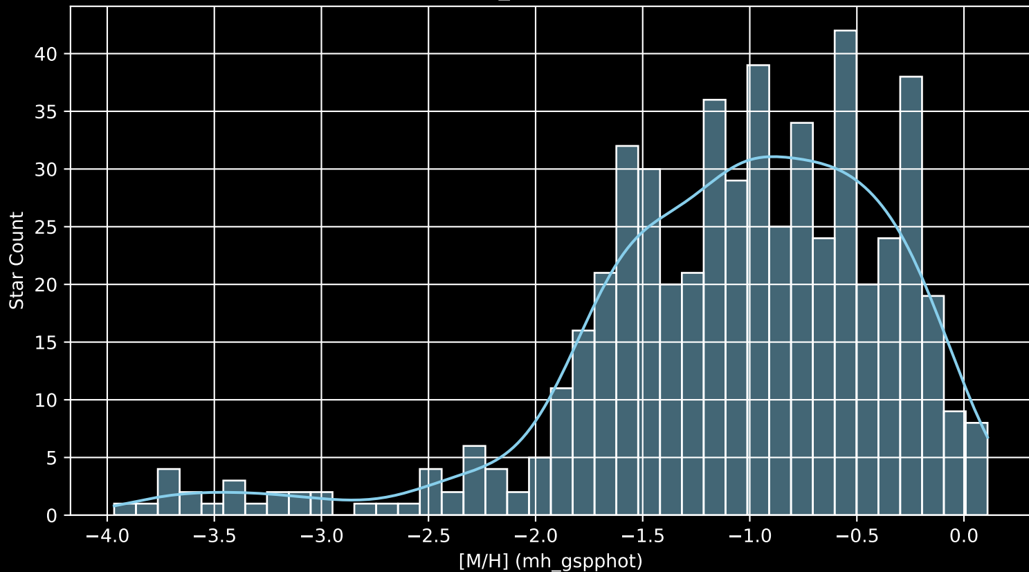
Gaia Cluster: [NGC_2421 [M/H] (mh_gspphot) (n= 543)
