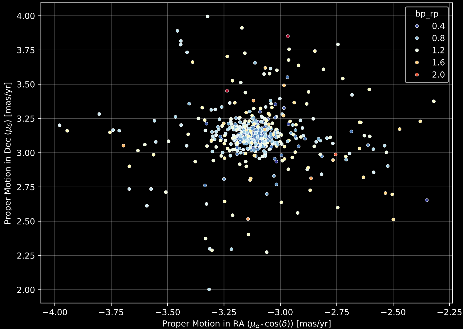
Gaia Cluster: [NGC_2421] Proper Motion Diagram (n= 544)
