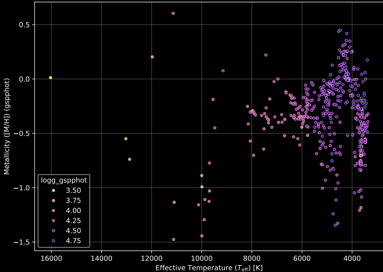
Gaia Cluster: [NGC_2422] Stellar Population Parameters (n= 424)
