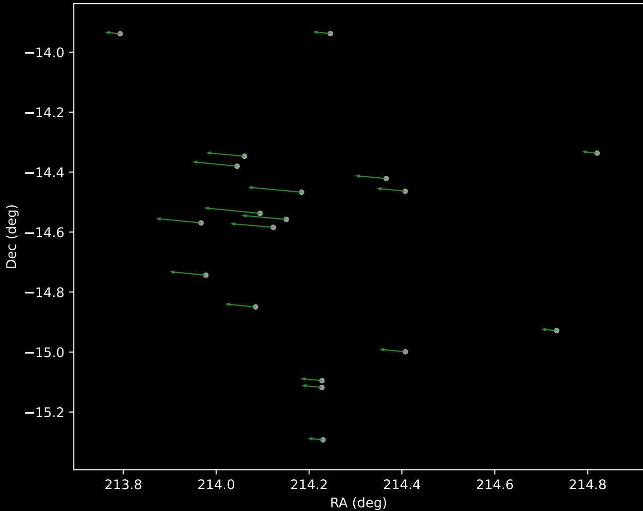
Gaia DR3 Cluster 24 Proper Motion Vectors (n=19)
