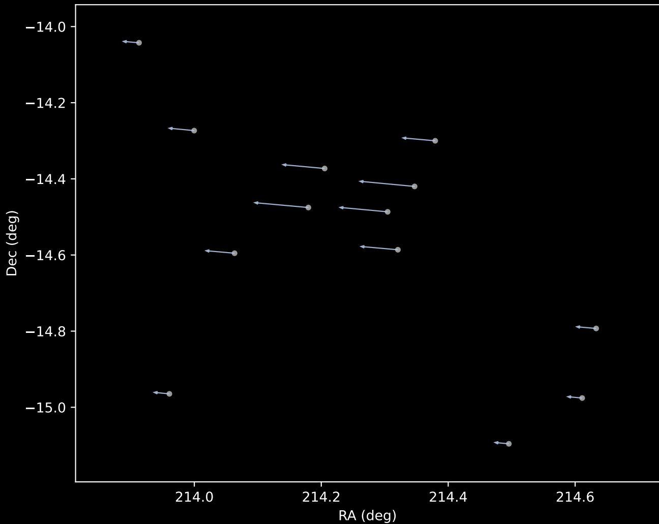
Gaia DR3 Cluster 21 Proper Motion Vectors (n=13)
