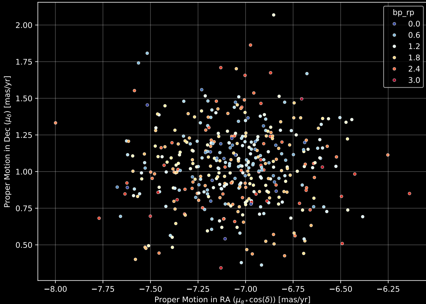
Gaia Cluster: [NGC_2422] Proper Motion Diagram (n= 424)
