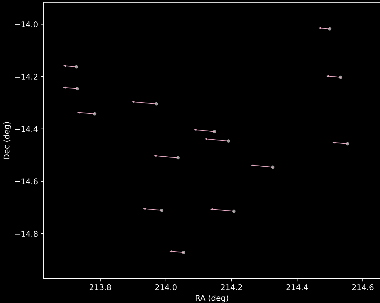
Gaia DR3 Cluster 13 Proper Motion Vectors (n=14)
