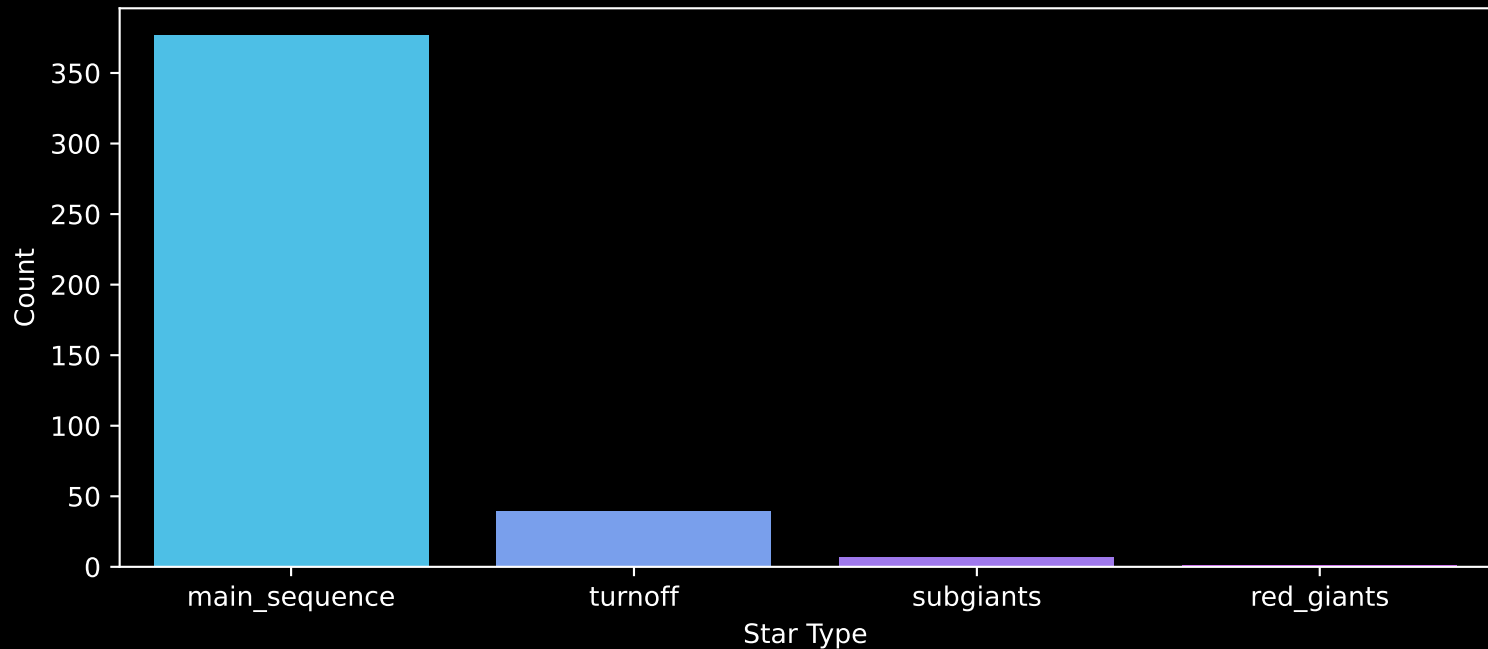
Gaia Cluster: [NGC_2422] Count plot of Star Type
