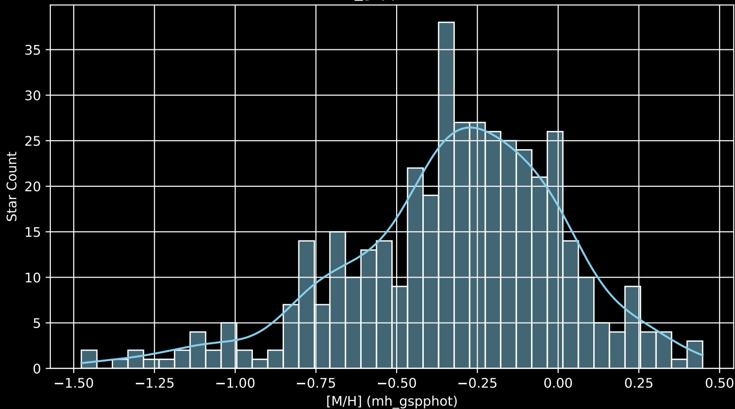
Gaia Cluster: [NGC_2422 [M/H] (mh_gspphot) (n= 423)
