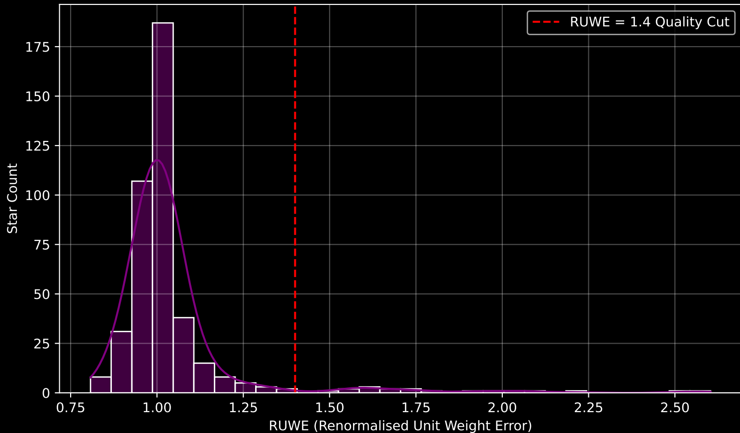
Gaia Cluster: [NGC_2422] RUWE Distribution (n= 422)
