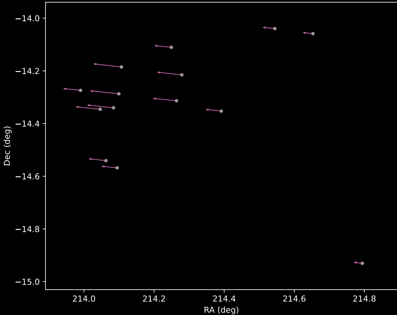
Gaia DR3 Cluster 12 Proper Motion Vectors (n=14)
