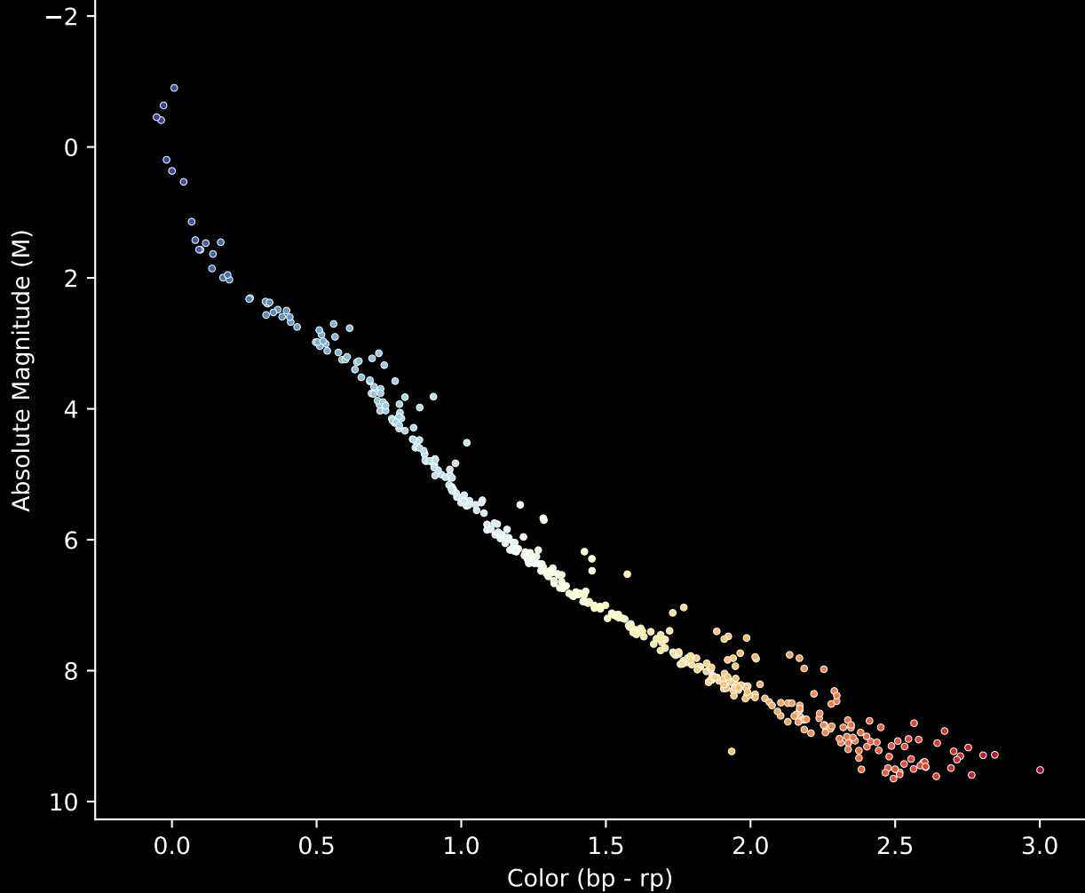
Gaia Cluster: [NGC_2422] Stars (n= 424) Hertzsprung-Russel Diagram
