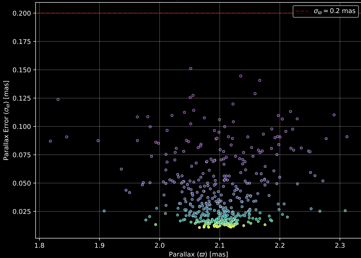
Gaia Cluster: [NGC_2422] Parallax Quality (n= 424)
