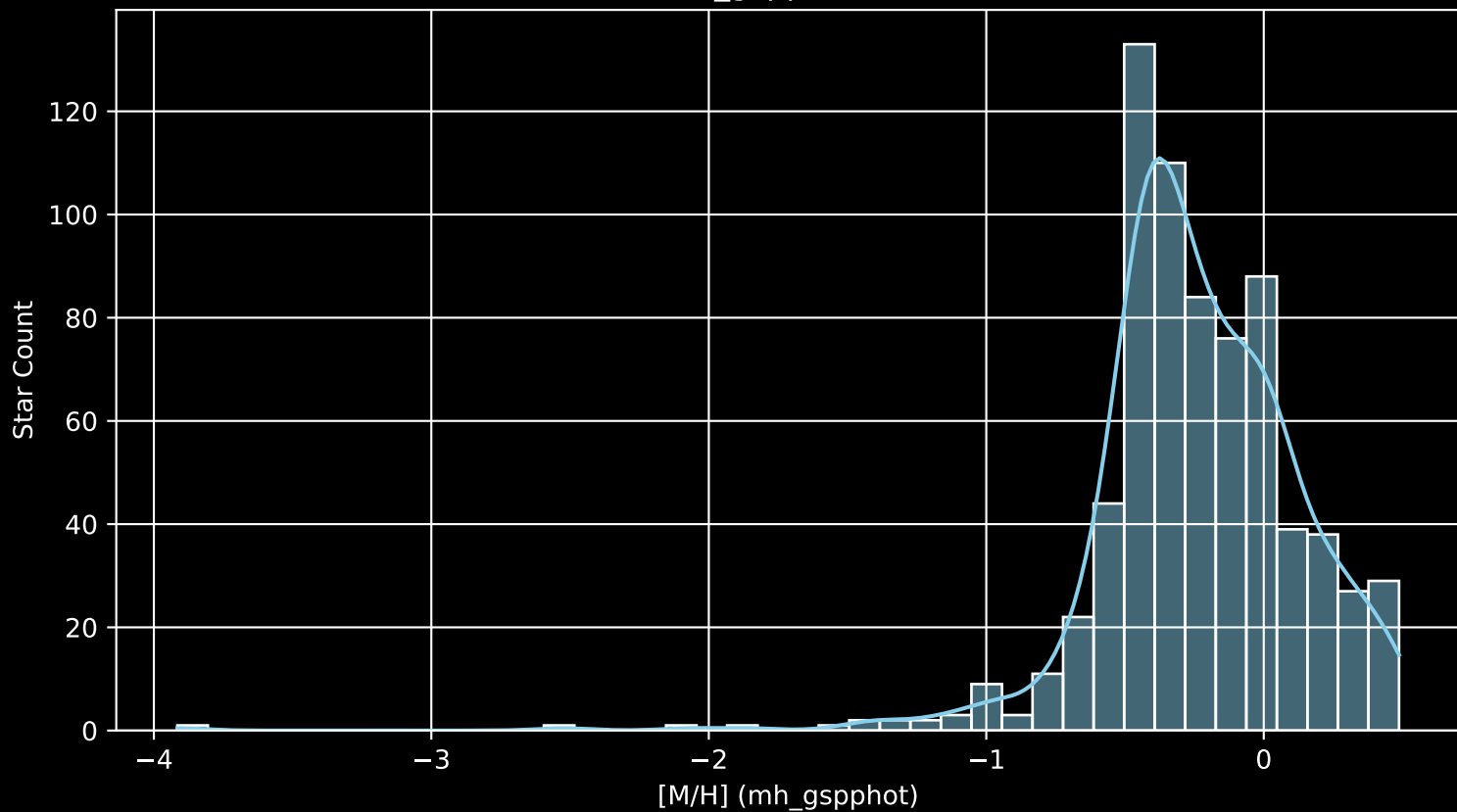
Gaia Cluster: [NGC_2447 [M/H] (mh_gspphot) (n= 727)
