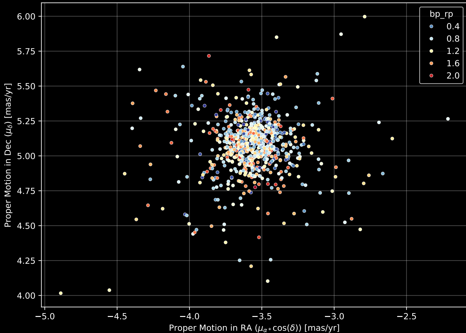
Gaia Cluster: [NGC_2447] Proper Motion Diagram (n= 730)
