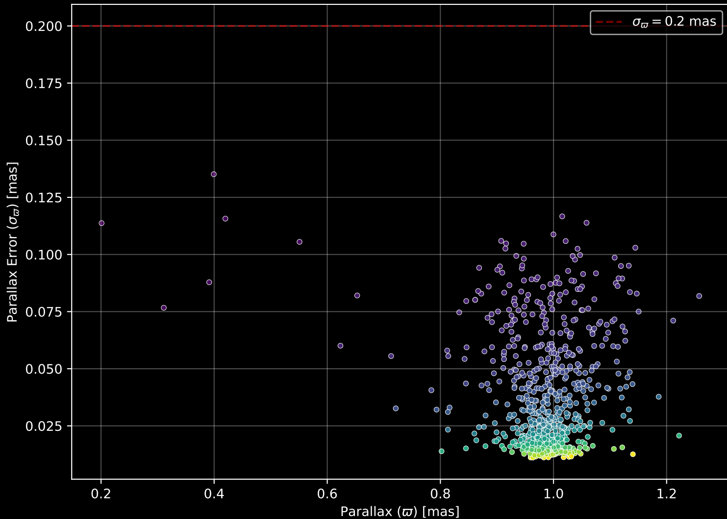
Gaia Cluster: [NGC_2447] Parallax Quality (n= 730)
