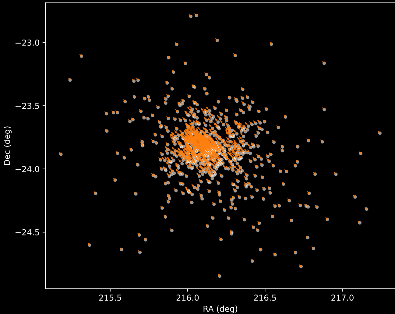
Gaia DR3 Cluster 2 Proper Motion Vectors (n=639)
