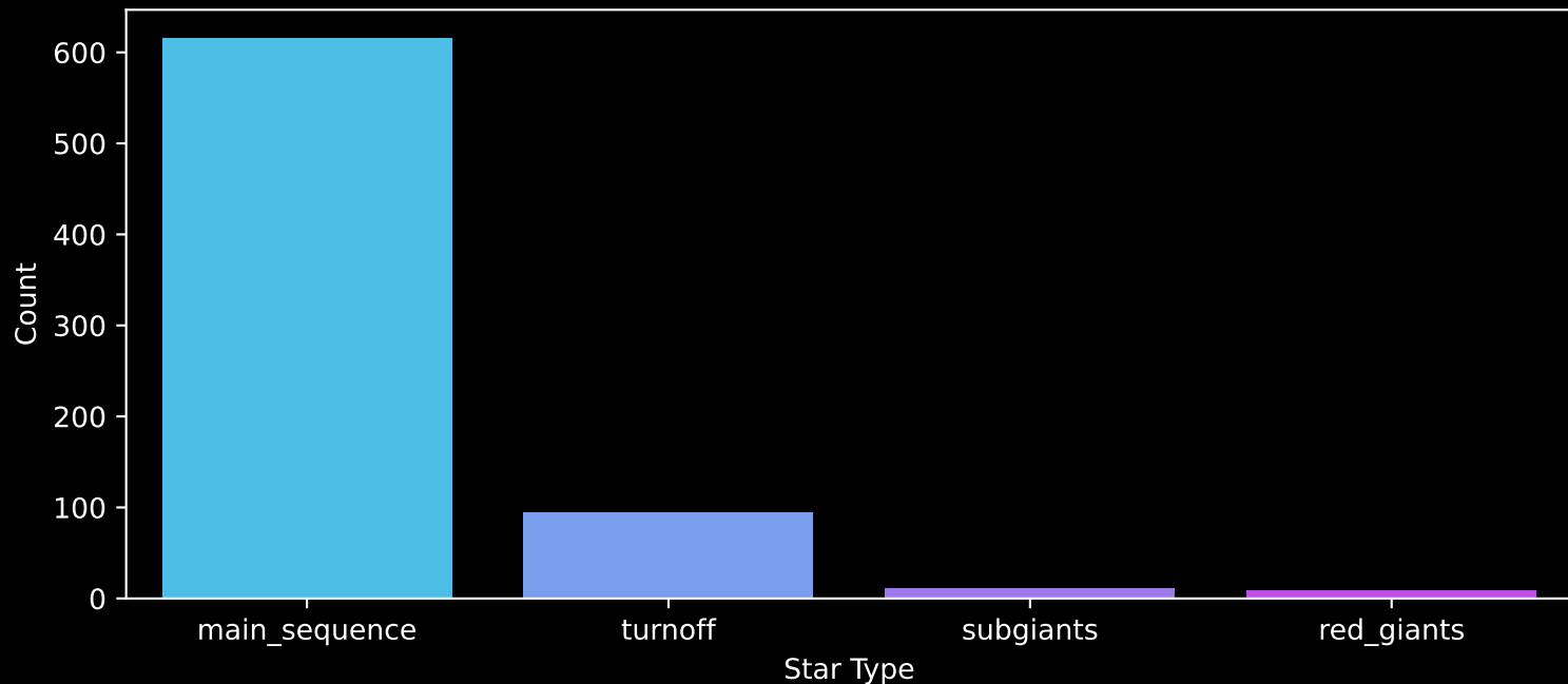
Gaia Cluster: [NGC_2447] Count plot of Star Type
