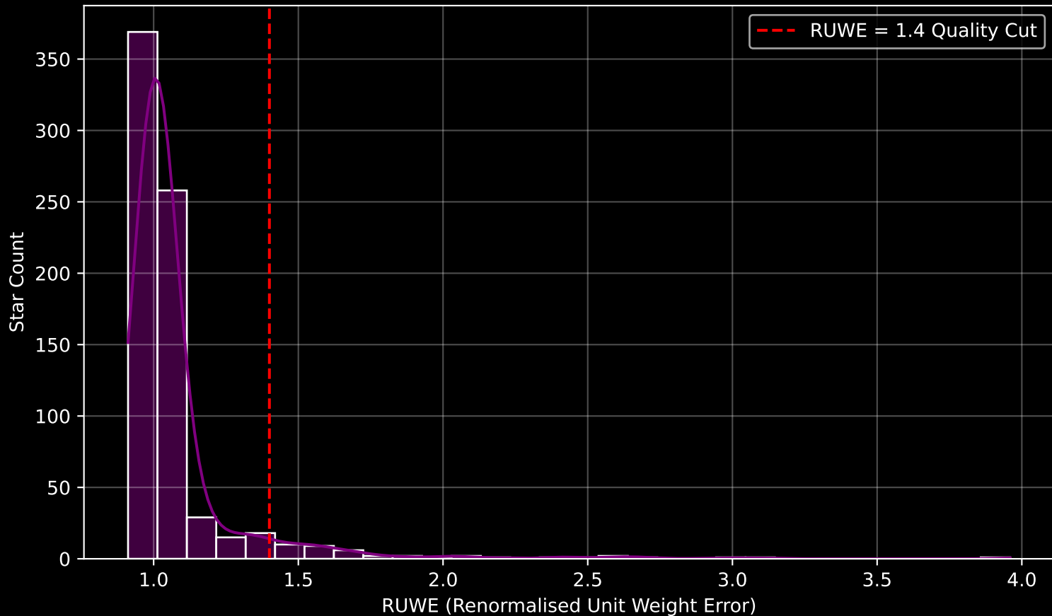
Gaia Cluster: [NGC_2447] RUWE Distribution (n= 730)
