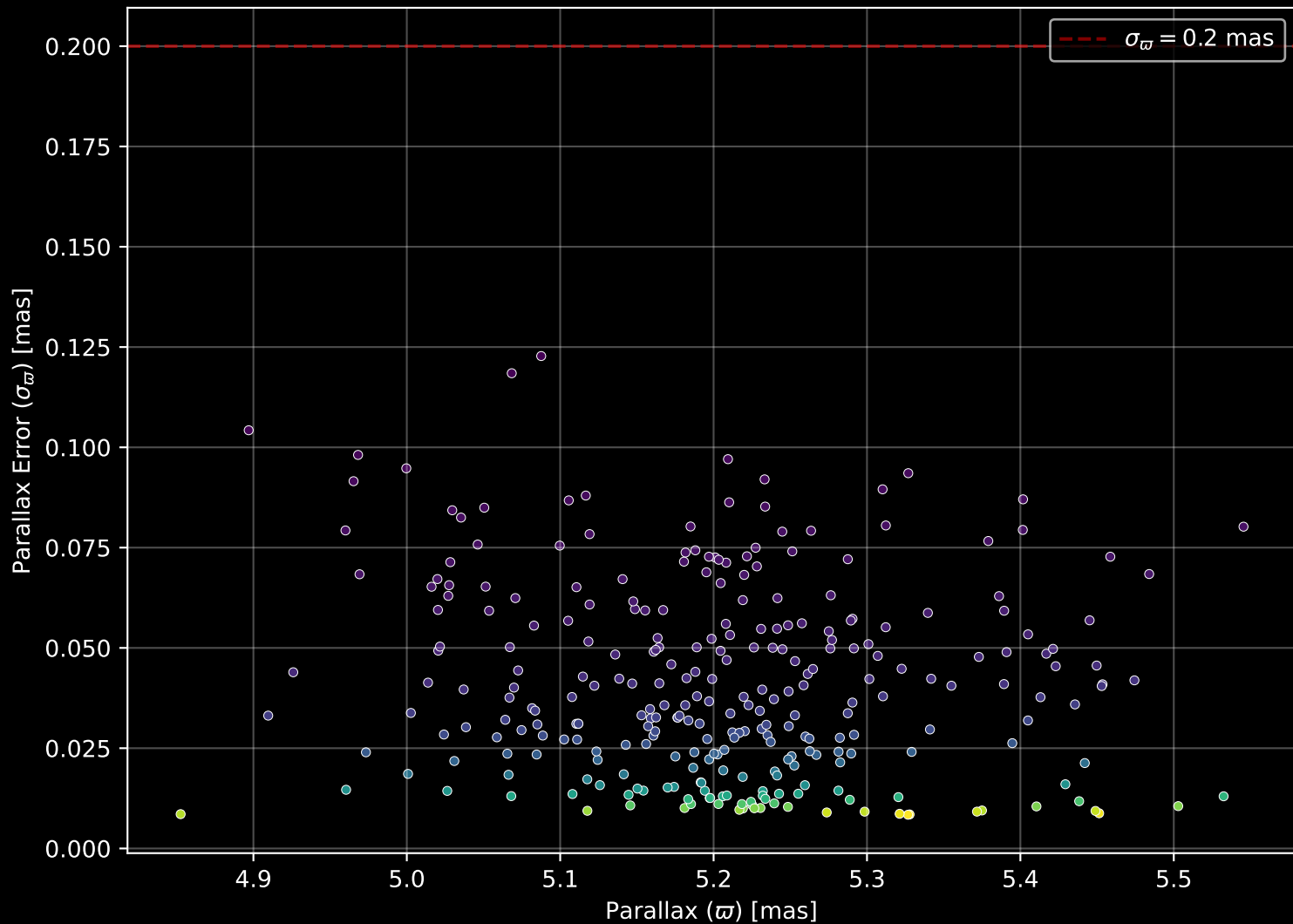
Gaia Cluster: [NGC_2451A] Parallax Quality (n= 289)
