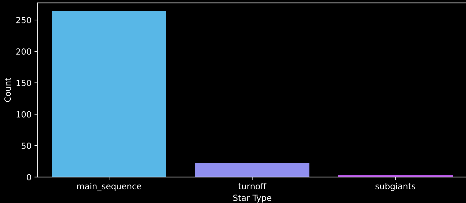
Gaia Cluster: [NGC_2451A] Count plot of Star Type
