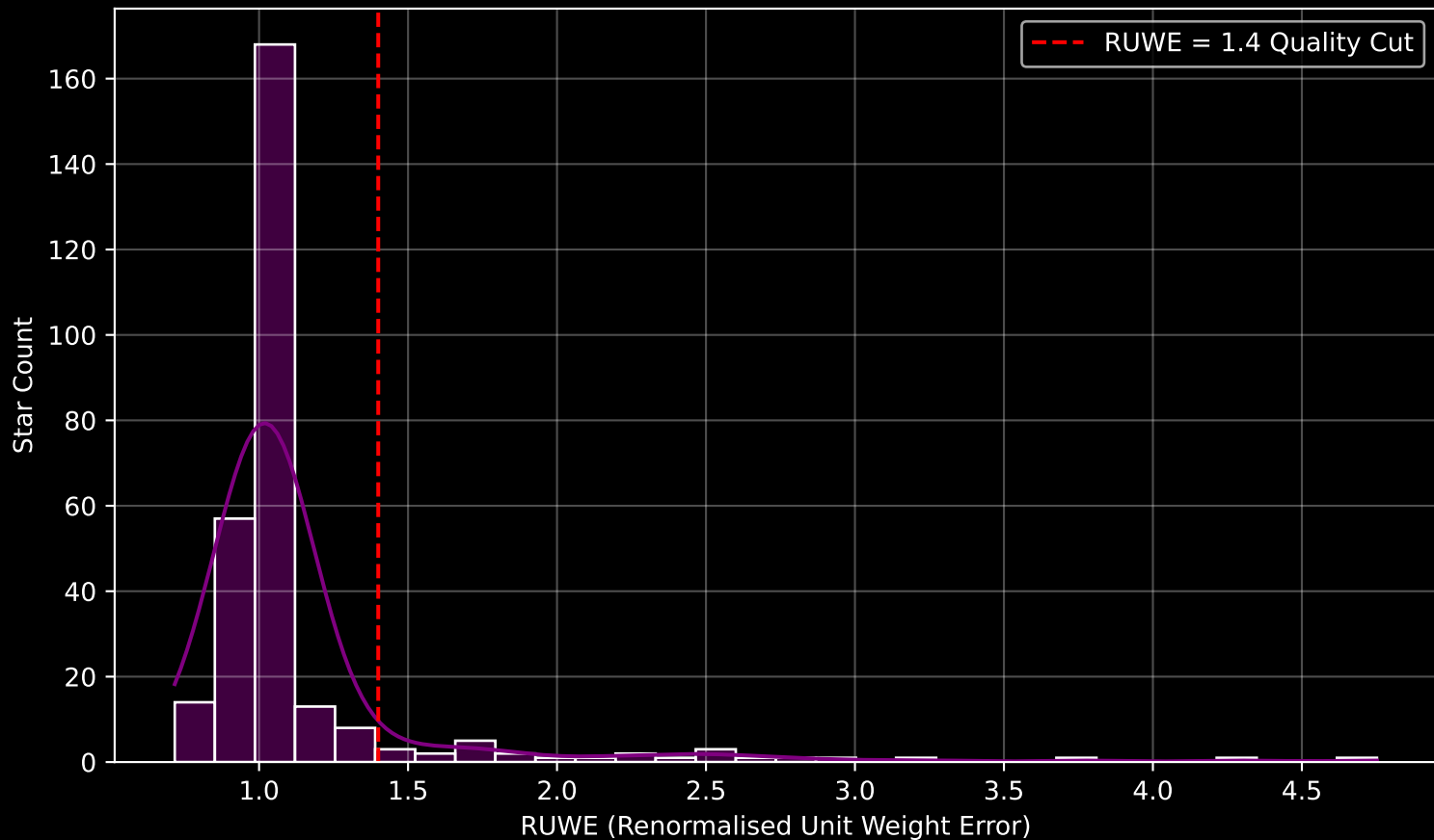
Gaia Cluster: [NGC_2451A] RUWE Distribution (n= 287)
