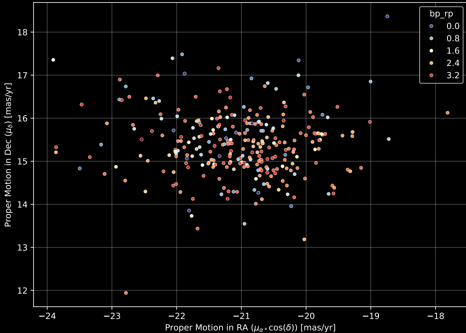
Gaia Cluster: [NGC_2451A] Proper Motion Diagram (n= 289)
