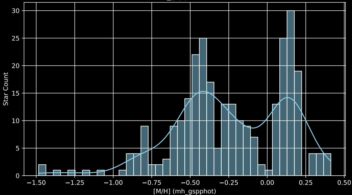
Gaia Cluster: [NGC_2451A [M/H] (mh_gspphot) (n= 287)
