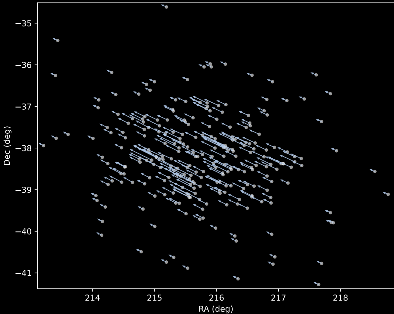
Gaia DR3 Cluster 1 Proper Motion Vectors (n=251)
