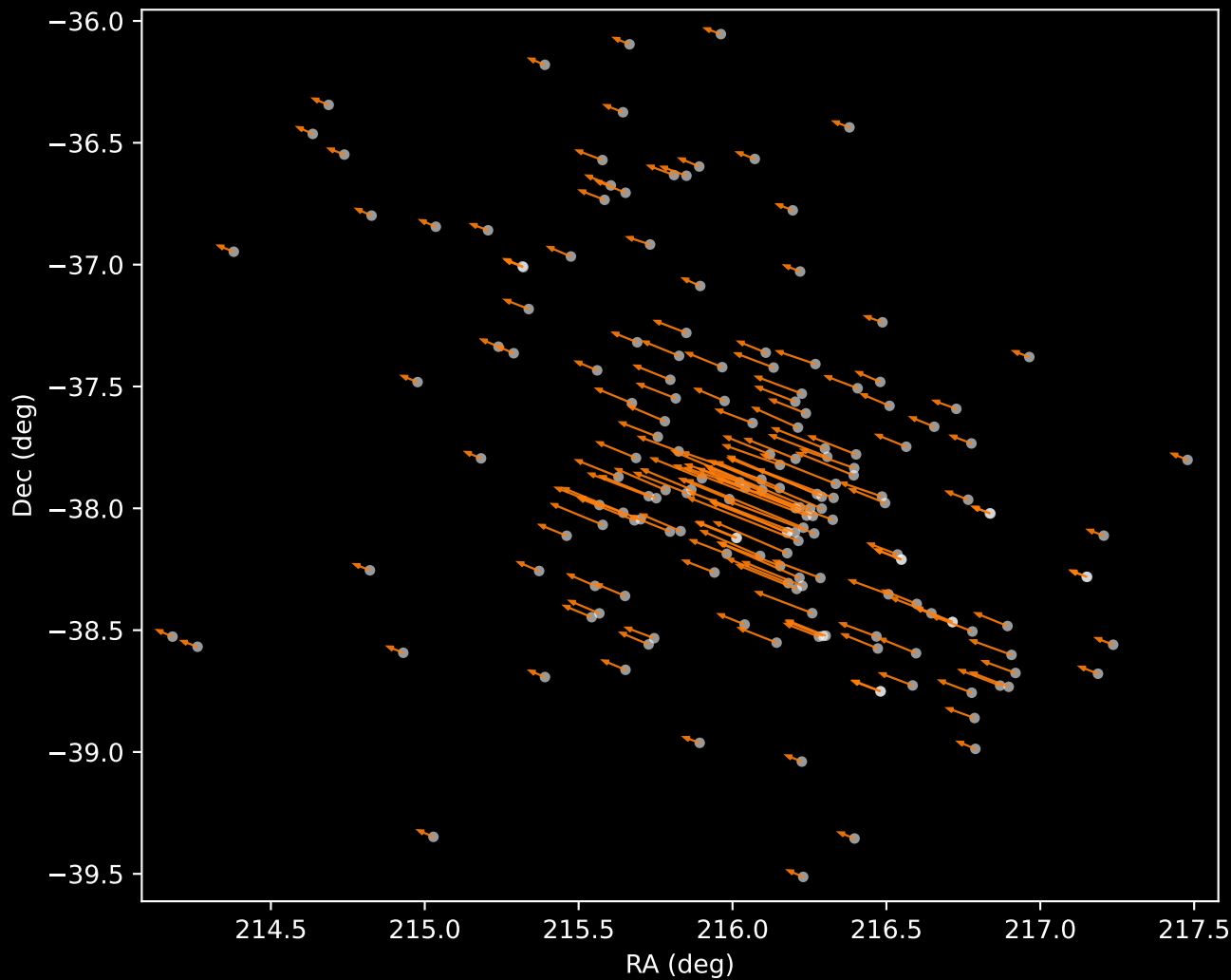
Gaia DR3 Cluster 2 Proper Motion Vectors (n=178)
