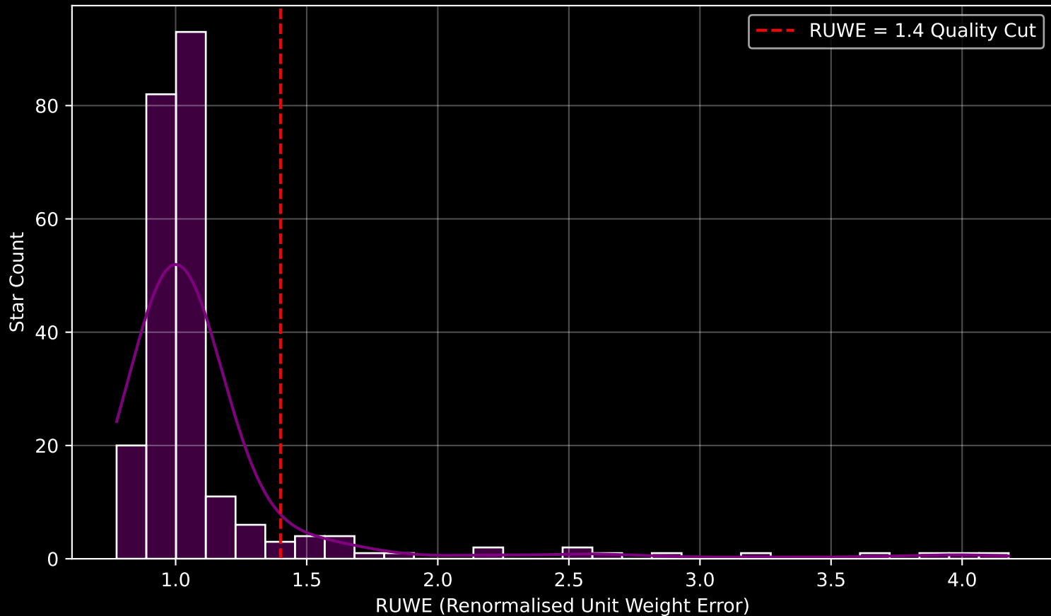
Gaia Cluster: [NGC_2451B] RUWE Distribution (n= 236)
