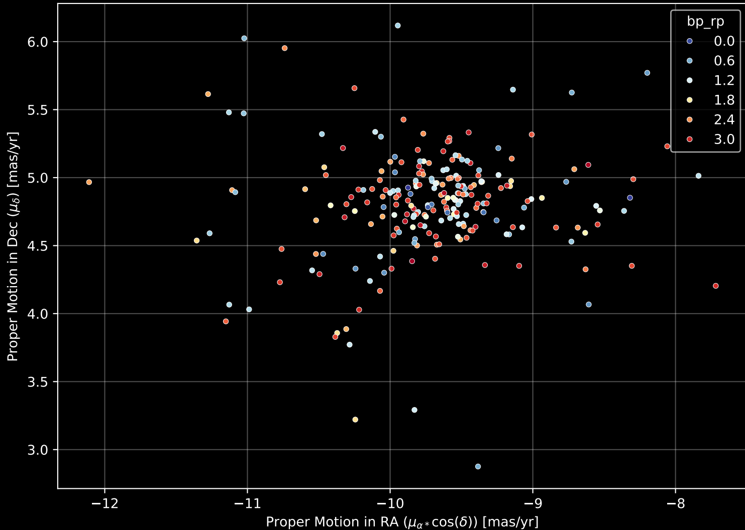
Gaia Cluster: [NGC_2451B] Proper Motion Diagram (n= 236)
