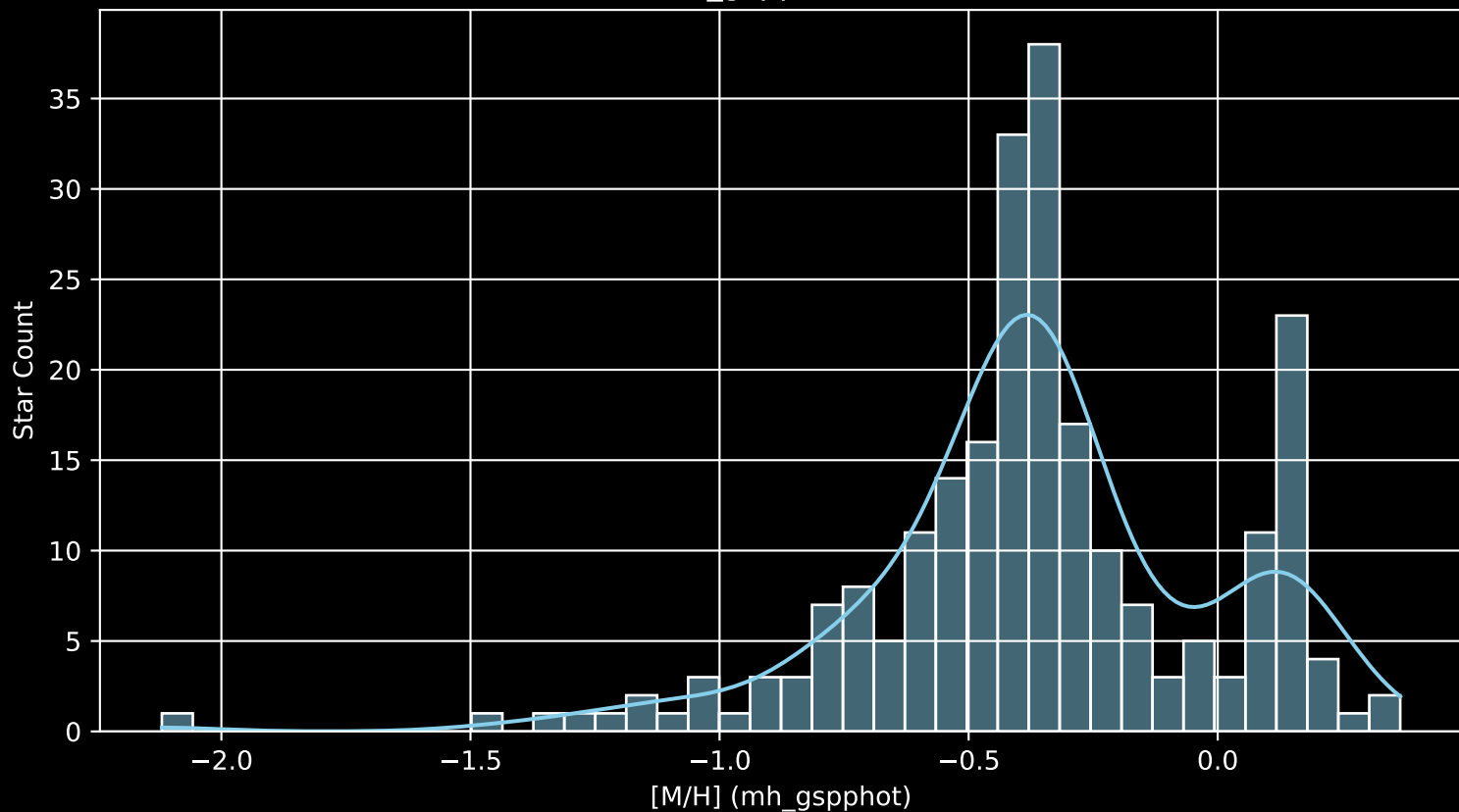
Gaia Cluster: [NGC_2451B [M/H] (mh_gspphot) (n= 236)
