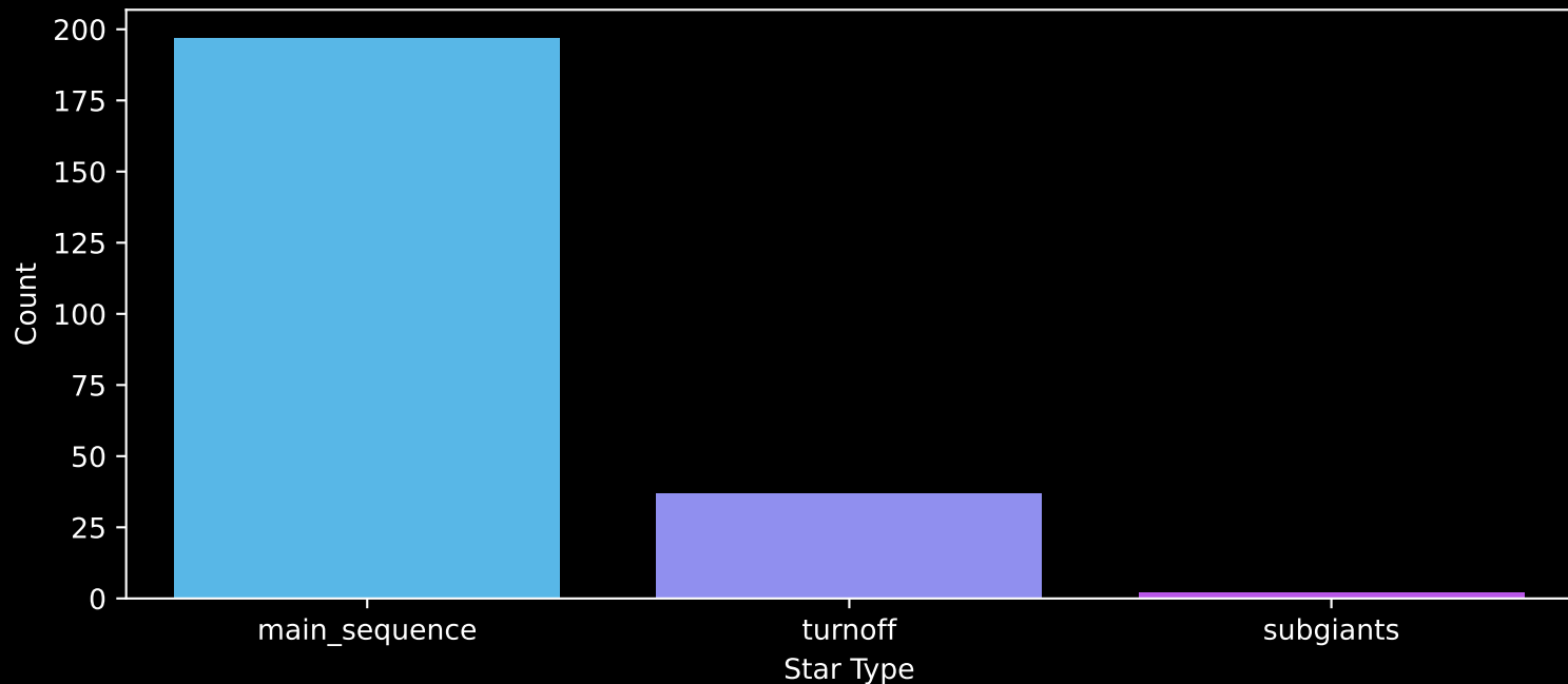
Gaia Cluster: [NGC_2451B] Count plot of Star Type
