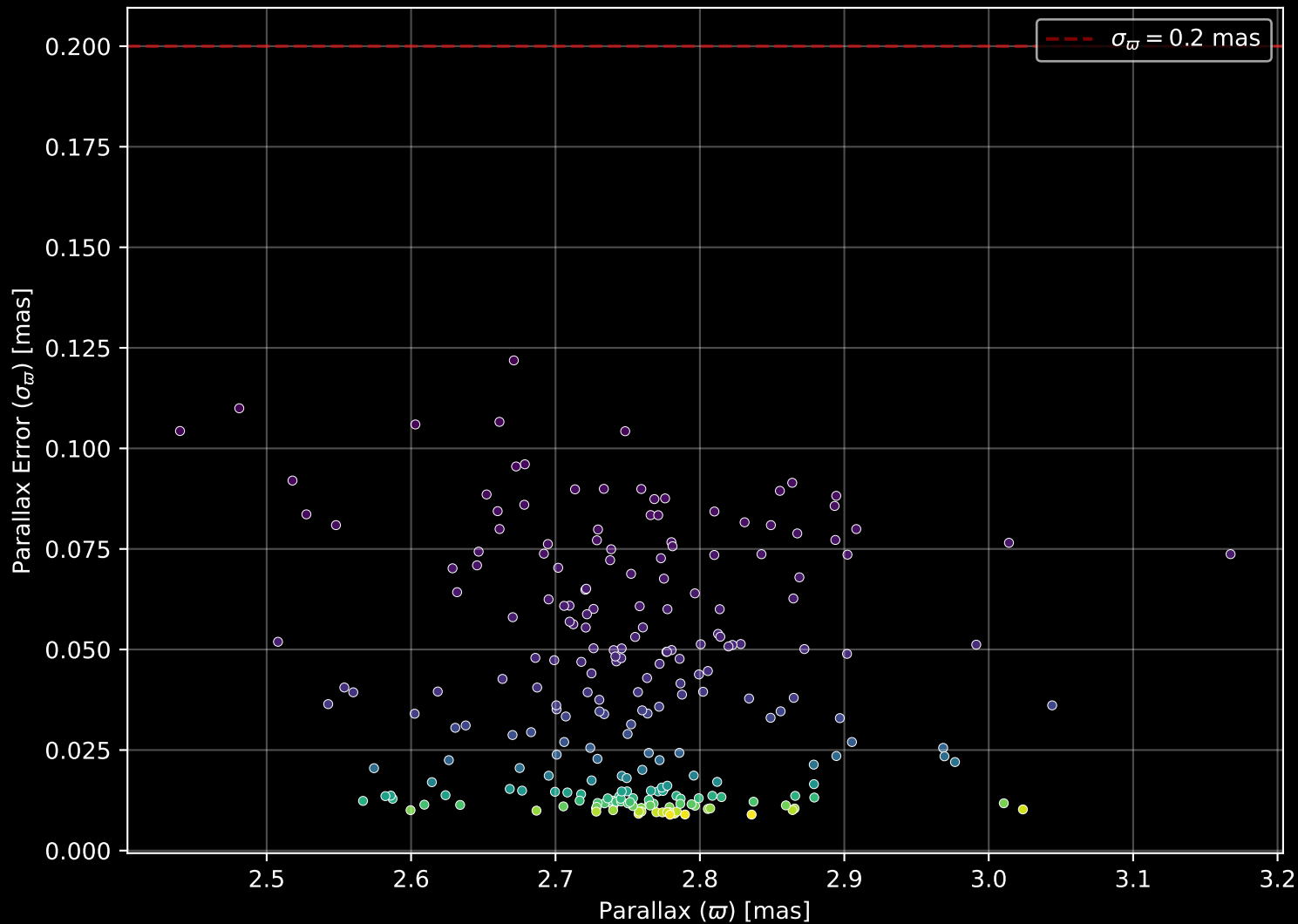
Gaia Cluster: [NGC_2451B] Parallax Quality (n= 236)
