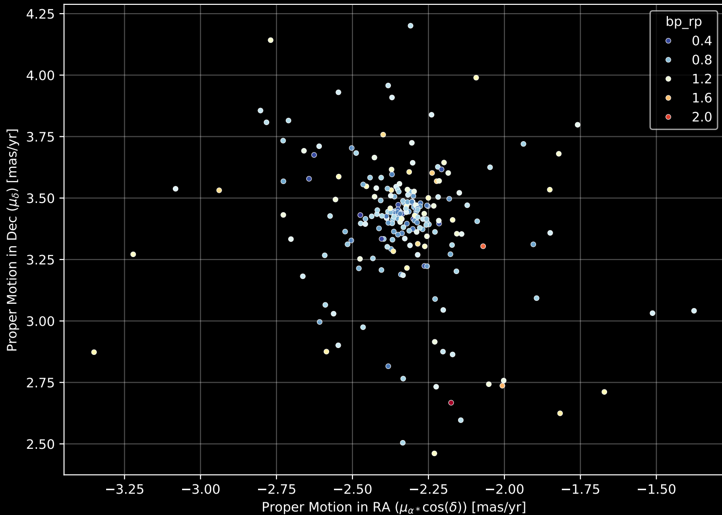
Gaia Cluster: [NGC_2453] Proper Motion Diagram (n= 220)
