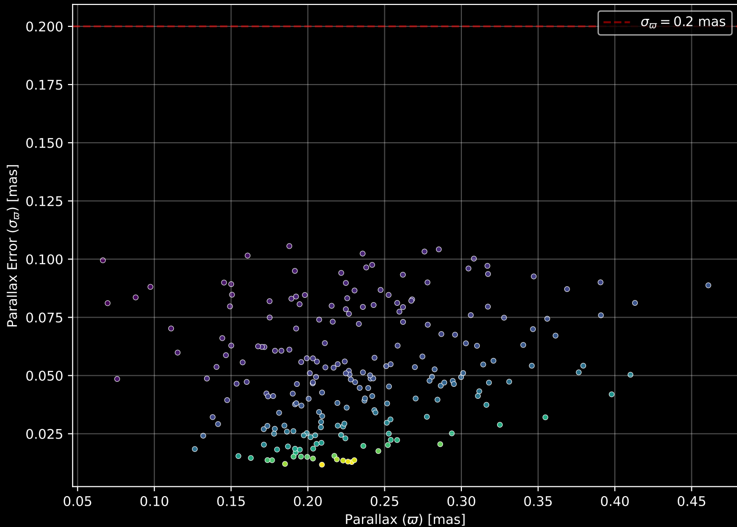
Gaia Cluster: [NGC_2453] Parallax Quality (n= 220)
