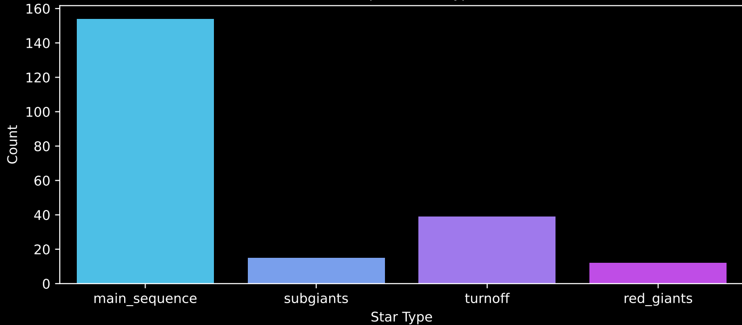
Gaia Cluster: [NGC_2453] Count plot of Star Type
