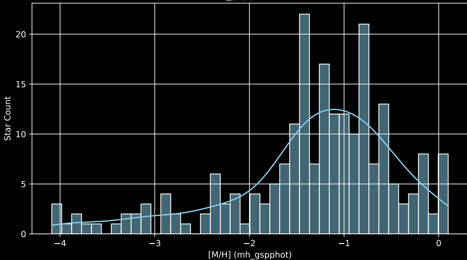
Gaia Cluster: [NGC_2453 [M/H] (mh_gspphot) (n= 220)
