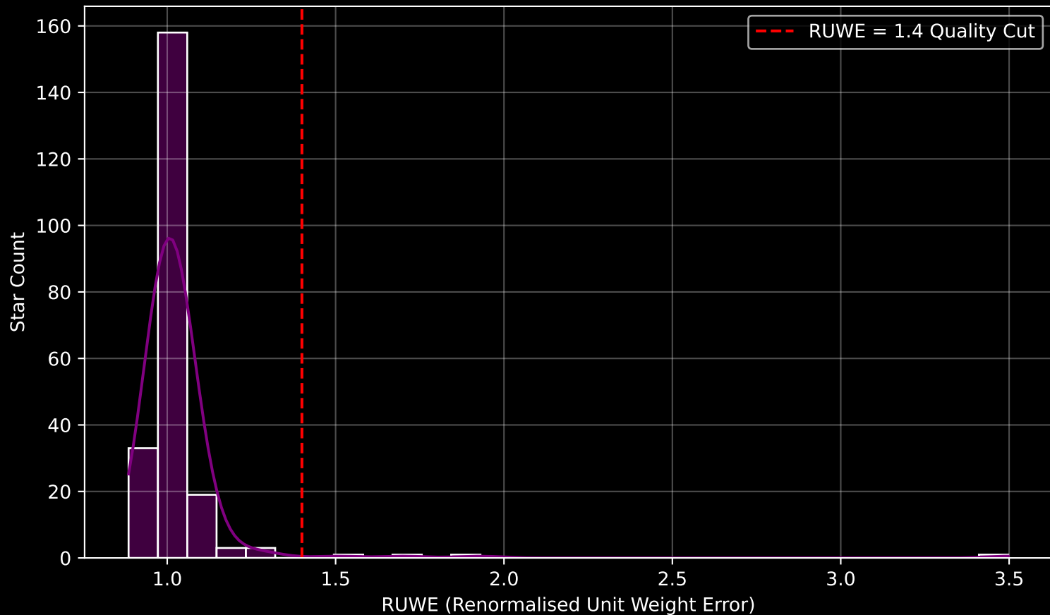
Gaia Cluster: [NGC_2453] RUWE Distribution (n= 220)
