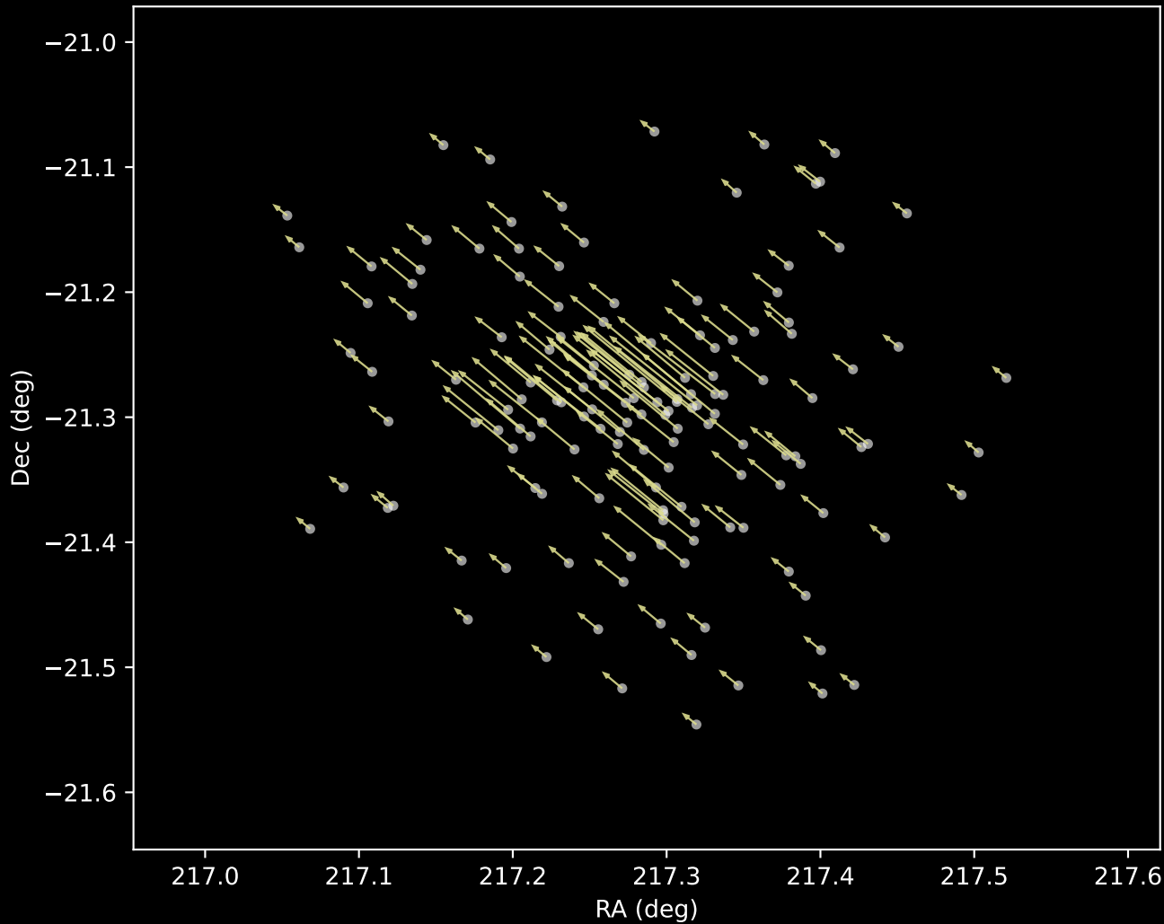
Gaia DR3 Cluster 17 Proper Motion Vectors (n=145)
