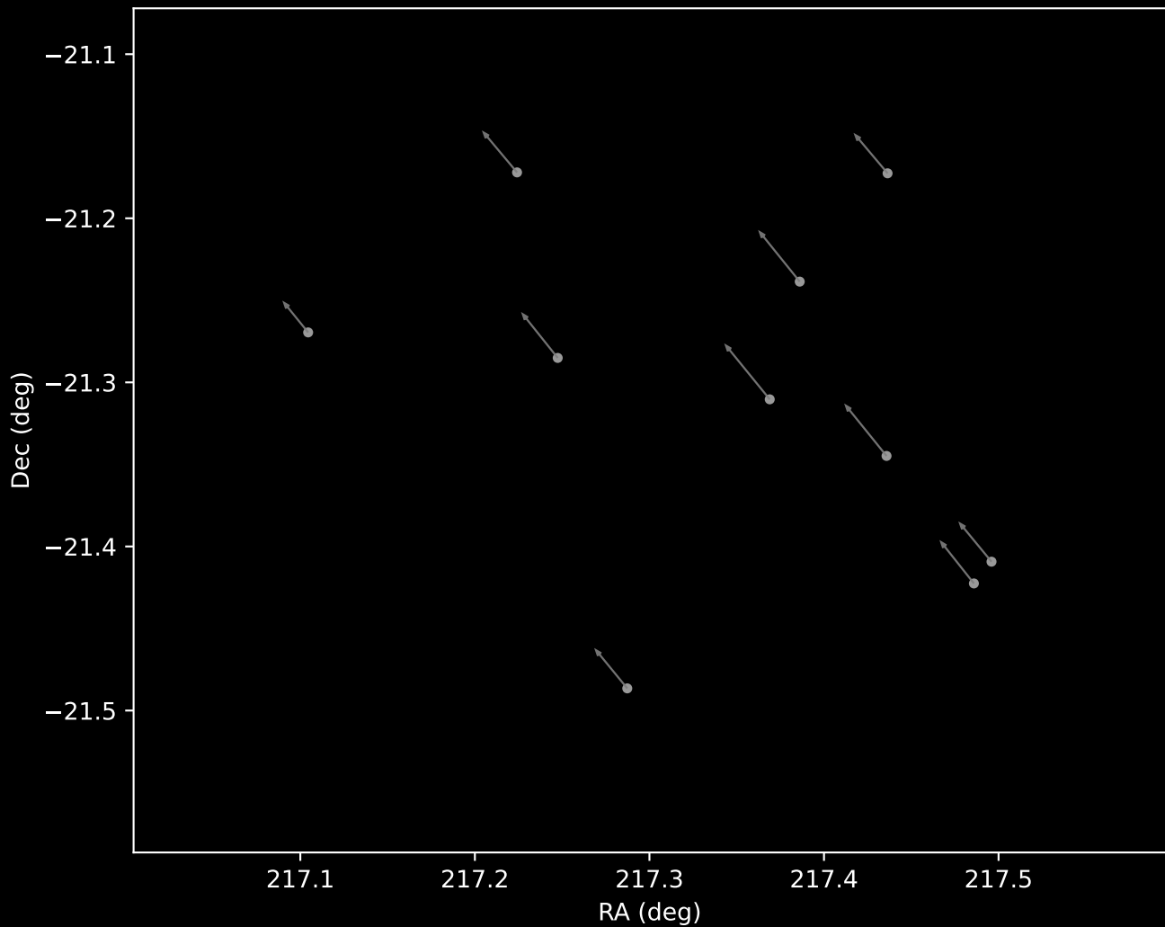
Gaia DR3 Cluster 14 Proper Motion Vectors (n=10)
