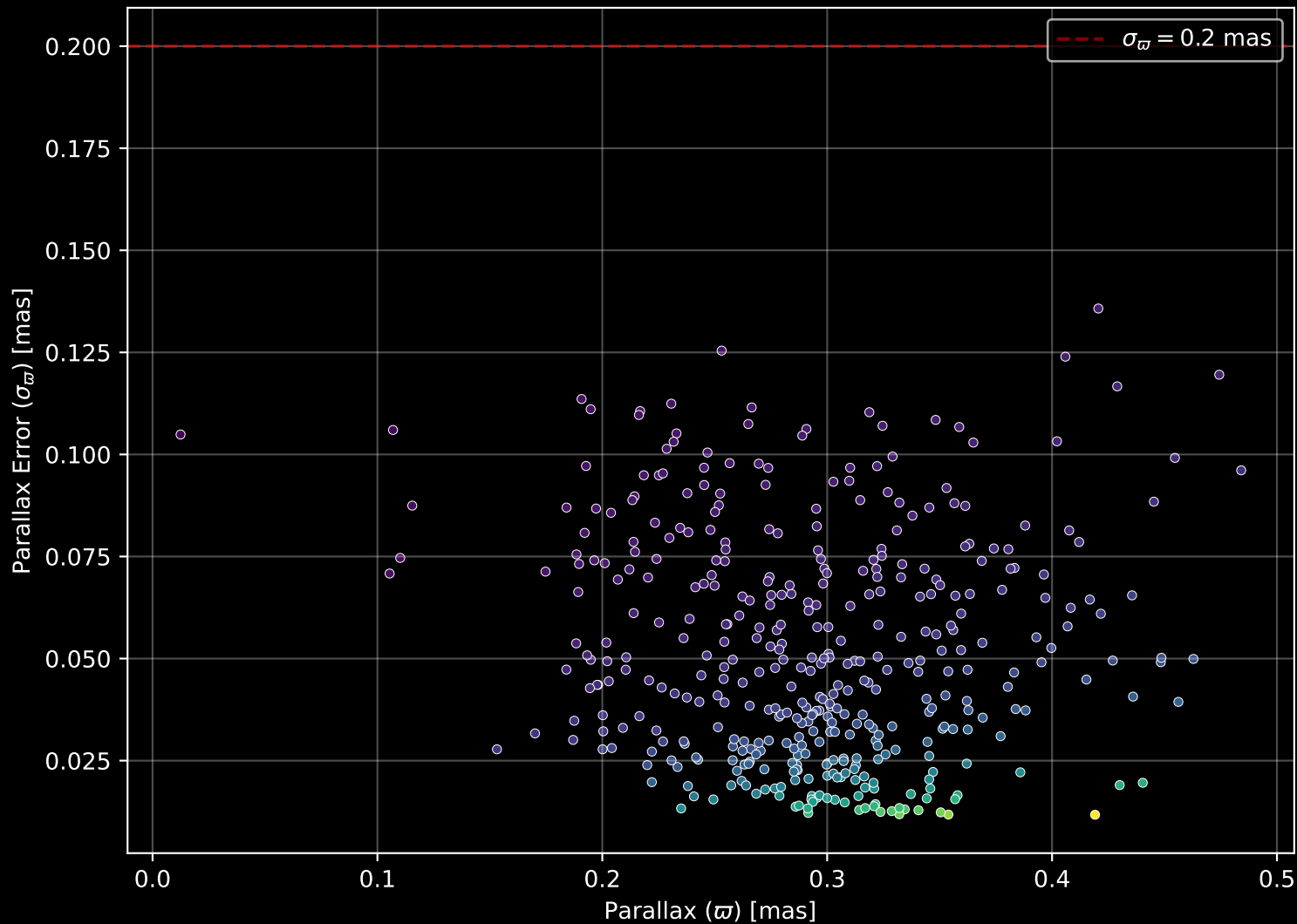
Gaia Cluster: [NGC_2455] Parallax Quality (n= 412)
