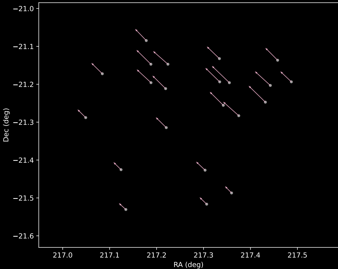
Gaia DR3 Cluster 13 Proper Motion Vectors (n=22)
