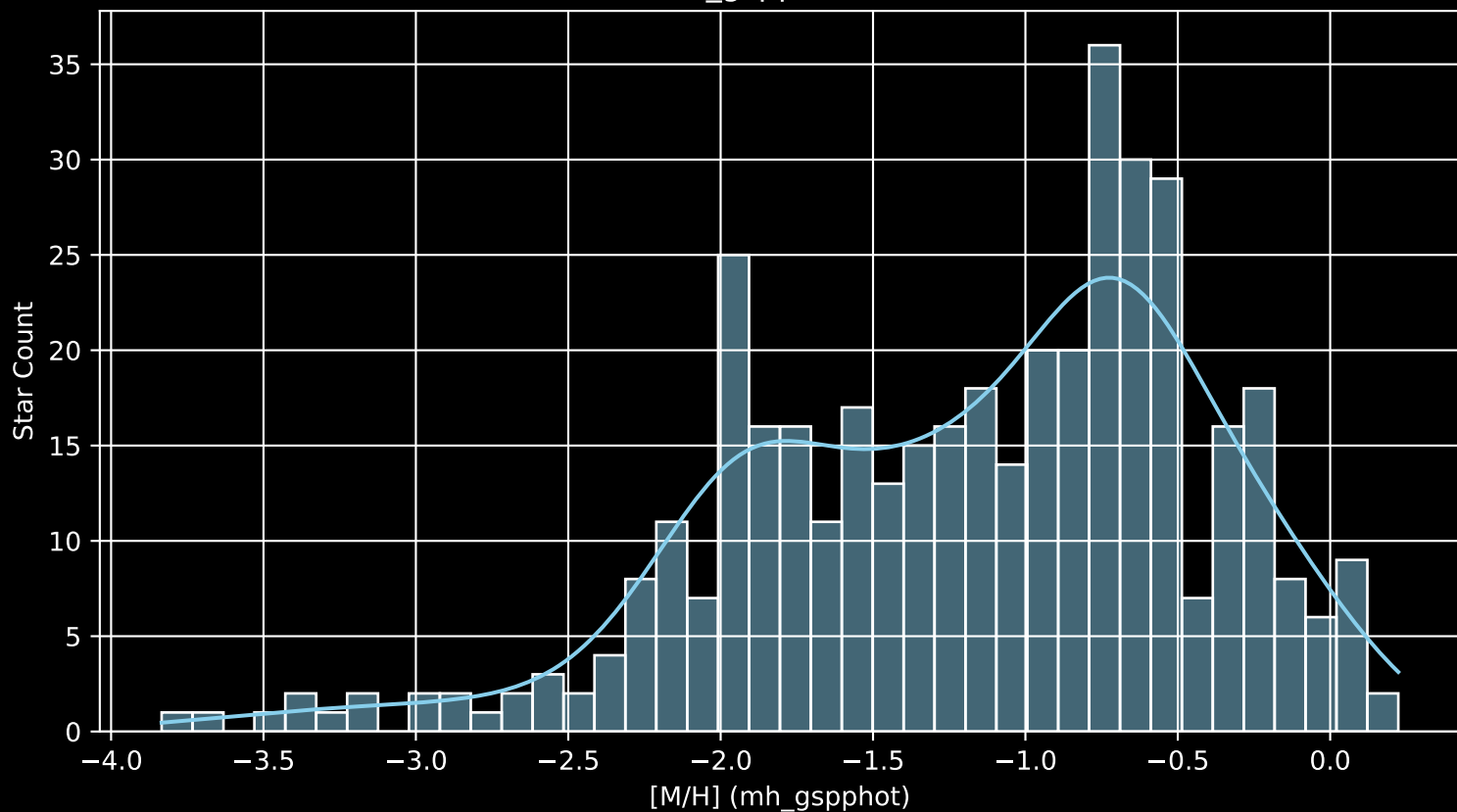
Gaia Cluster: [NGC_2455 [M/H] (mh_gspphot) (n= 412)
