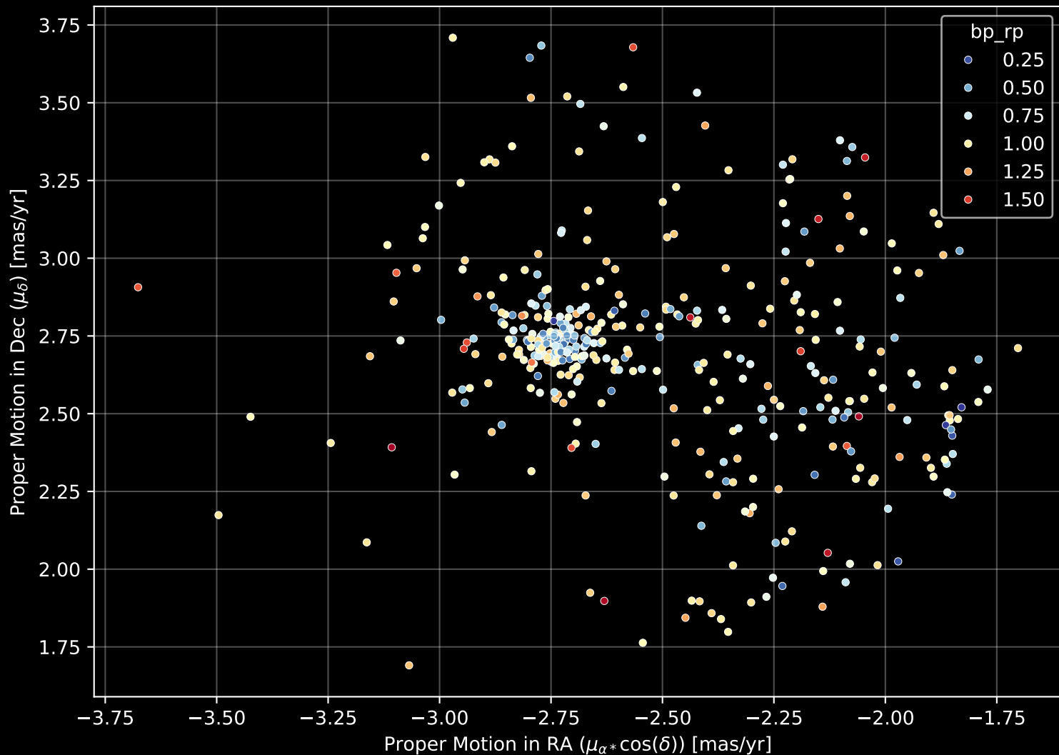
Gaia Cluster: [NGC_2455] Proper Motion Diagram (n= 412)
