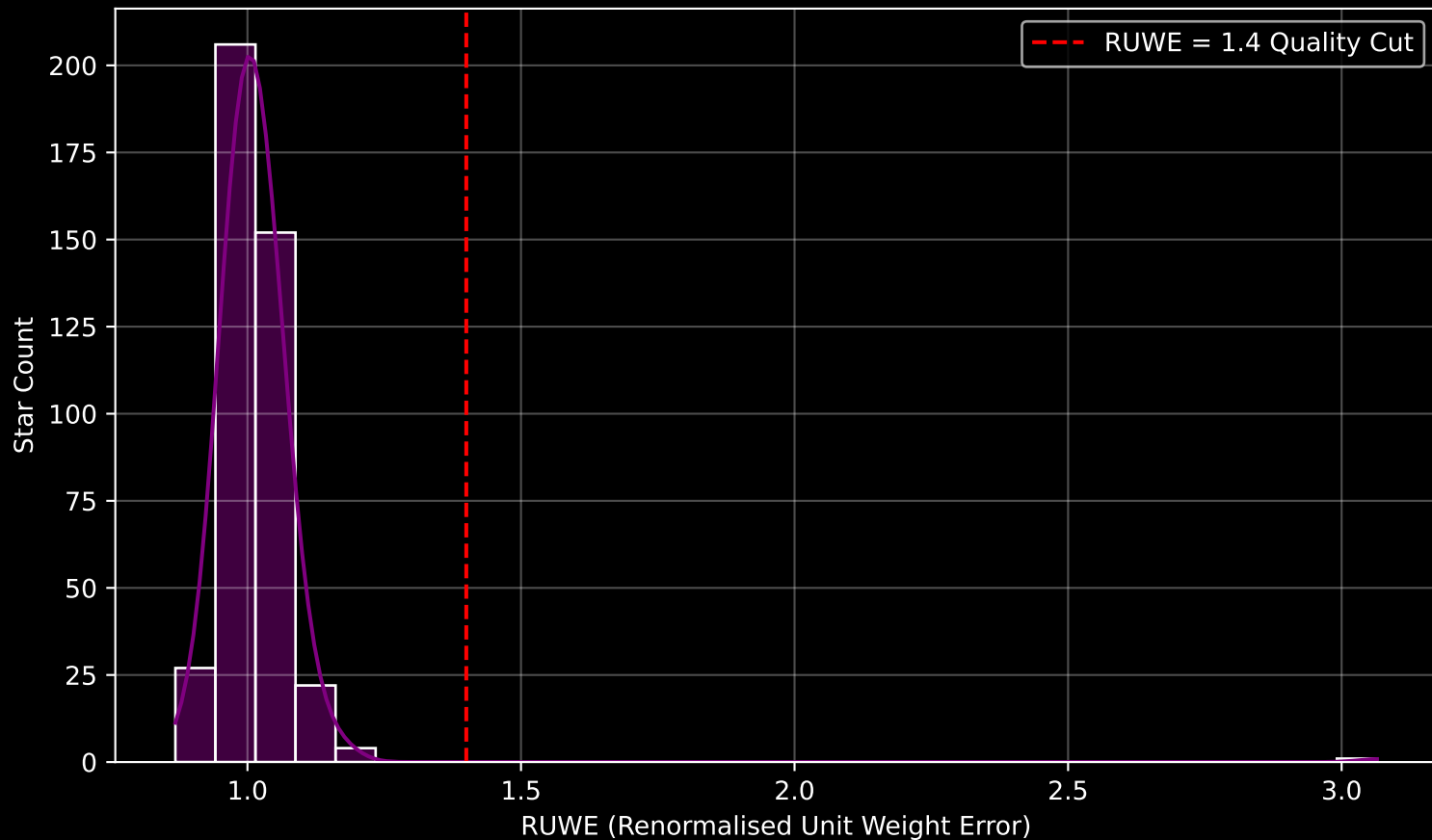
Gaia Cluster: [NGC_2455] RUWE Distribution (n= 412)
