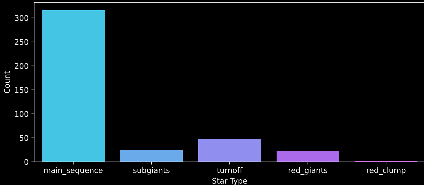
Gaia Cluster: [NGC_2455] Count plot of Star Type
