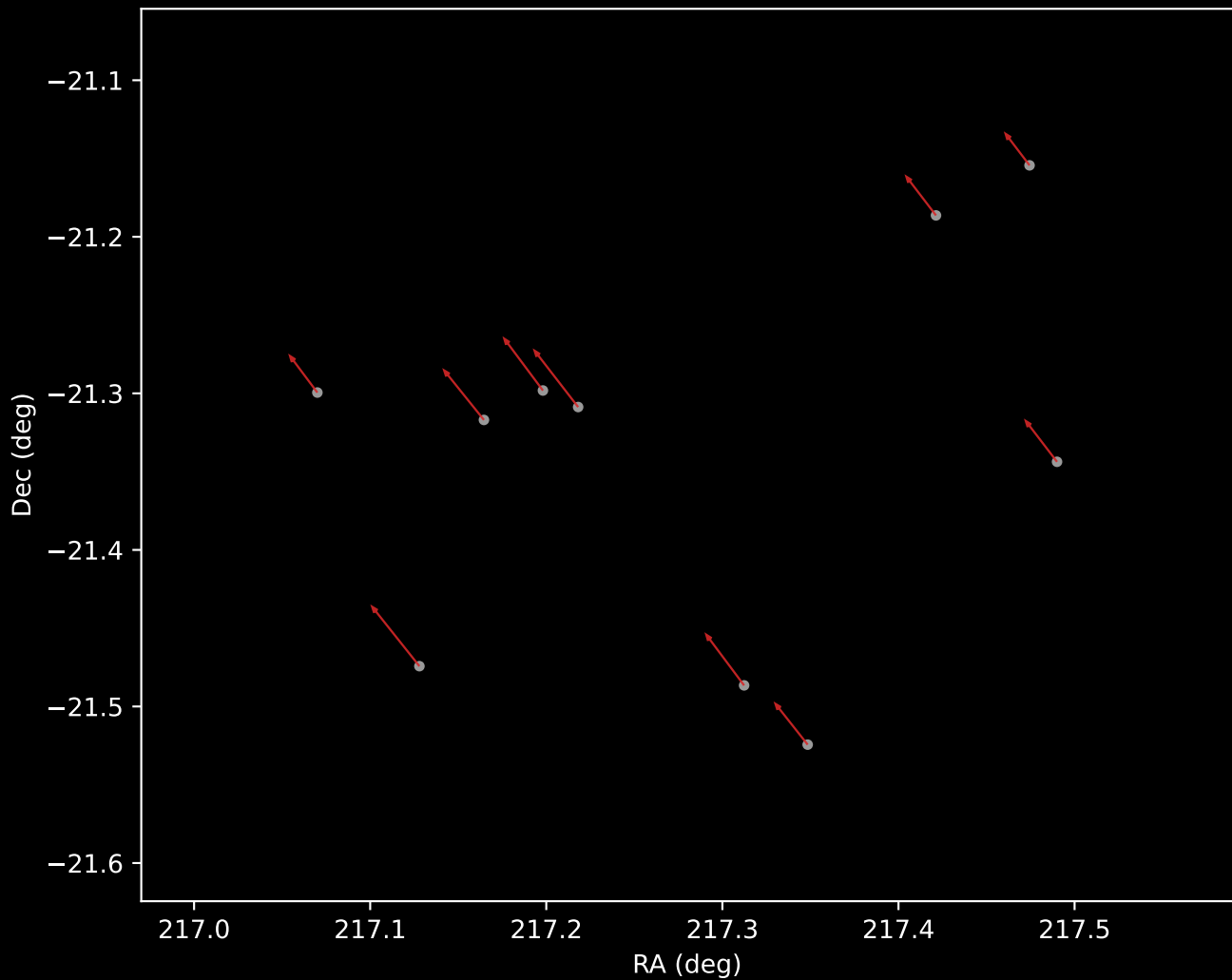
Gaia DR3 Cluster 6 Proper Motion Vectors (n=10)
