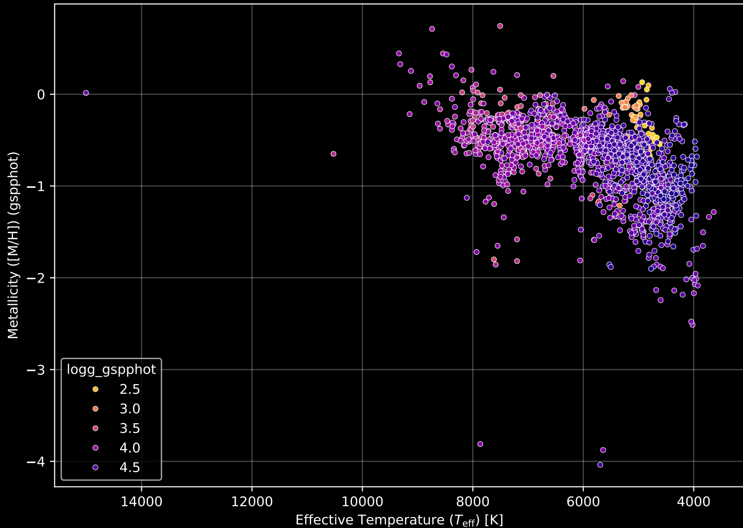
Gaia Cluster: [NGC_2477] Stellar Population Parameters (n= 1825)
