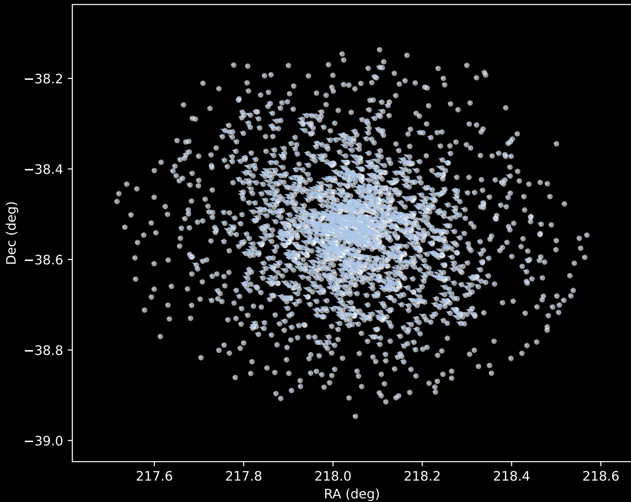
Gaia DR3 Cluster 1 Proper Motion Vectors (n=1801)
