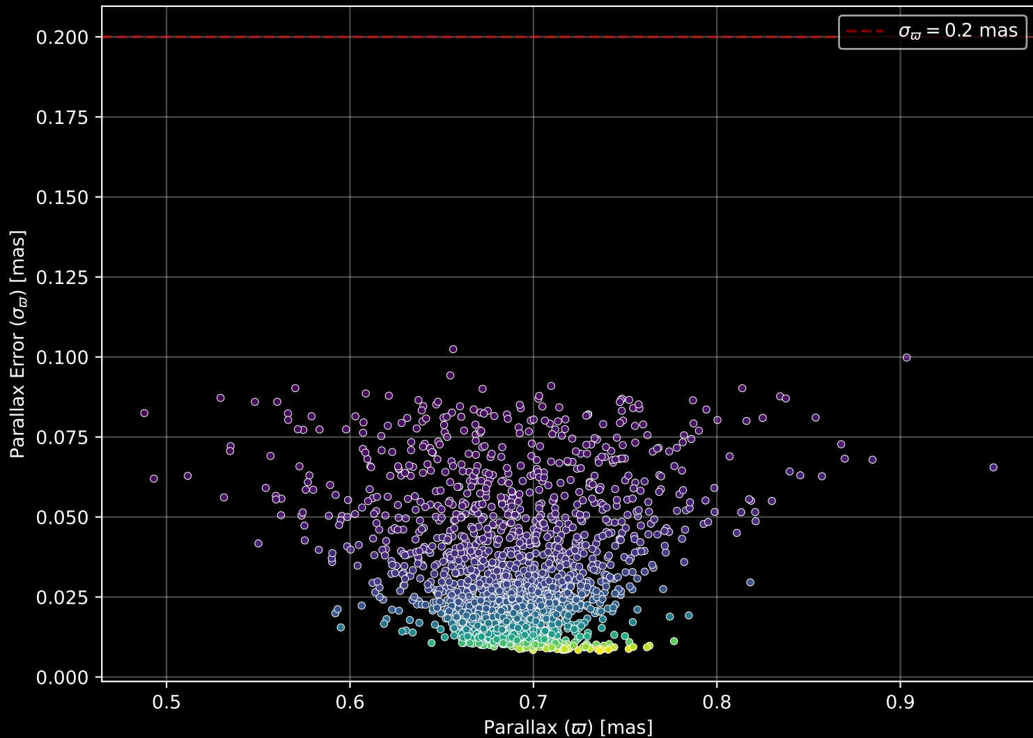
Gaia Cluster: [NGC_2477] Parallax Quality (n= 1825)
