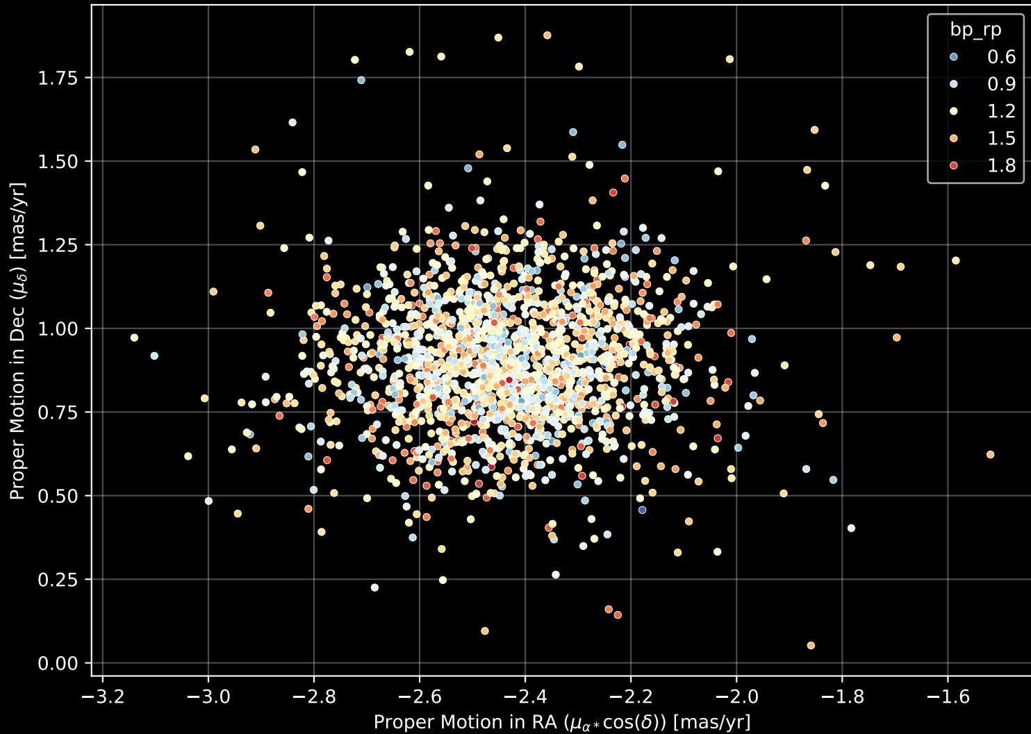
Gaia Cluster: [NGC_2477] Proper Motion Diagram (n= 1825)
