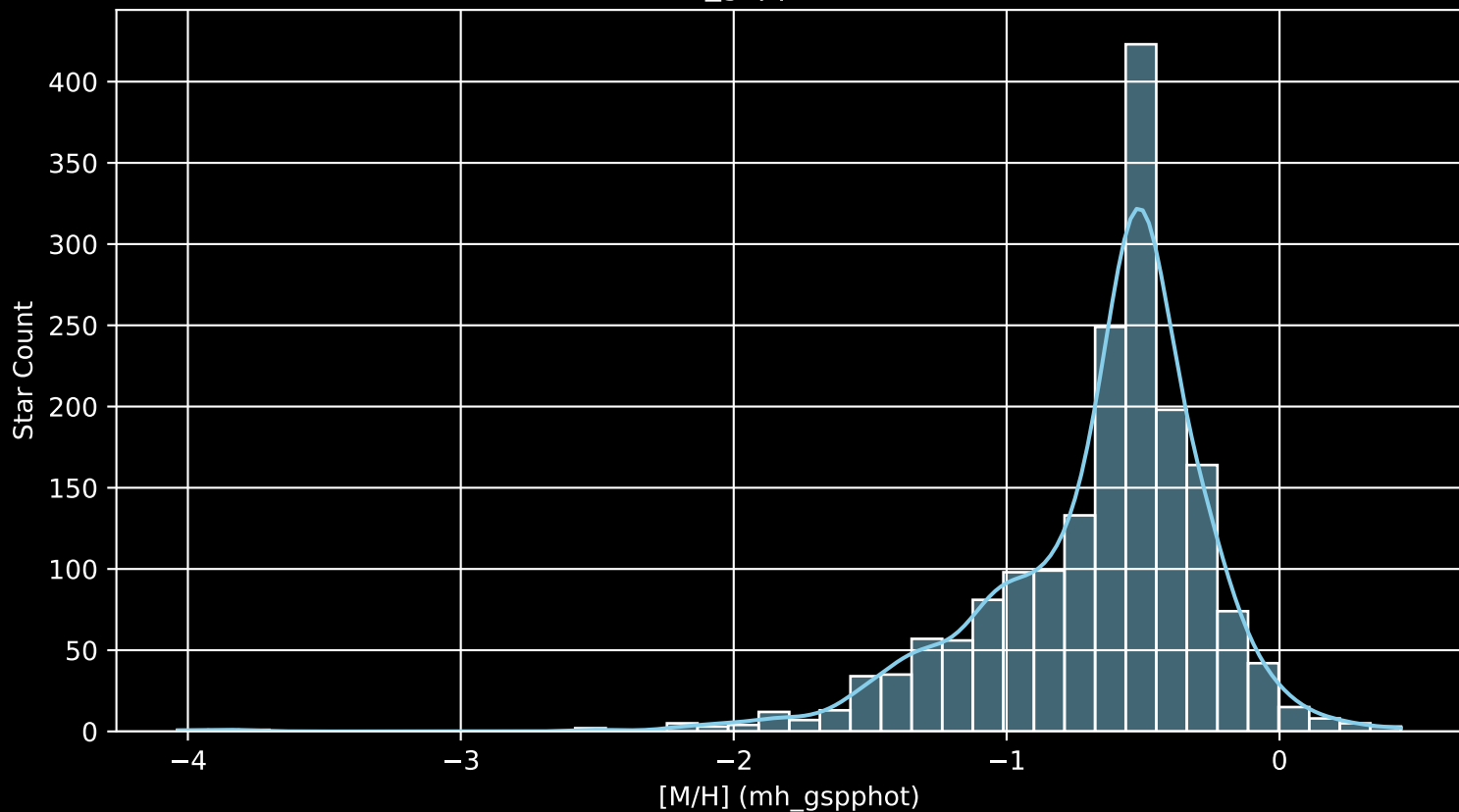
Gaia Cluster: [NGC_2477 [M/H] (mh_gspphot) (n= 1823)
