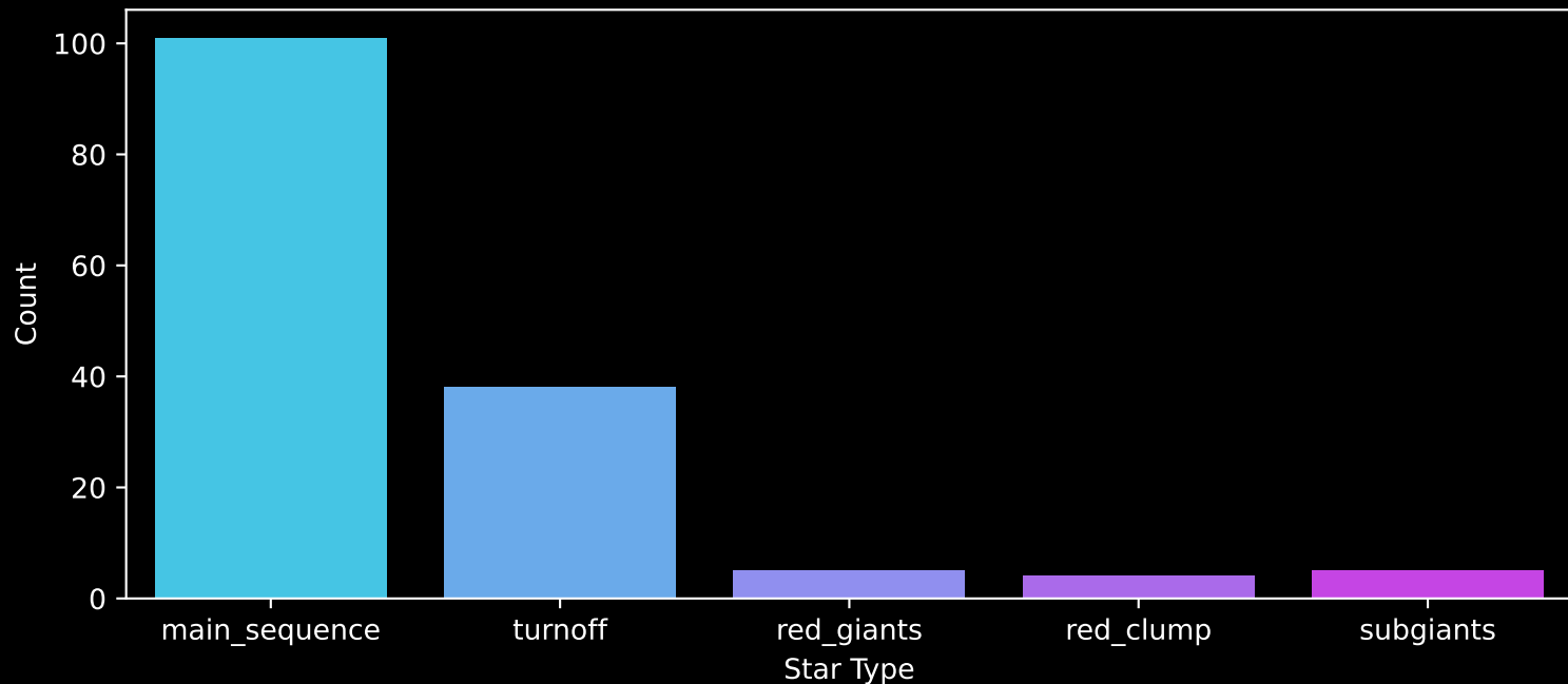
Gaia Cluster: [NGC_2479] Count plot of Star Type
