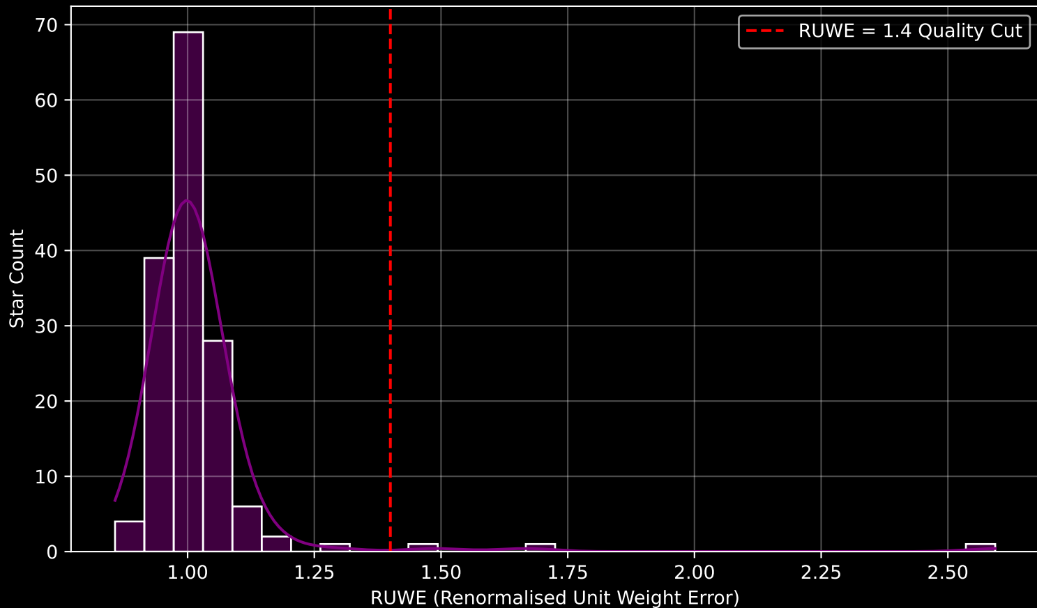
Gaia Cluster: [NGC_2479] RUWE Distribution (n= 152)
