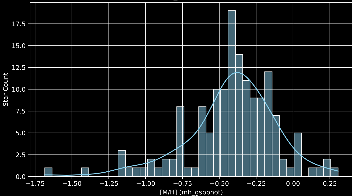
Gaia Cluster: [NGC_2479 [M/H] (mh_gspphot) (n= 152)
