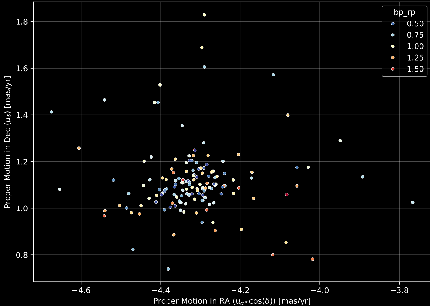
Gaia Cluster: [NGC_2479] Proper Motion Diagram (n= 153)
