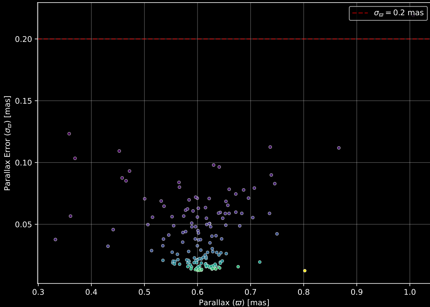
Gaia Cluster: [NGC_2479] Parallax Quality (n= 153)
