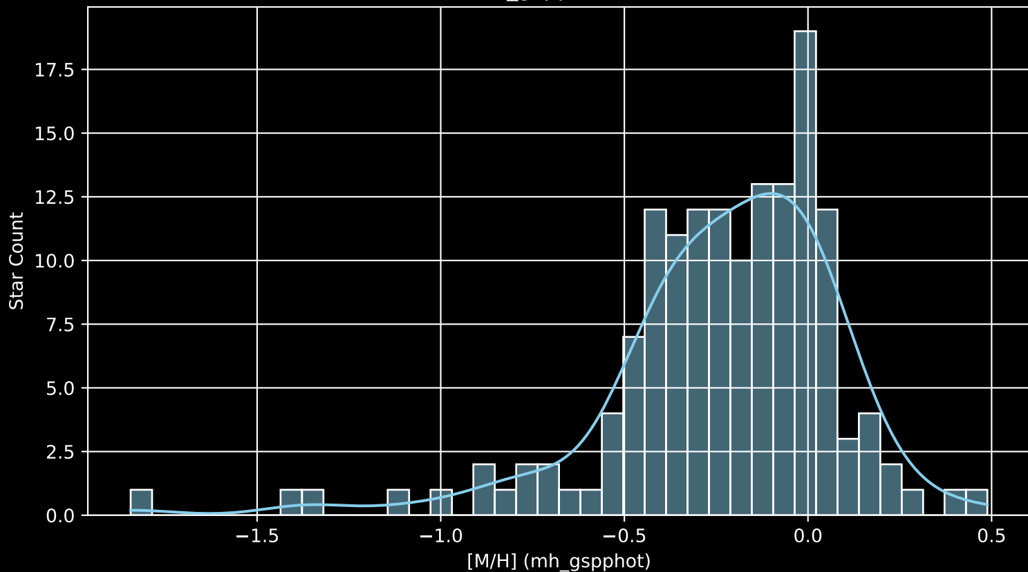
Gaia Cluster: [NGC_2482 [M/H] (mh_gspphot) (n= 151)
