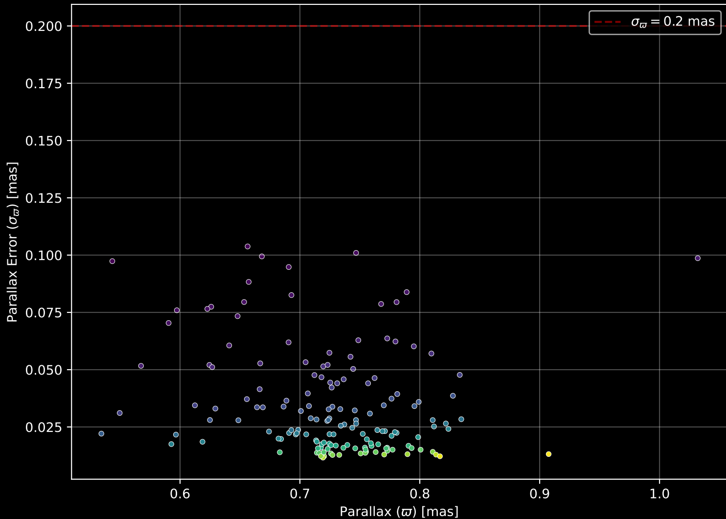
Gaia Cluster: [NGC_2482] Parallax Quality (n= 152)
