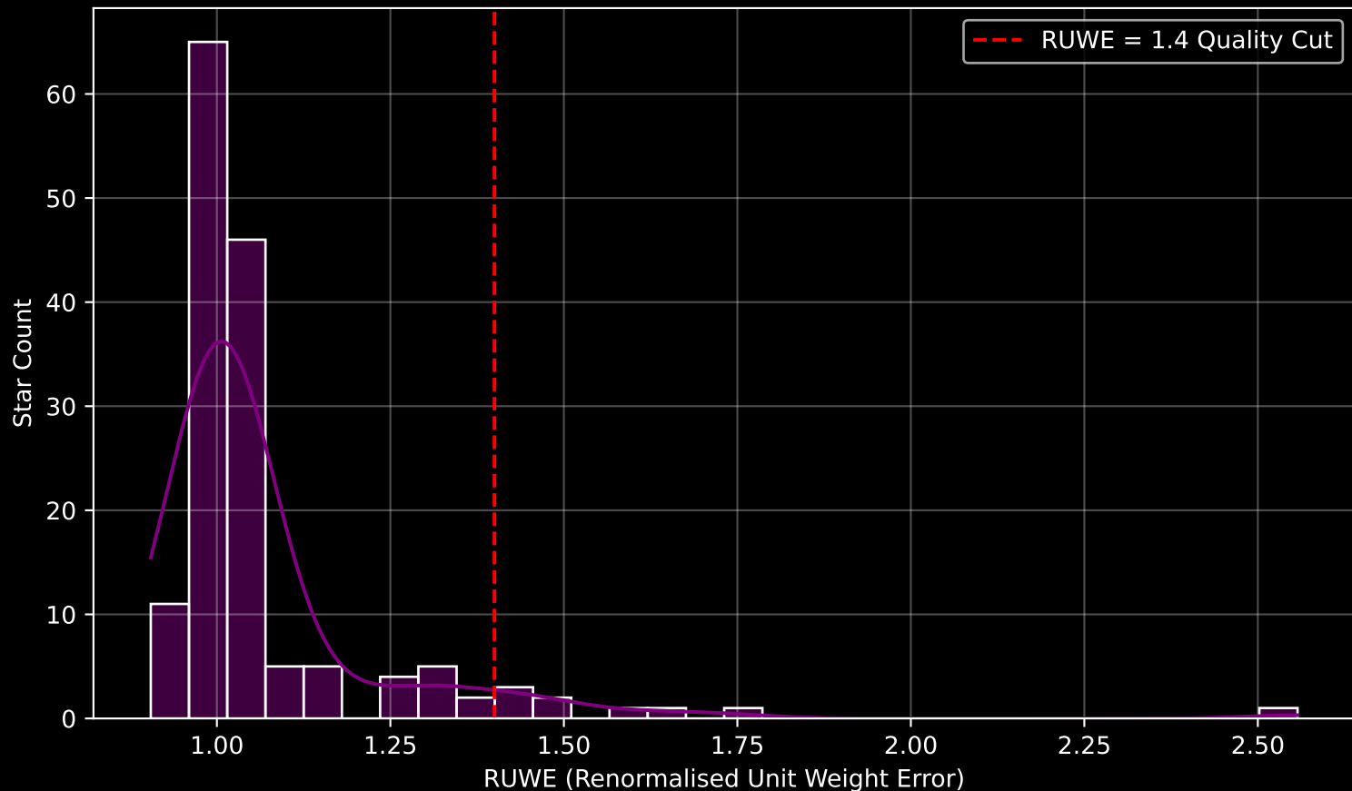
Gaia Cluster: [NGC_2482] RUWE Distribution (n= 152)
