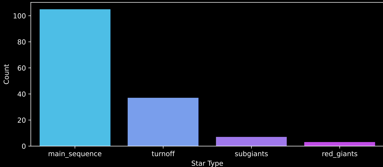
Gaia Cluster: [NGC_2482] Count plot of Star Type
