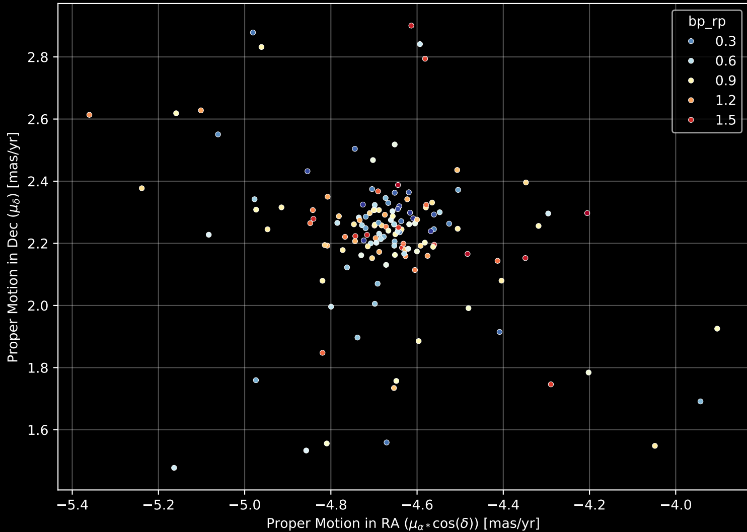
Gaia Cluster: [NGC_2482] Proper Motion Diagram (n= 152)
