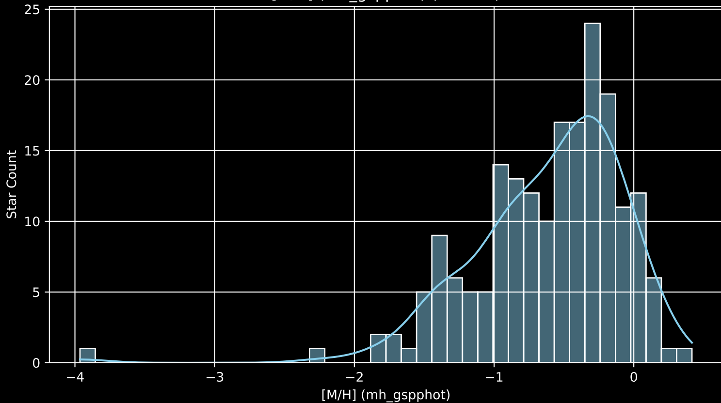
Gaia Cluster: [NGC_2571 [M/H] (mh_gspphot) (n= 194)
