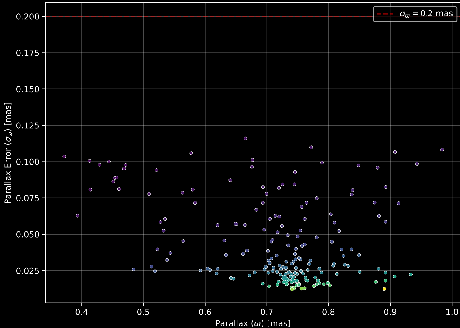
Gaia Cluster: [NGC_2571] Parallax Quality (n= 194)
