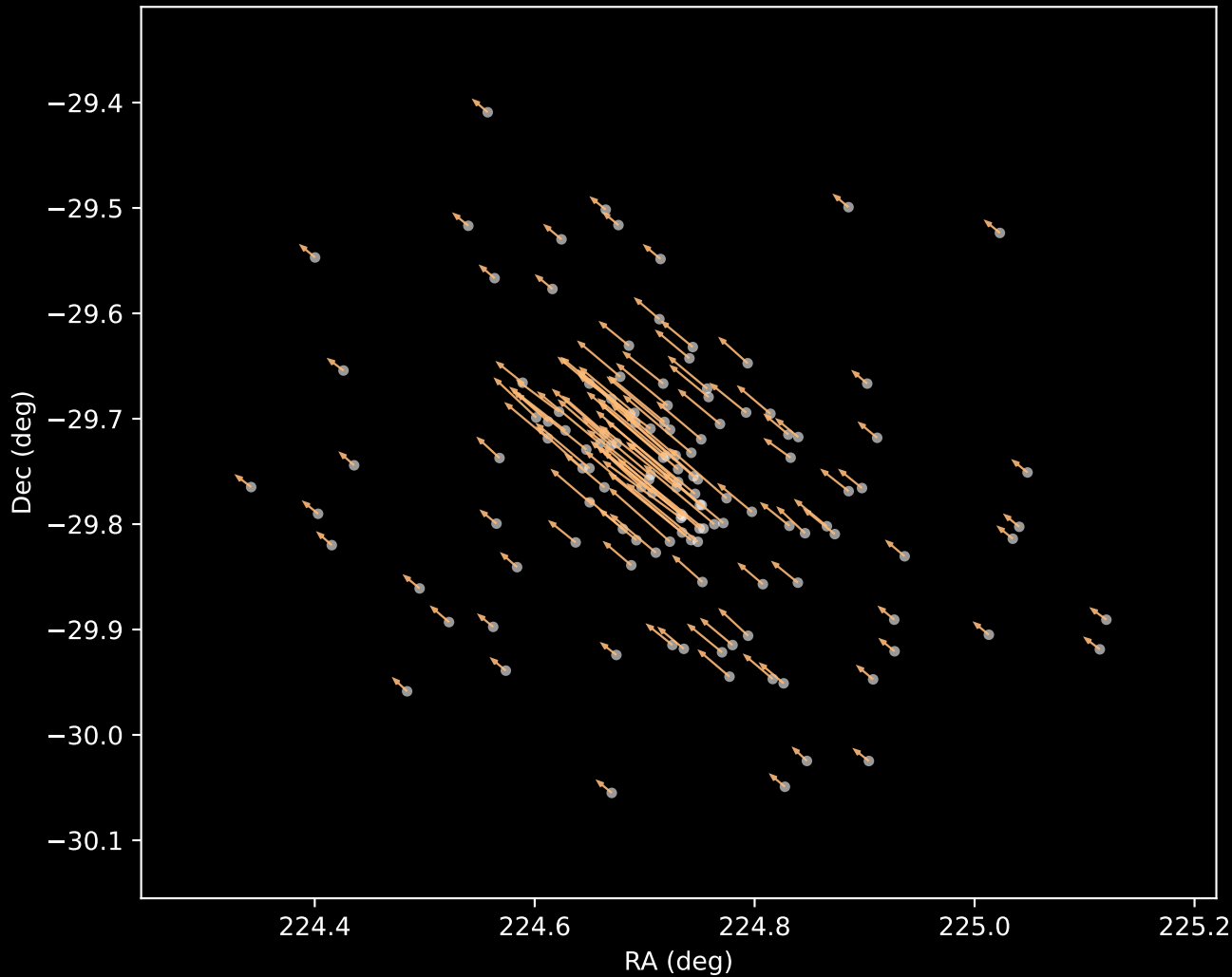
Gaia DR3 Cluster 3 Proper Motion Vectors (n=132)
