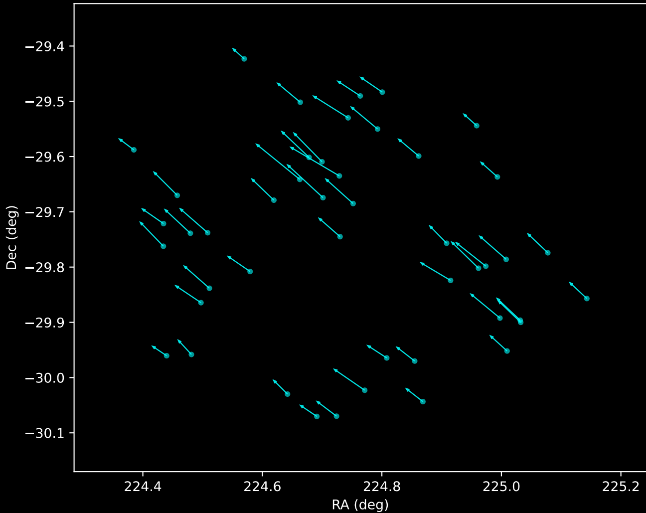
Gaia DR3 Noise Stream Proper Motion Vectors (n=46)
