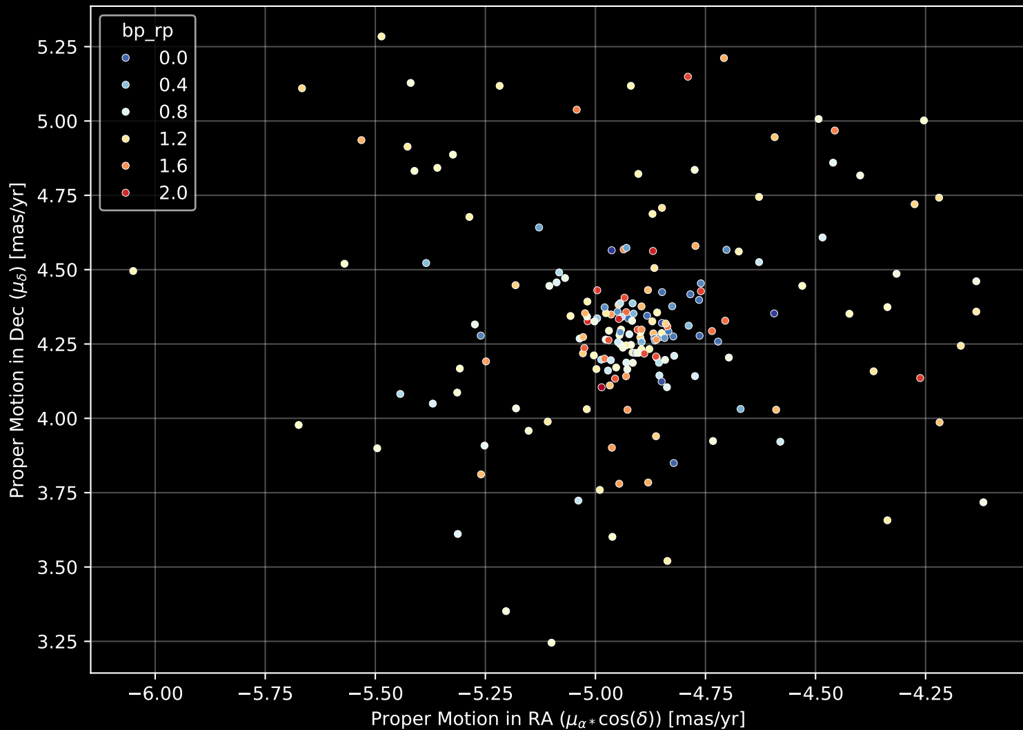
Gaia Cluster: [NGC_2571] Proper Motion Diagram (n= 194)
