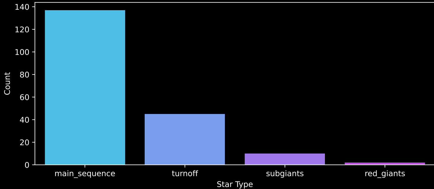
Gaia Cluster: [NGC_2571] Count plot of Star Type
