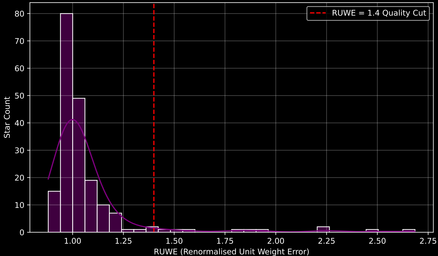
Gaia Cluster: [NGC_2571] RUWE Distribution (n= 194)
