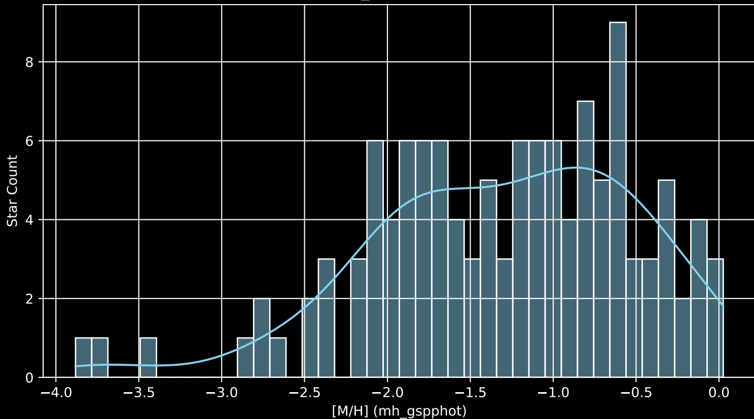
Gaia Cluster: [NGC_2588 [M/H] (mh_gspphot) (n= 121)
