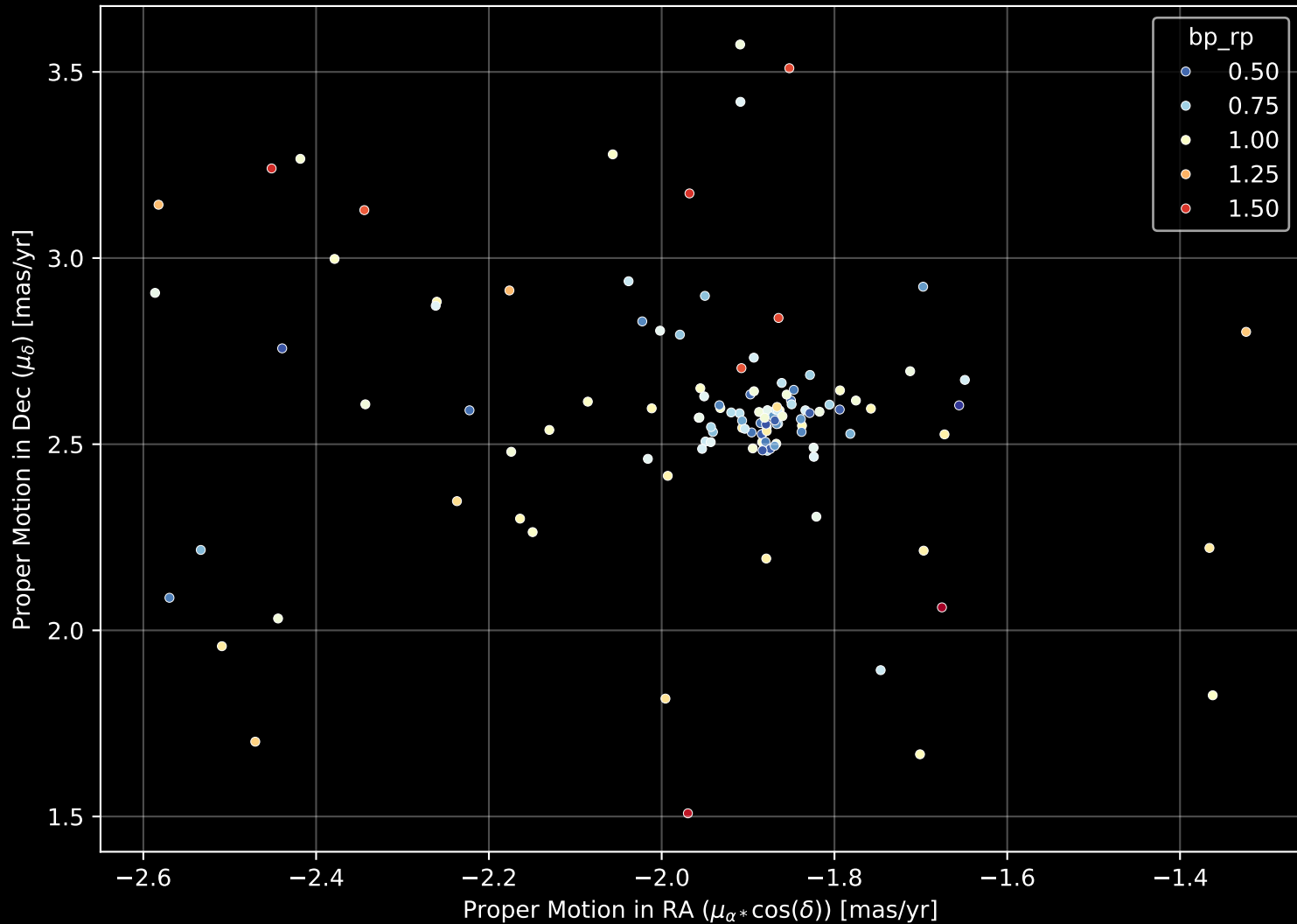
Gaia Cluster: [NGC_2588] Proper Motion Diagram (n= 121)
