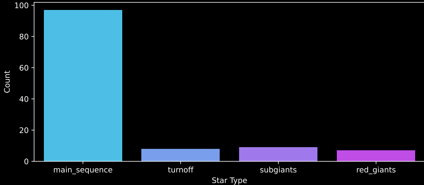
Gaia Cluster: [NGC_2588] Count plot of Star Type
