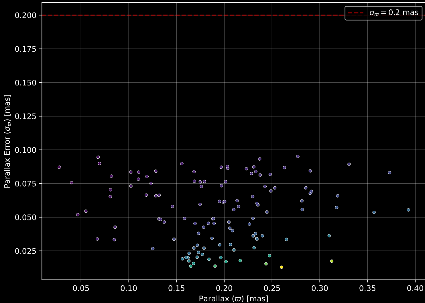
Gaia Cluster: [NGC_2588] Parallax Quality (n= 121)
