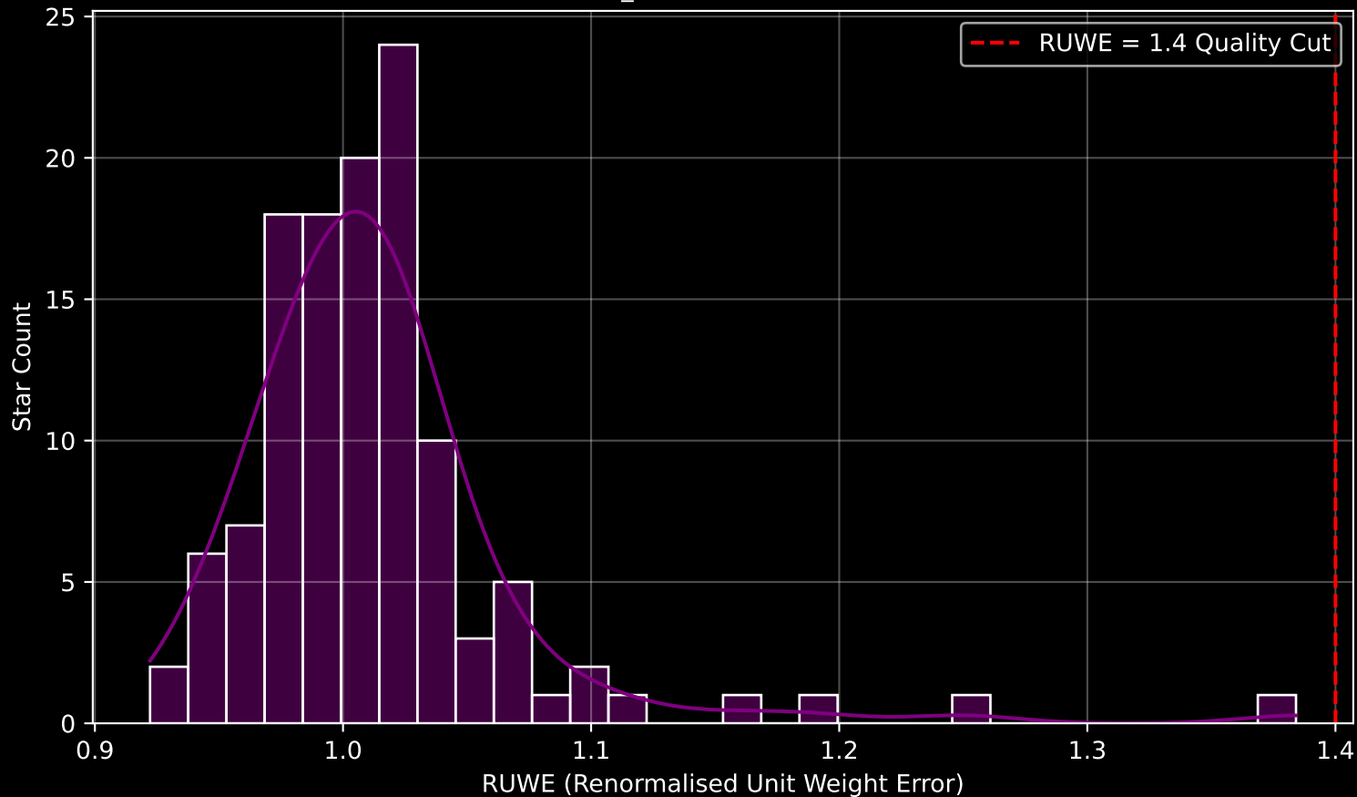
Gaia Cluster: [NGC_2588] RUWE Distribution (n= 121)
