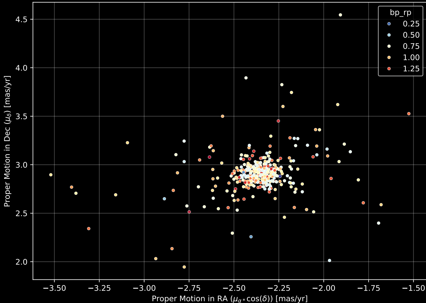
Gaia Cluster: [NGC_2627] Proper Motion Diagram (n= 384)
