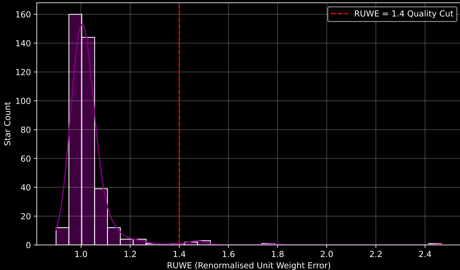
Gaia Cluster: [NGC_2627] RUWE Distribution (n= 384)
