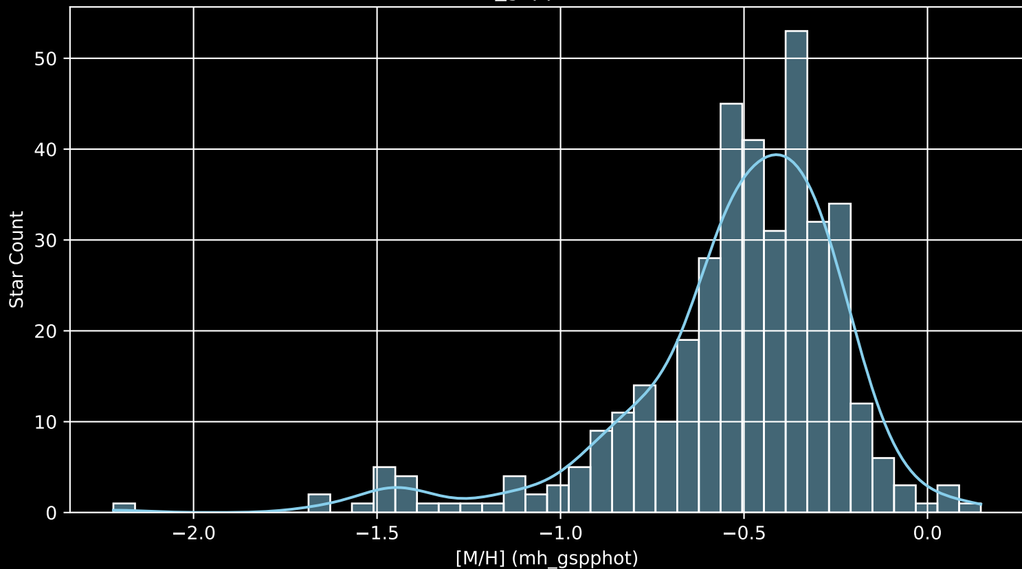
Gaia Cluster: [NGC_2627 [M/H] (mh_gspphot) (n= 384)
