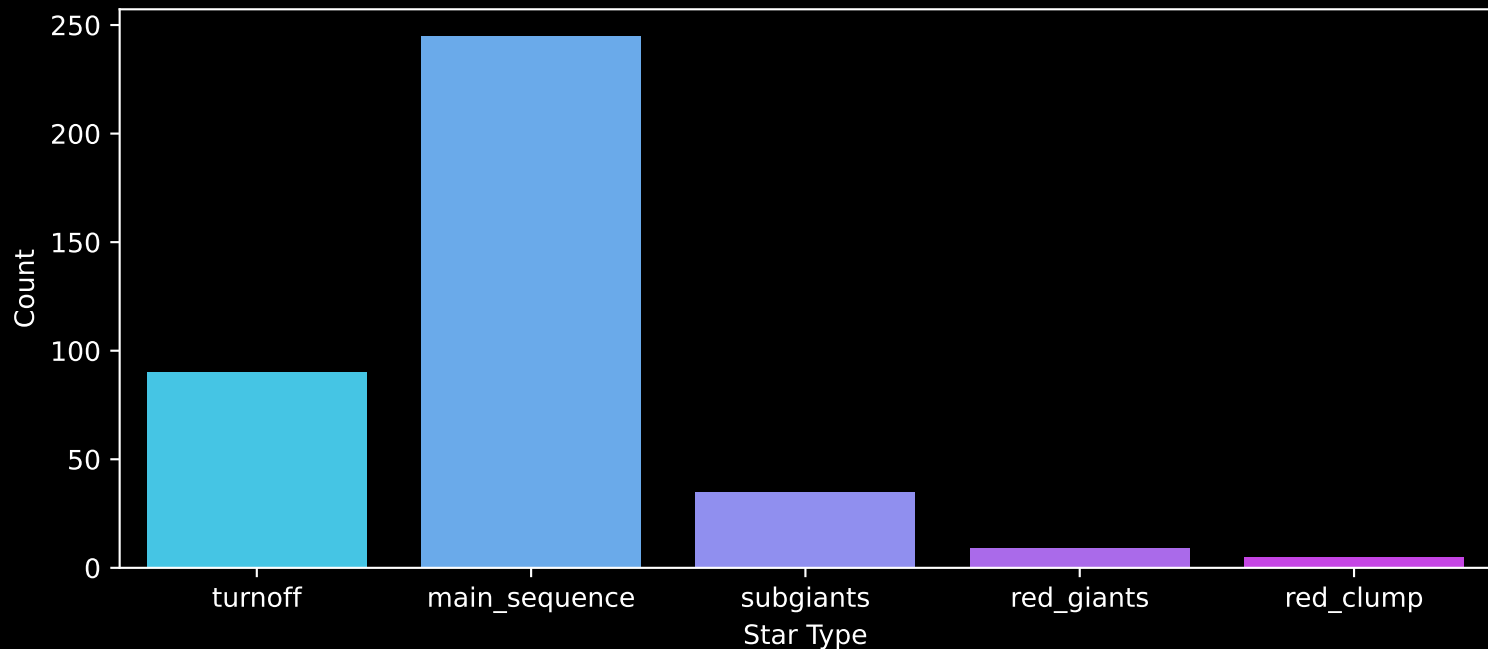
Gaia Cluster: [NGC_2627] Count plot of Star Type
