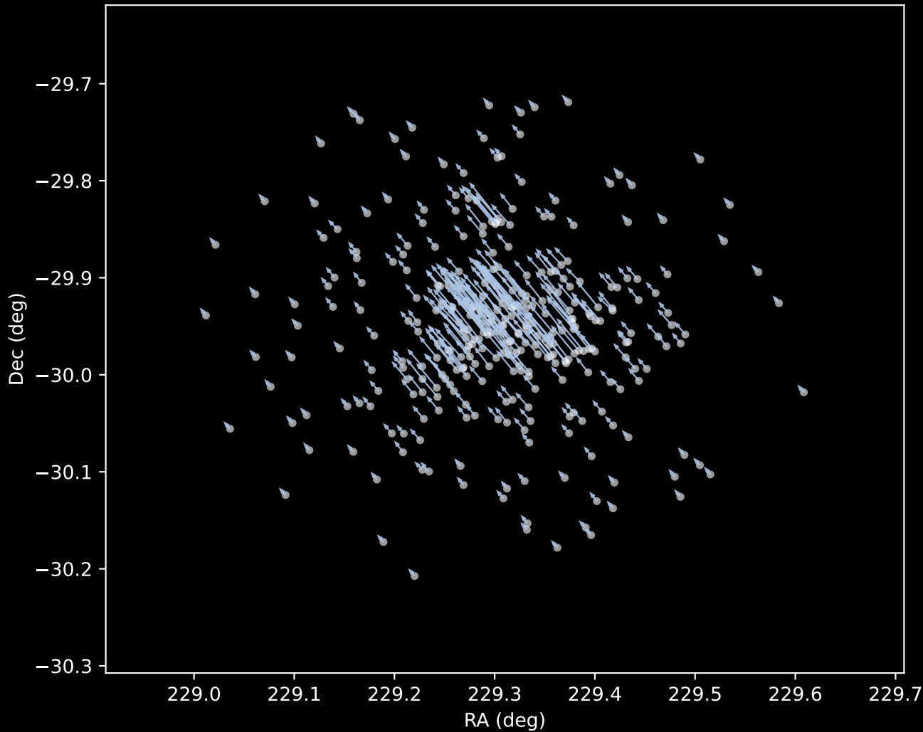
Gaia DR3 Cluster 1 Proper Motion Vectors (n=329)
