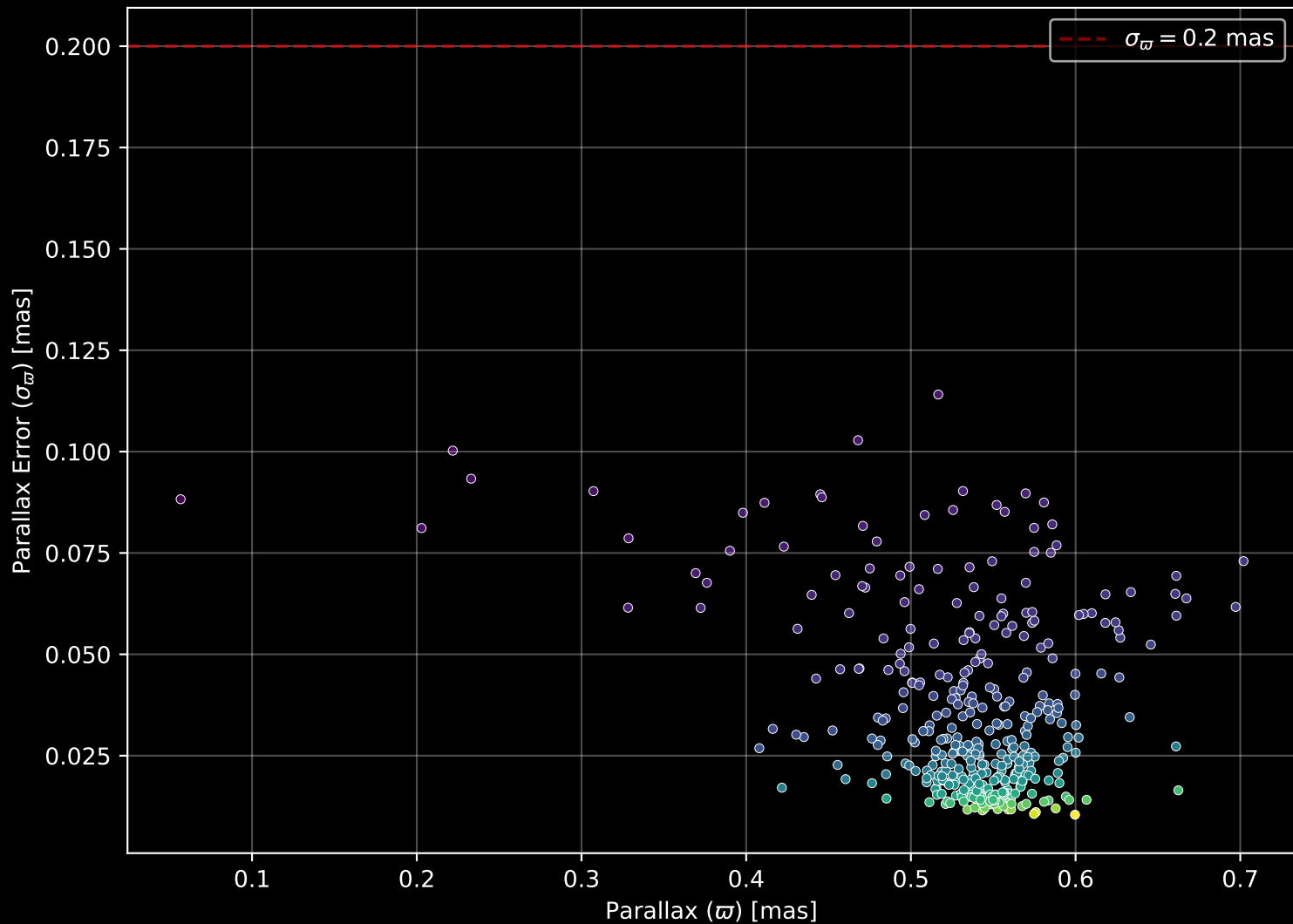
Gaia Cluster: [NGC_2627] Parallax Quality (n= 384)
