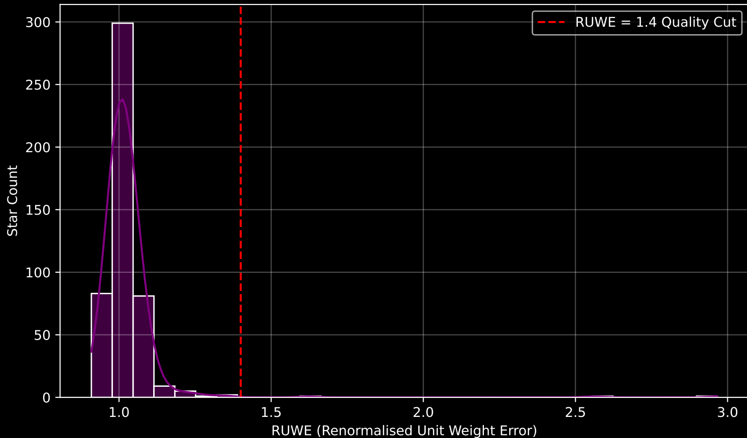
Gaia Cluster: [NGC_2658] RUWE Distribution (n= 483)
