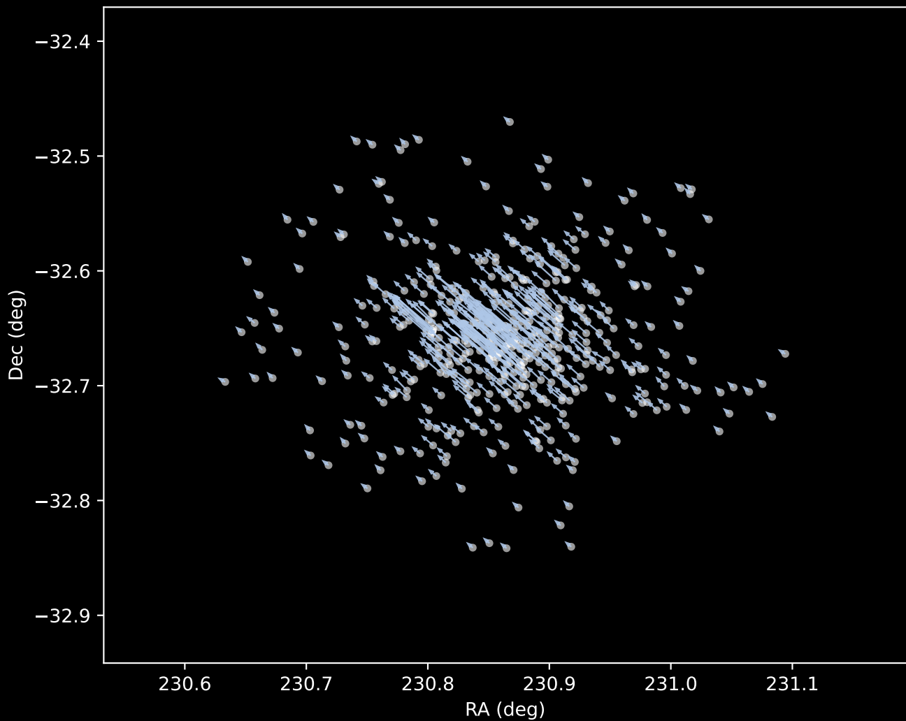
Gaia DR3 Cluster 1 Proper Motion Vectors (n=443)
