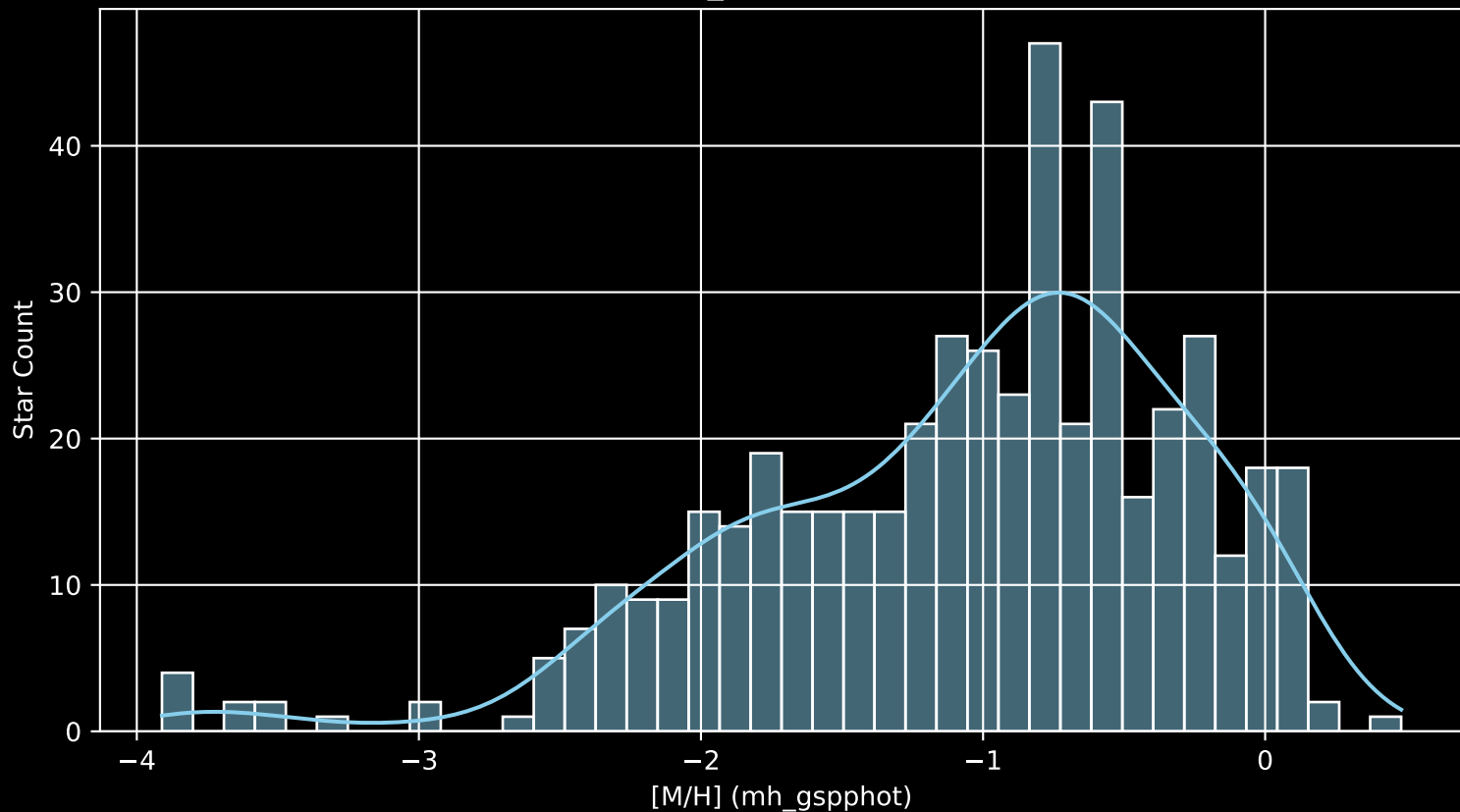
Gaia Cluster: [NGC_2658 [M/H] (mh_gspphot) (n= 484)
