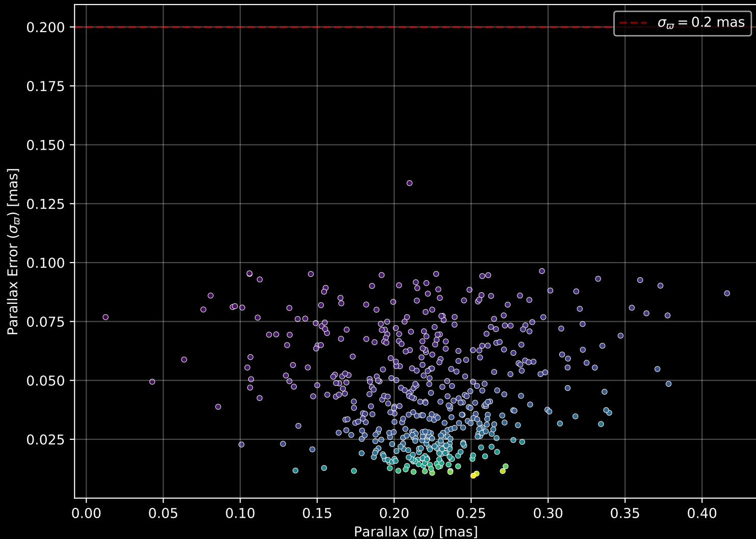
Gaia Cluster: [NGC_2658] Parallax Quality (n= 484)
