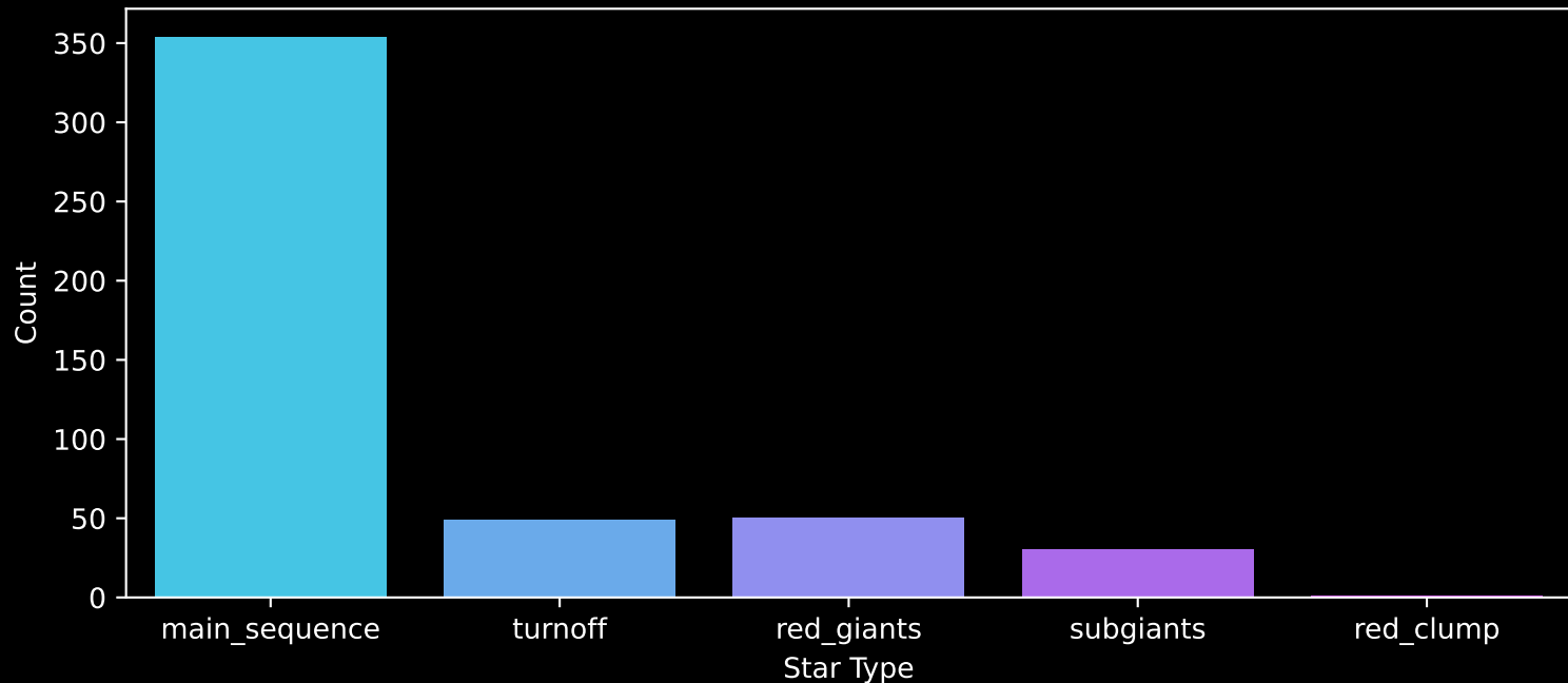
Gaia Cluster: [NGC_2658] Count plot of Star Type
