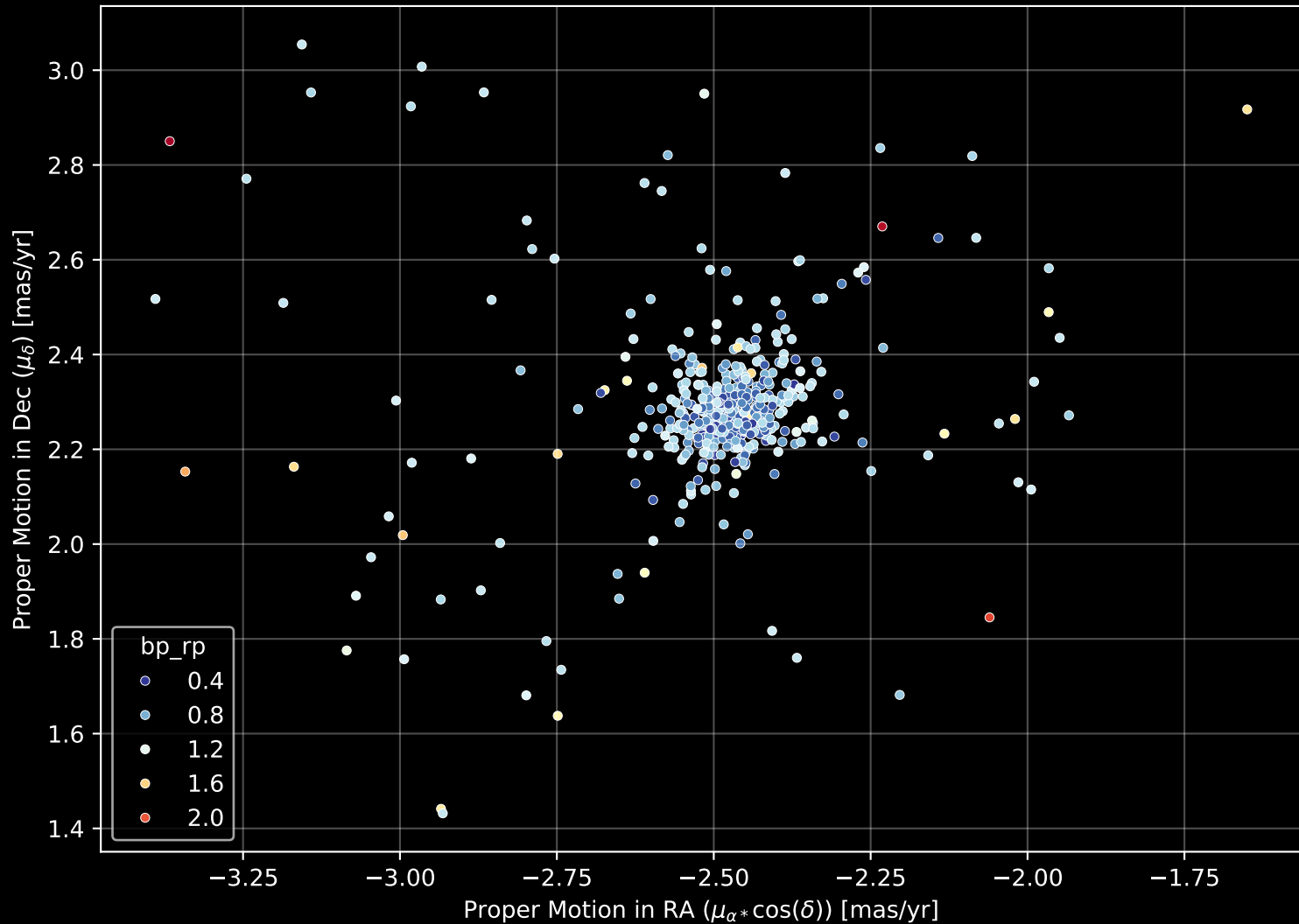
Gaia Cluster: [NGC_2658] Proper Motion Diagram (n= 484)
