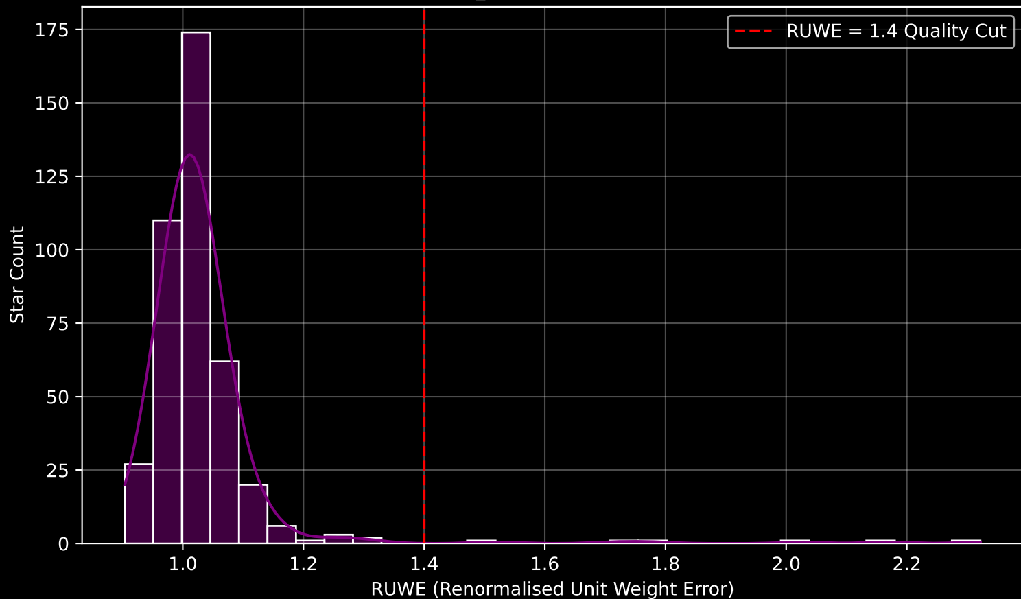
Gaia Cluster: [NGC_2660] RUWE Distribution (n= 411)
