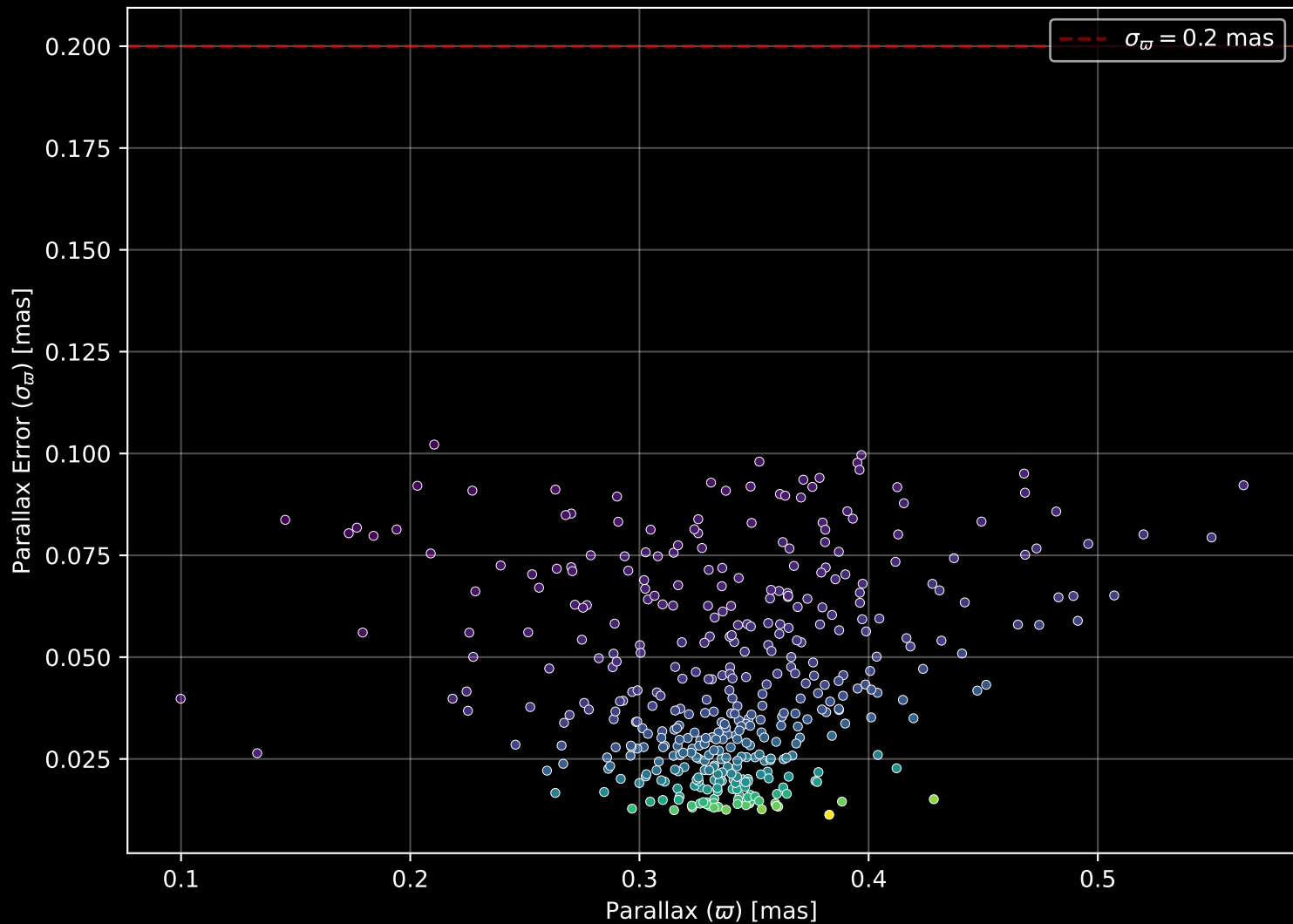
Gaia Cluster: [NGC_2660] Parallax Quality (n= 411)
