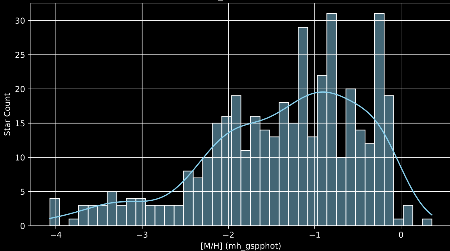
Gaia Cluster: [NGC_2660 [M/H] (mh_gspphot) (n= 410)
