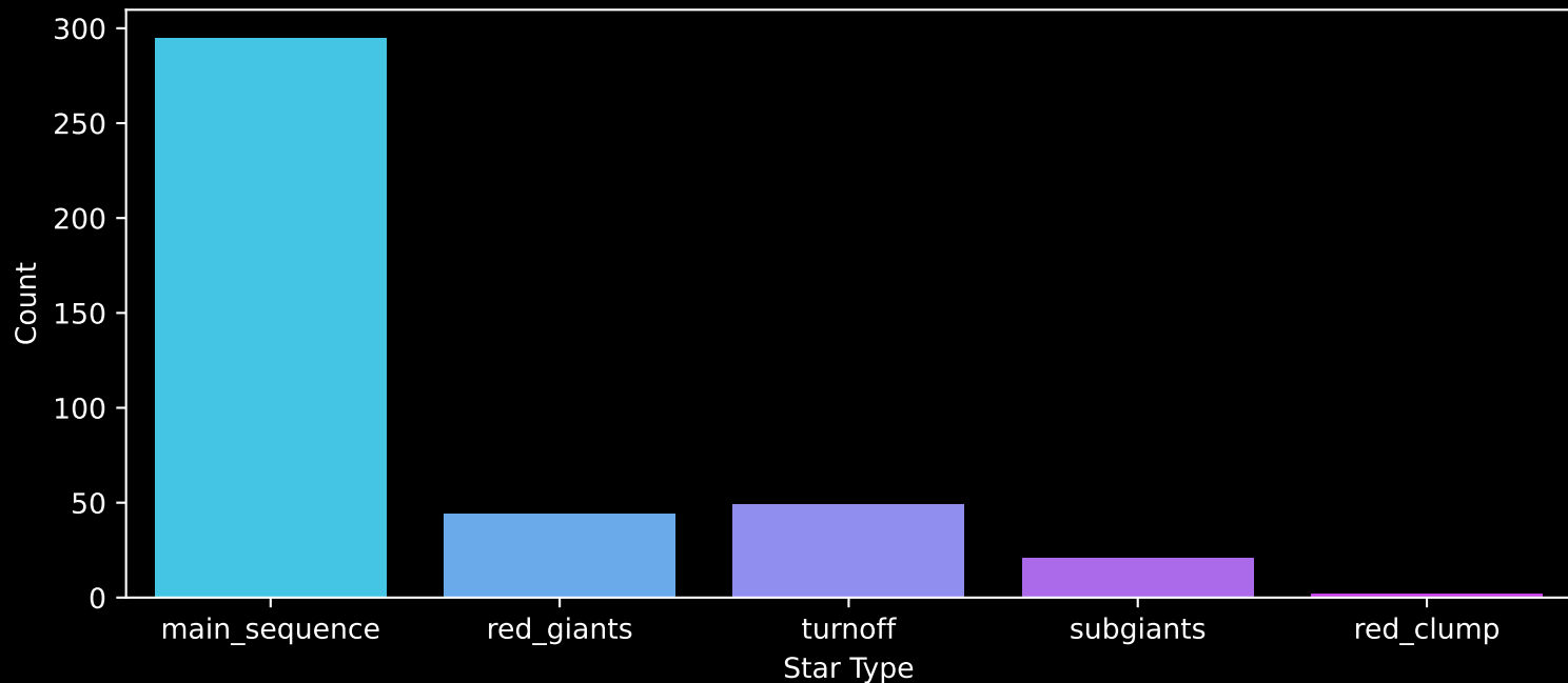
Gaia Cluster: [NGC_2660] Count plot of Star Type
