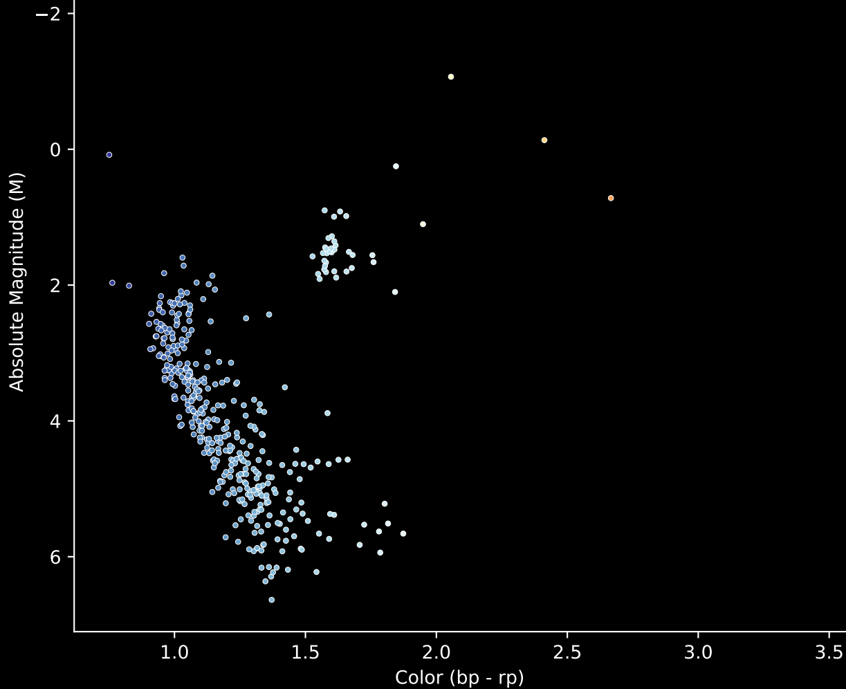
Gaia Cluster: [NGC 2660] Stars (n= 411) Hertzsprung-Russel Diagram
