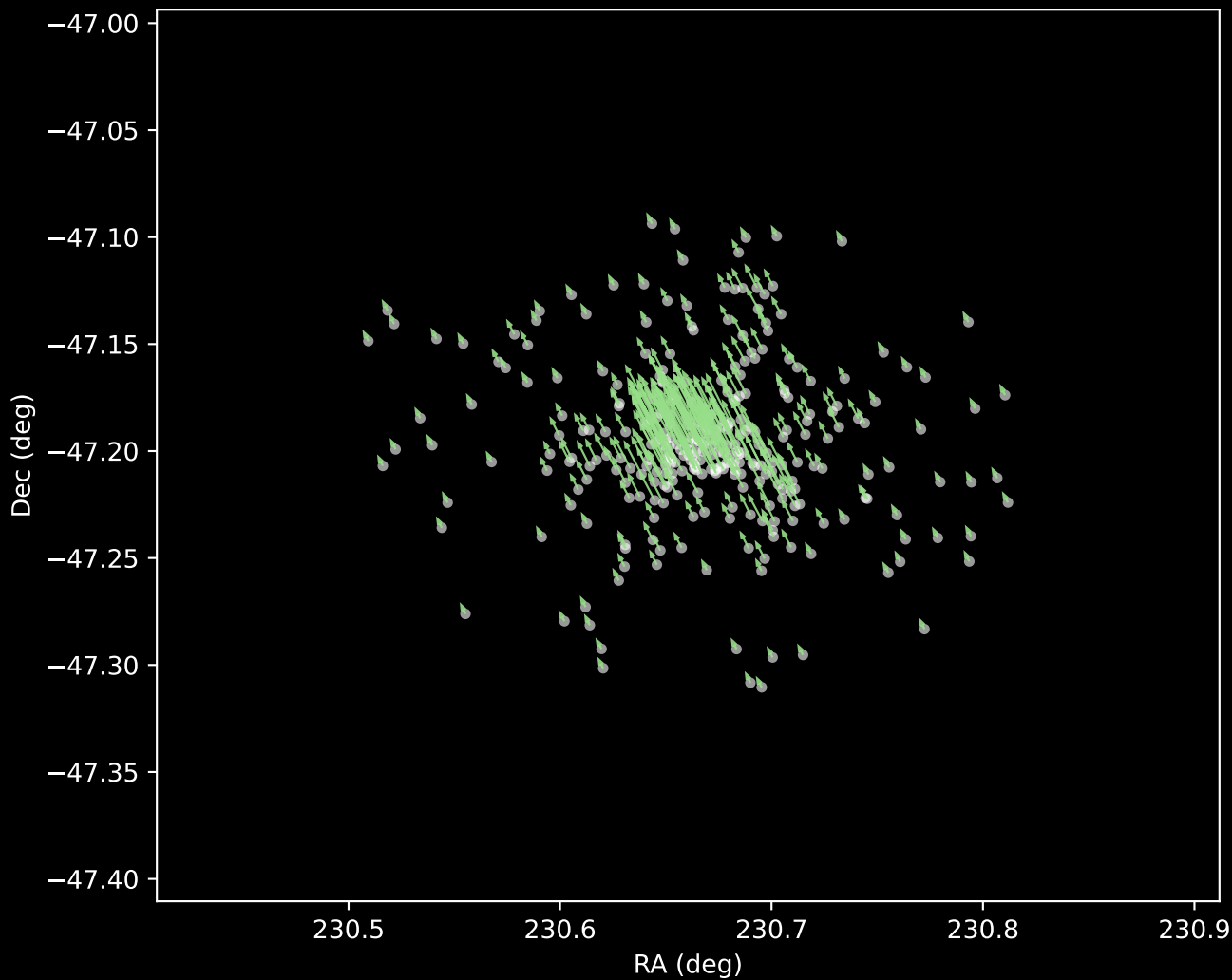
Gaia DR3 Cluster 5 Proper Motion Vectors (n=312)
