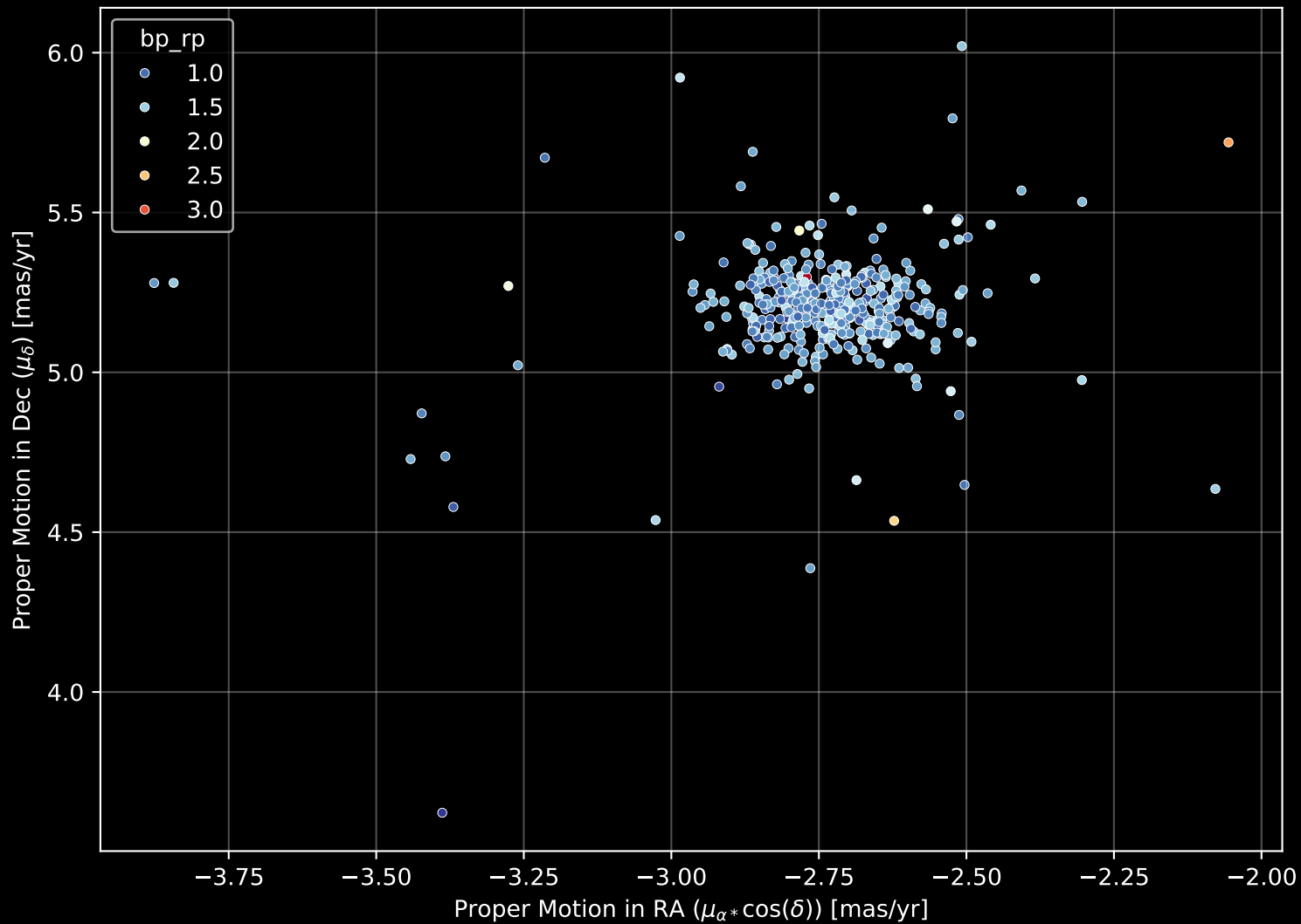
Gaia Cluster: [NGC_2660] Proper Motion Diagram (n= 411)
