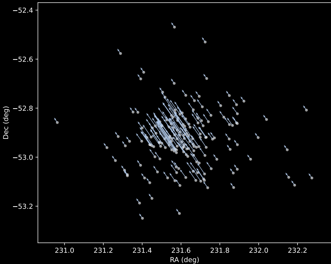
Gaia DR3 Cluster 1 Proper Motion Vectors (n=169)
