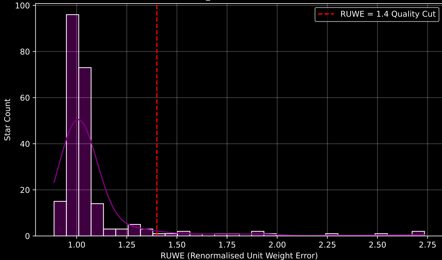
Gaia Cluster: [NGC_2669] RUWE Distribution (n= 226)
