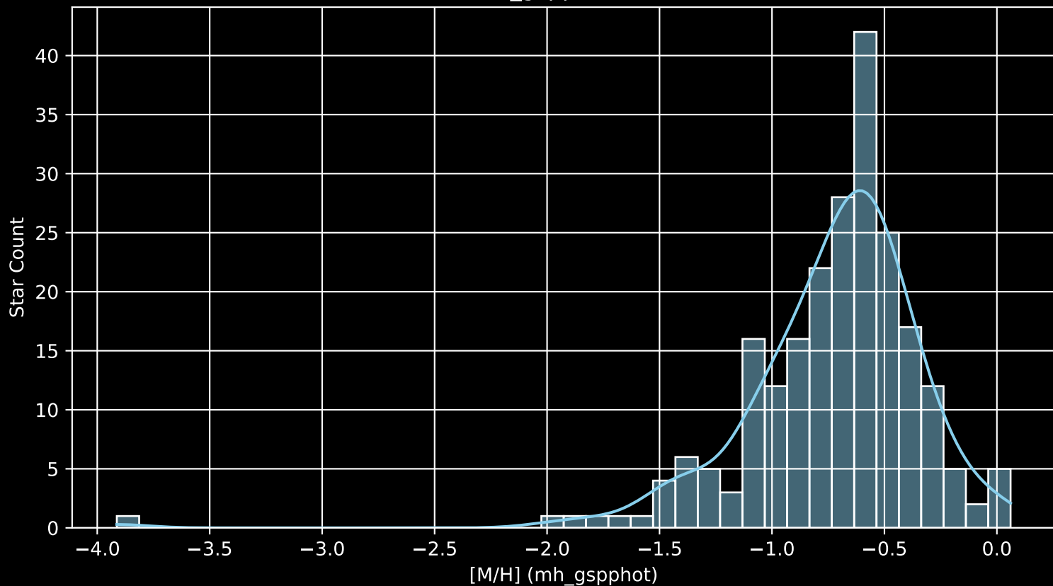
Gaia Cluster: [NGC_2669 [M/H] (mh_gspphot) (n= 226)
