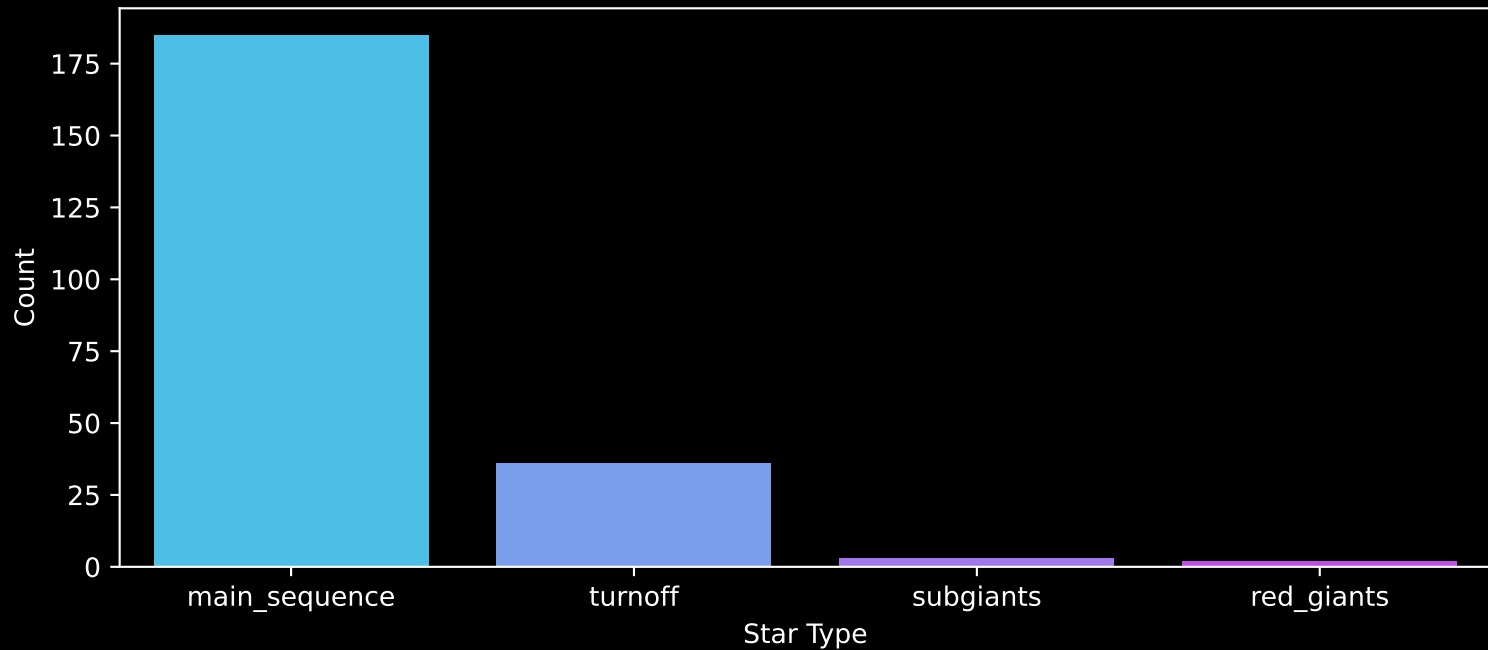
Gaia Cluster: [NGC_2669] Count plot of Star Type
