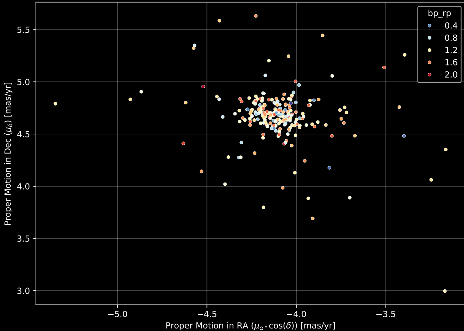
Gaia Cluster: [NGC_2669] Proper Motion Diagram (n= 226)
