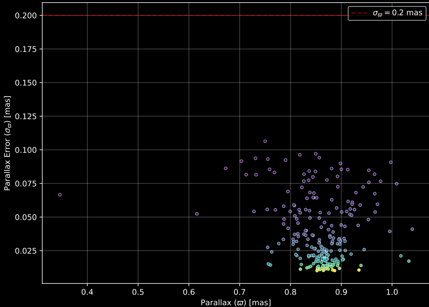
Gaia Cluster: [NGC_2669] Parallax Quality (n= 226)
