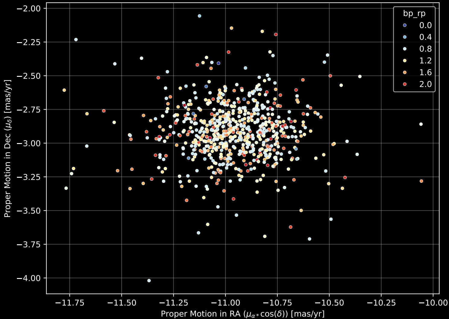
Gaia Cluster: [NGC_2682] Proper Motion Diagram (n= 720)
