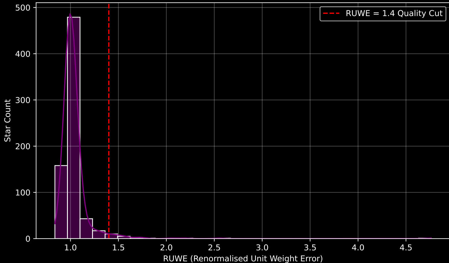
Gaia Cluster: [NGC_2682] RUWE Distribution (n= 719)
