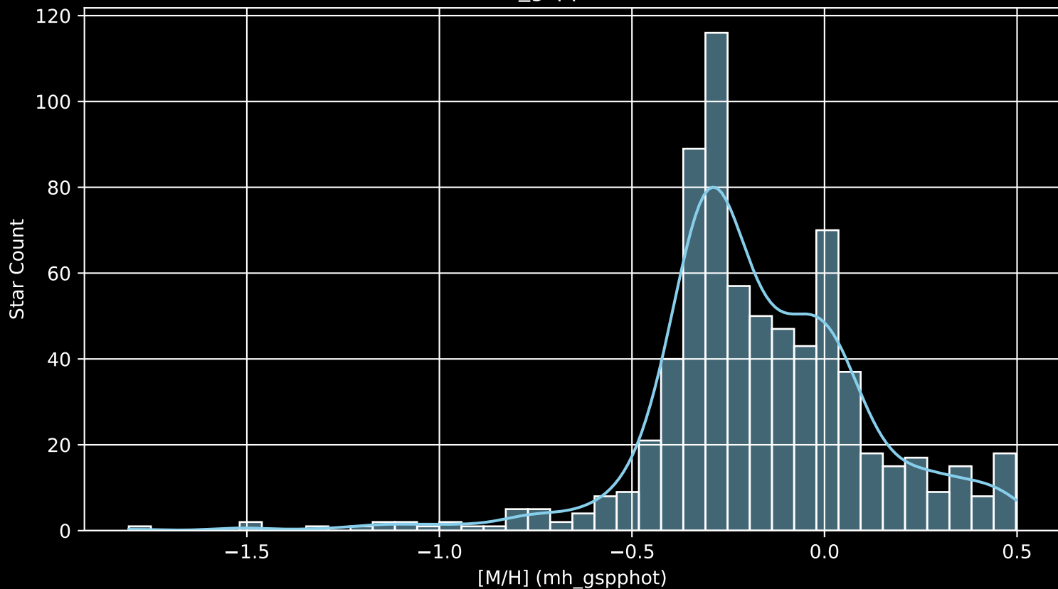
Gaia Cluster: [NGC_2682 [M/H] (mh_gspphot) (n= 717)
