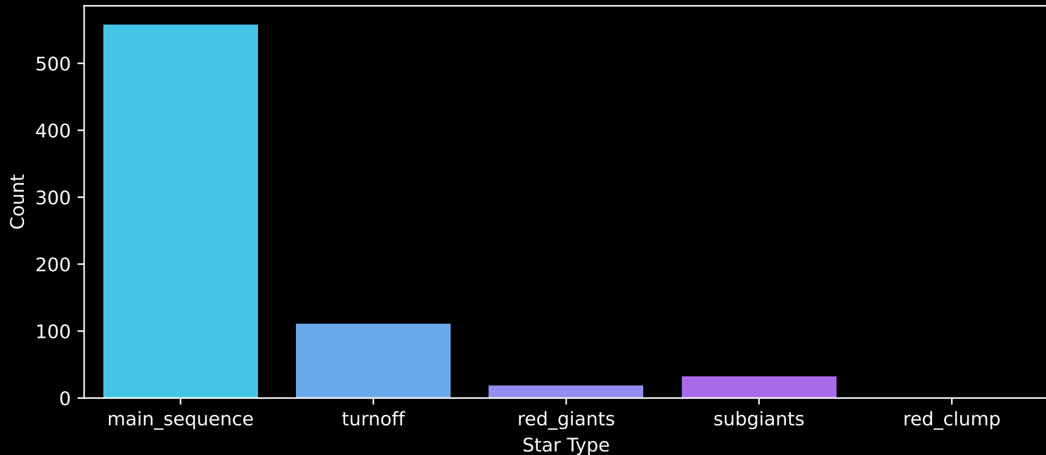
Gaia Cluster: [NGC_2682] Count plot of Star Type
