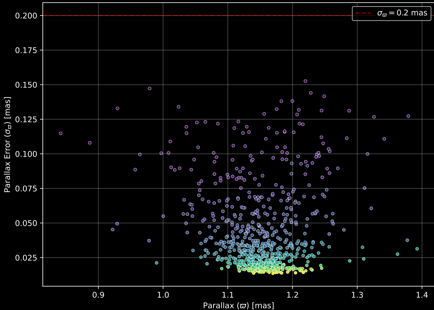
Gaia Cluster: [NGC_2682] Parallax Quality (n= 720)
