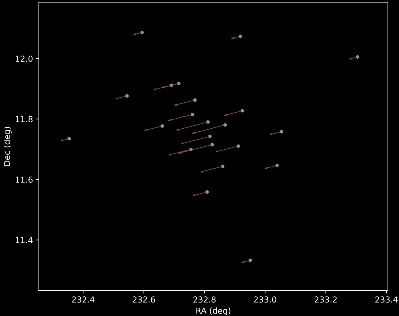
Gaia DR3 Cluster 30 Proper Motion Vectors (n=22)
