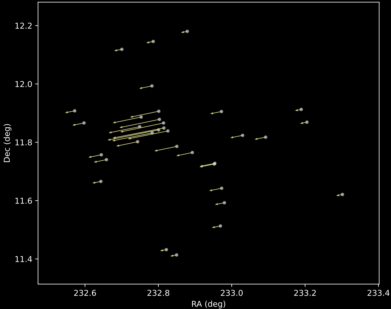
Gaia DR3 Cluster 17 Proper Motion Vectors (n=34)
