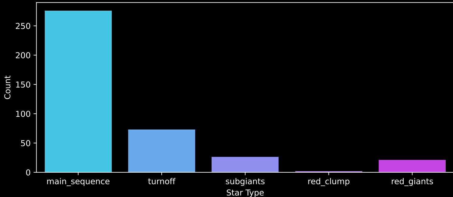
Gaia Cluster: [NGC_2818] Count plot of Star Type
