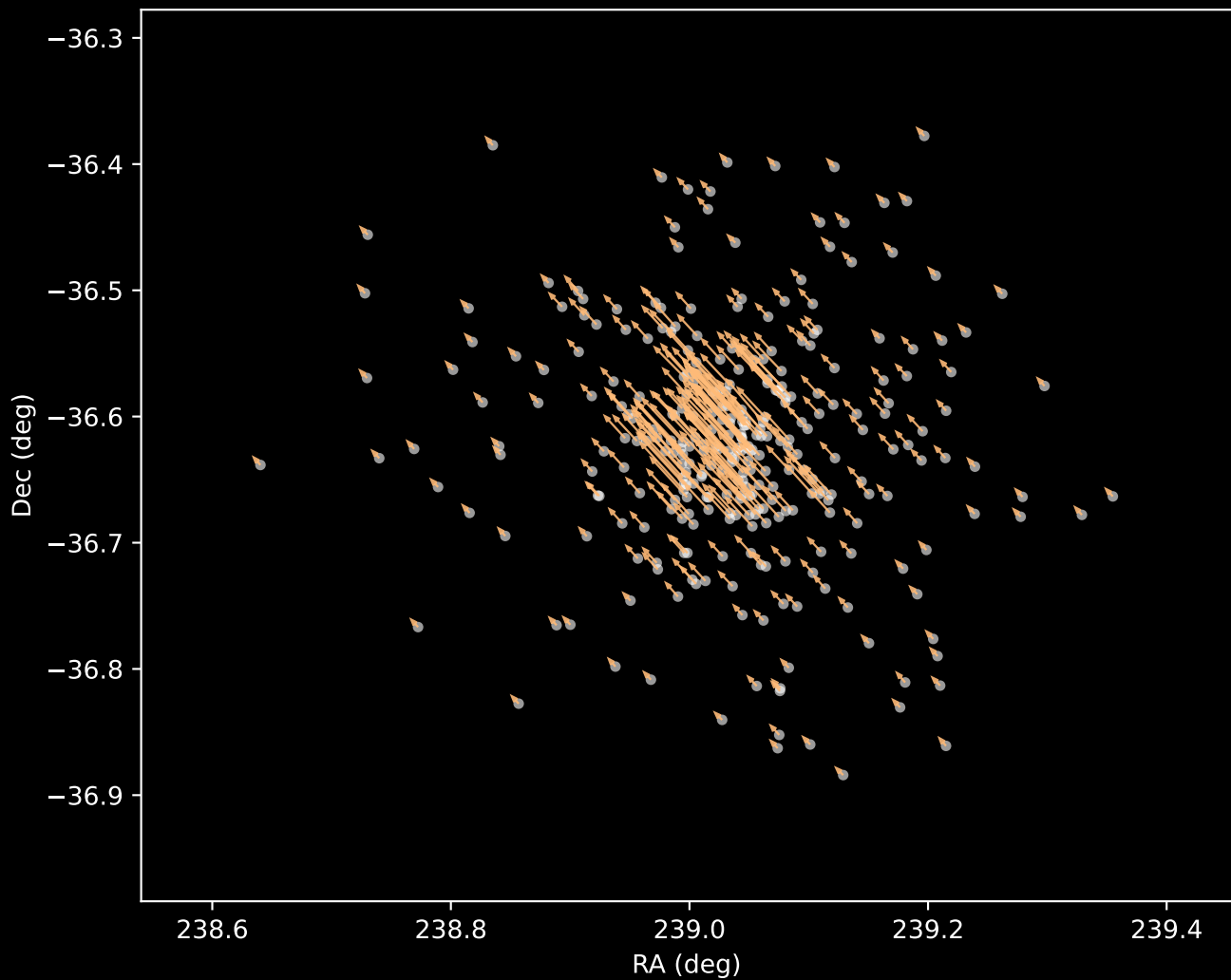
Gaia DR3 Cluster 3 Proper Motion Vectors (n=311)
