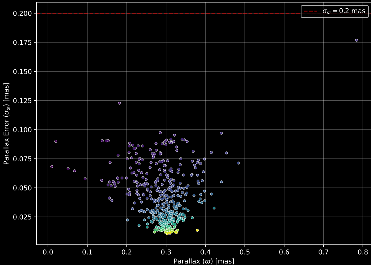
Gaia Cluster: [NGC_2818] Parallax Quality (n= 398)
