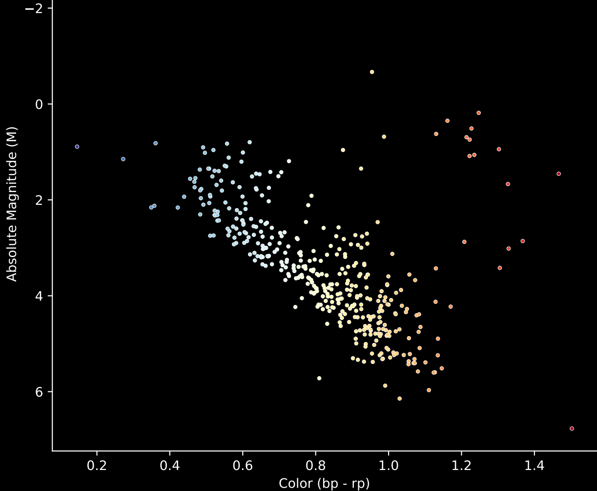
Gaia Cluster: [NGC 2818] Stars (n= 398) Hertzsprung-Russel Diagram
