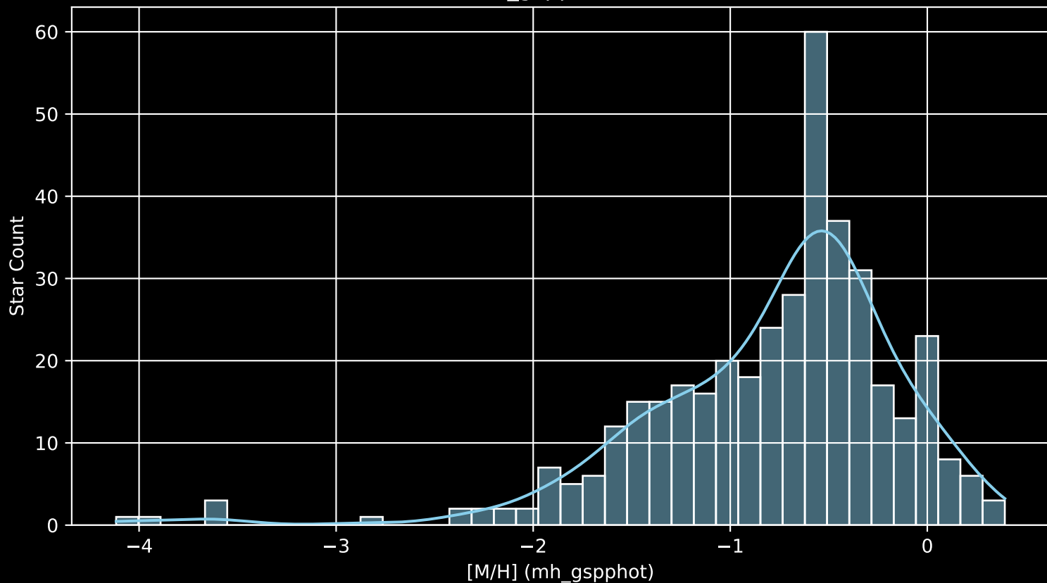
Gaia Cluster: [NGC_2818 [M/H] (mh_gspphot) (n= 395)
