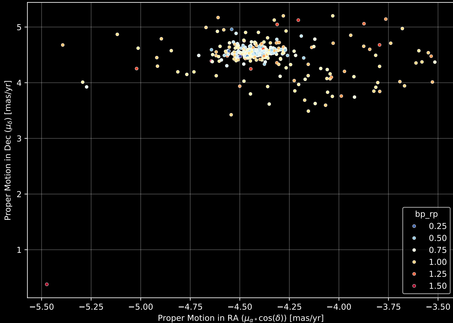
Gaia Cluster: [NGC_2818] Proper Motion Diagram (n= 398)
