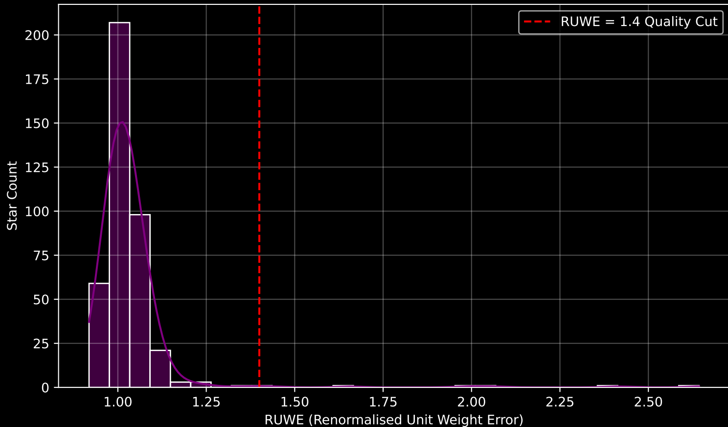
Gaia Cluster: [NGC_2818] RUWE Distribution (n= 398)
