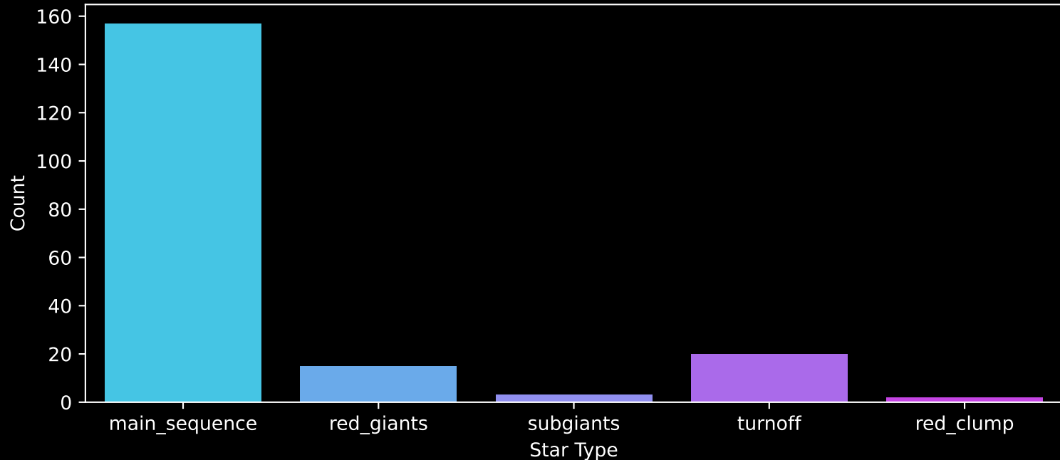
Gaia Cluster: [NGC_2849] Count plot of Star Type
