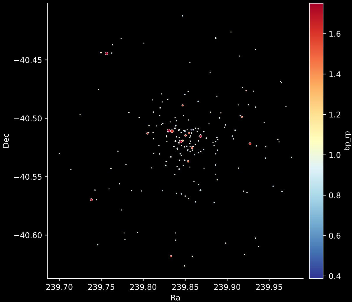
Gaia Cluster: [NGC_2849] Stars: 197
