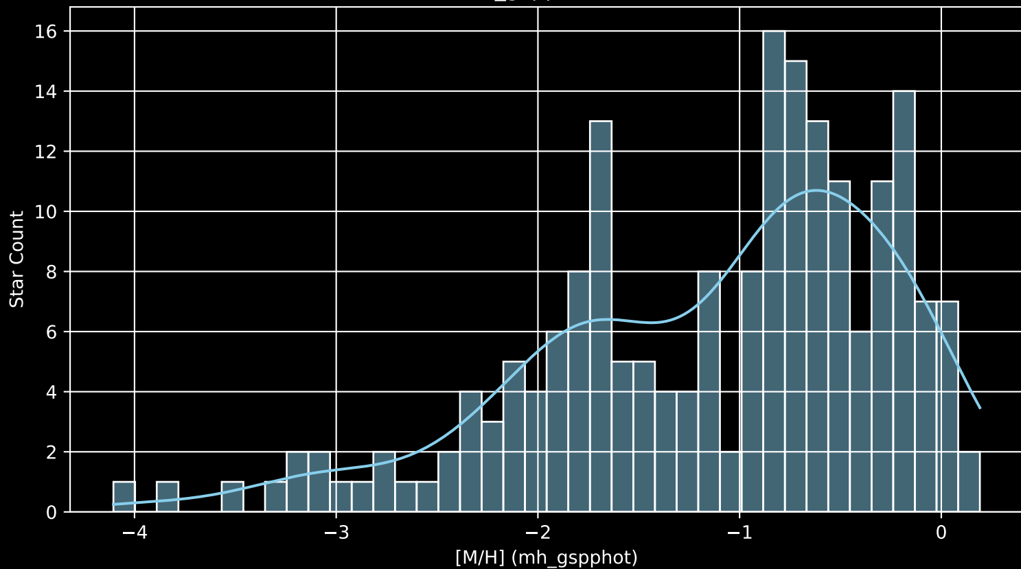
Gaia Cluster: [NGC_2849 [M/H] (mh_gspphot) (n= 197)
