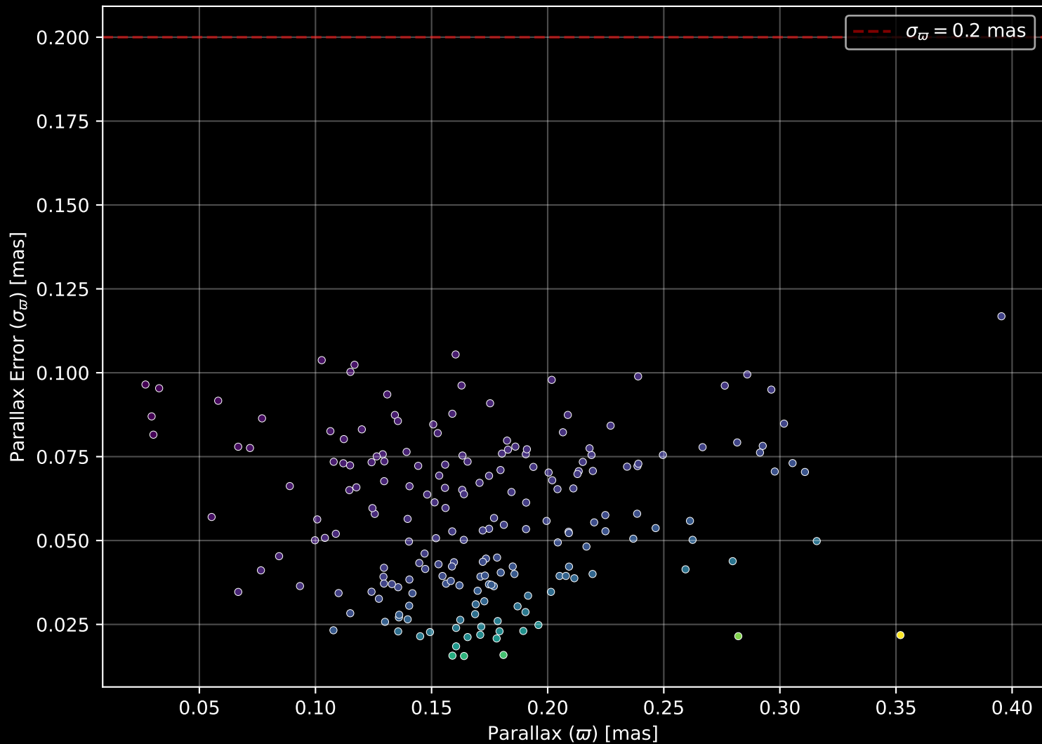
Gaia Cluster: [NGC_2849] Parallax Quality (n= 197)
