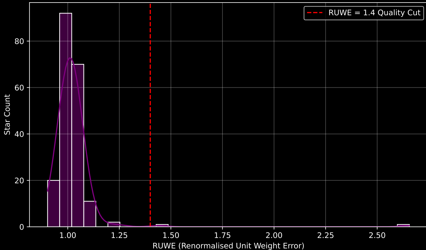
Gaia Cluster: [NGC_2849] RUWE Distribution (n= 197)
