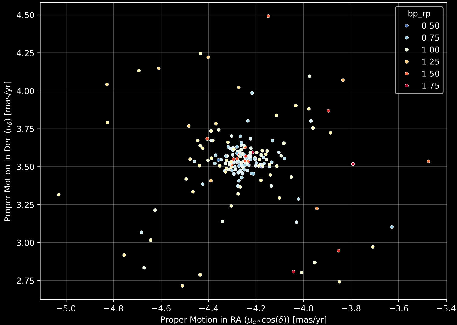
Gaia Cluster: [NGC_2849] Proper Motion Diagram (n= 197)
