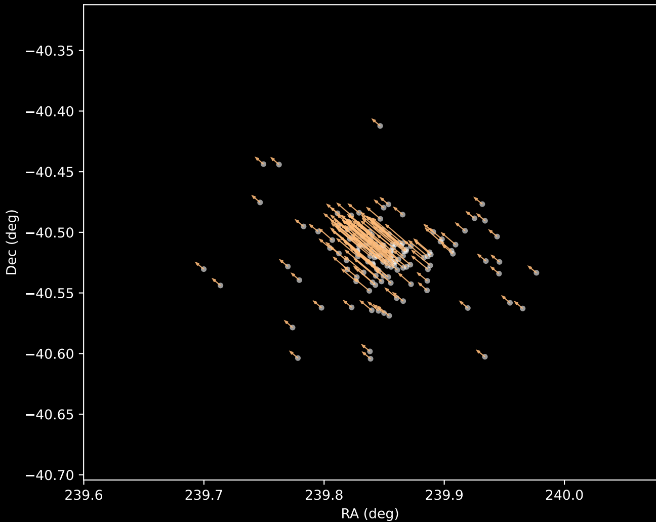
Gaia DR3 Cluster 3 Proper Motion Vectors (n=135)
