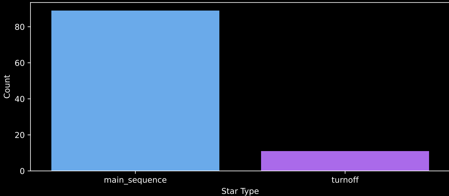
Gaia Cluster: [NGC_2925] Count plot of Star Type
