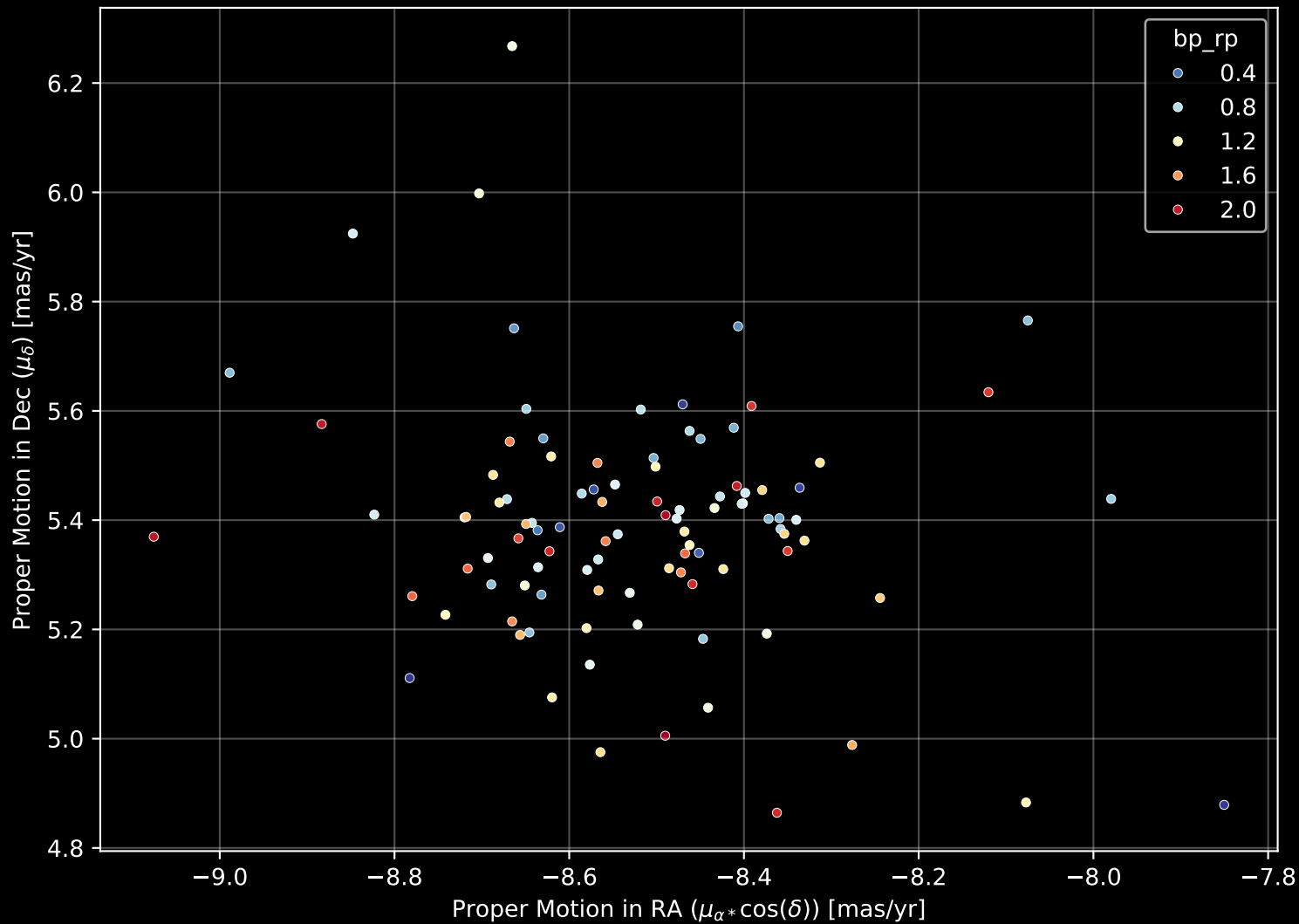
Gaia Cluster: [NGC_2925] Proper Motion Diagram (n= 100)
