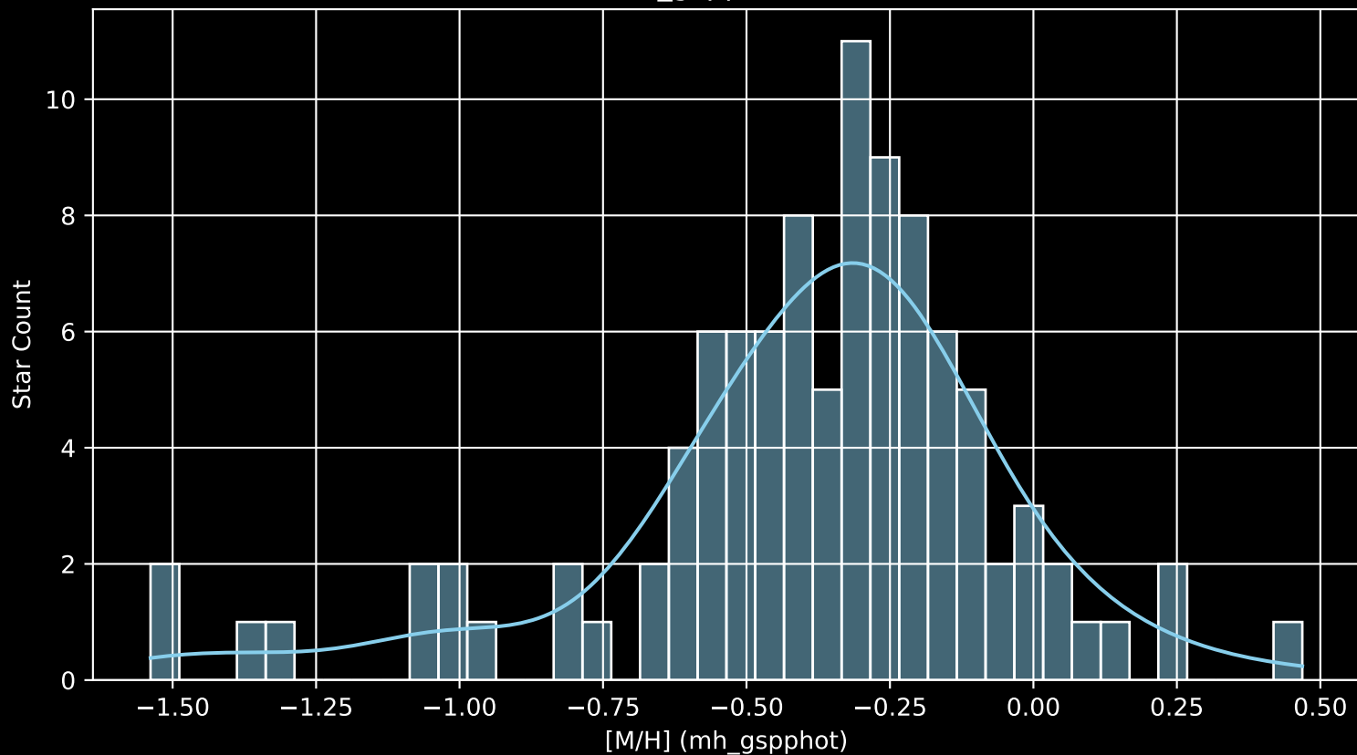
Gaia Cluster: [NGC_2925 [M/H] (mh_gspphot) (n= 100)
