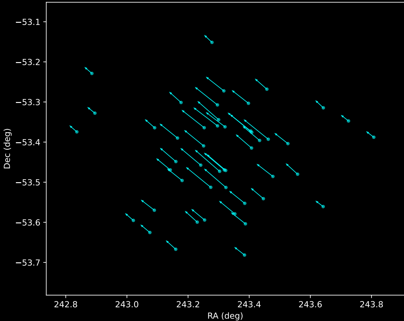
Gaia DR3 Noise Stream Proper Motion Vectors (n=48)
