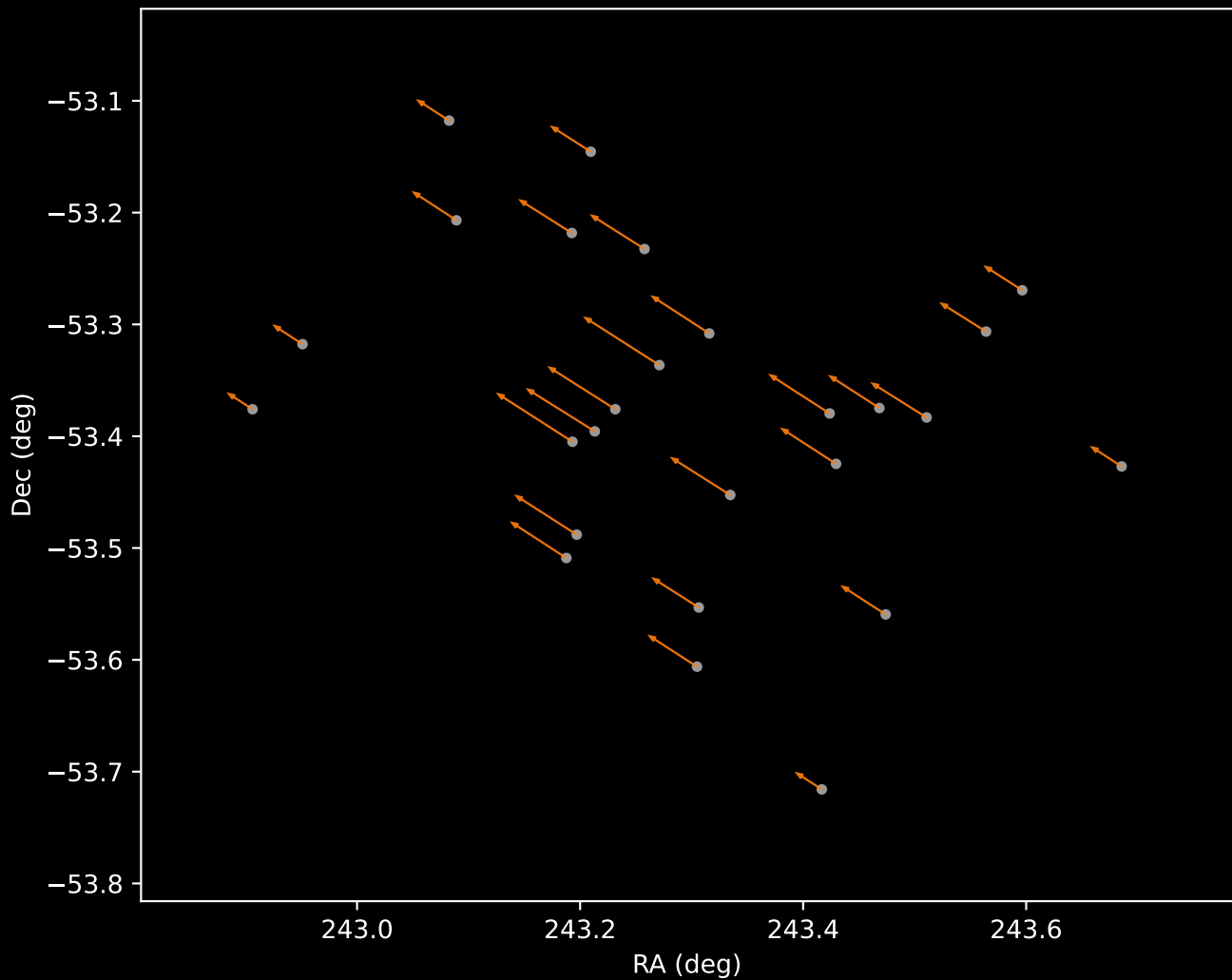
Gaia DR3 Cluster 2 Proper Motion Vectors (n=26)
