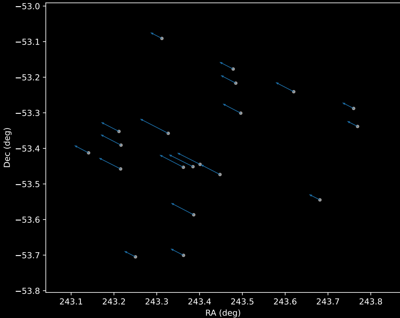
Gaia DR3 Cluster 0 Proper Motion Vectors (n=20)
