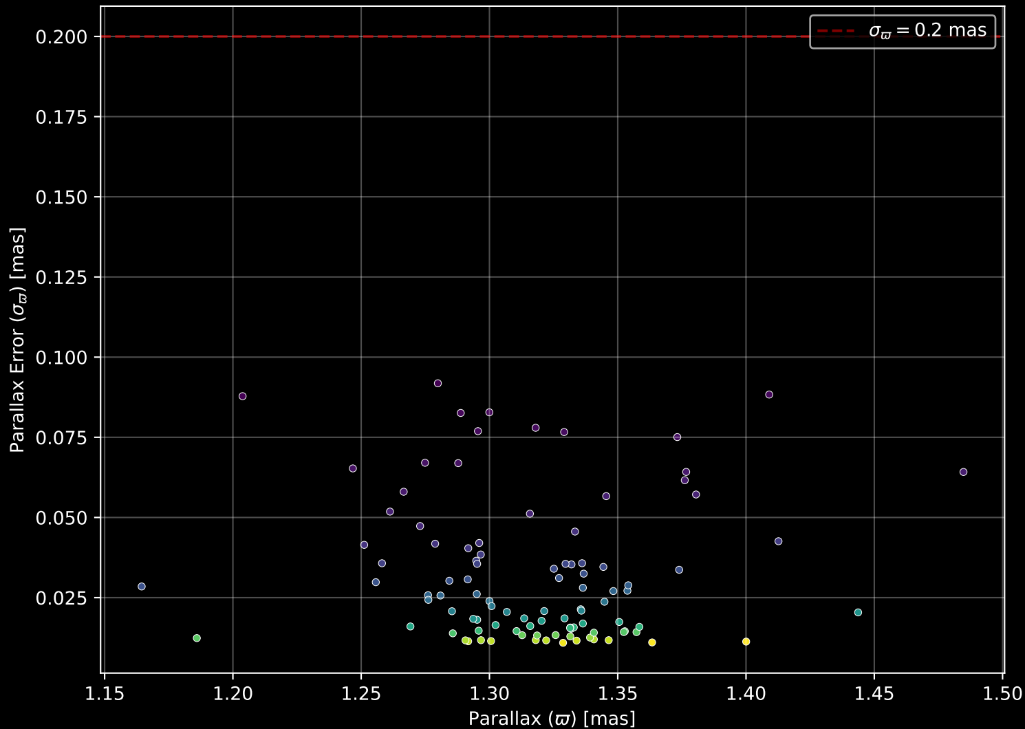
Gaia Cluster: [NGC_2925] Parallax Quality (n= 100)
