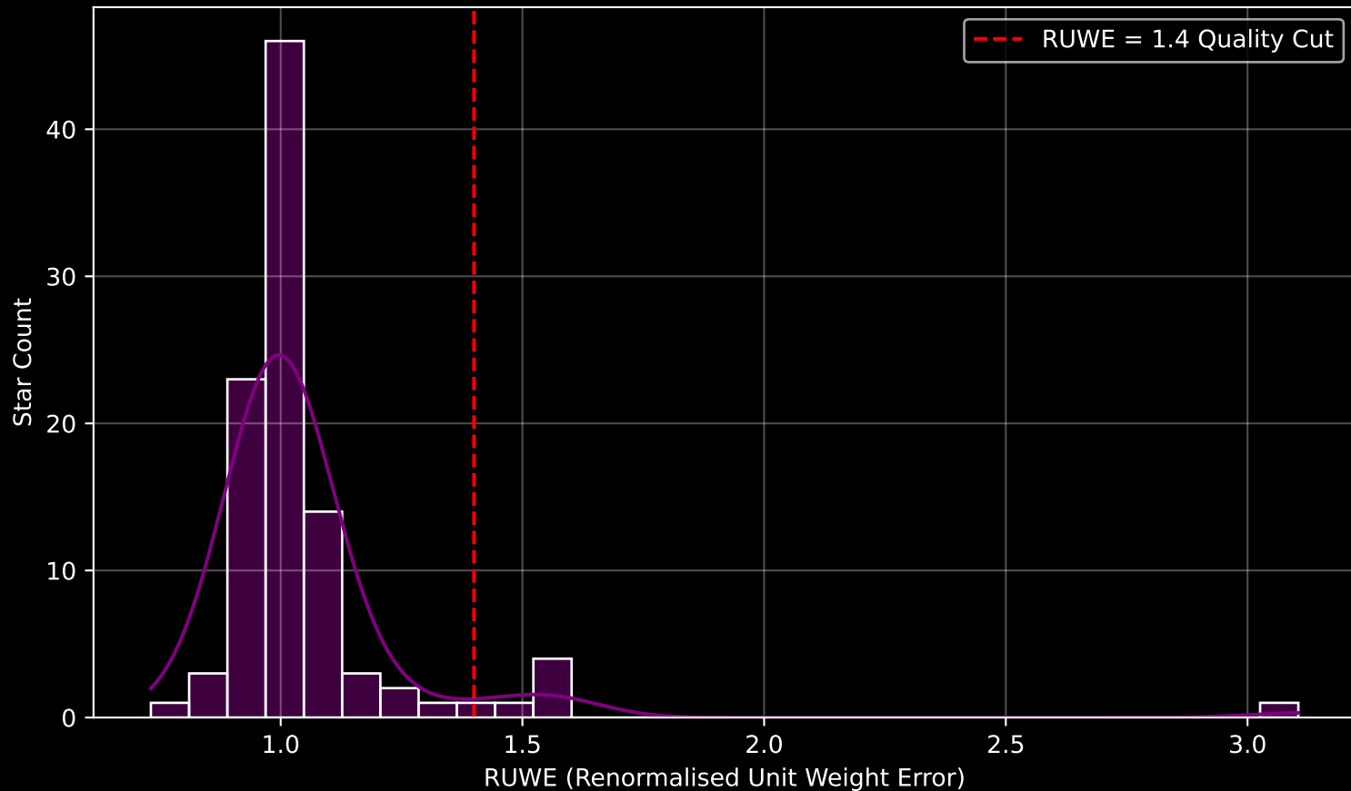
Gaia Cluster: [NGC_2925] RUWE Distribution (n= 100)
