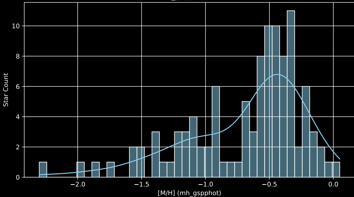
Gaia Cluster: [NGC_3033 [M/H] (mh_gspphot) (n= 106)
