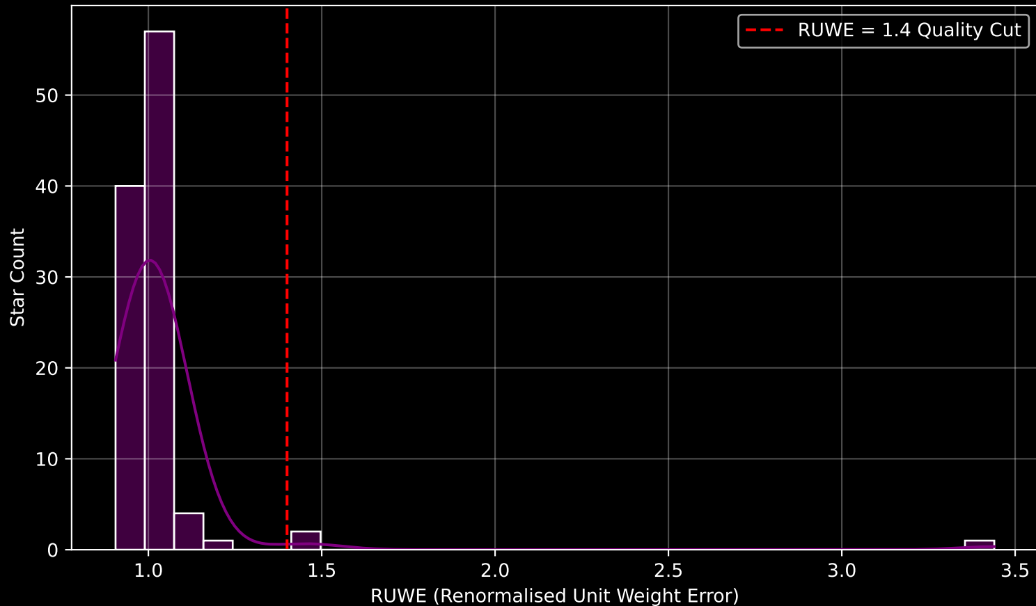
Gaia Cluster: [NGC_3033] RUWE Distribution (n= 105)
