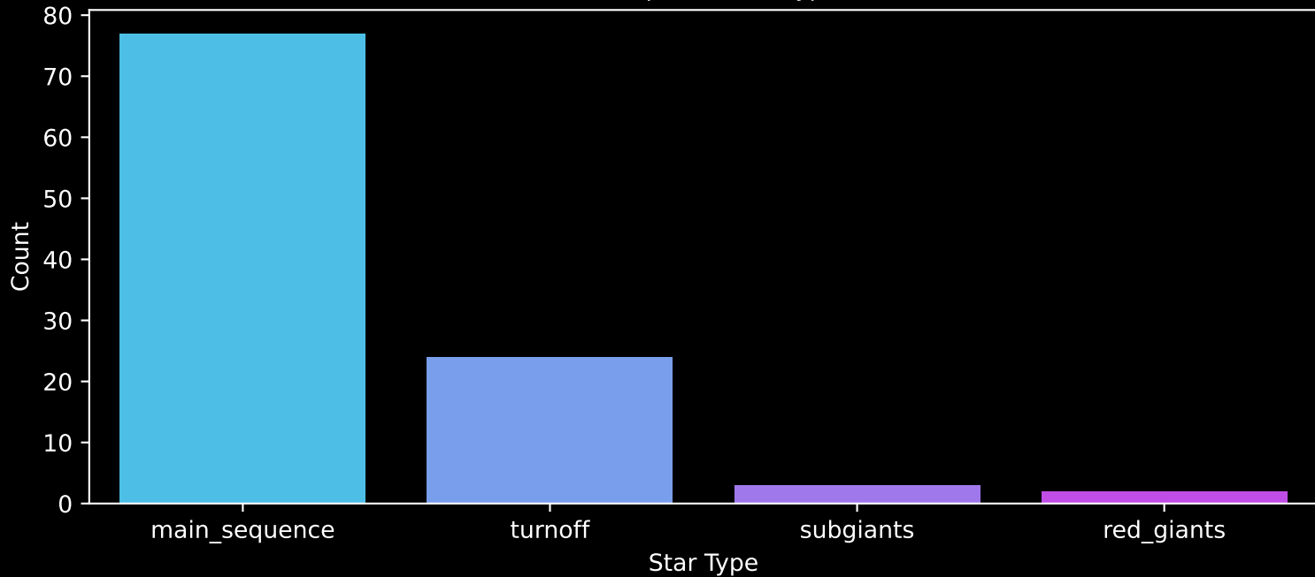
Gaia Cluster: [NGC_3033] Count plot of Star Type
