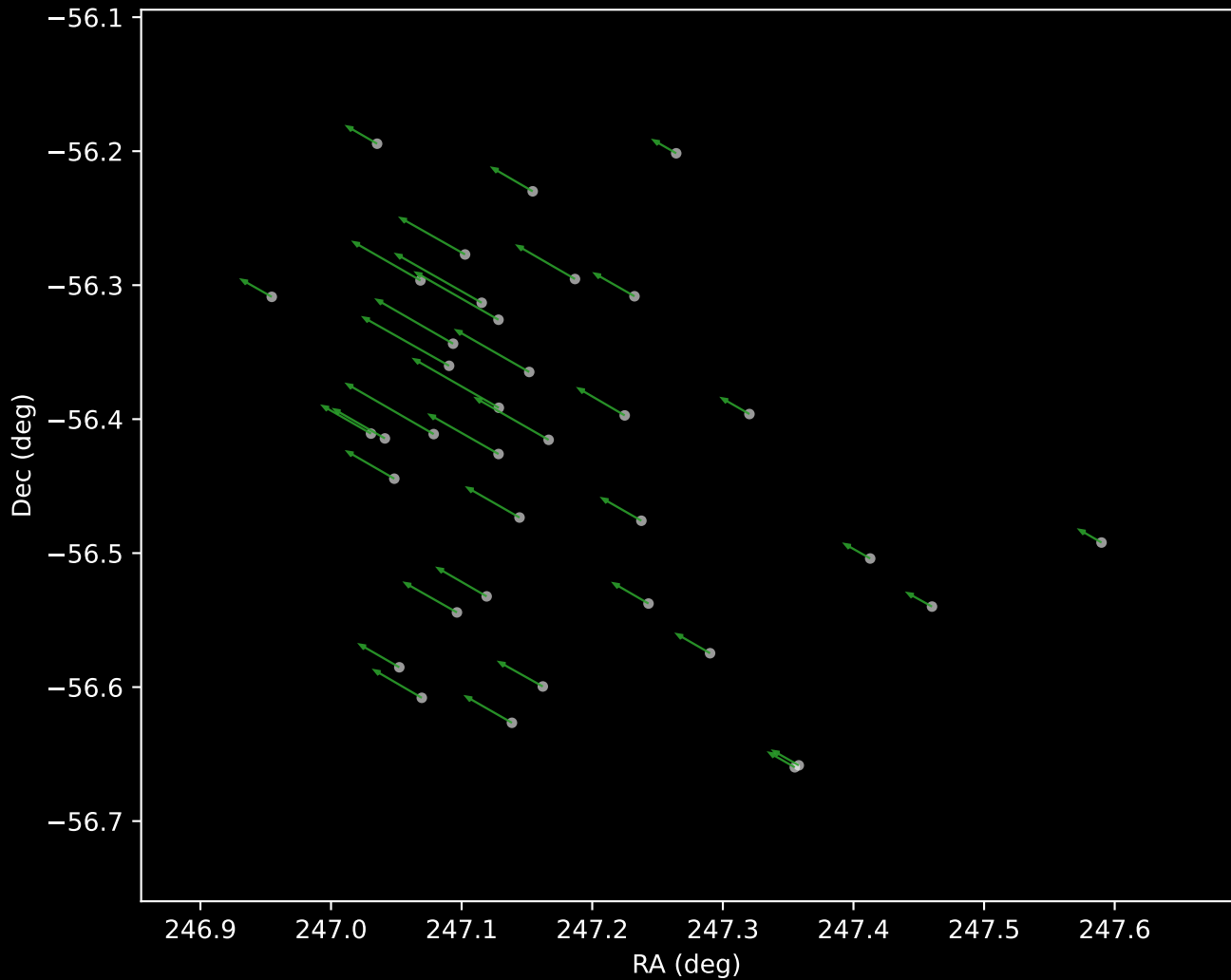
Gaia DR3 Cluster 4 Proper Motion Vectors (n=37)
