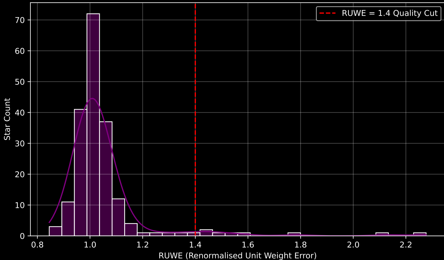
Gaia Cluster: [NGC_3255] RUWE Distribution (n= 193)
