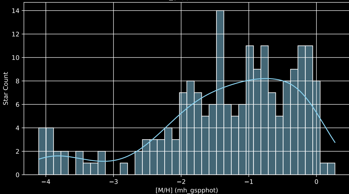
Gaia Cluster: [NGC_3255 [M/H] (mh_gspphot) (n= 193)
