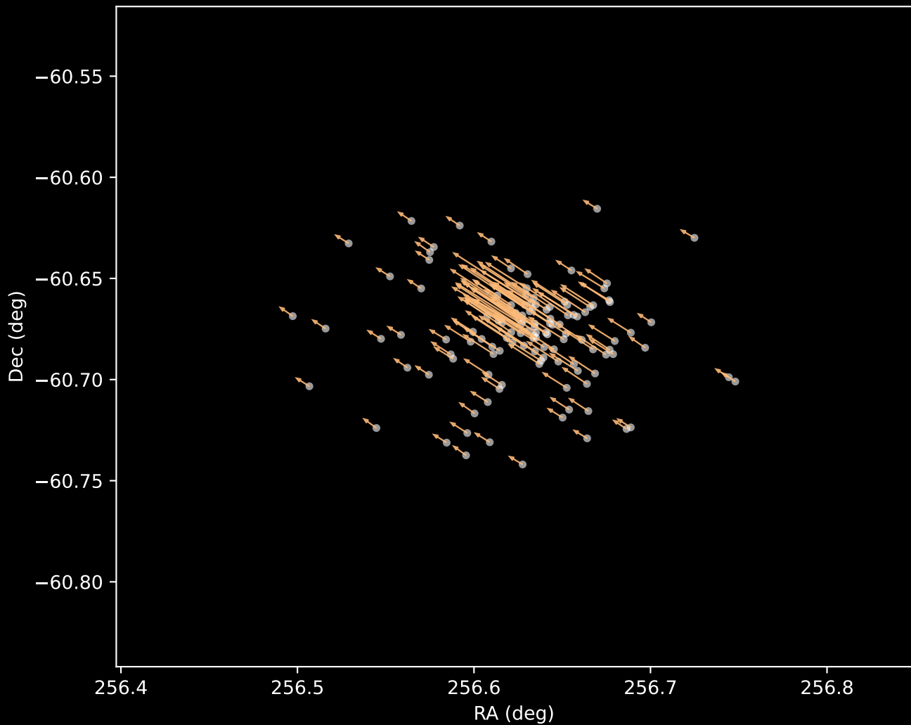
Gaia DR3 Cluster 3 Proper Motion Vectors (n=123)
