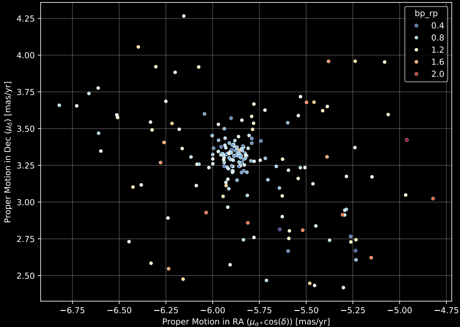
Gaia Cluster: [NGC_3255] Proper Motion Diagram (n= 193)
