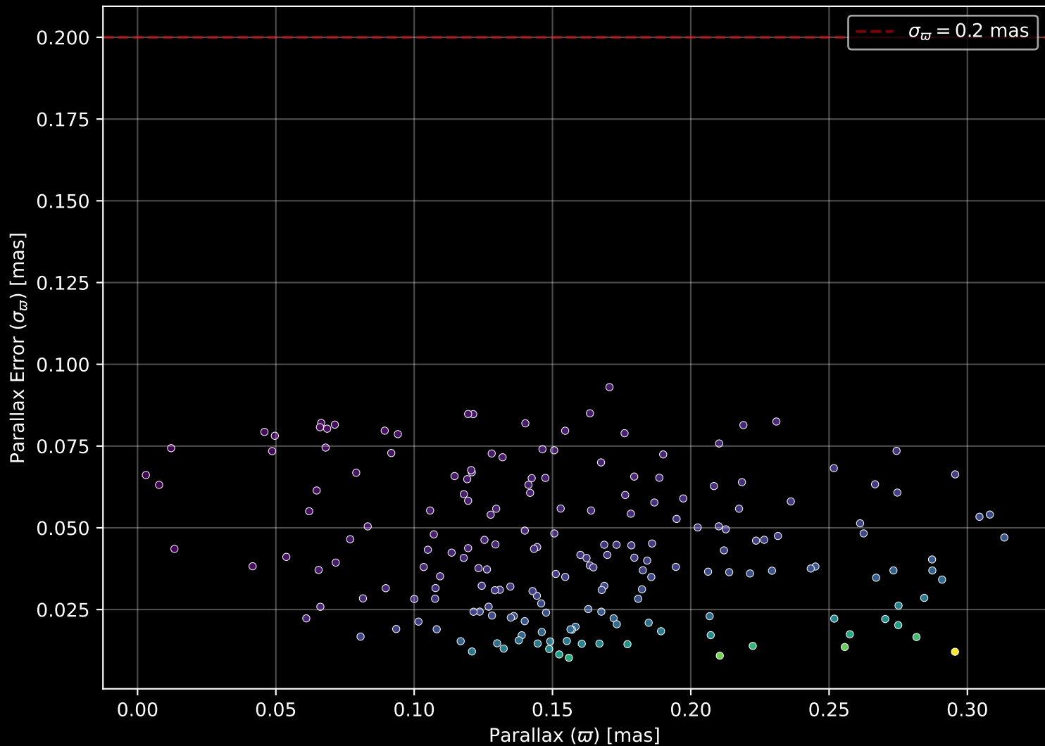
Gaia Cluster: [NGC_3255] Parallax Quality (n= 193)
