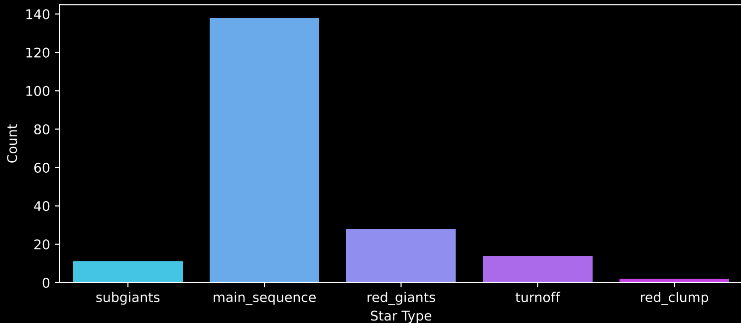
Gaia Cluster: [NGC_3255] Count plot of Star Type
