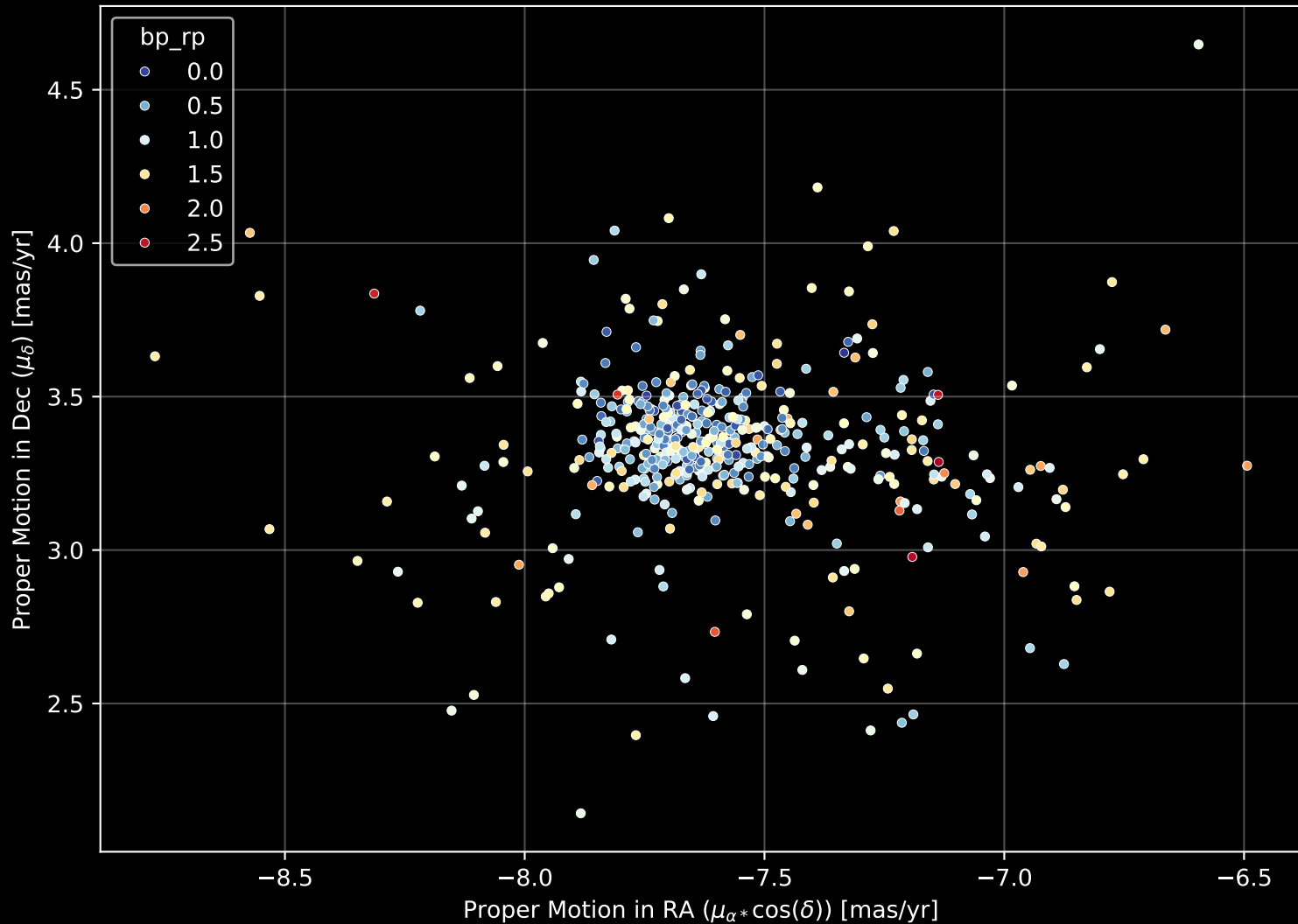
Gaia Cluster: [NGC_3293] Proper Motion Diagram (n= 490)
