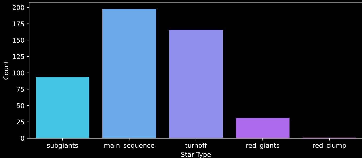
Gaia Cluster: [NGC_3293] Count plot of Star Type
