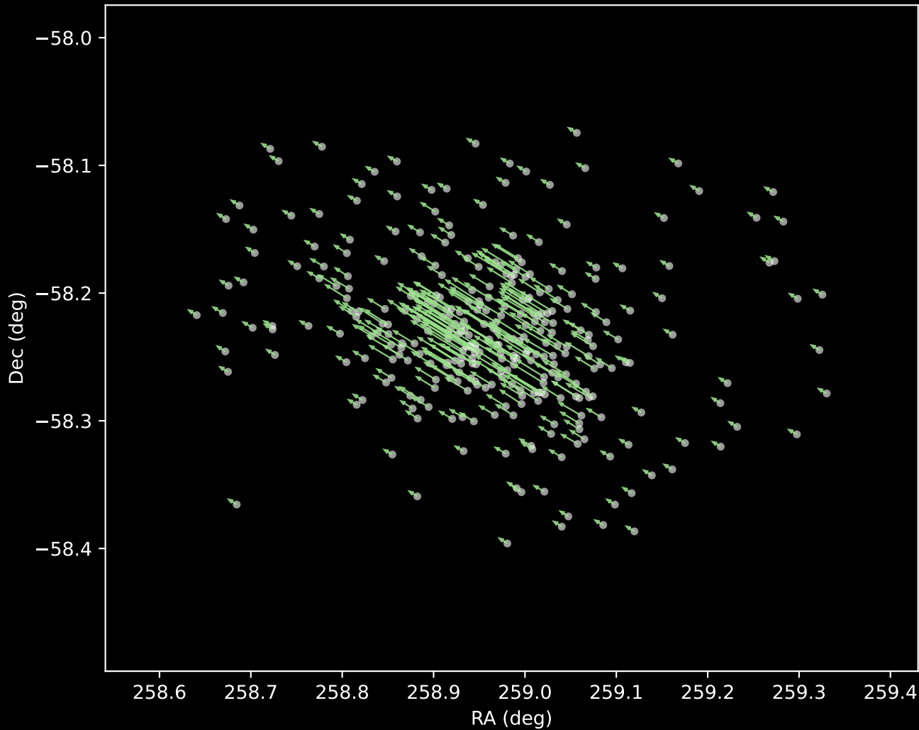
Gaia DR3 Cluster 5 Proper Motion Vectors (n=311)
