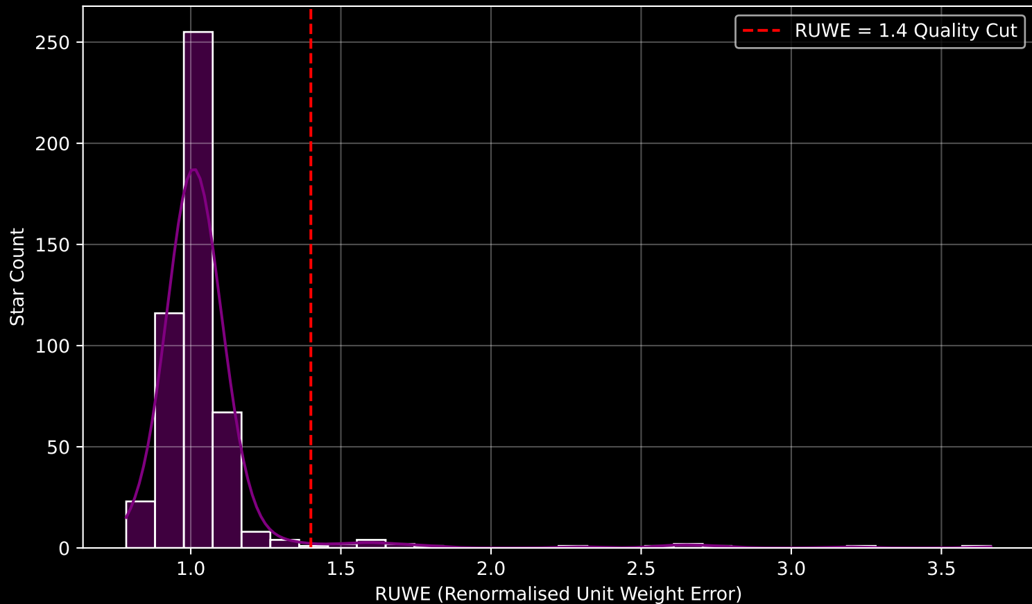
Gaia Cluster: [NGC_3293] RUWE Distribution (n= 490)
