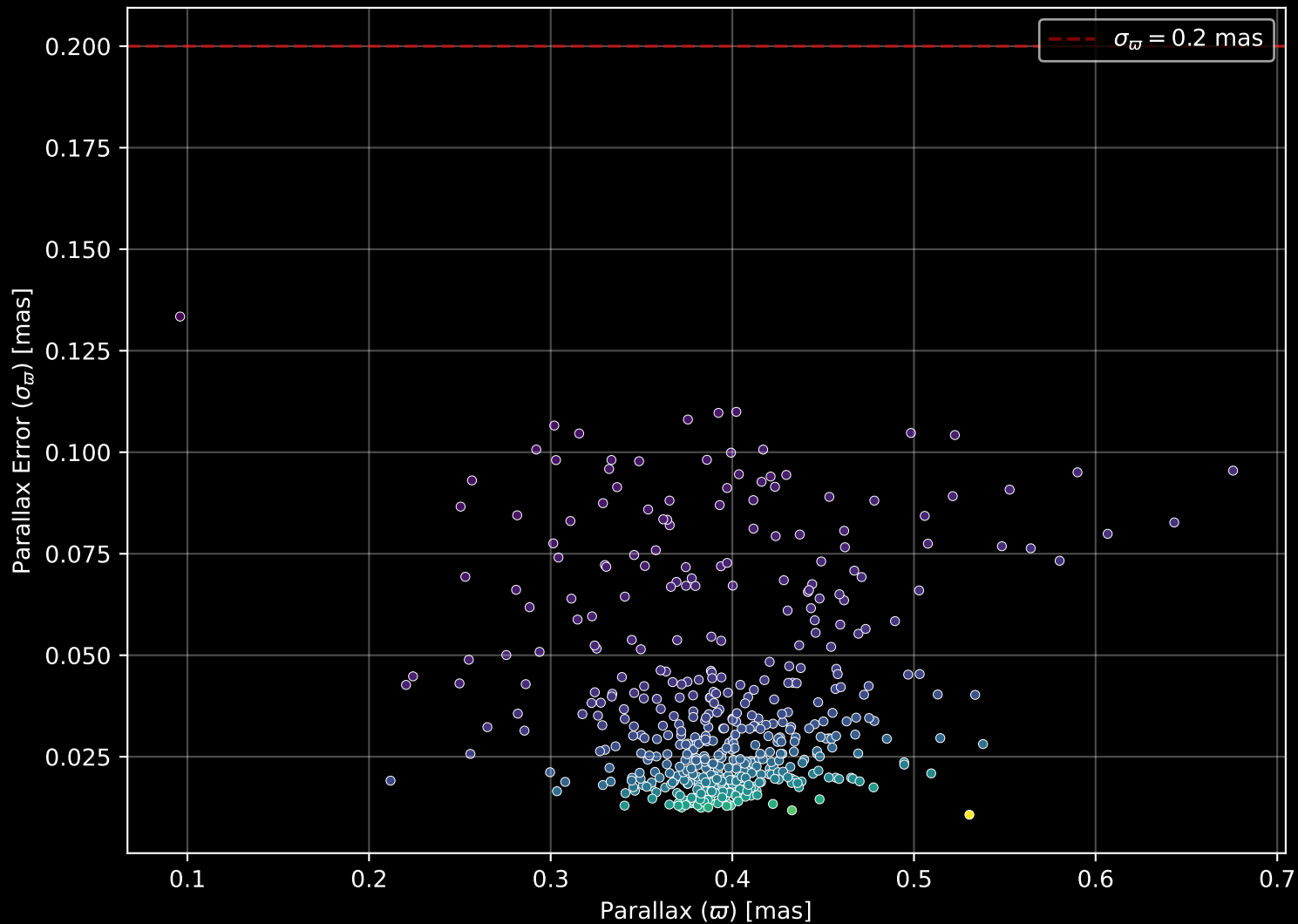
Gaia Cluster: [NGC_3293] Parallax Quality (n= 490)
