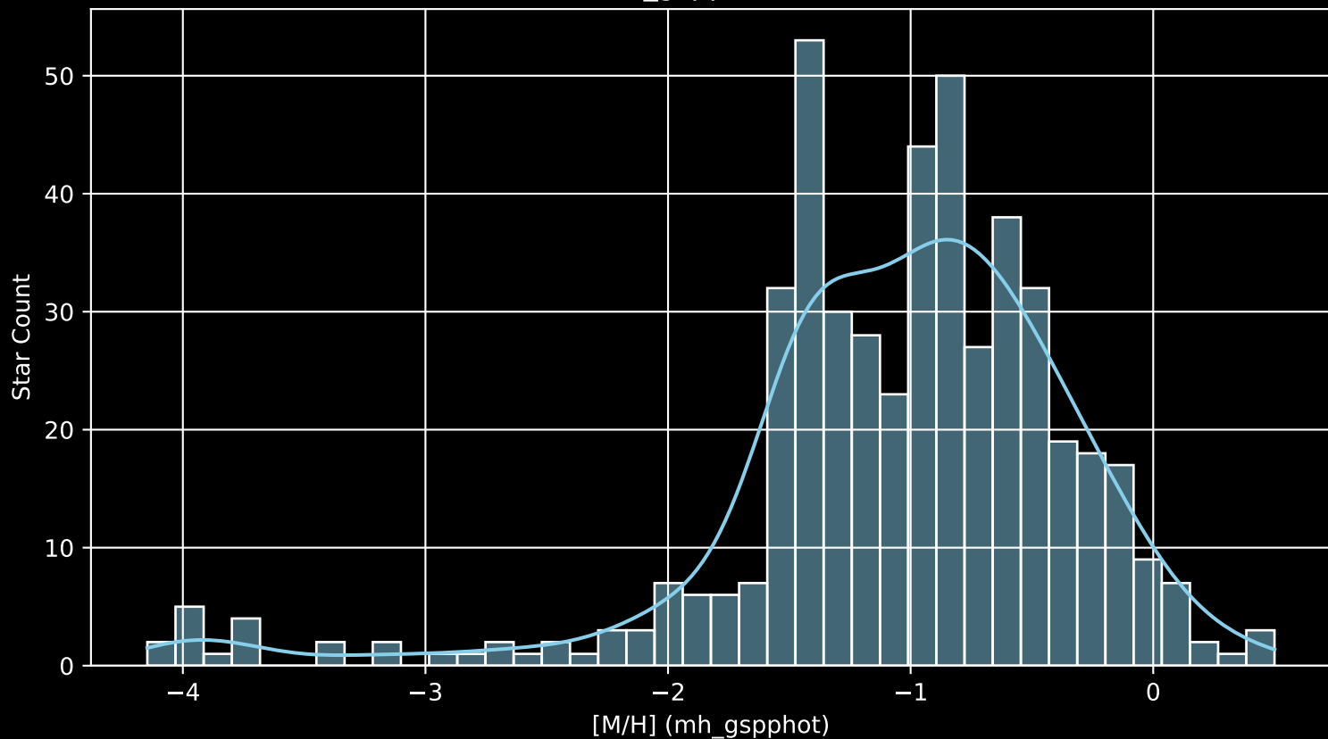
Gaia Cluster: [NGC_3293 [M/H] (mh_gspphot) (n= 489)
