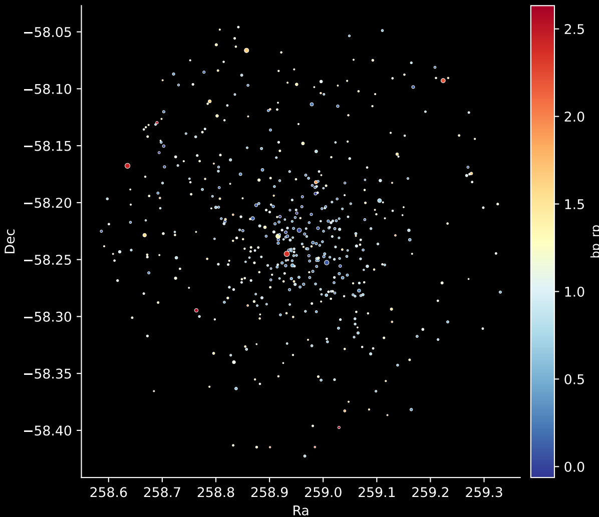
Gaia Cluster: [NGC_3293] Stars: 490
