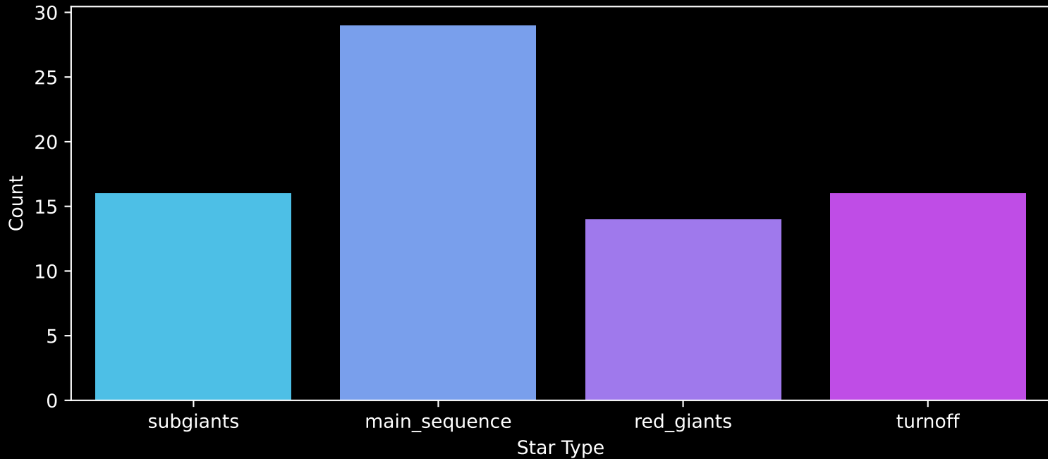
Gaia Cluster: [NGC_3324] Count plot of Star Type
