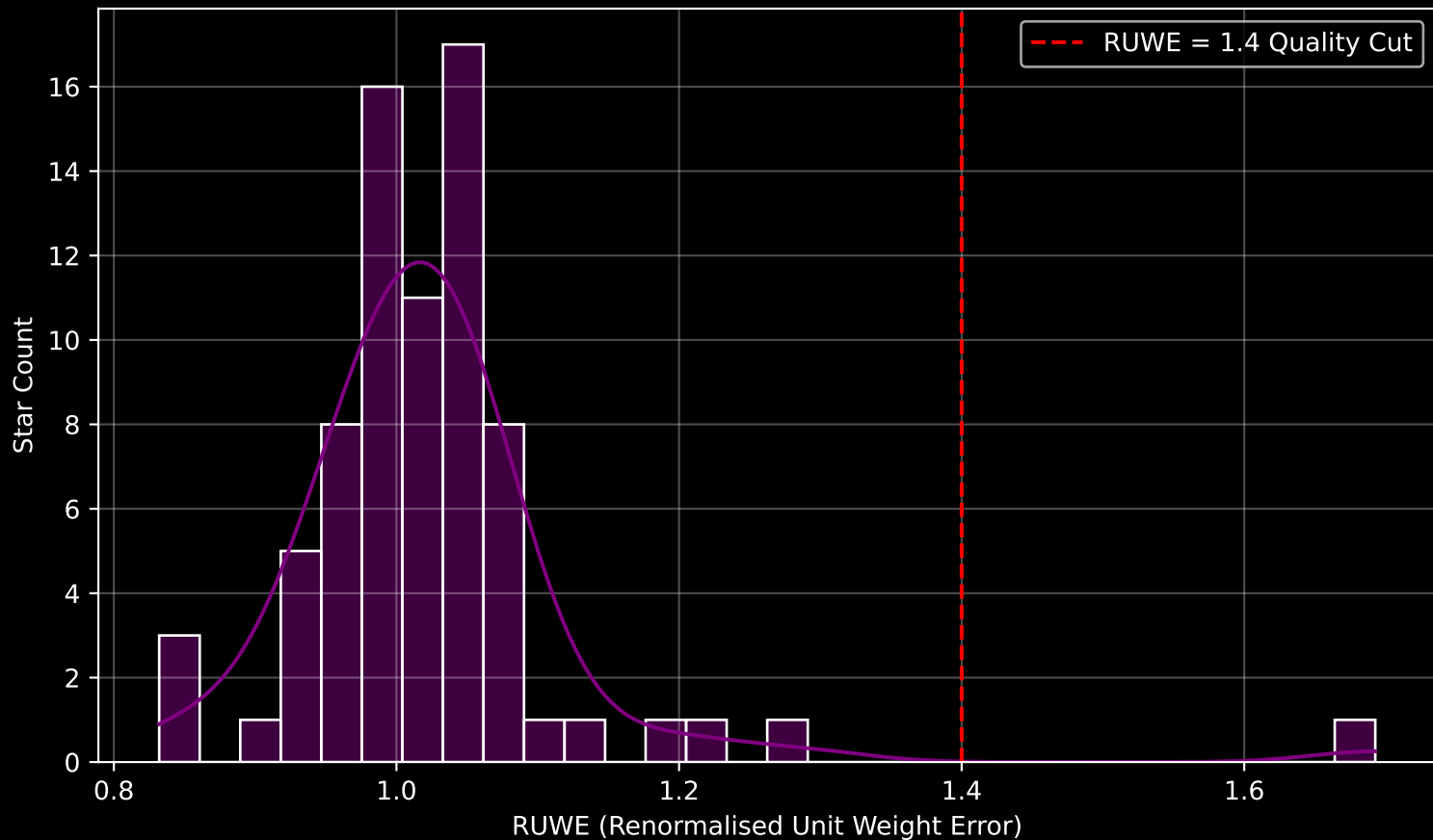
Gaia Cluster: [NGC_3324] RUWE Distribution (n= 75)
