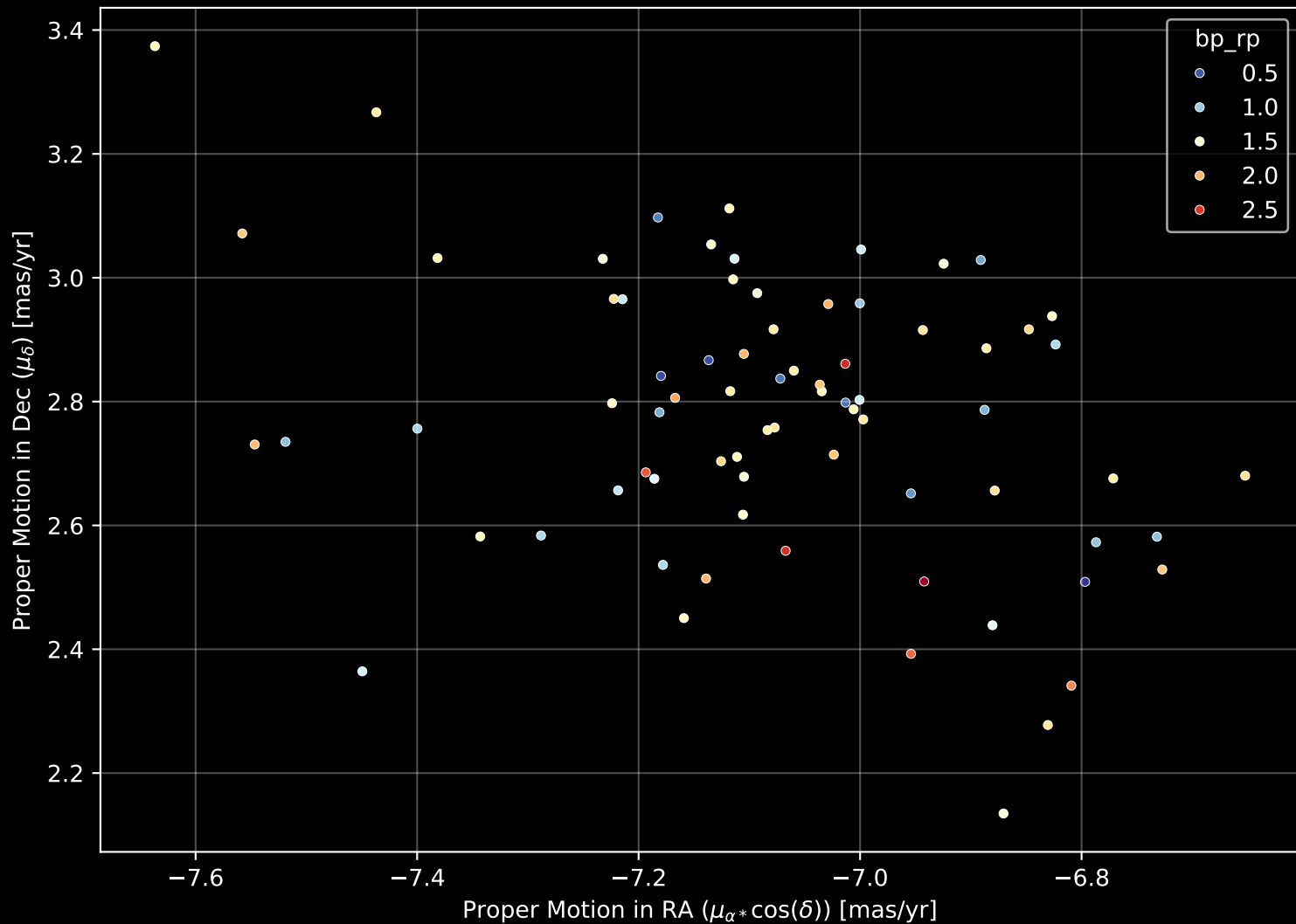
Gaia Cluster: [NGC_3324] Proper Motion Diagram (n= 75)
