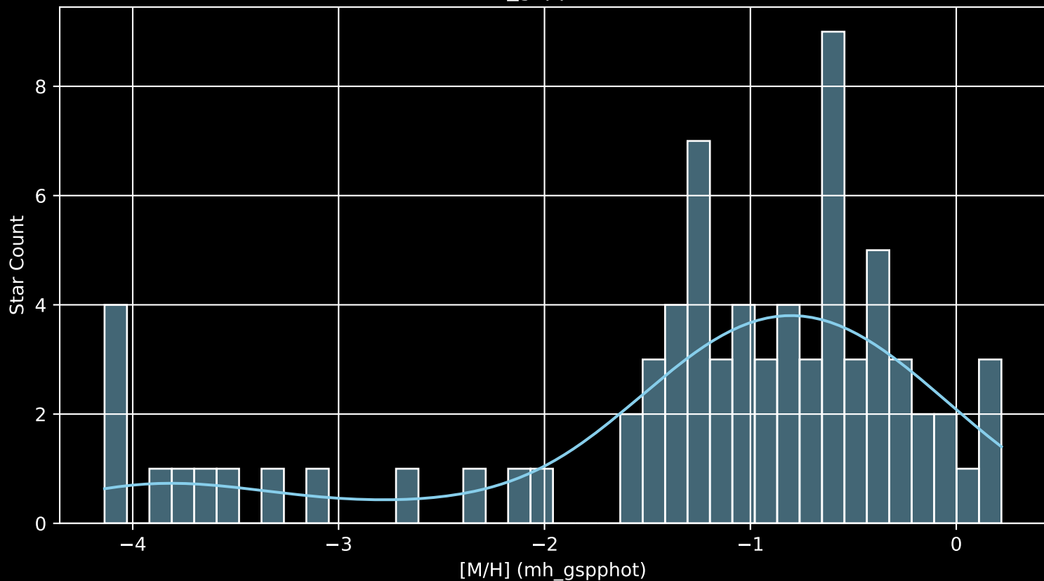
Gaia Cluster: [NGC_3324 [M/H] (mh_gspphot) (n= 75)
