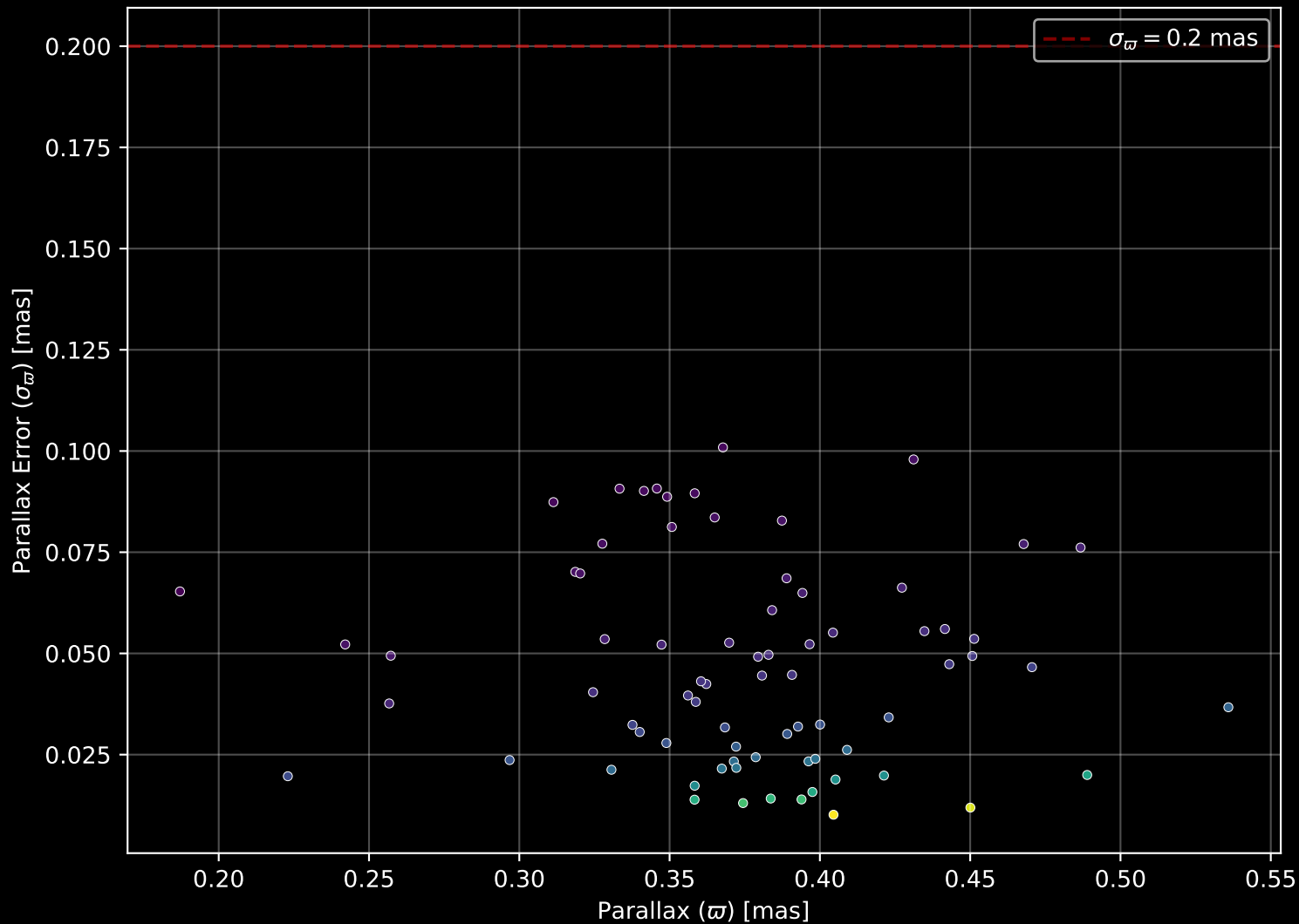
Gaia Cluster: [NGC_3324] Parallax Quality (n= 75)
