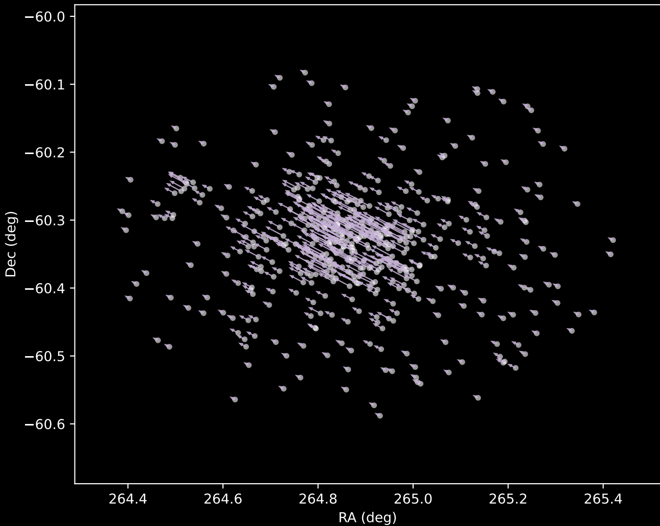
Gaia DR3 Cluster 9 Proper Motion Vectors (n=471)
