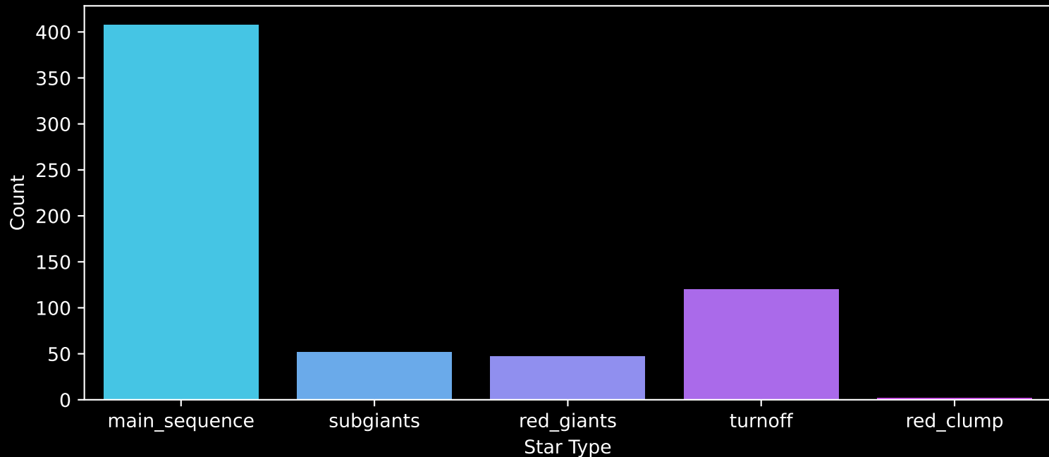
Gaia Cluster: [NGC_3496] Count plot of Star Type
