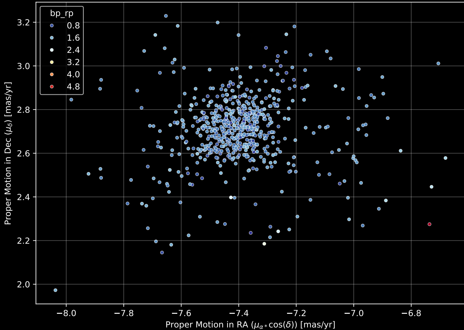
Gaia Cluster: [NGC_3496] Proper Motion Diagram (n= 629)
