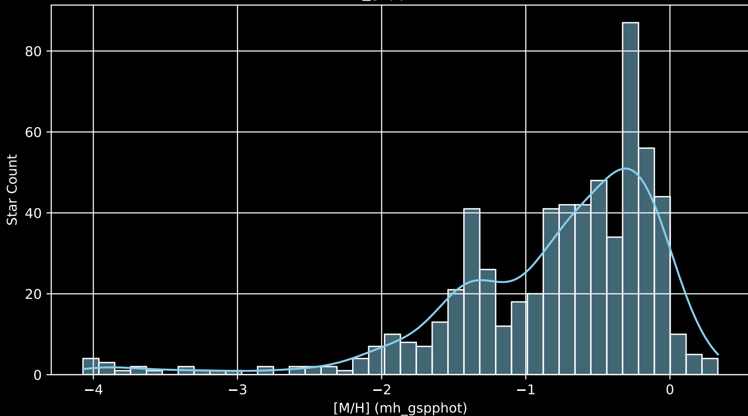
Gaia Cluster: [NGC_3496 [M/H] (mh_gspphot) (n= 625)
