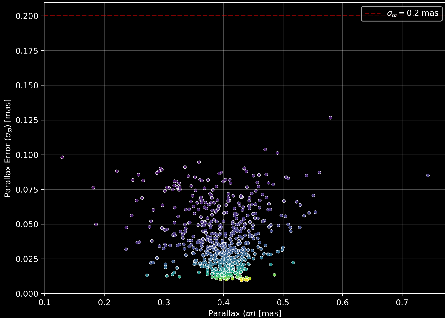
Gaia Cluster: [NGC_3496] Parallax Quality (n= 629)
