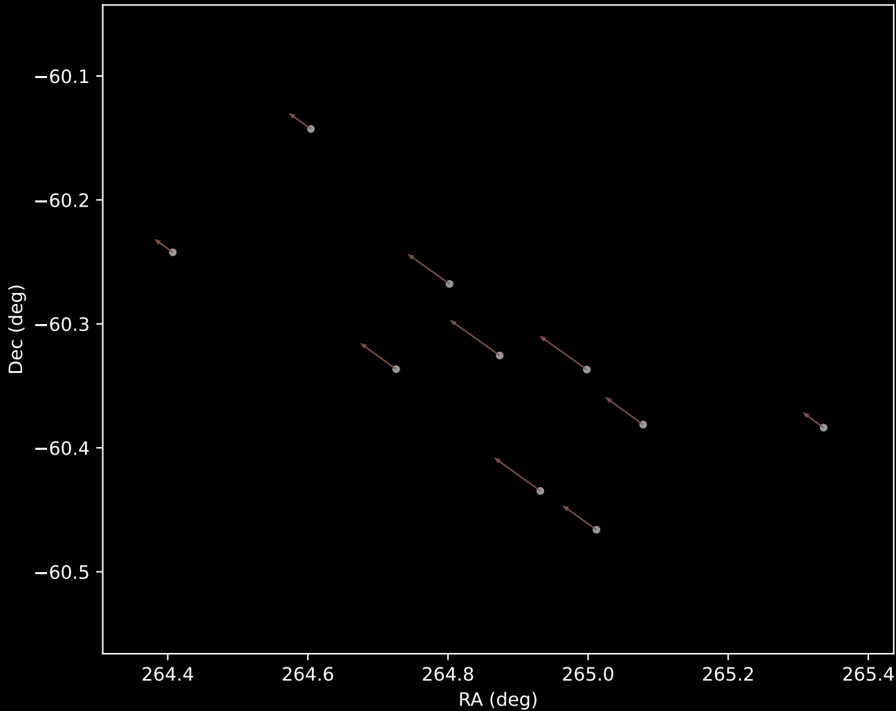
Gaia DR3 Cluster 10 Proper Motion Vectors (n=10)
