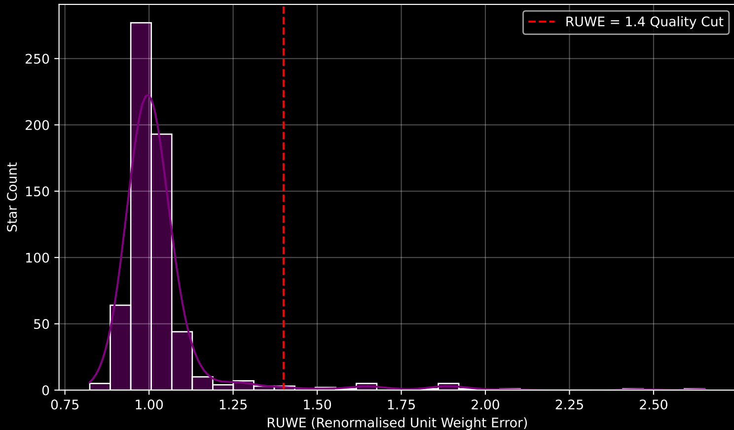
Gaia Cluster: [NGC_3496] RUWE Distribution (n= 629)
