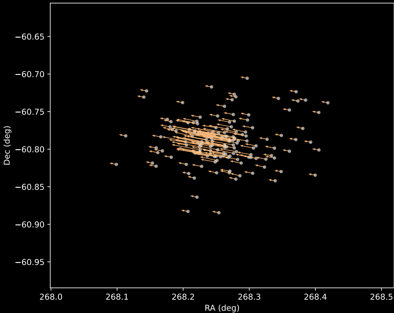
Gaia DR3 Cluster 3 Proper Motion Vectors (n=154)
