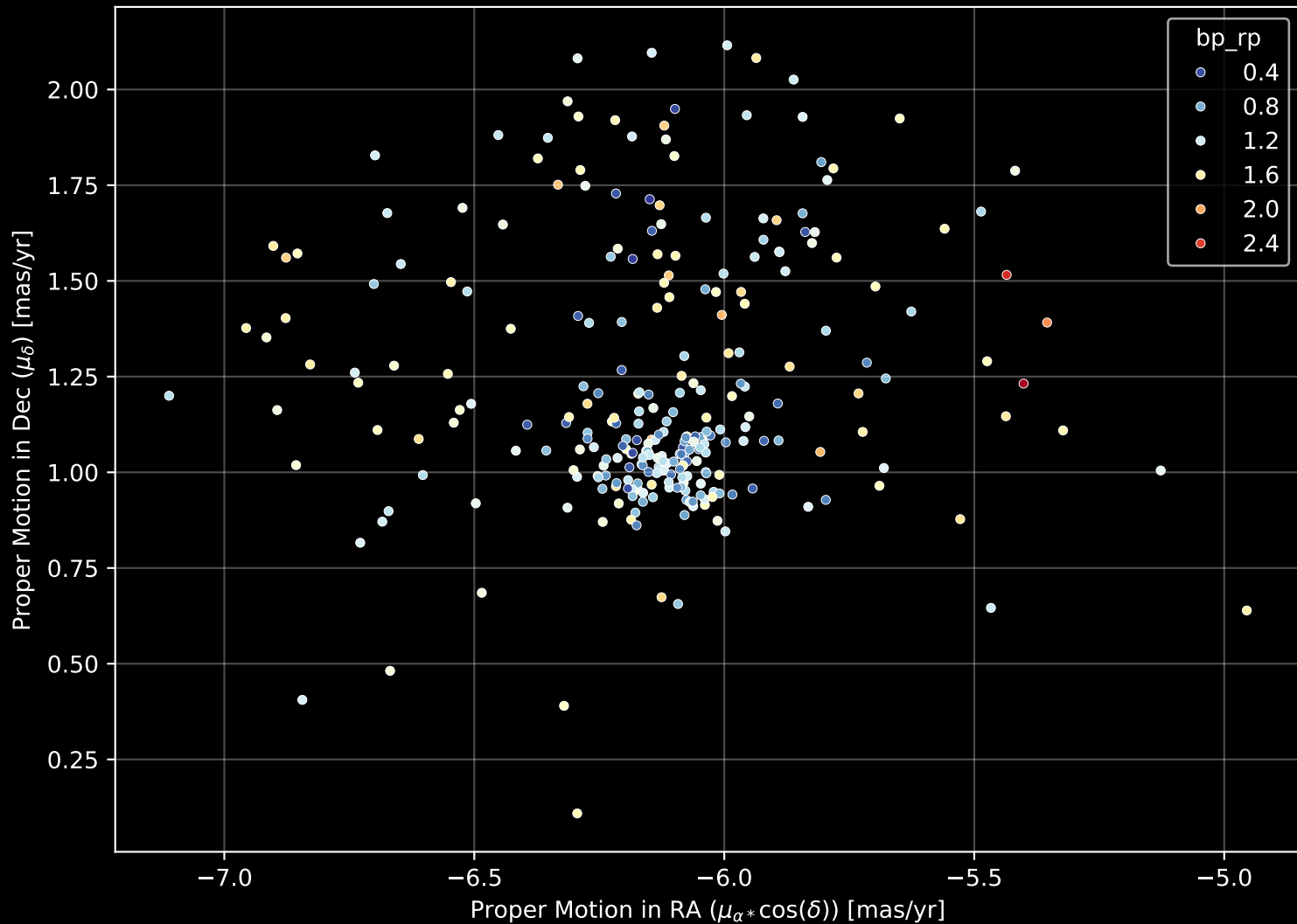
Gaia Cluster: [NGC_3590] Proper Motion Diagram (n= 282)
