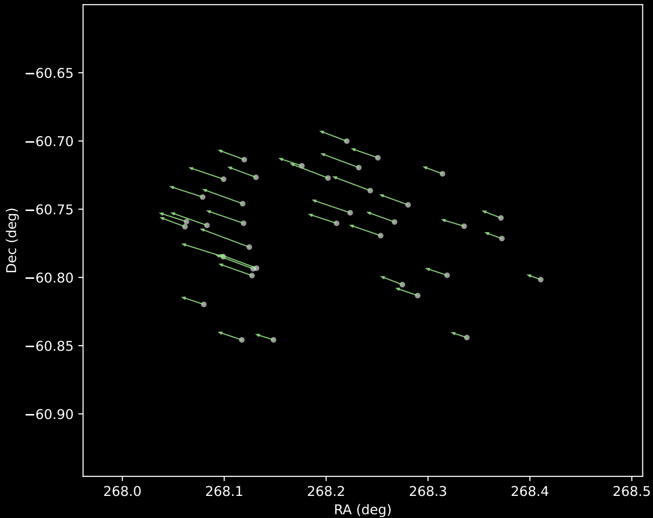
Gaia DR3 Cluster 5 Proper Motion Vectors (n=37)
