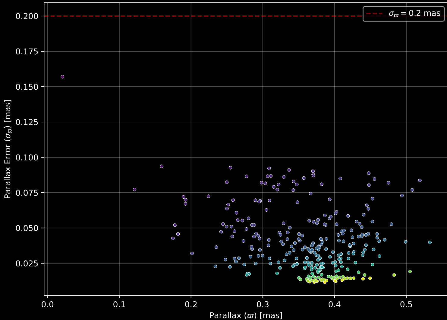
Gaia Cluster: [NGC_3590] Parallax Quality (n= 282)
