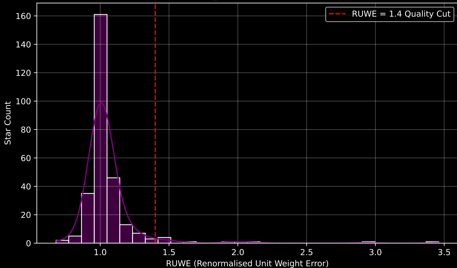
Gaia Cluster: [NGC_3590] RUWE Distribution (n= 282)
