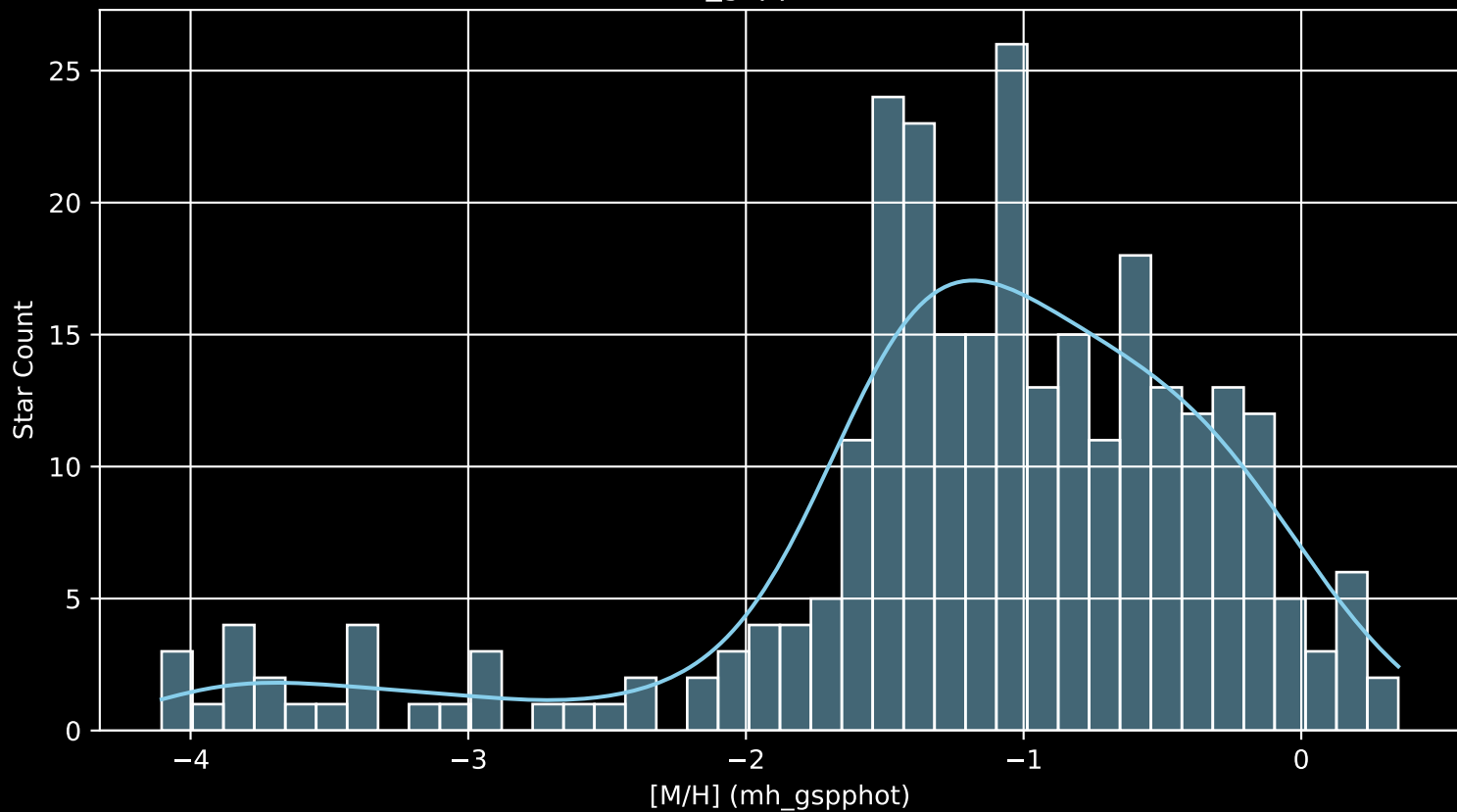
Gaia Cluster: [NGC_3590 [M/H] (mh_gspphot) (n= 281)
