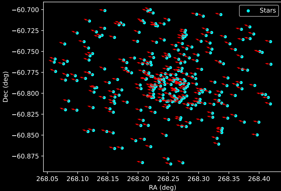
Gaia Cluster: [NGC_3590] Proper Motion Vectors for Gaia Star Field (n= 282)
