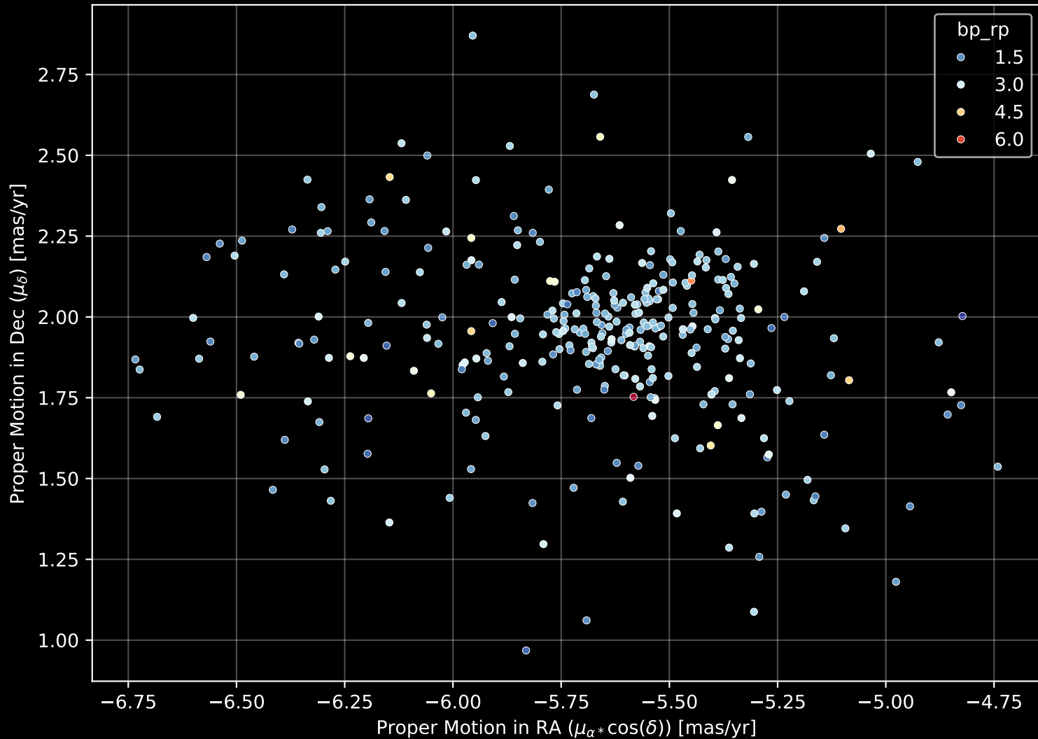
Gaia Cluster: [NGC_3603] Proper Motion Diagram (n= 327)
