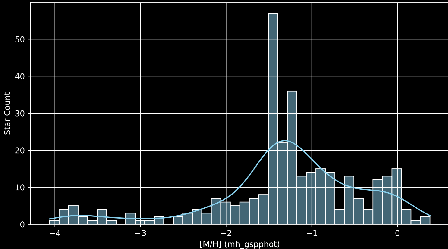
Gaia Cluster: [NGC_3603 [M/H] (mh_gspphot) (n= 322)
