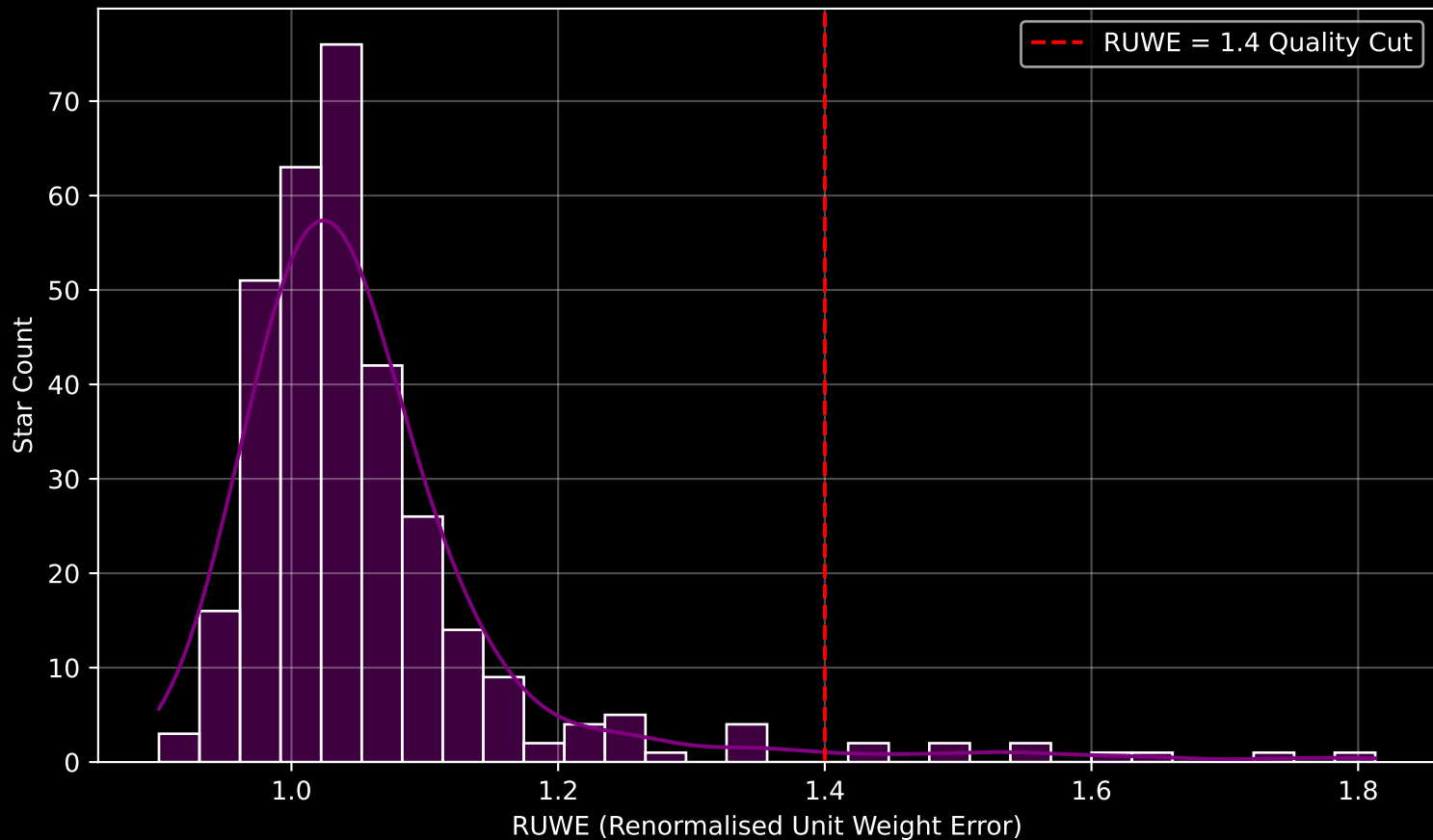
Gaia Cluster: [NGC_3603] RUWE Distribution (n= 326)
