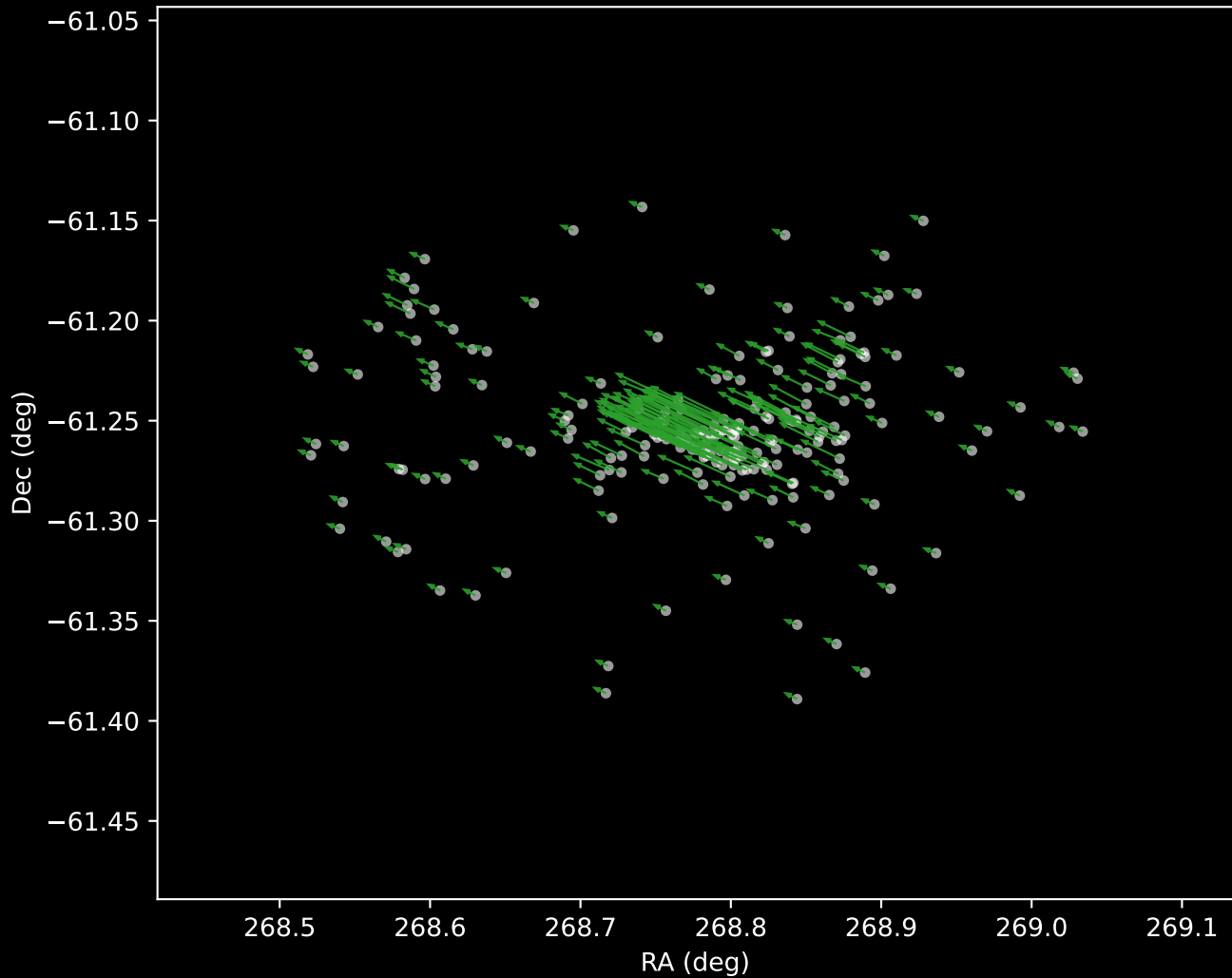
Gaia DR3 Cluster 4 Proper Motion Vectors (n=214)
