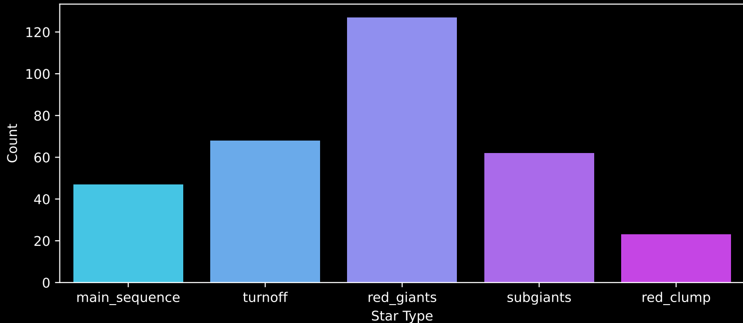
Gaia Cluster: [NGC_3603] Count plot of Star Type
