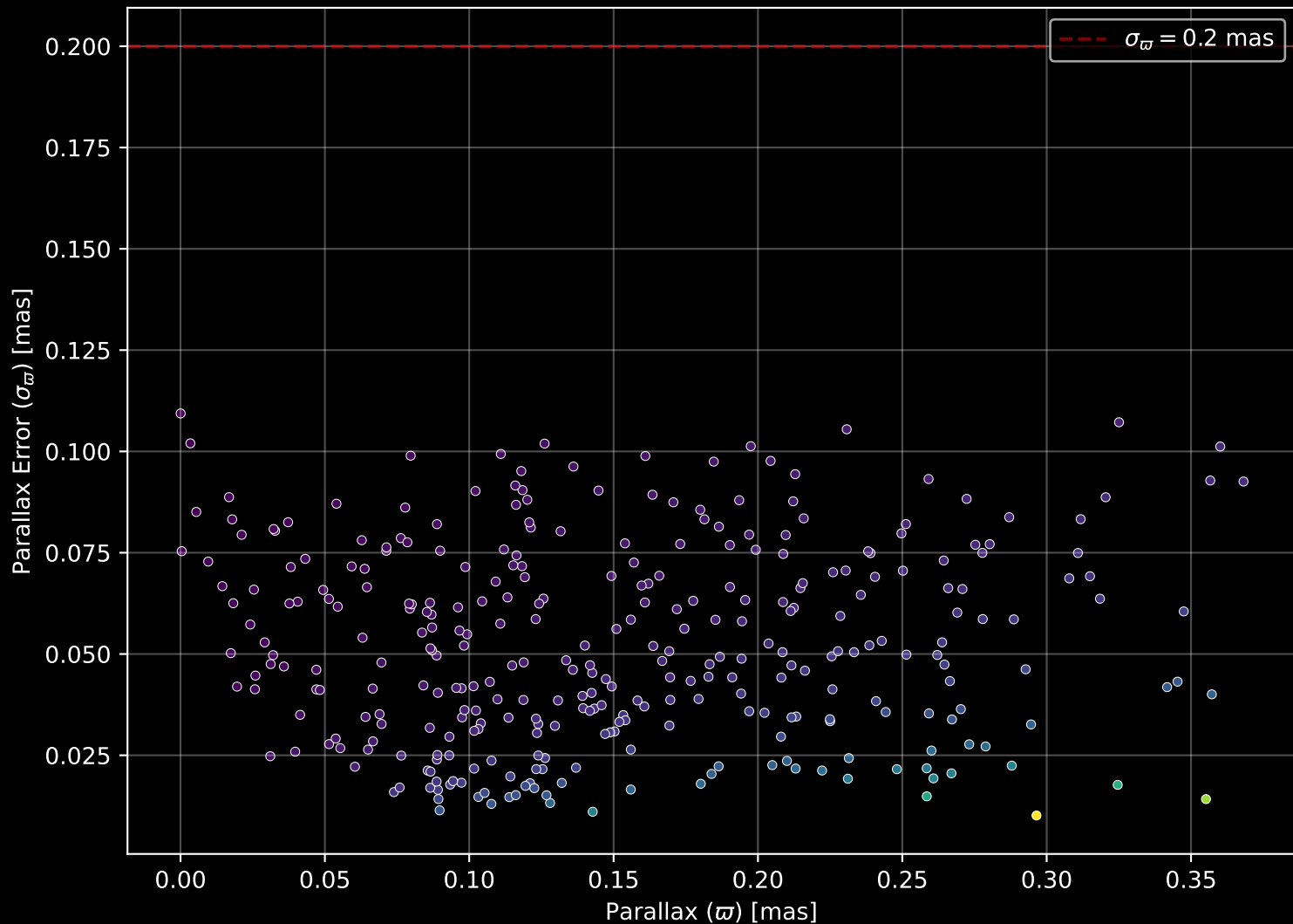
Gaia Cluster: [NGC_3603] Parallax Quality (n= 327)
