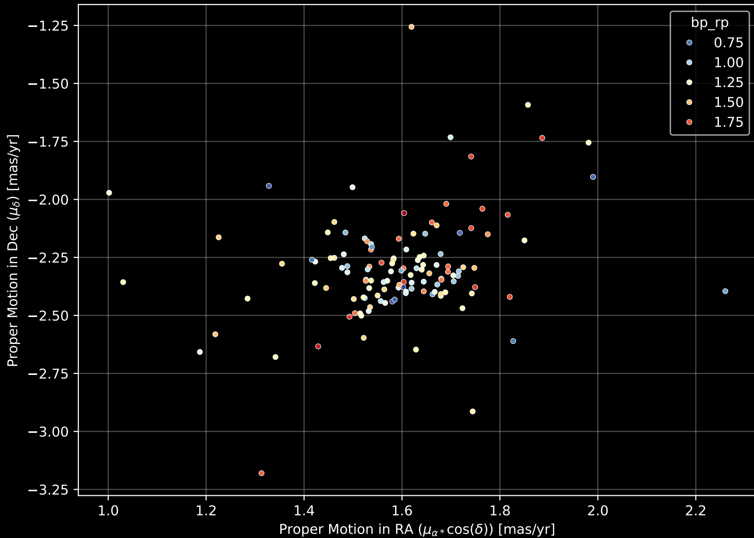
Gaia Cluster: [NGC_381] Proper Motion Diagram (n= 126)
