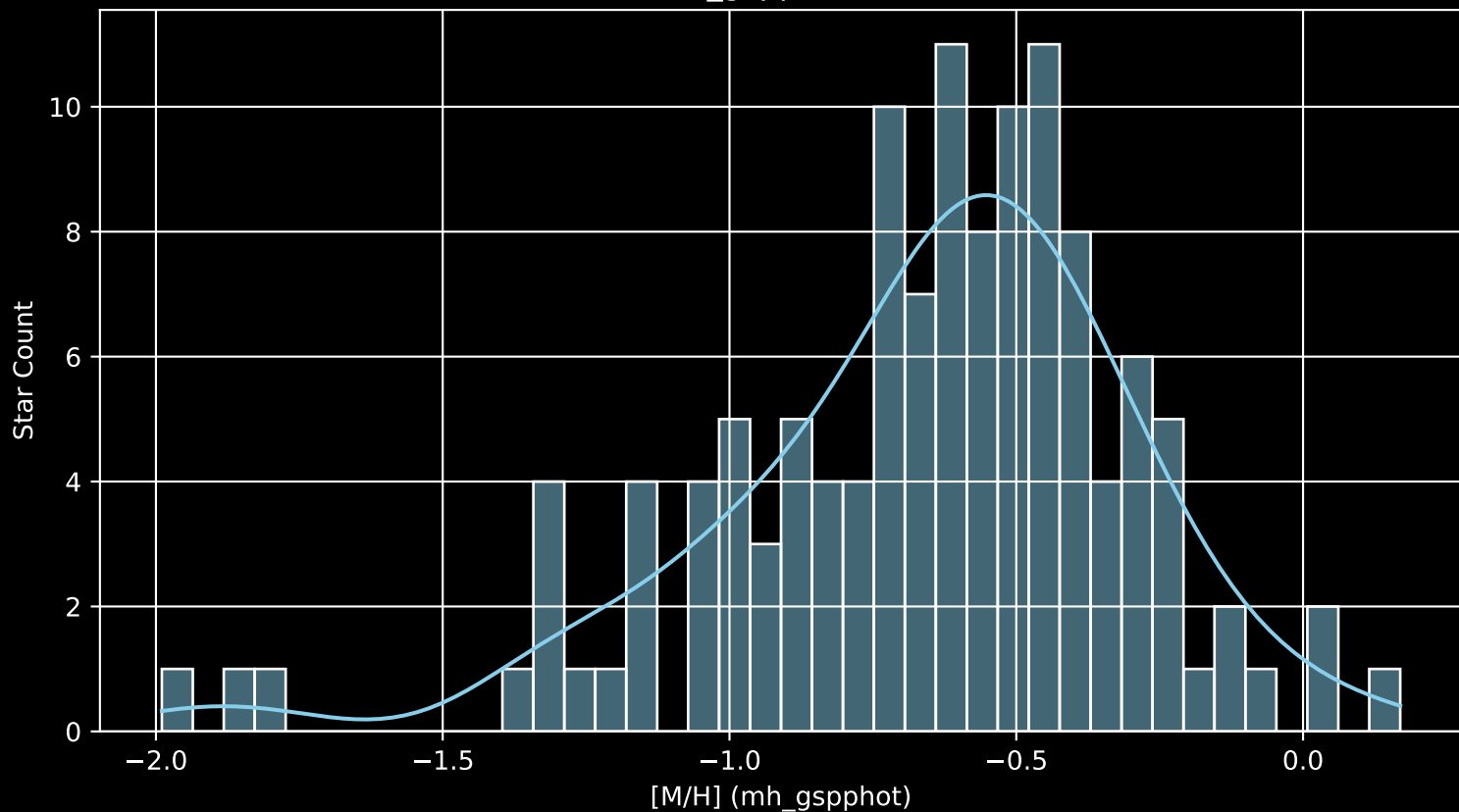
Gaia Cluster: [NGC_381 [M/H] (mh_gspphot) (n= 126)
