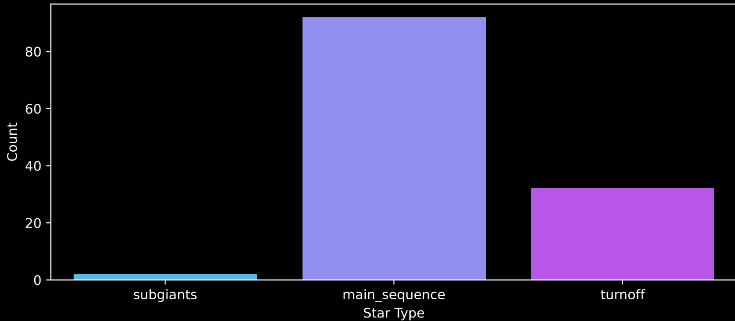
Gaia Cluster: [NGC_381] Count plot of Star Type
