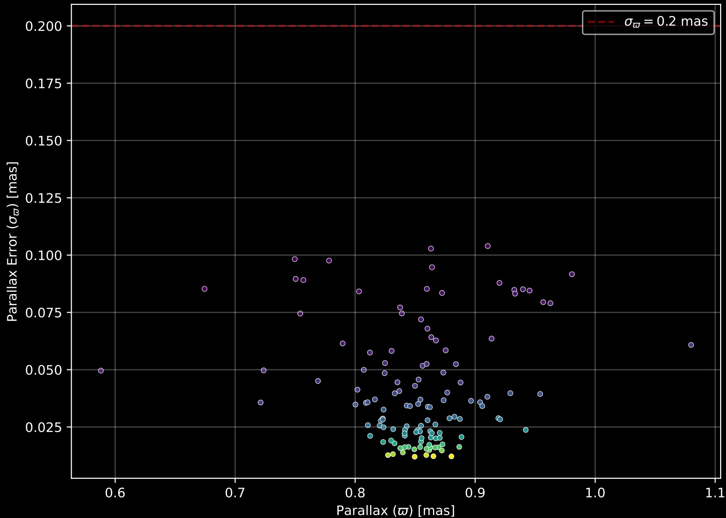
Gaia Cluster: [NGC_381] Parallax Quality (n= 126)
