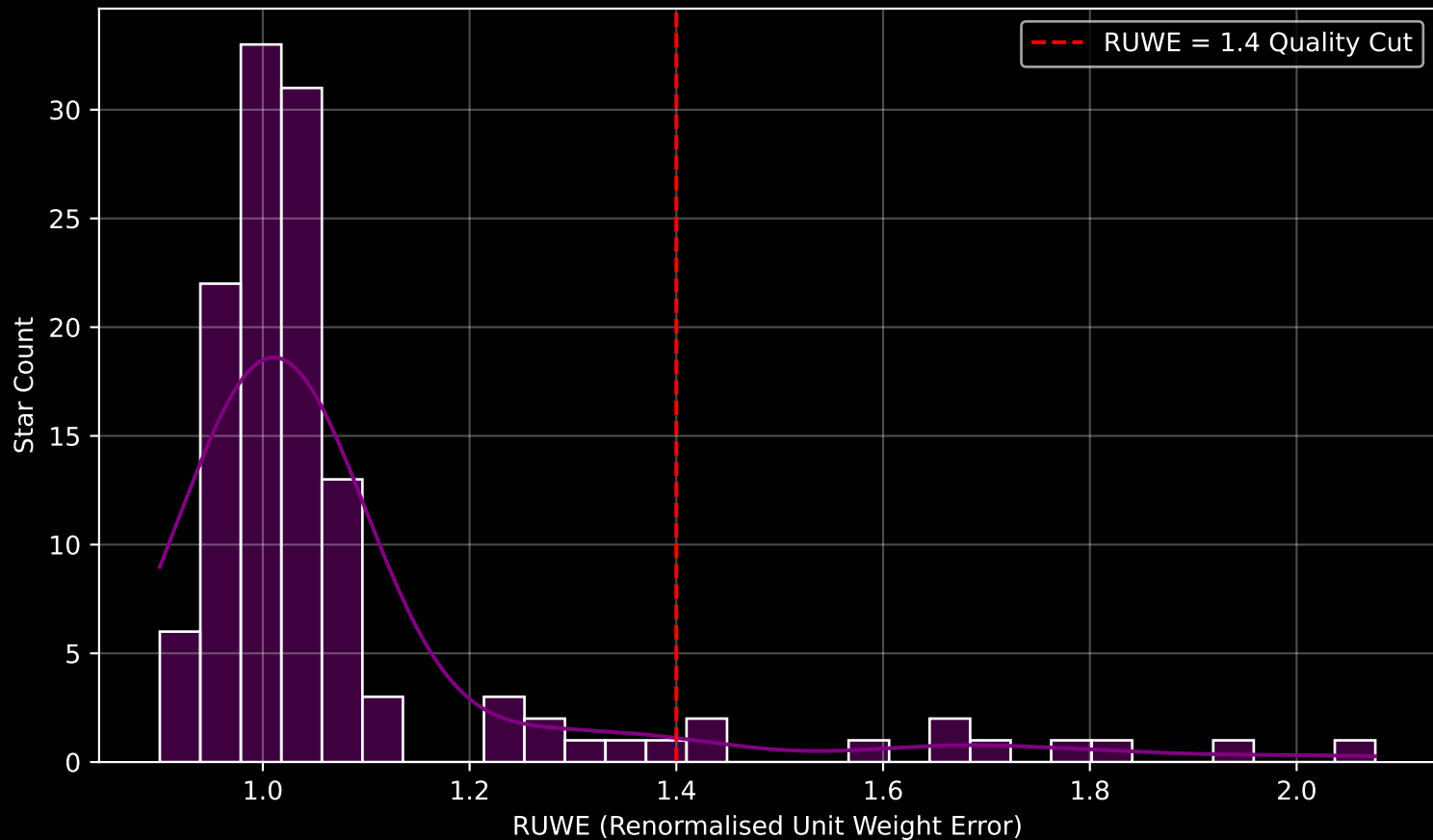
Gaia Cluster: [NGC_381] RUWE Distribution (n= 126)
