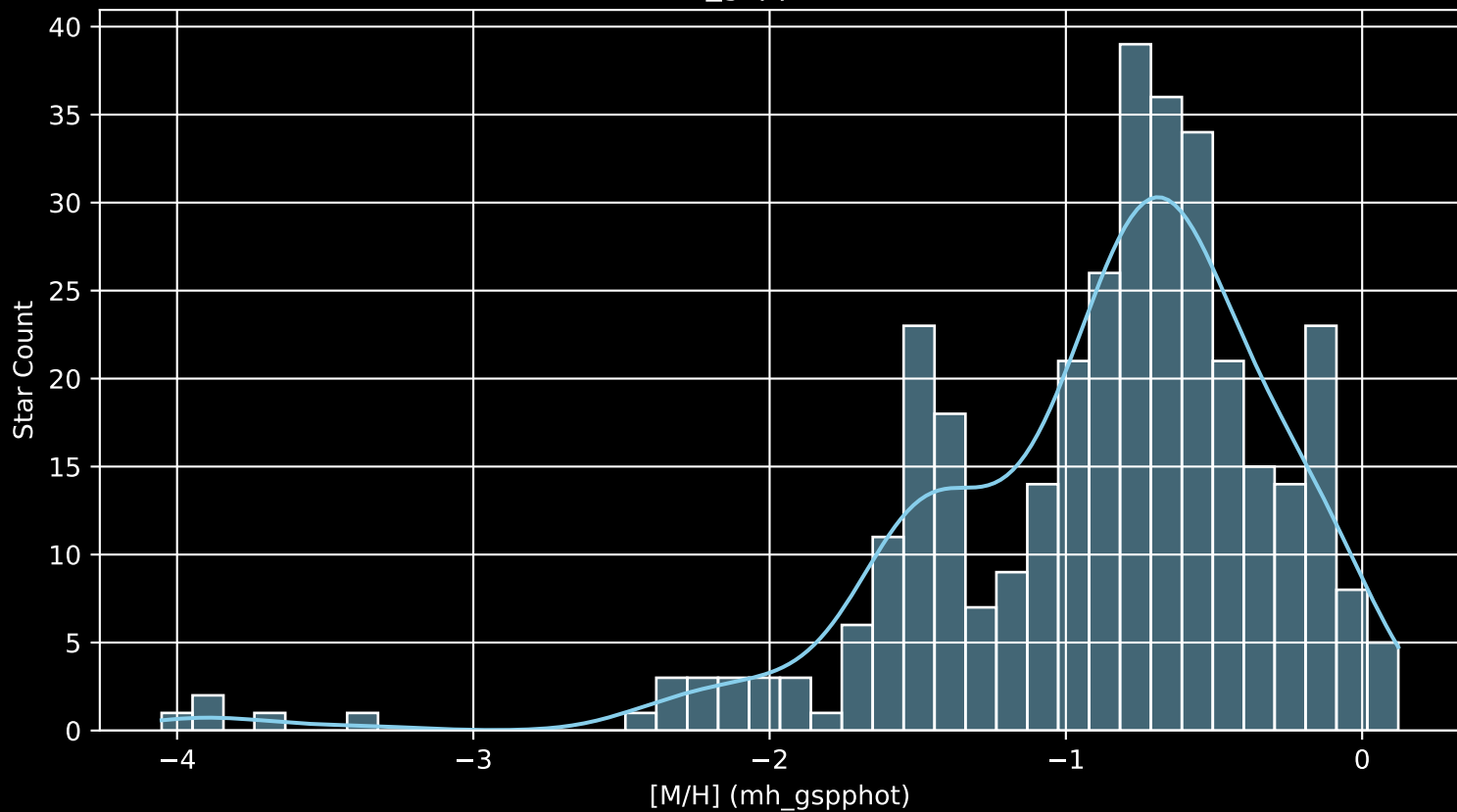
Gaia Cluster: [NGC_3960 [M/H] (mh_gspphot) (n= 352)
