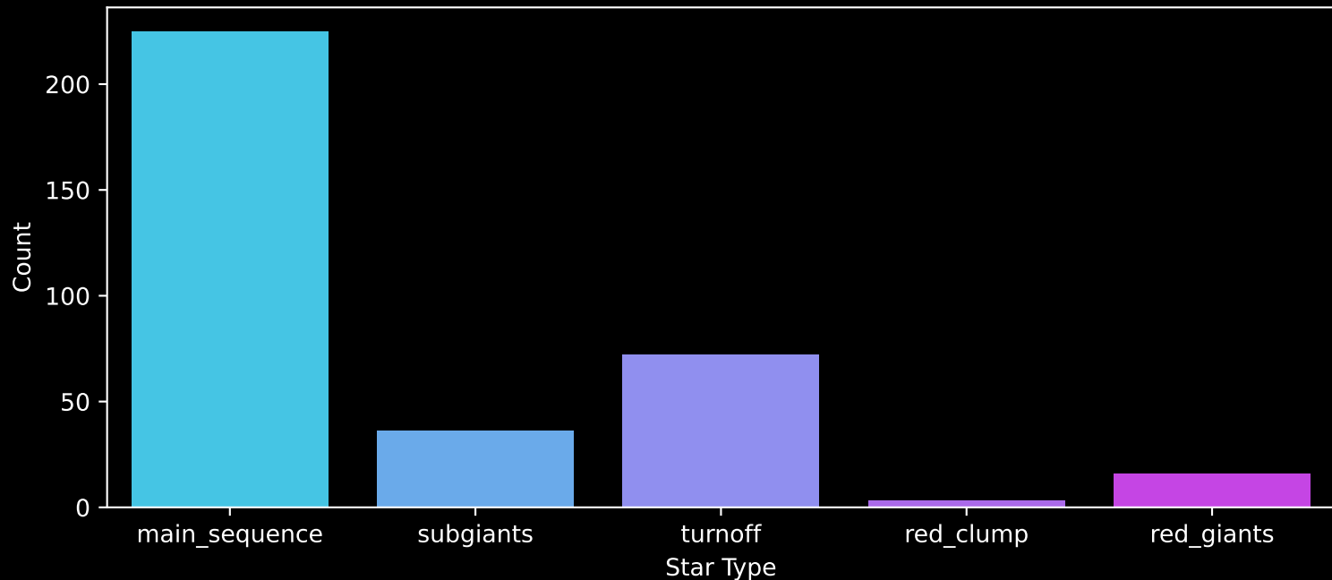
Gaia Cluster: [NGC_3960] Count plot of Star Type
