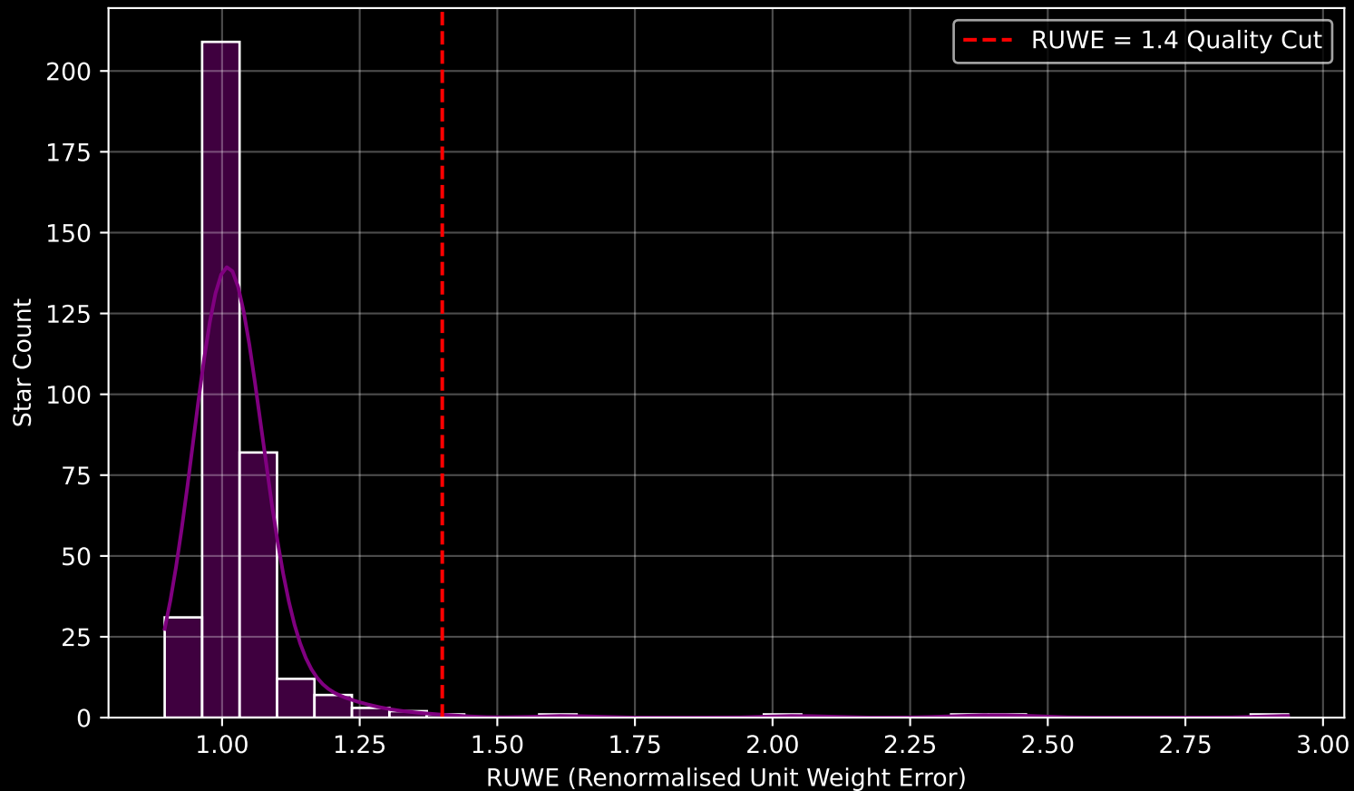
Gaia Cluster: [NGC_3960] RUWE Distribution (n= 352)
