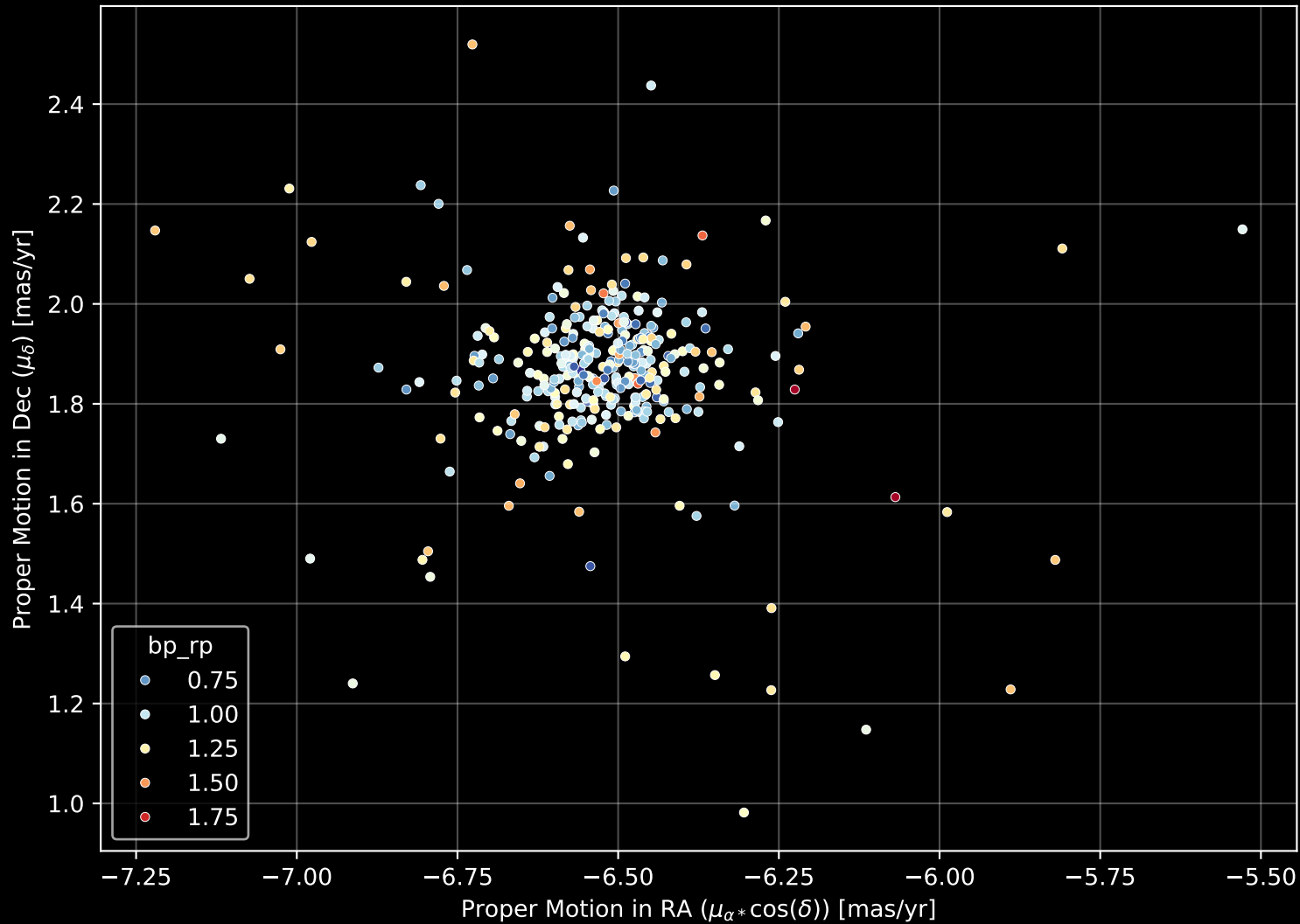
Gaia Cluster: [NGC_3960] Proper Motion Diagram (n= 352)
