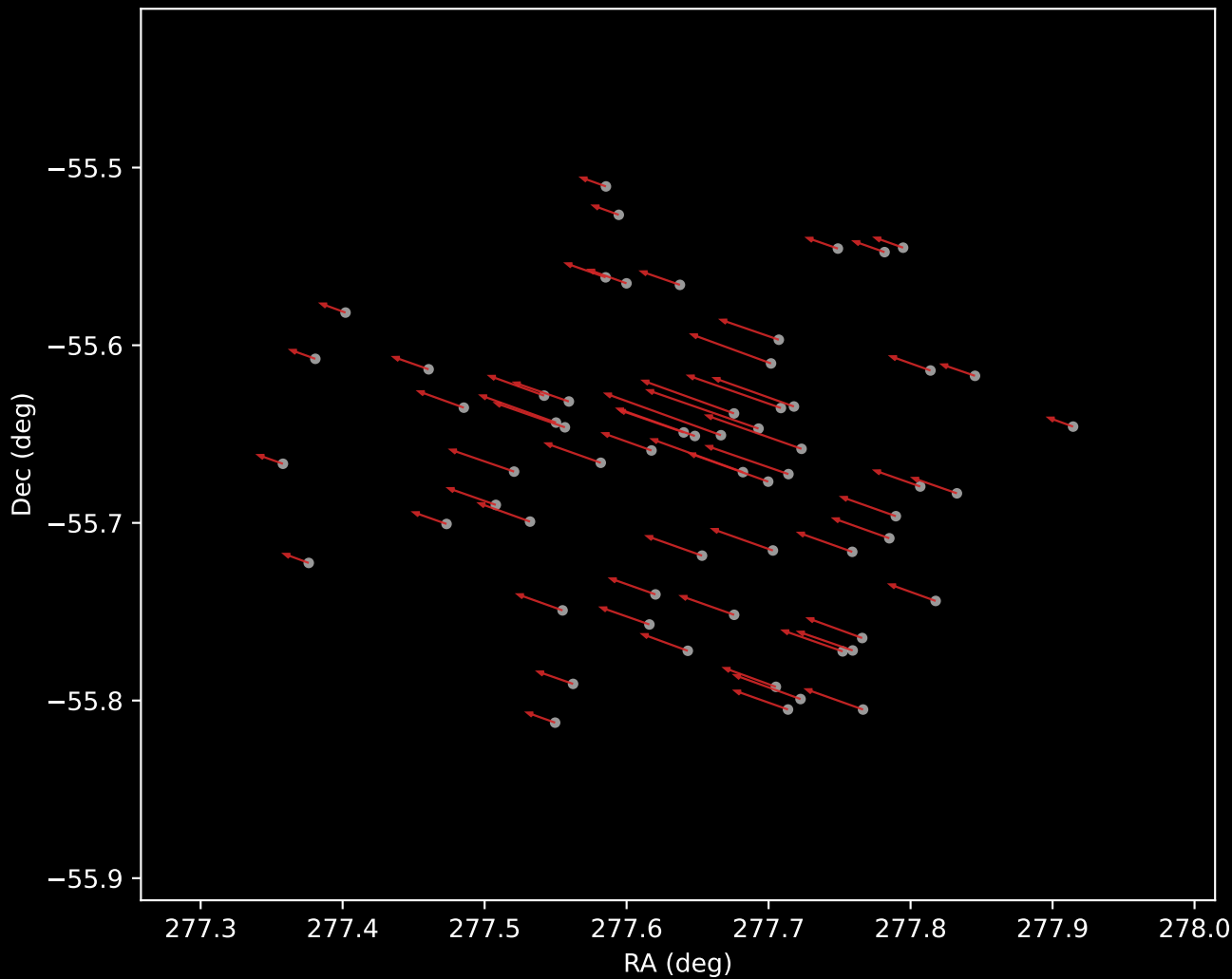
Gaia DR3 Cluster 6 Proper Motion Vectors (n=62)
