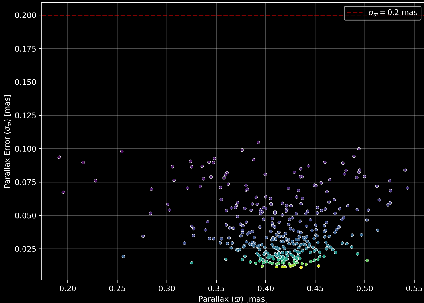
Gaia Cluster: [NGC_3960] Parallax Quality (n= 352)
