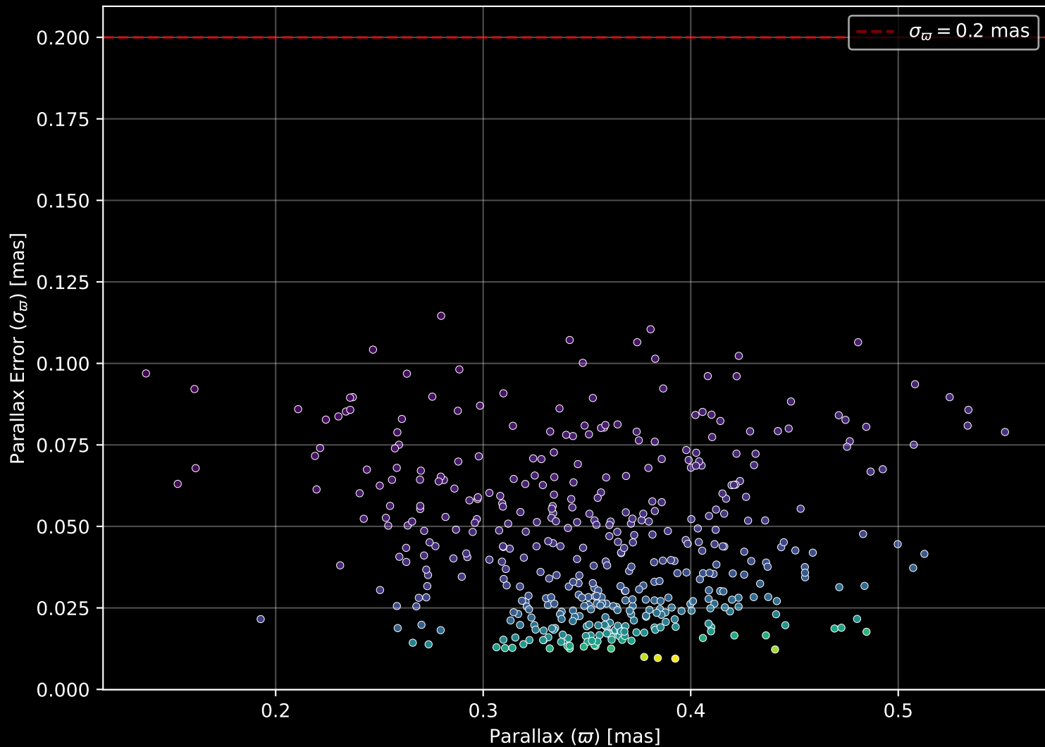
Gaia Cluster: [NGC_4052] Parallax Quality (n= 443)
