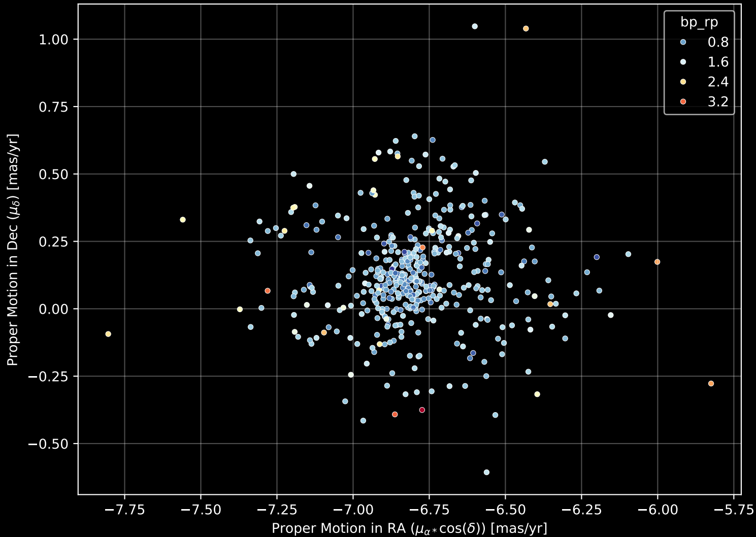
Gaia Cluster: [NGC_4052] Proper Motion Diagram (n= 443)
