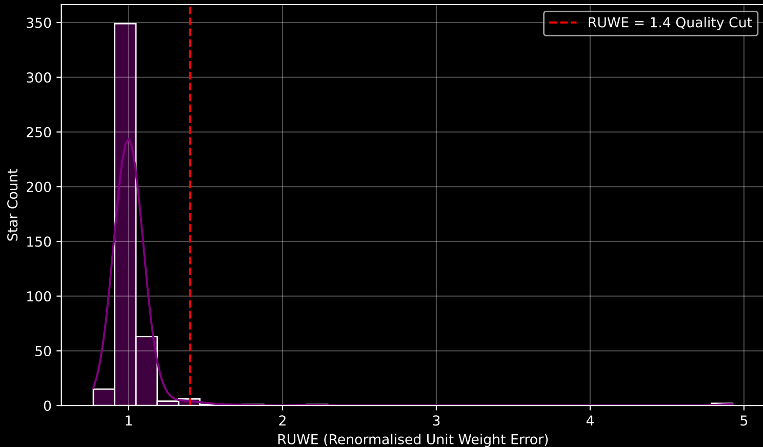
Gaia Cluster: [NGC_4052] RUWE Distribution (n= 442)
