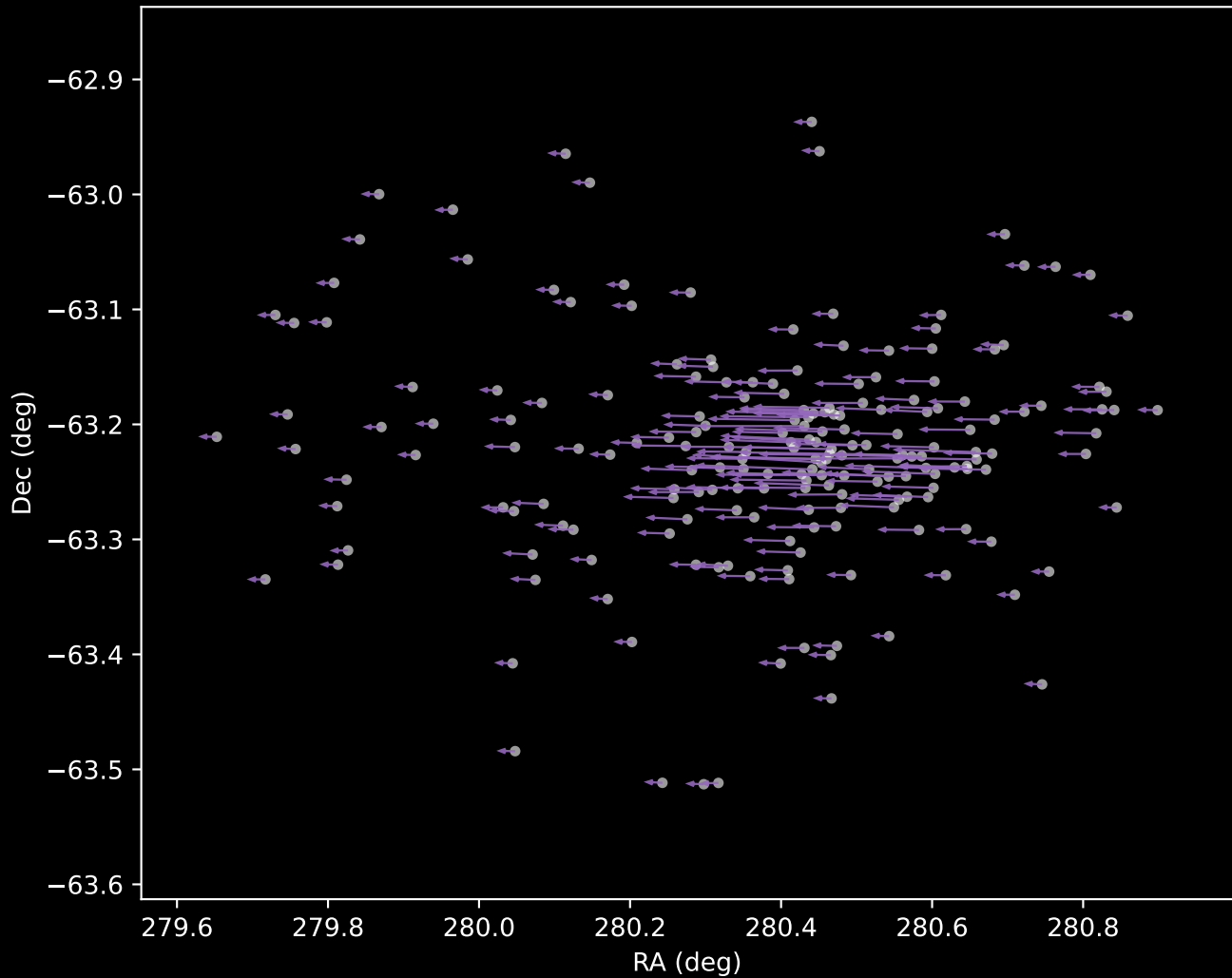
Gaia DR3 Cluster 8 Proper Motion Vectors (n=201)
