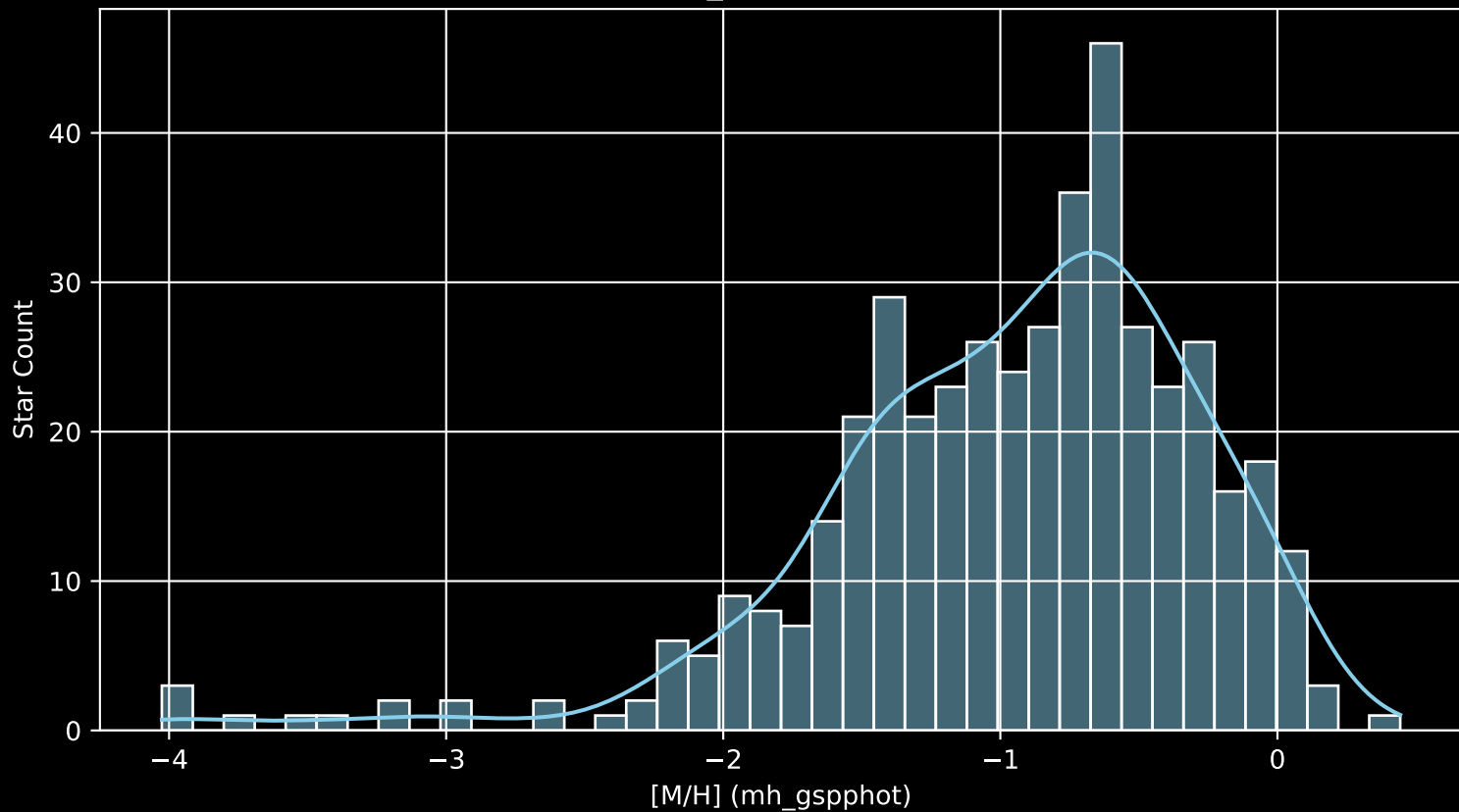
Gaia Cluster: [NGC_4052 [M/H] (mh_gspphot) (n= 443)
