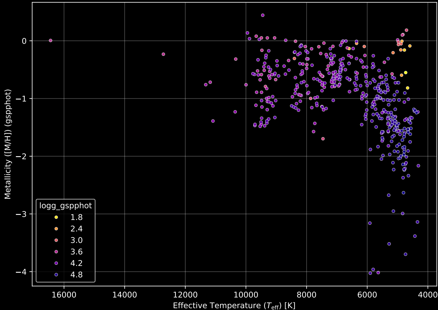
Gaia Cluster: [NGC_4052] Stellar Population Parameters (n= 443)
