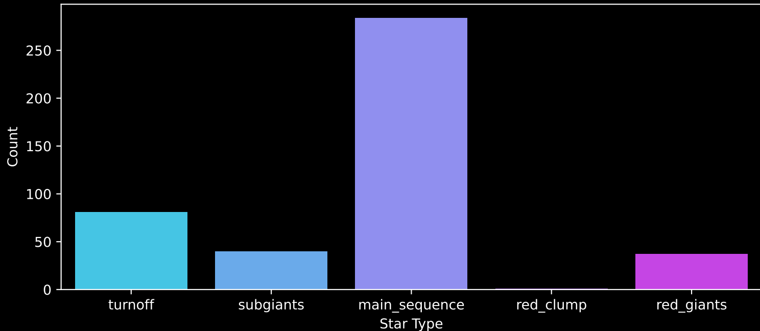
Gaia Cluster: [NGC_4052] Count plot of Star Type
