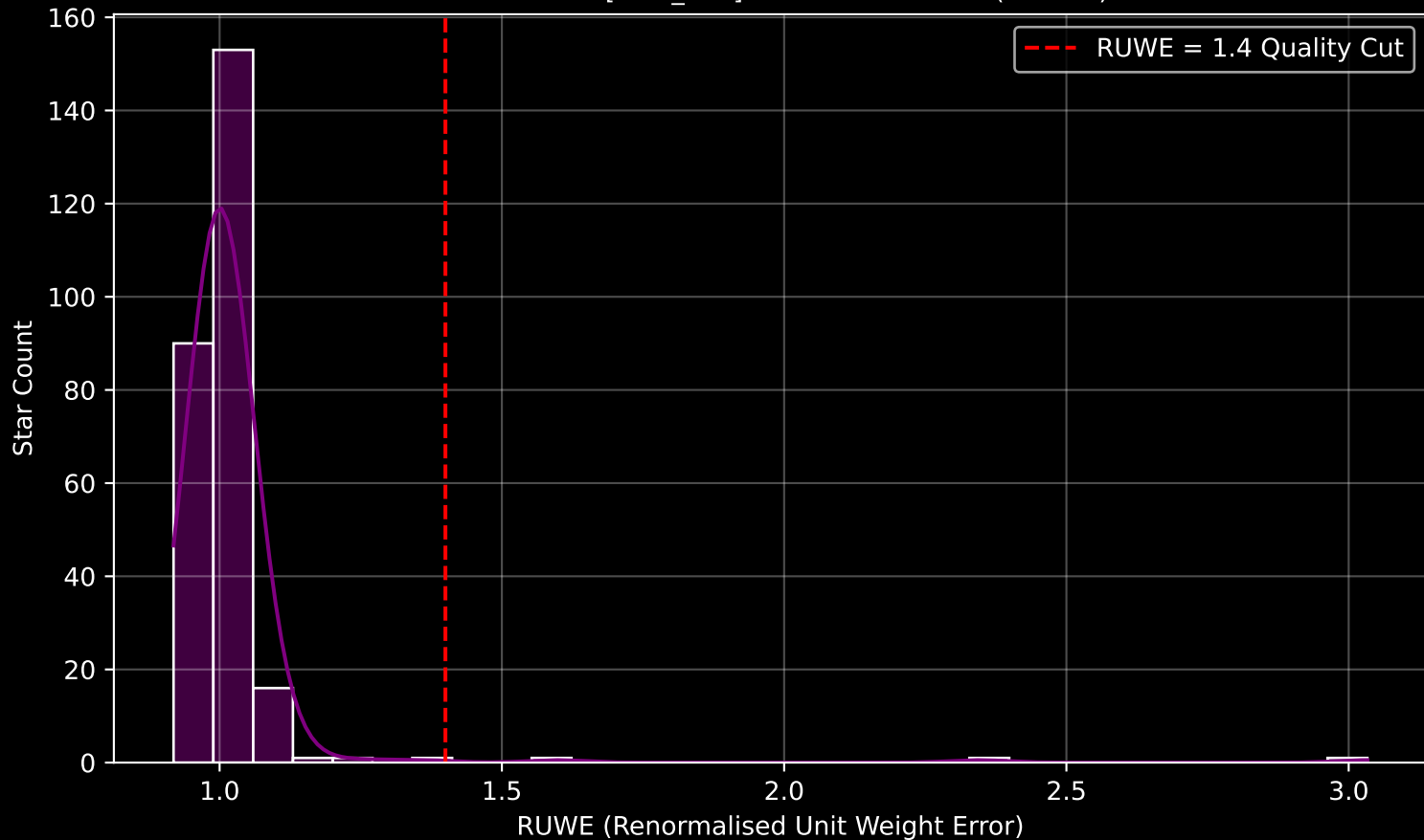
Gaia Cluster: [NGC_436] RUWE Distribution (n= 265)
