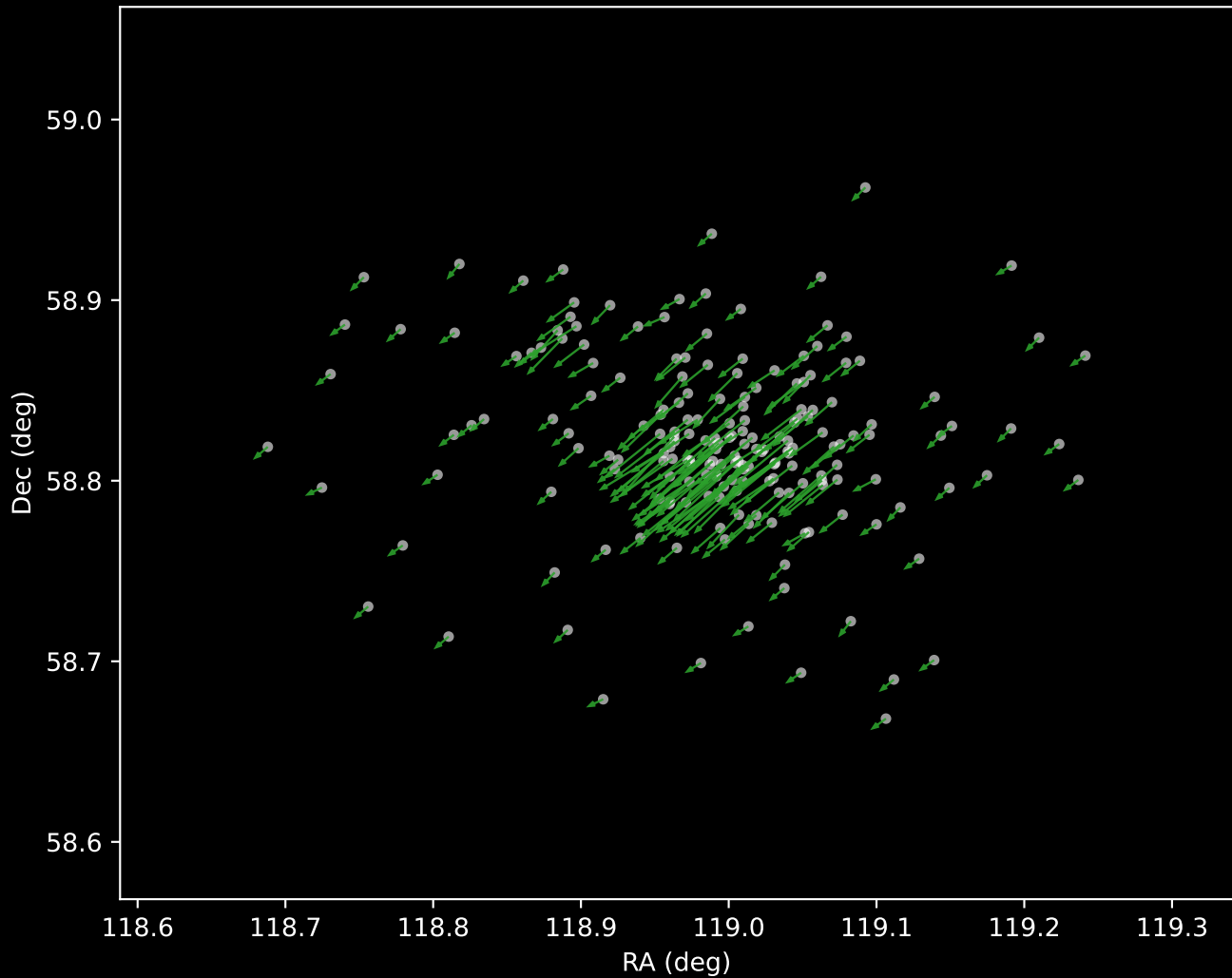
Gaia DR3 Cluster 4 Proper Motion Vectors (n=193)
