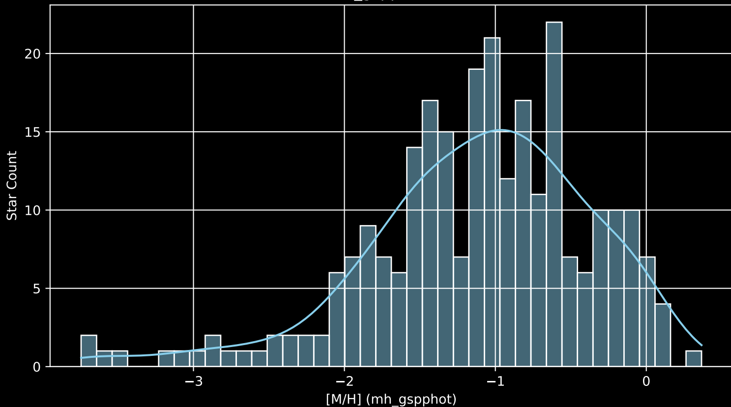
Gaia Cluster: [NGC_436 [M/H] (mh_gspphot) (n= 265)
