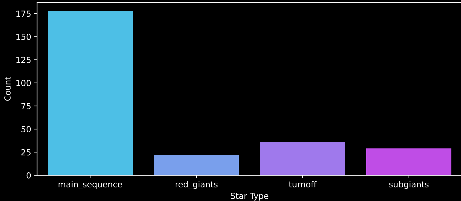
Gaia Cluster: [NGC_436] Count plot of Star Type
