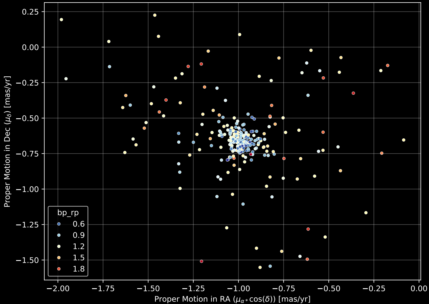
Gaia Cluster: [NGC_436] Proper Motion Diagram (n= 265)
