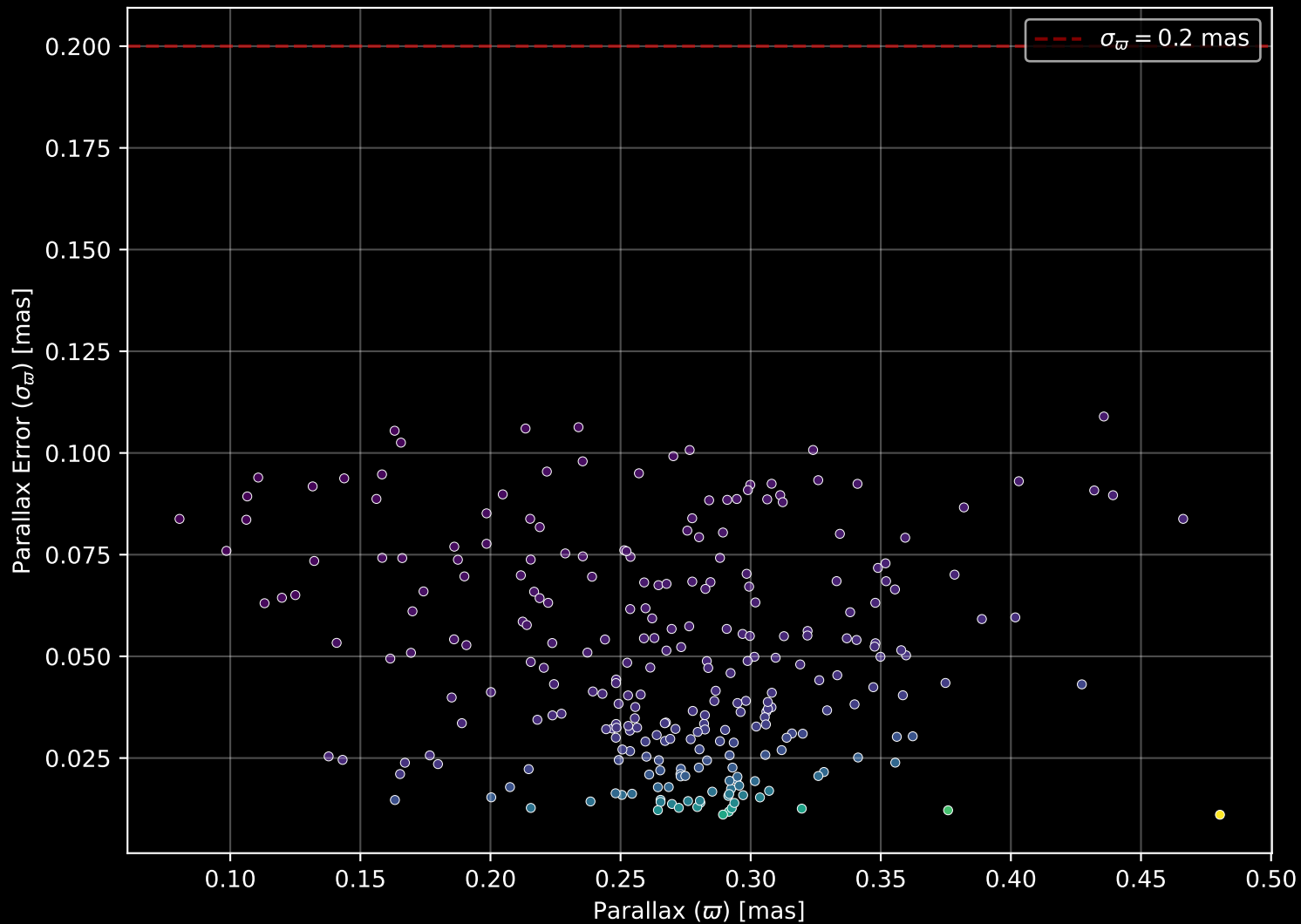
Gaia Cluster: [NGC_436] Parallax Quality (n= 265)
