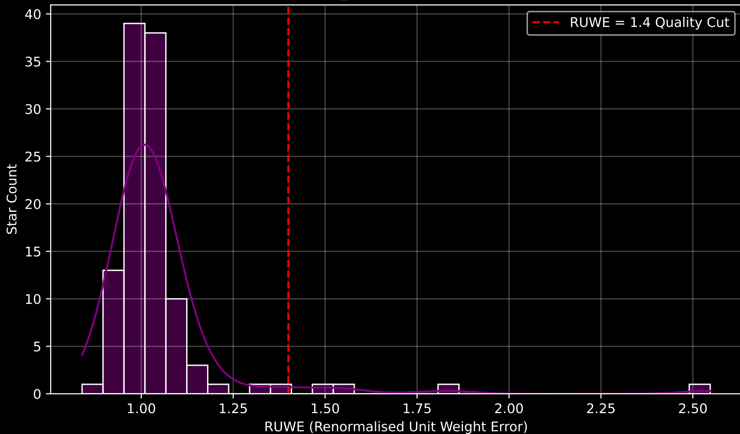
Gaia Cluster: [NGC_4463] RUWE Distribution (n= 111)
