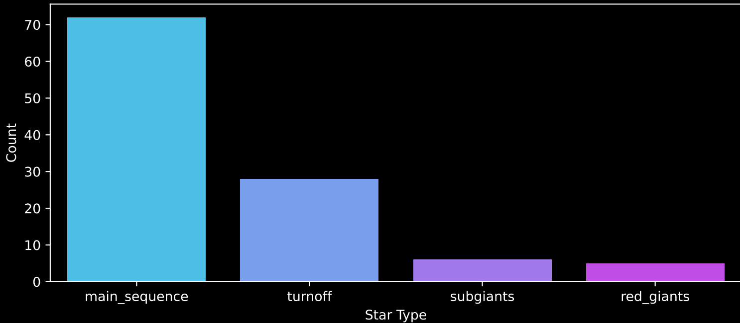
Gaia Cluster: [NGC_4463] Count plot of Star Type
