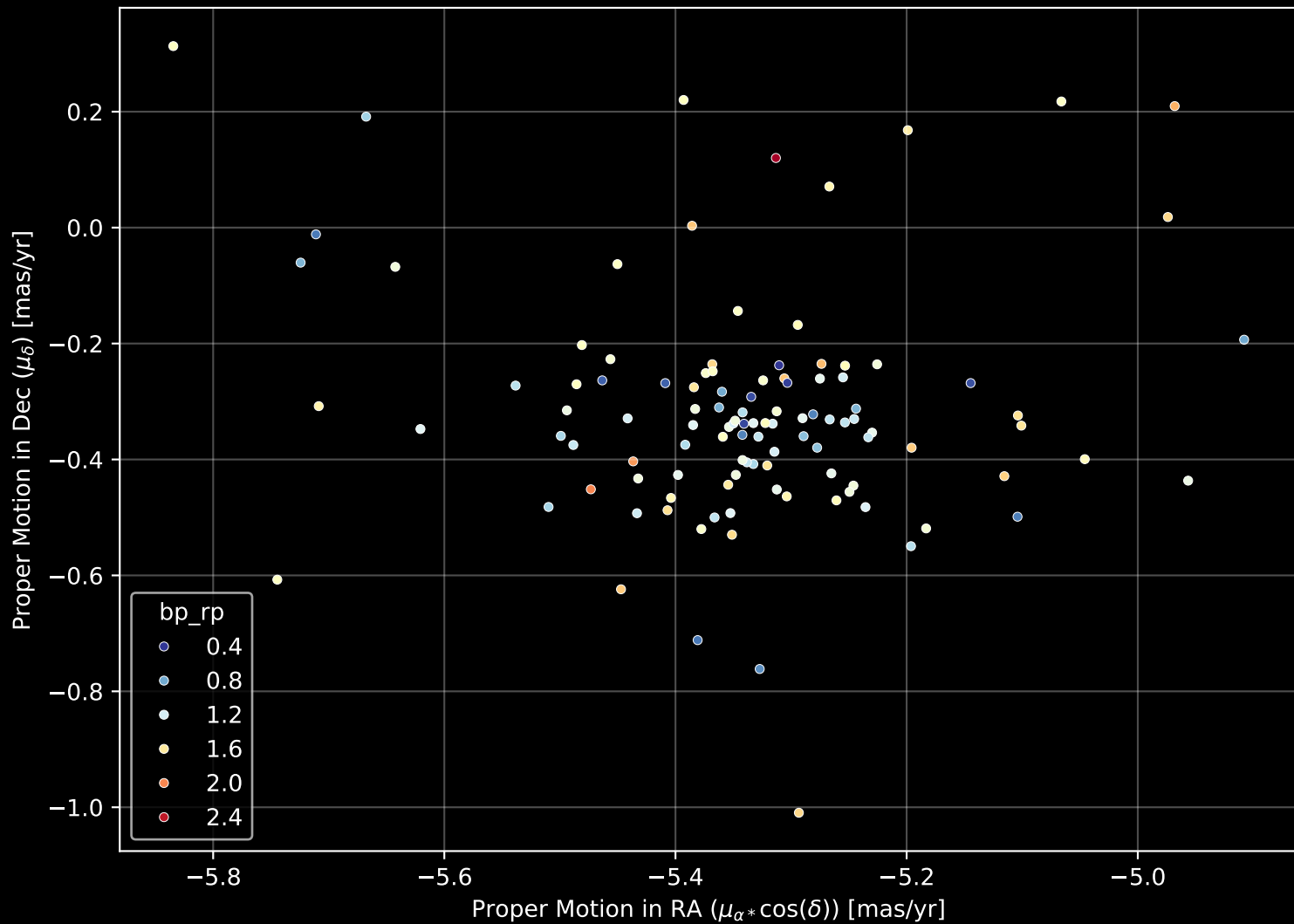
Gaia Cluster: [NGC_4463] Proper Motion Diagram (n= 111)
