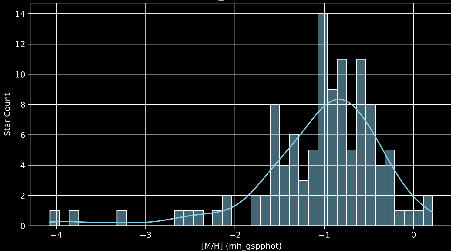
Gaia Cluster: [NGC_4463 [M/H] (mh_gspphot) (n= 111)
