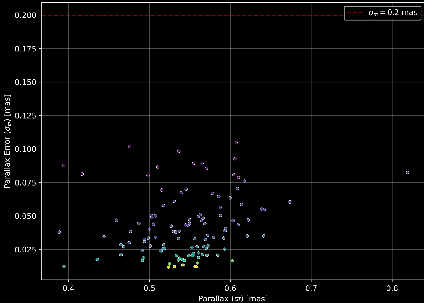
Gaia Cluster: [NGC_4463] Parallax Quality (n= 111)
