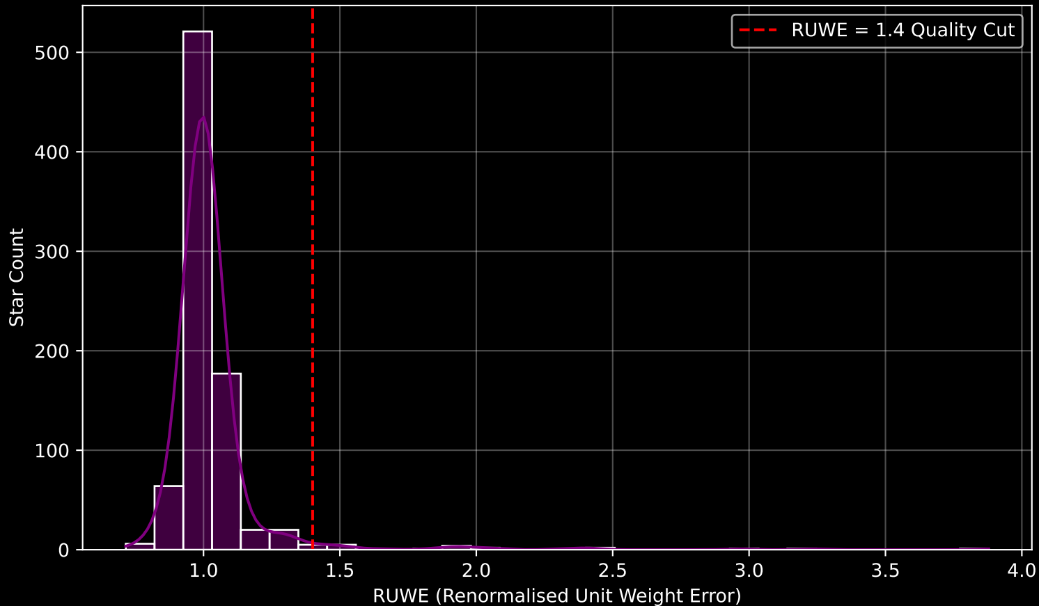
Gaia Cluster: [NGC_4755] RUWE Distribution (n= 832)
