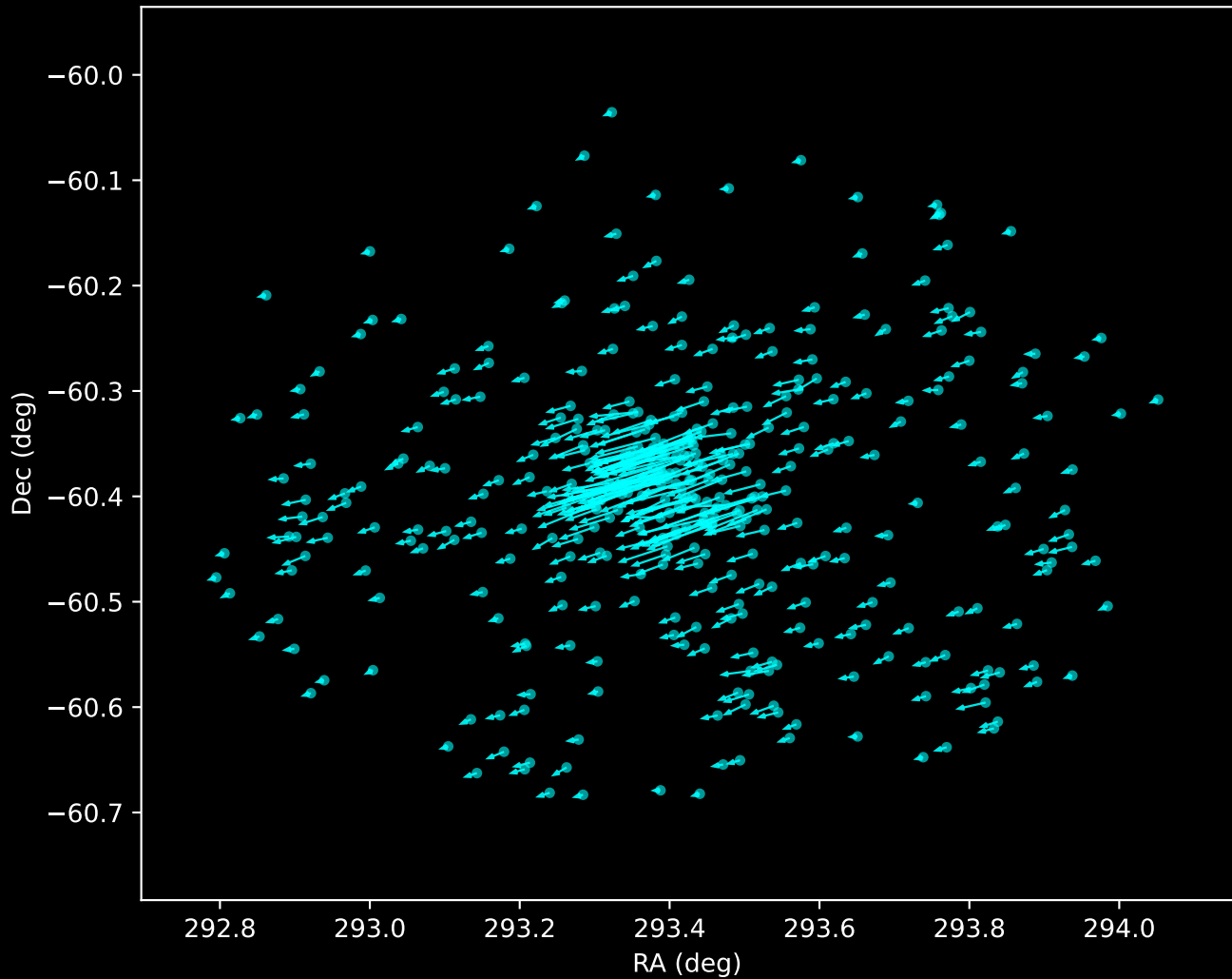
Gaia DR3 Noise Stream Proper Motion Vectors (n=389)
