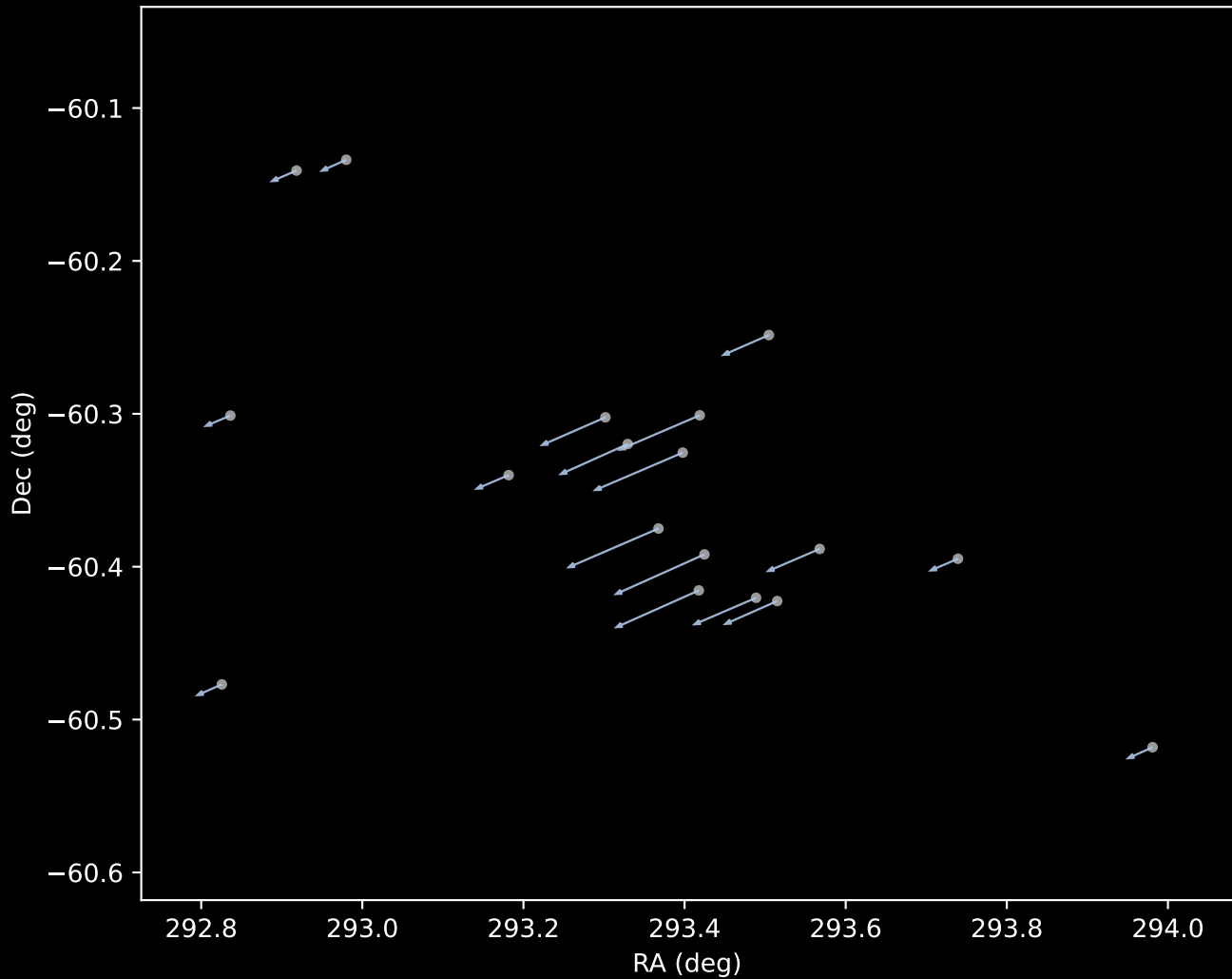
Gaia DR3 Cluster 41 Proper Motion Vectors (n=18)
