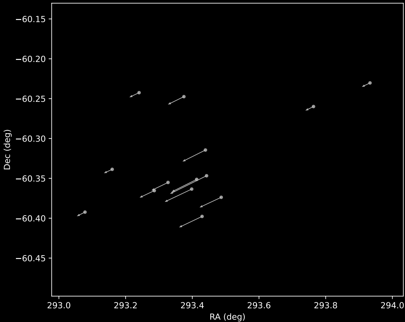
Gaia DR3 Cluster 35 Proper Motion Vectors (n=14)
