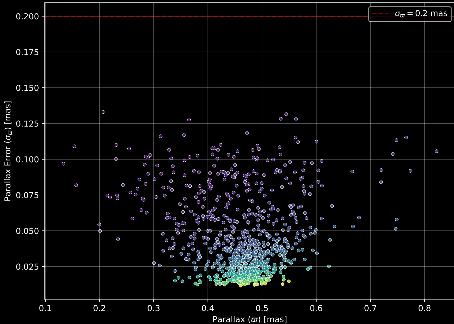
Gaia Cluster: [NGC_4755] Parallax Quality (n= 834)
