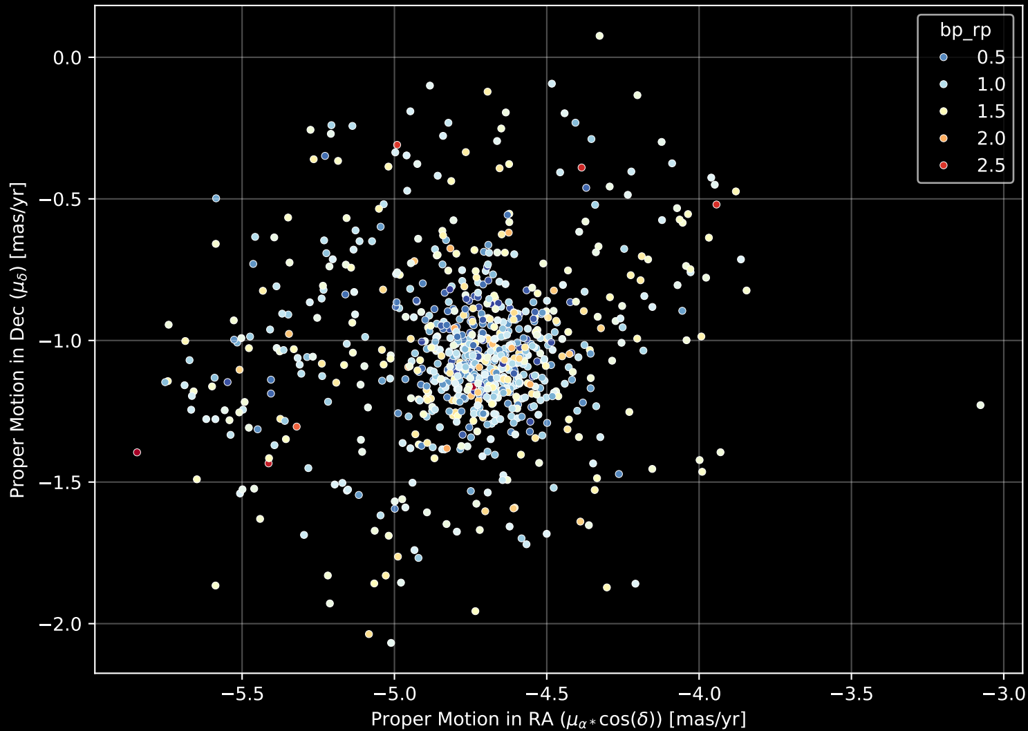
Gaia Cluster: [NGC_4755] Proper Motion Diagram (n= 834)
