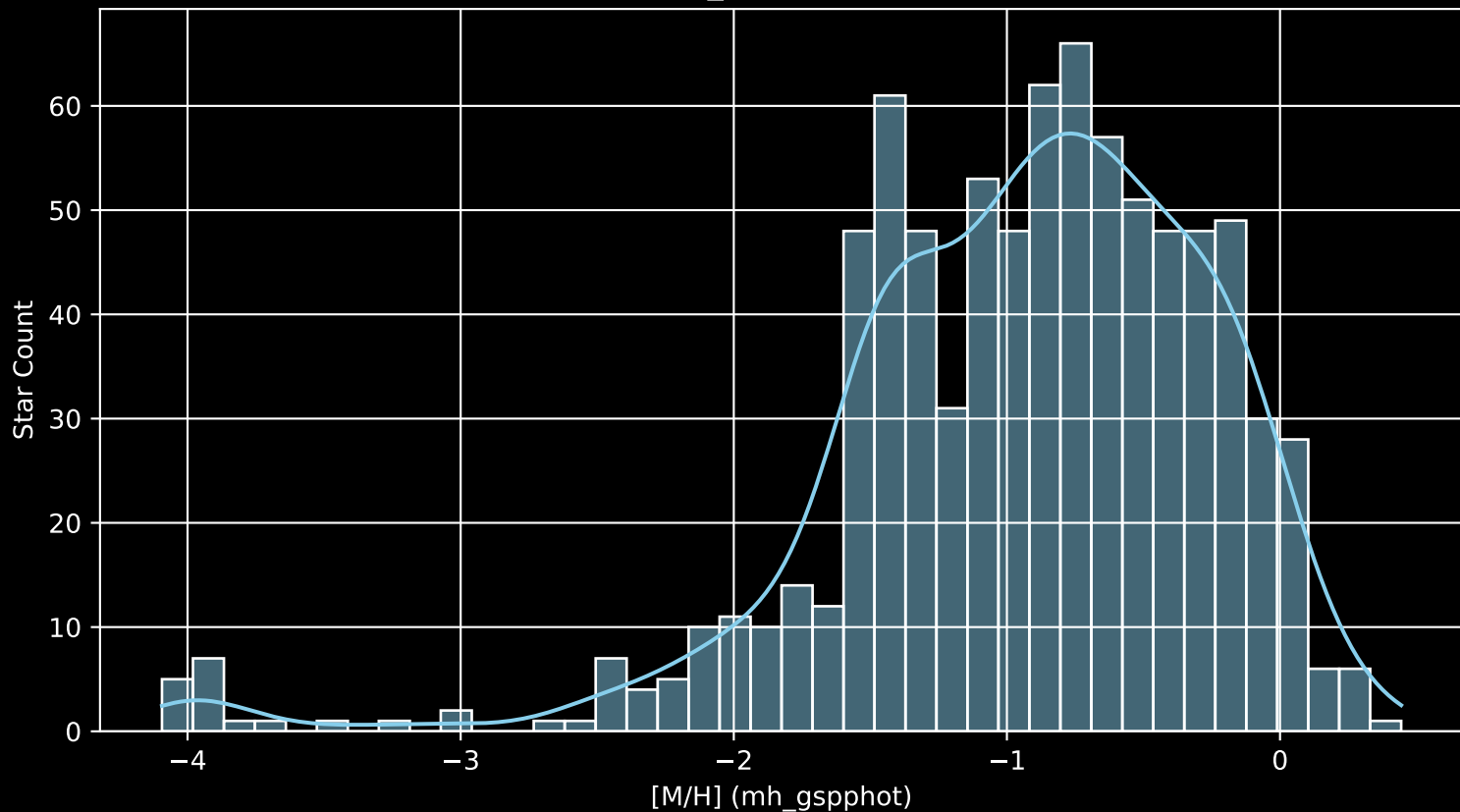
Gaia Cluster: [NGC_4755 [M/H] (mh_gspphot) (n= 834)
