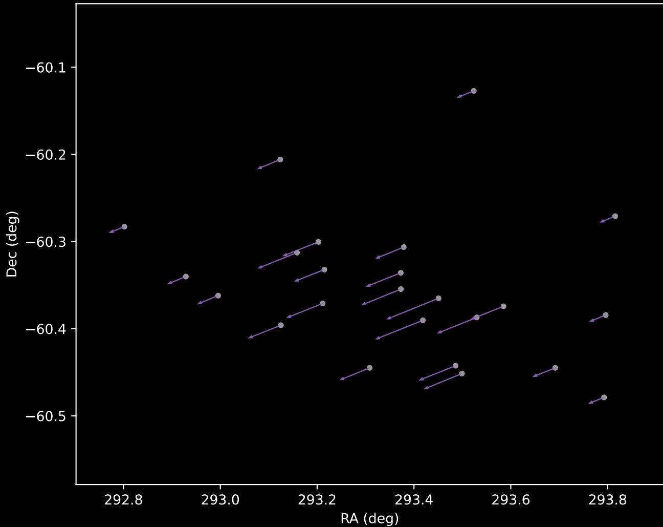
Gaia DR3 Cluster 48 Proper Motion Vectors (n=24)
