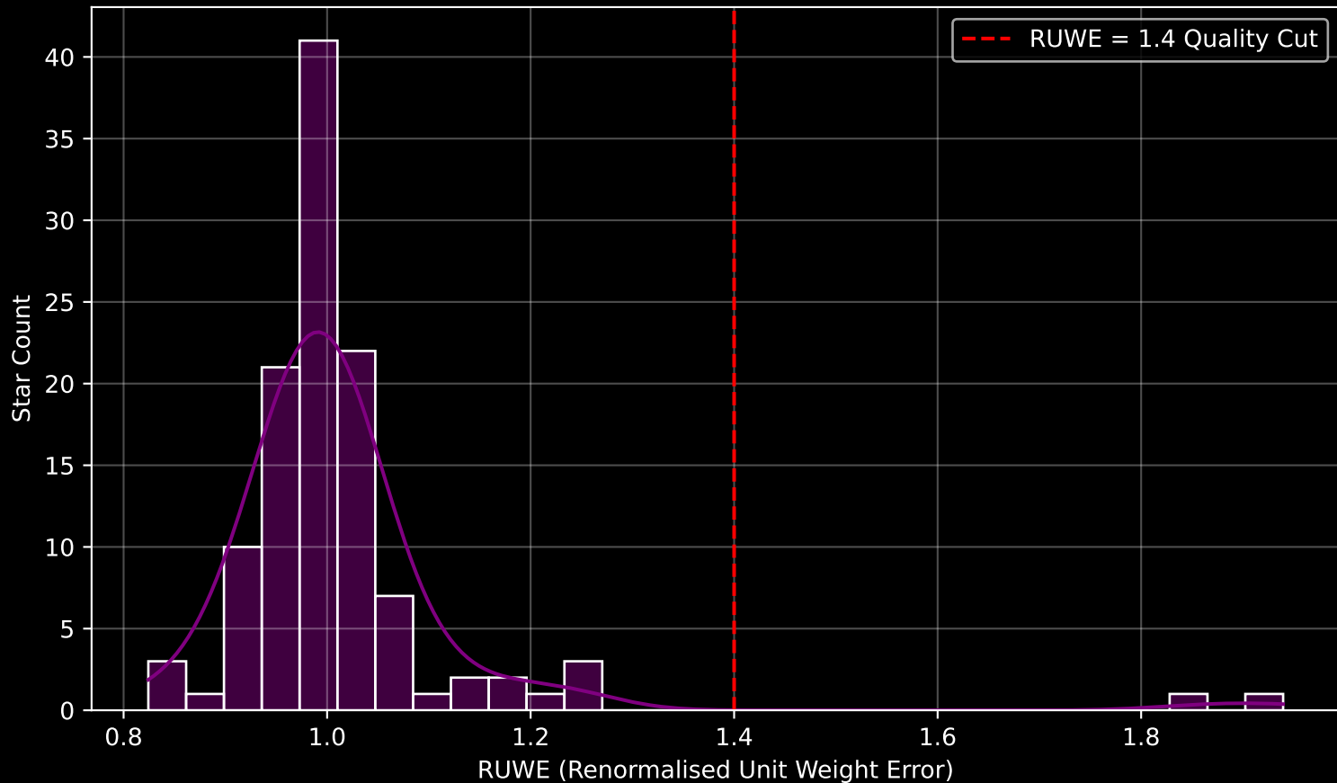
Gaia Cluster: [NGC_5281] RUWE Distribution (n= 116)
