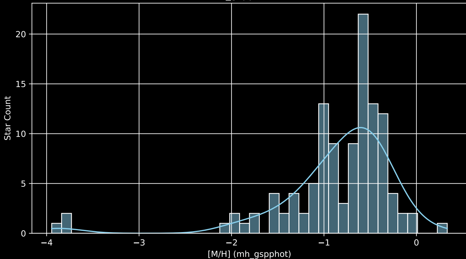
Gaia Cluster: [NGC_5281 [M/H] (mh_gspphot) (n= 116)
