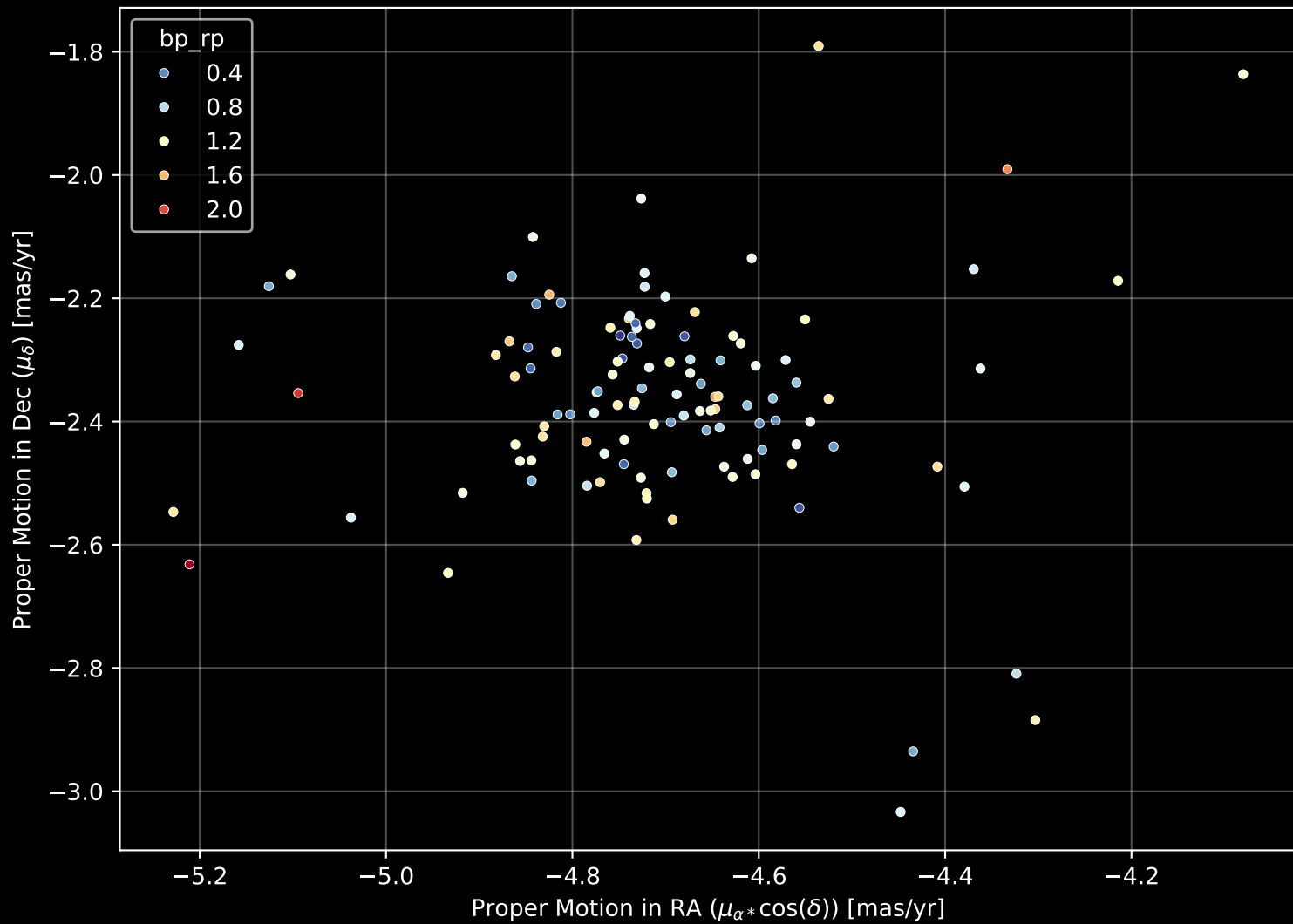
Gaia Cluster: [NGC_5281] Proper Motion Diagram (n= 116)
