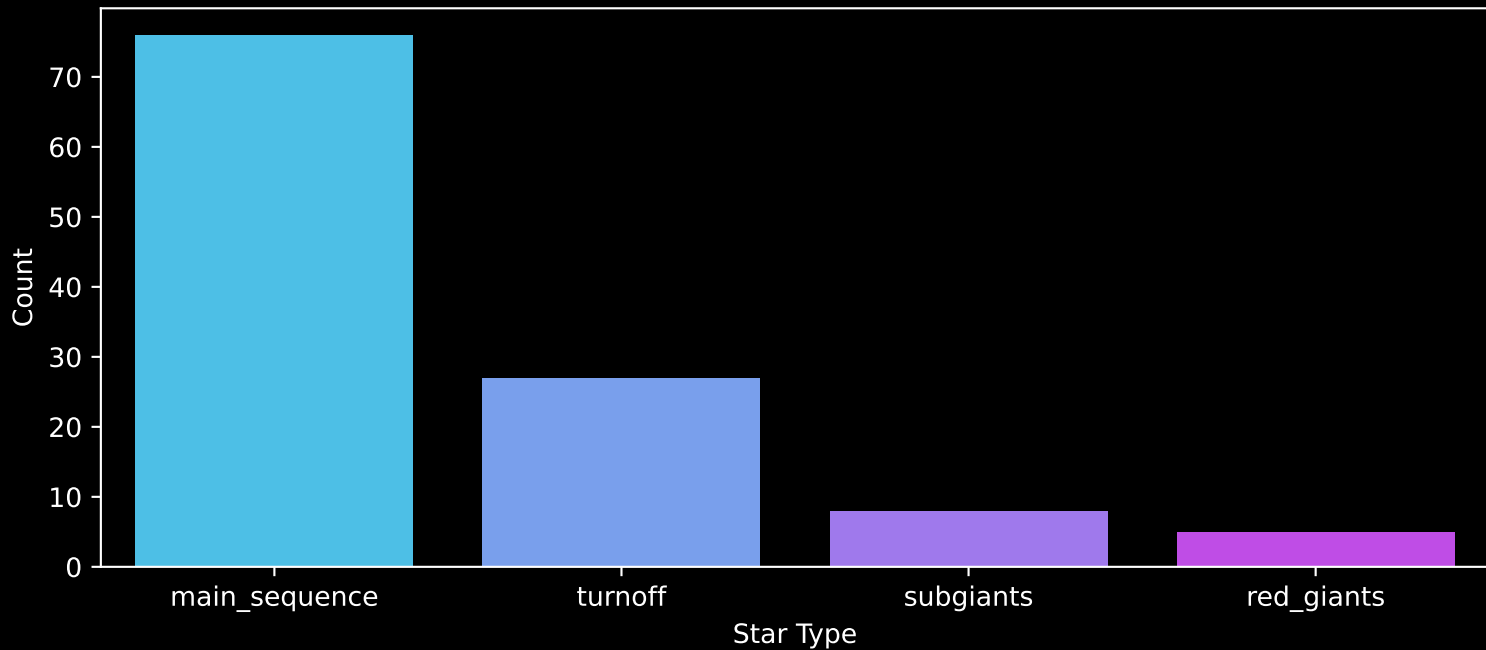
Gaia Cluster: [NGC_5281] Count plot of Star Type
