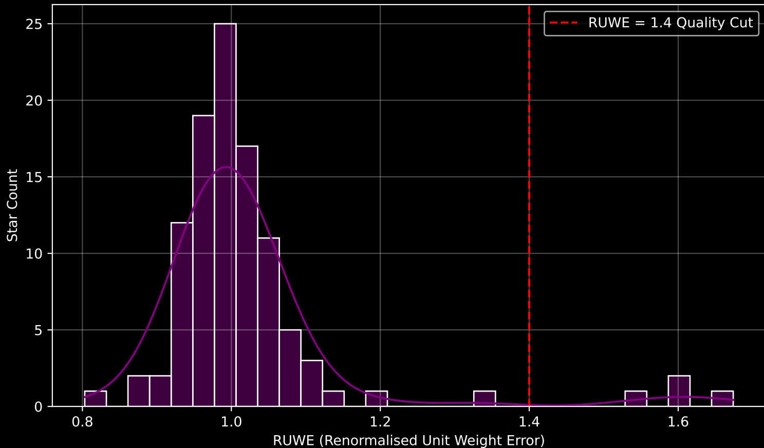
Gaia Cluster: [NGC_5288] RUWE Distribution (n= 104)
