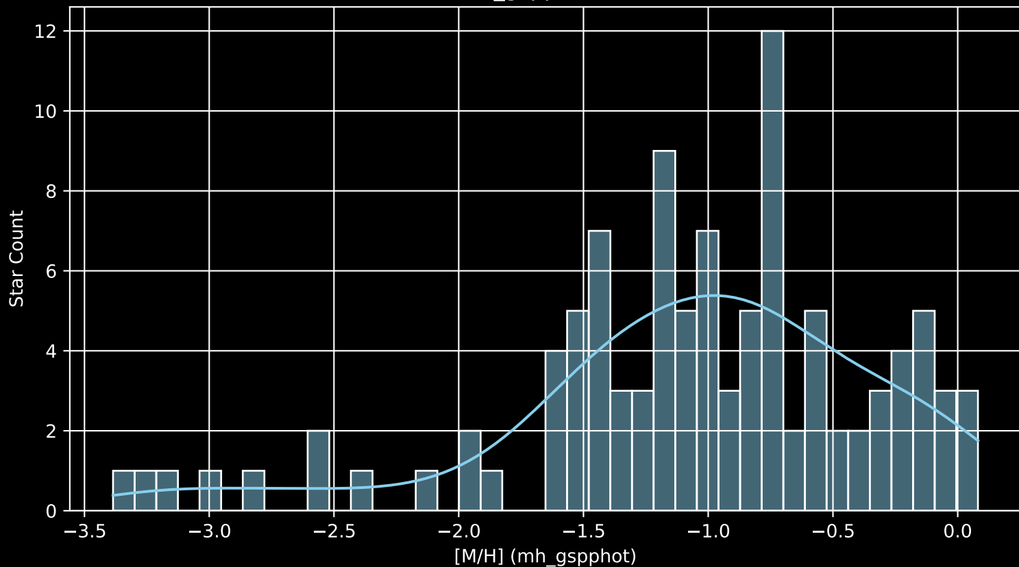
Gaia Cluster: [NGC_5288 [M/H] (mh_gspphot) (n= 104)
