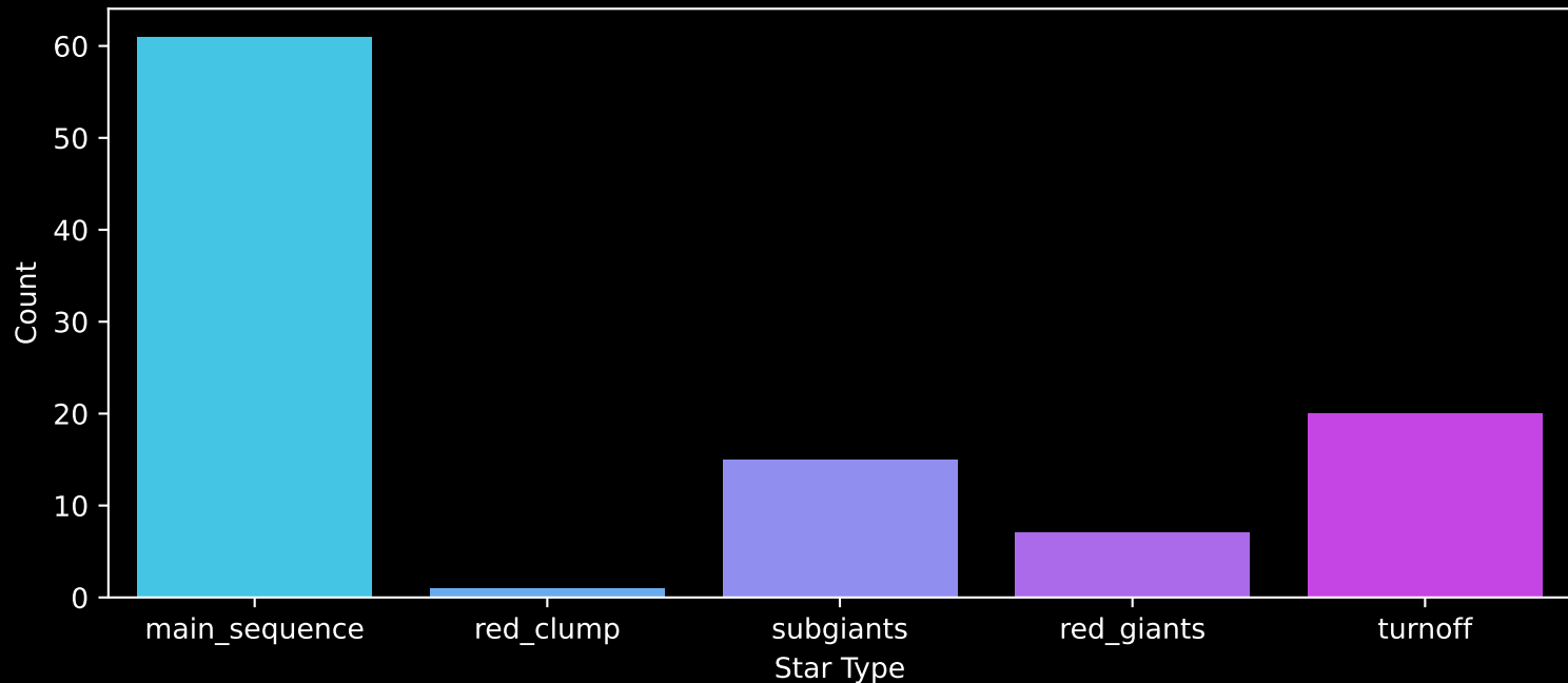
Gaia Cluster: [NGC_5288] Count plot of Star Type
