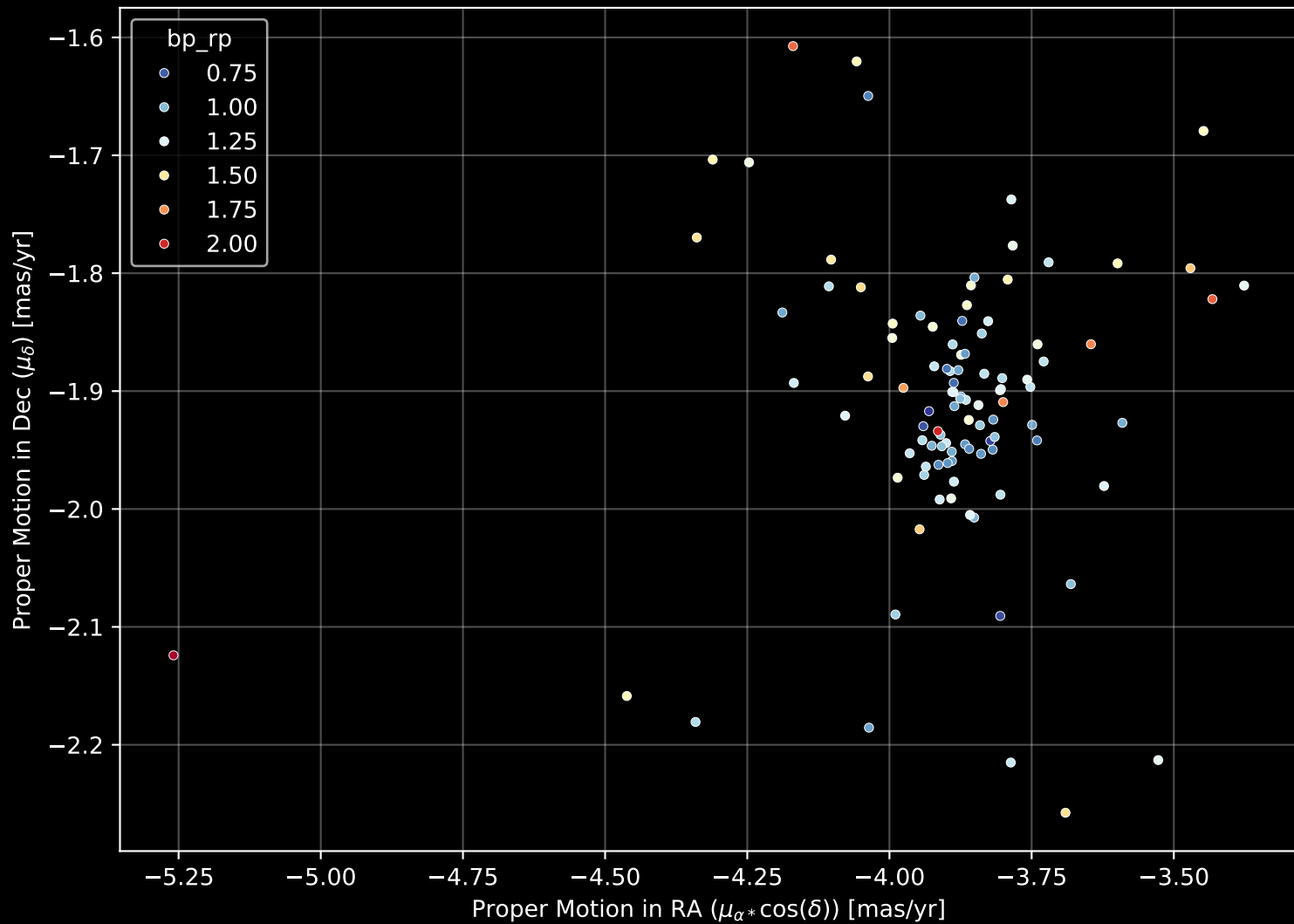
Gaia Cluster: [NGC_5288] Proper Motion Diagram (n= 104)
