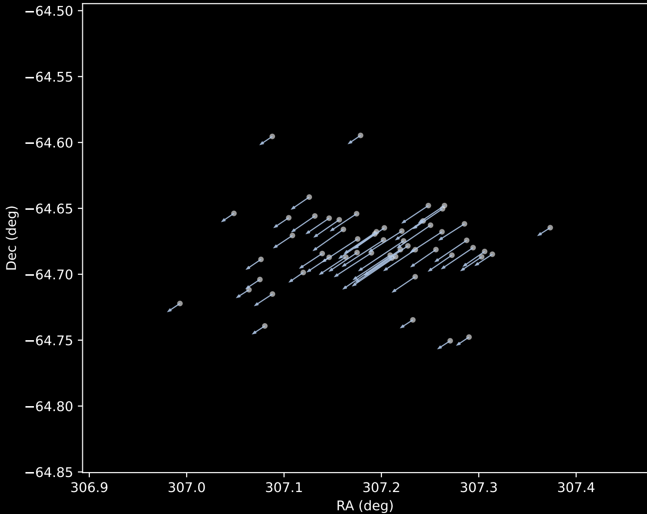
Gaia DR3 Cluster 1 Proper Motion Vectors (n=55)
