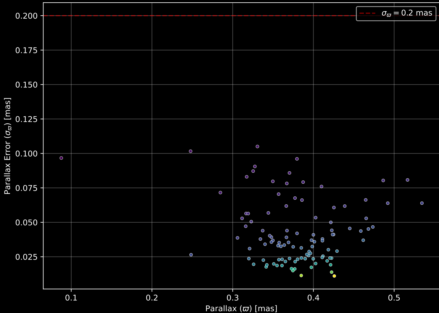
Gaia Cluster: [NGC_5288] Parallax Quality (n= 104)
