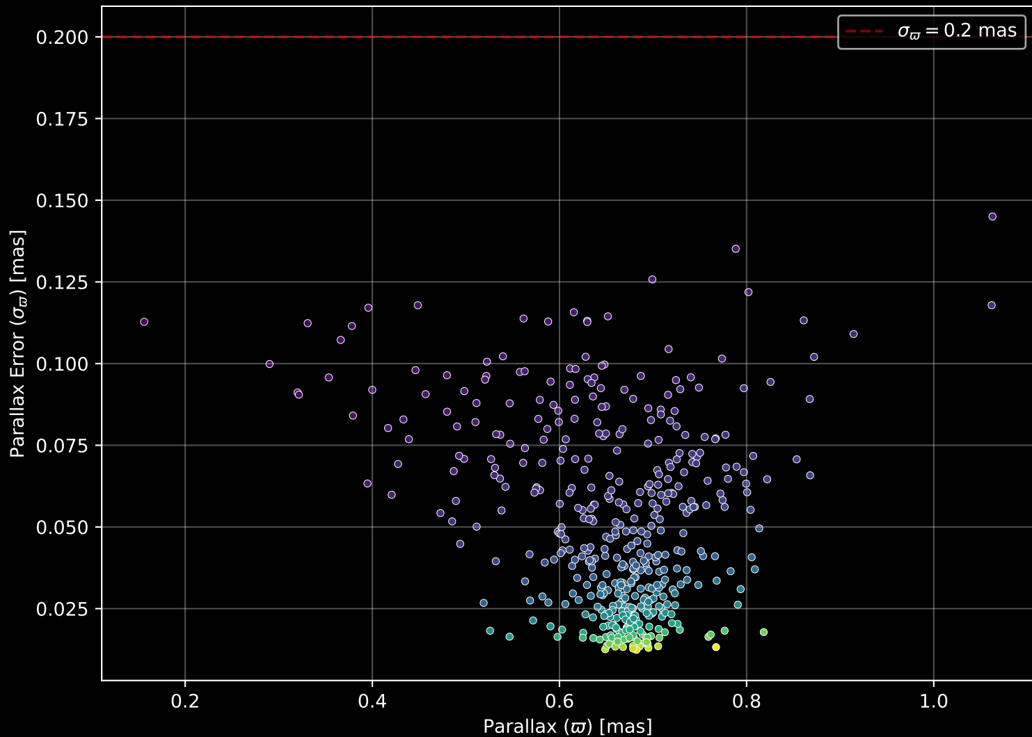
Gaia Cluster: [NGC_5316] Parallax Quality (n= 457)
