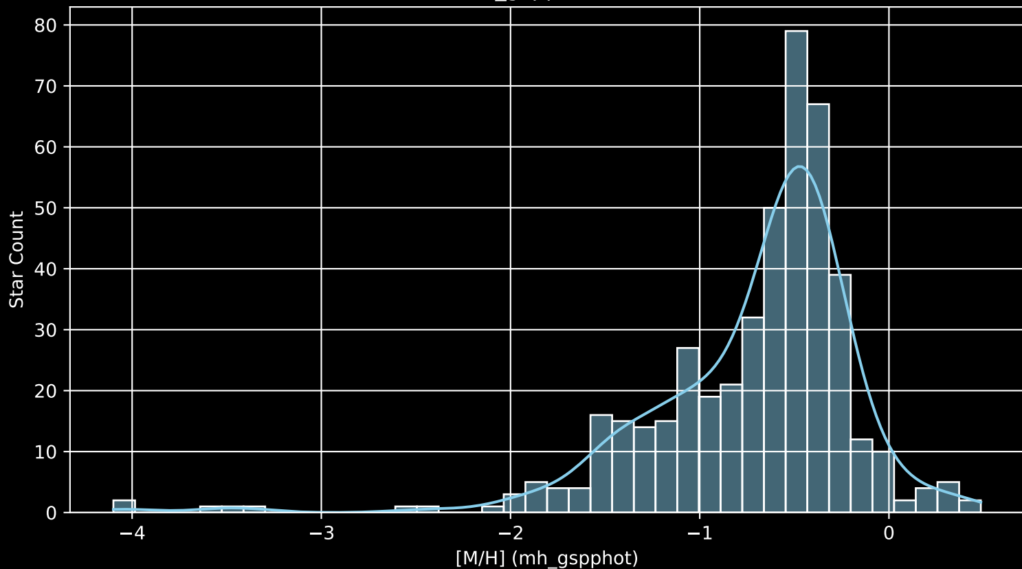
Gaia Cluster: [NGC_5316 [M/H] (mh_gspphot) (n= 453)
