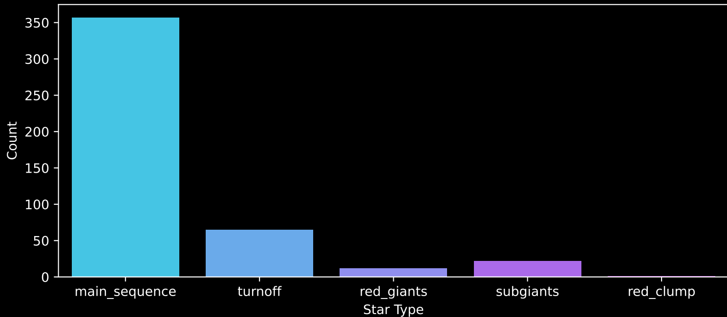
Gaia Cluster: [NGC_5316] Count plot of Star Type
