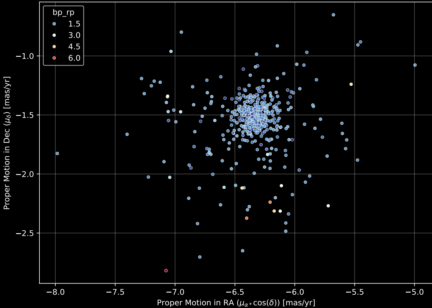
Gaia Cluster: [NGC_5316] Proper Motion Diagram (n= 457)
