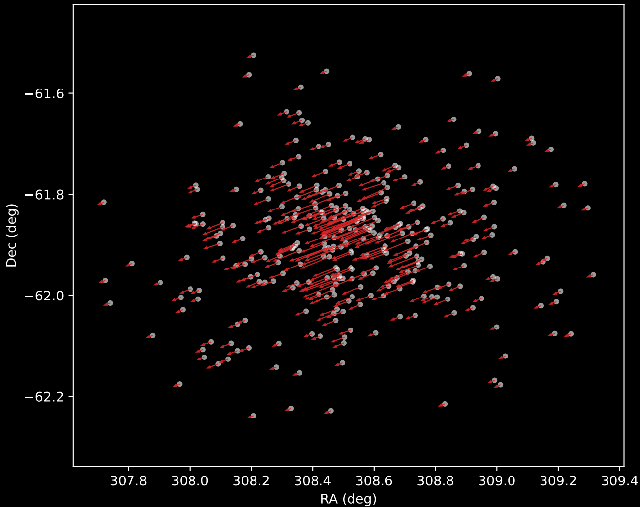
Gaia DR3 Cluster 6 Proper Motion Vectors (n=318)
