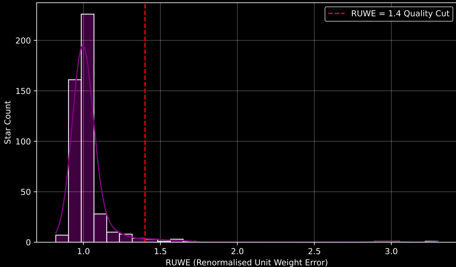
Gaia Cluster: [NGC_5316] RUWE Distribution (n= 455)
