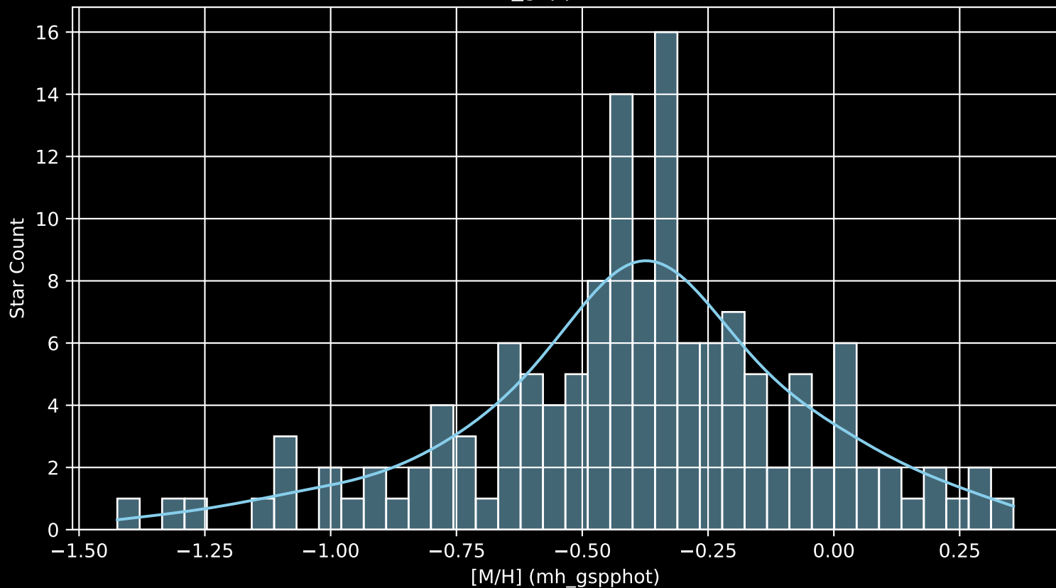
Gaia Cluster: [NGC_5460 [M/H] (mh_gspphot) (n= 139)
