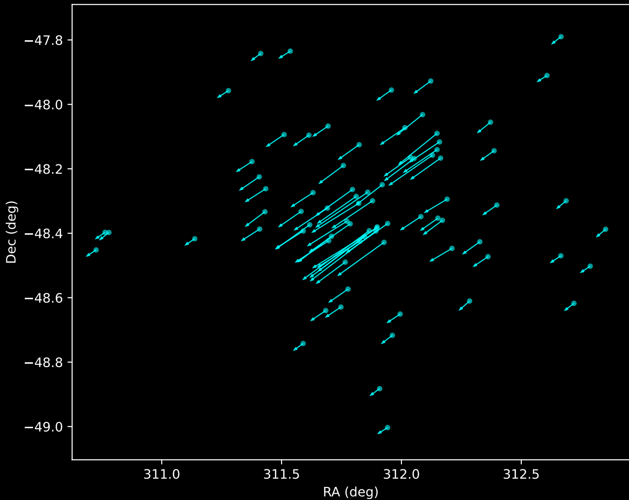
Gaia DR3 Noise Stream Proper Motion Vectors (n=78)
