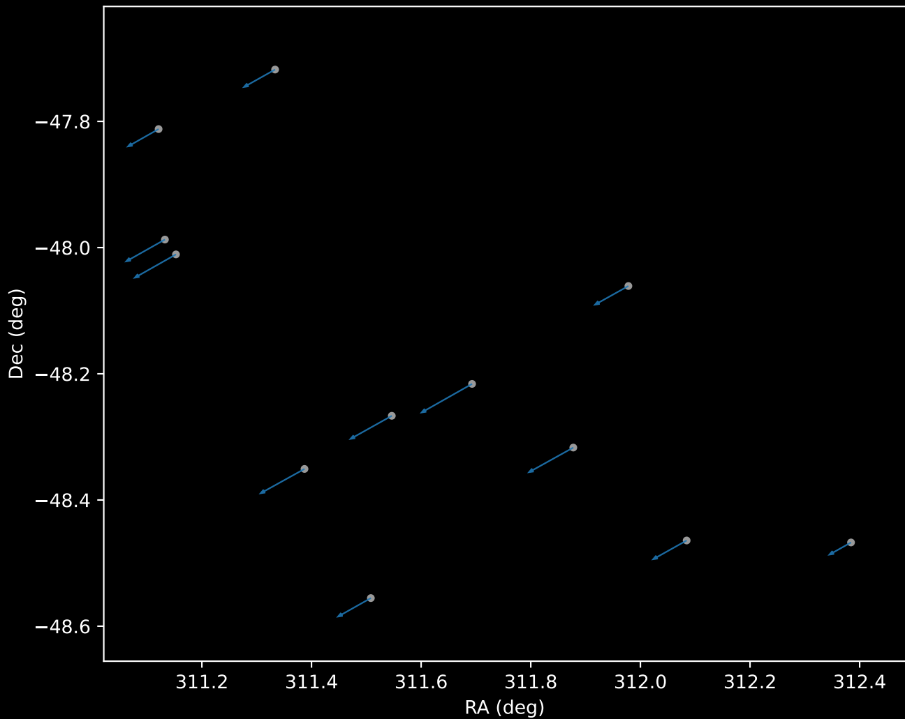
Gaia DR3 Cluster 0 Proper Motion Vectors (n=12)
