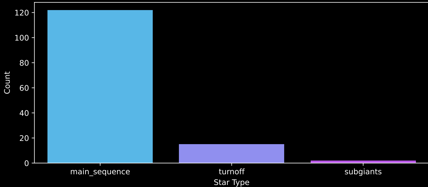
Gaia Cluster: [NGC_5460] Count plot of Star Type
