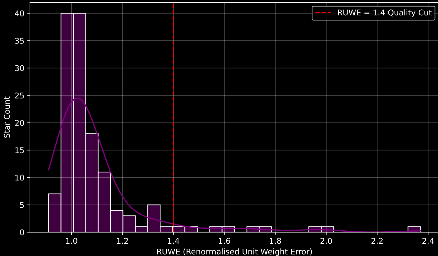
Gaia Cluster: [NGC_5460] RUWE Distribution (n= 139)
