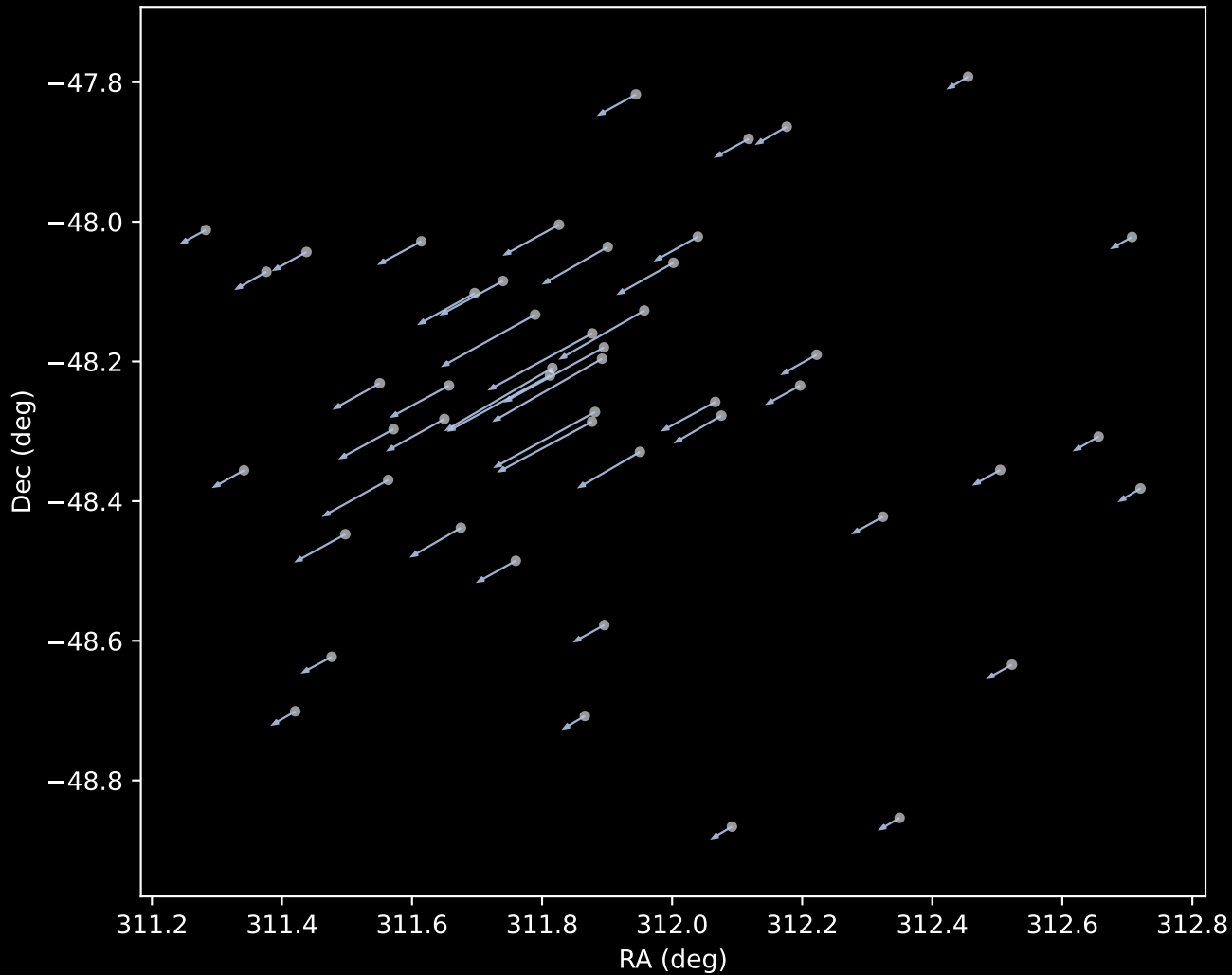
Gaia DR3 Cluster 1 Proper Motion Vectors (n=49)
