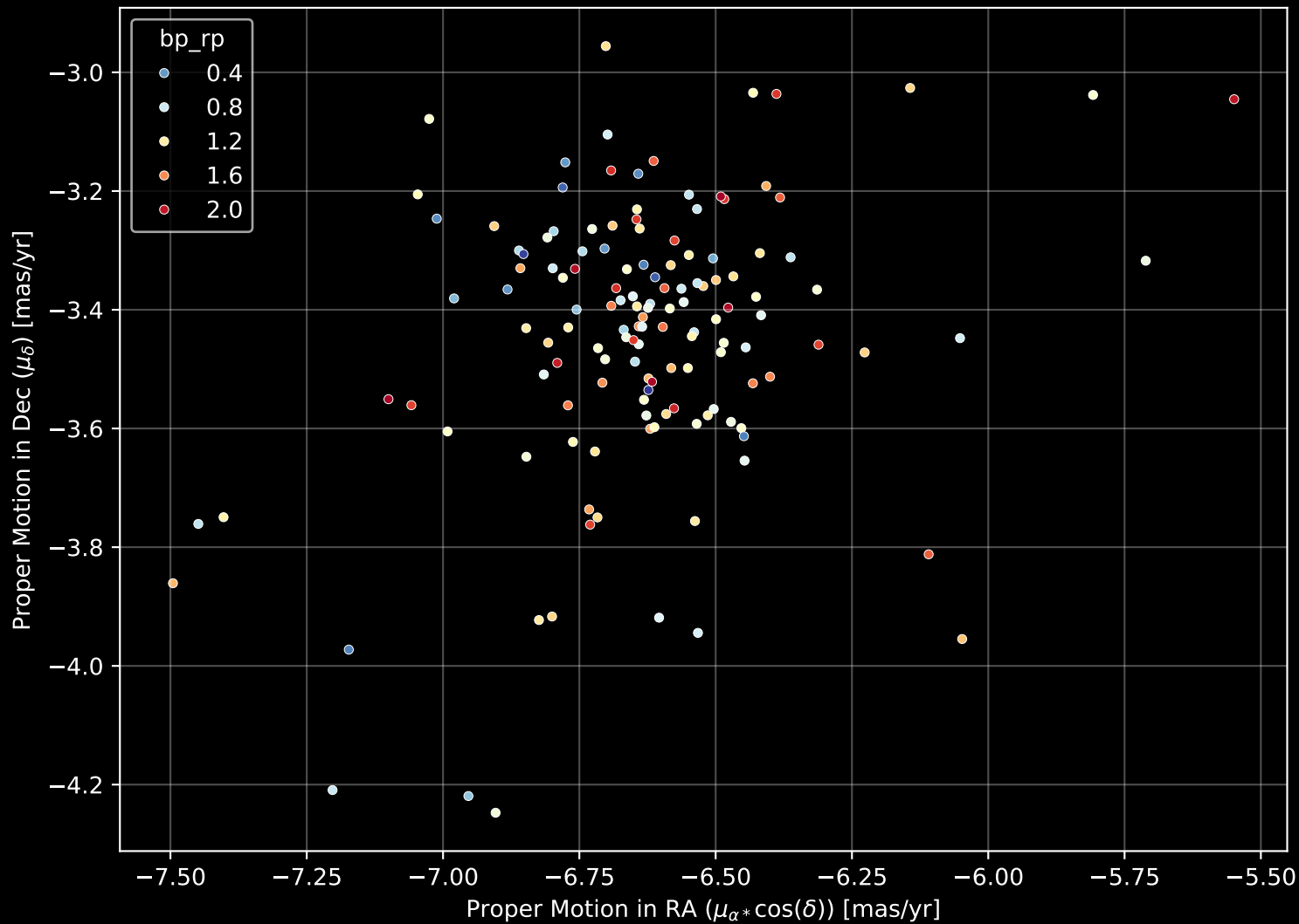
Gaia Cluster: [NGC_5460] Proper Motion Diagram (n= 139)
