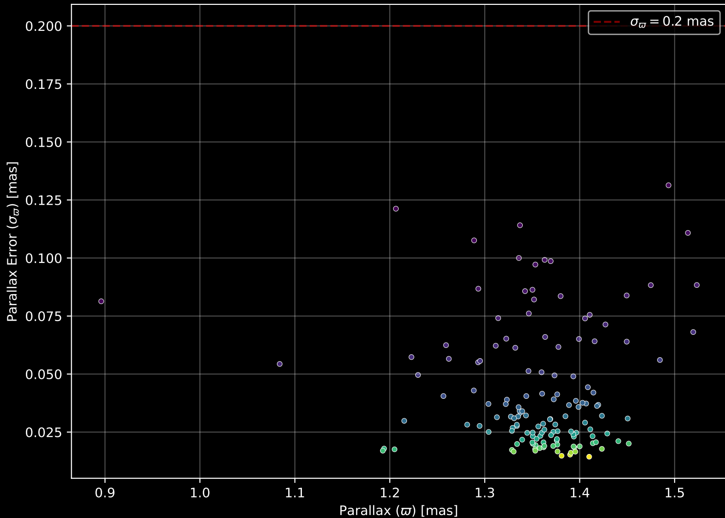
Gaia Cluster: [NGC_5460] Parallax Quality (n= 139)
