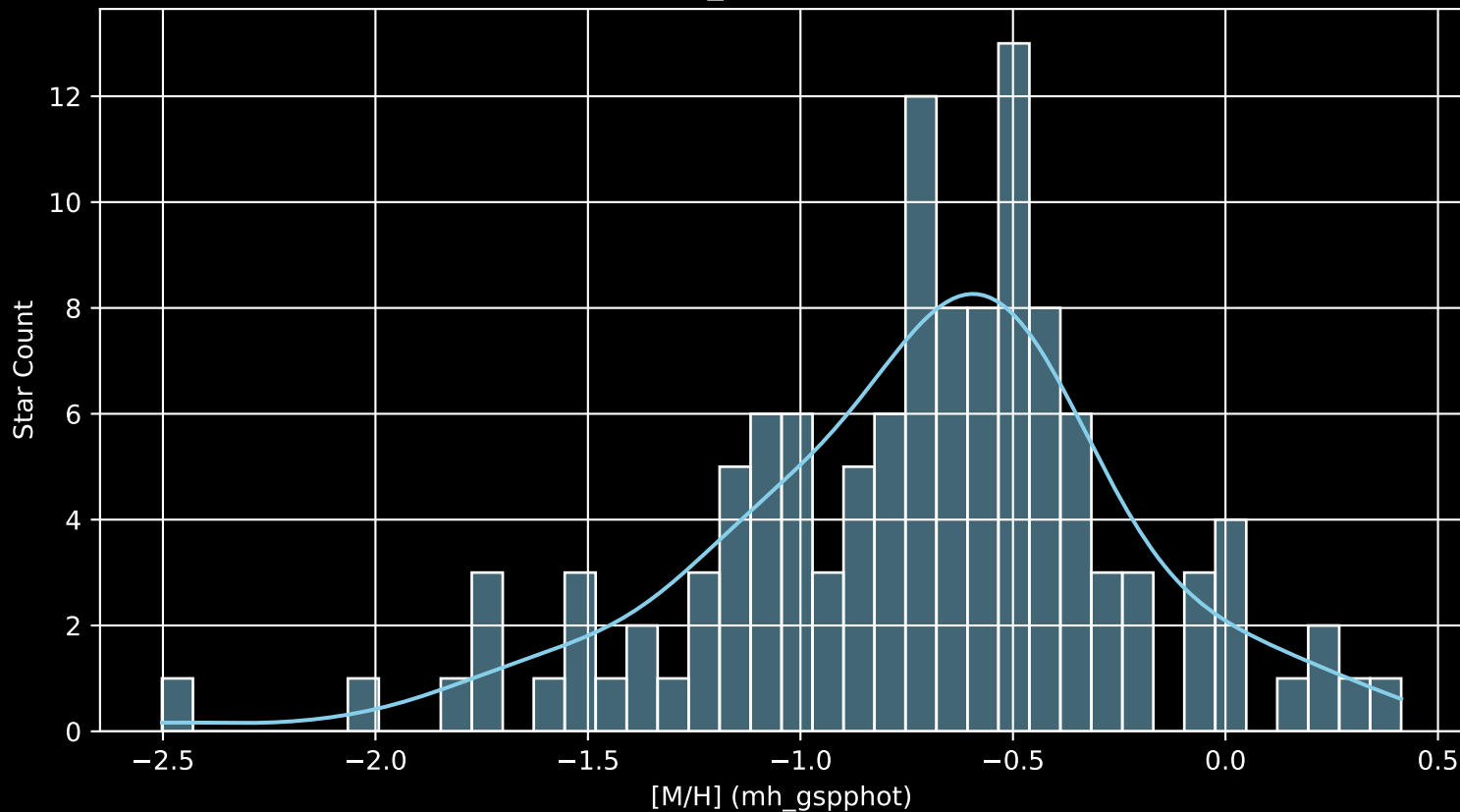
Gaia Cluster: [NGC_5593 [M/H] (mh_gspphot) (n= 121)
