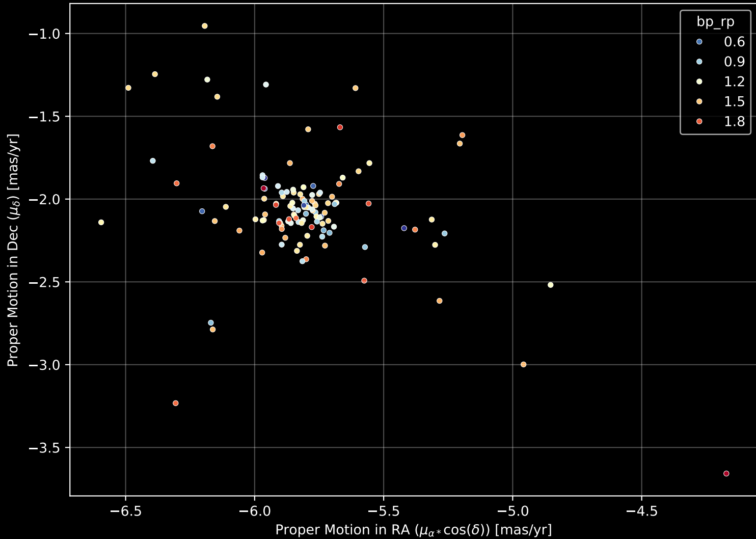
Gaia Cluster: [NGC_5593] Proper Motion Diagram (n= 121)
