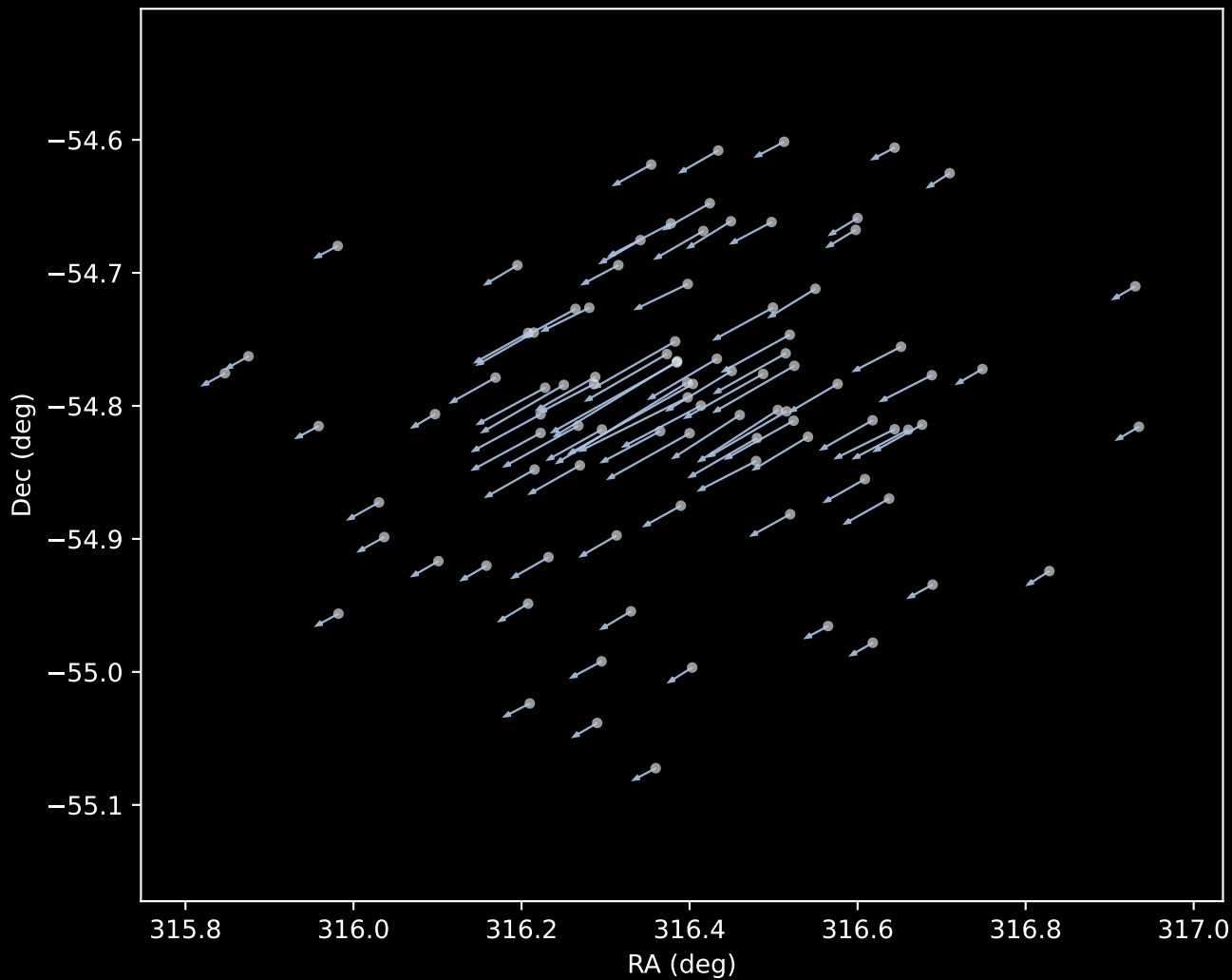
Gaia DR3 Cluster 1 Proper Motion Vectors (n=93)
