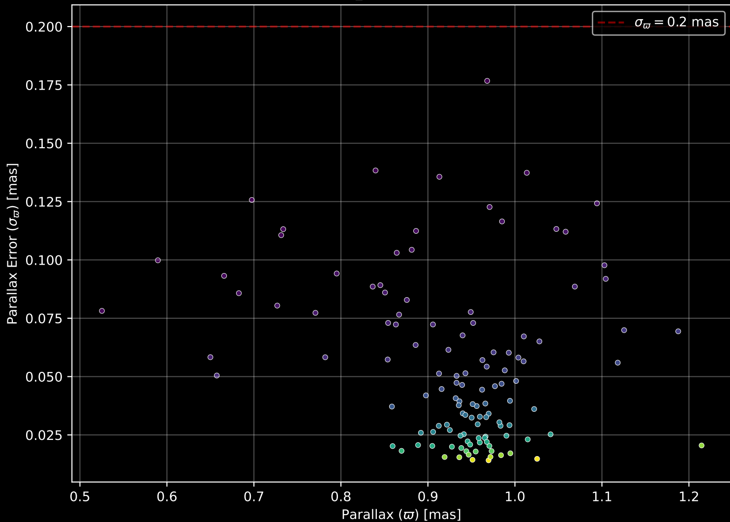
Gaia Cluster: [NGC_5593] Parallax Quality (n= 121)
