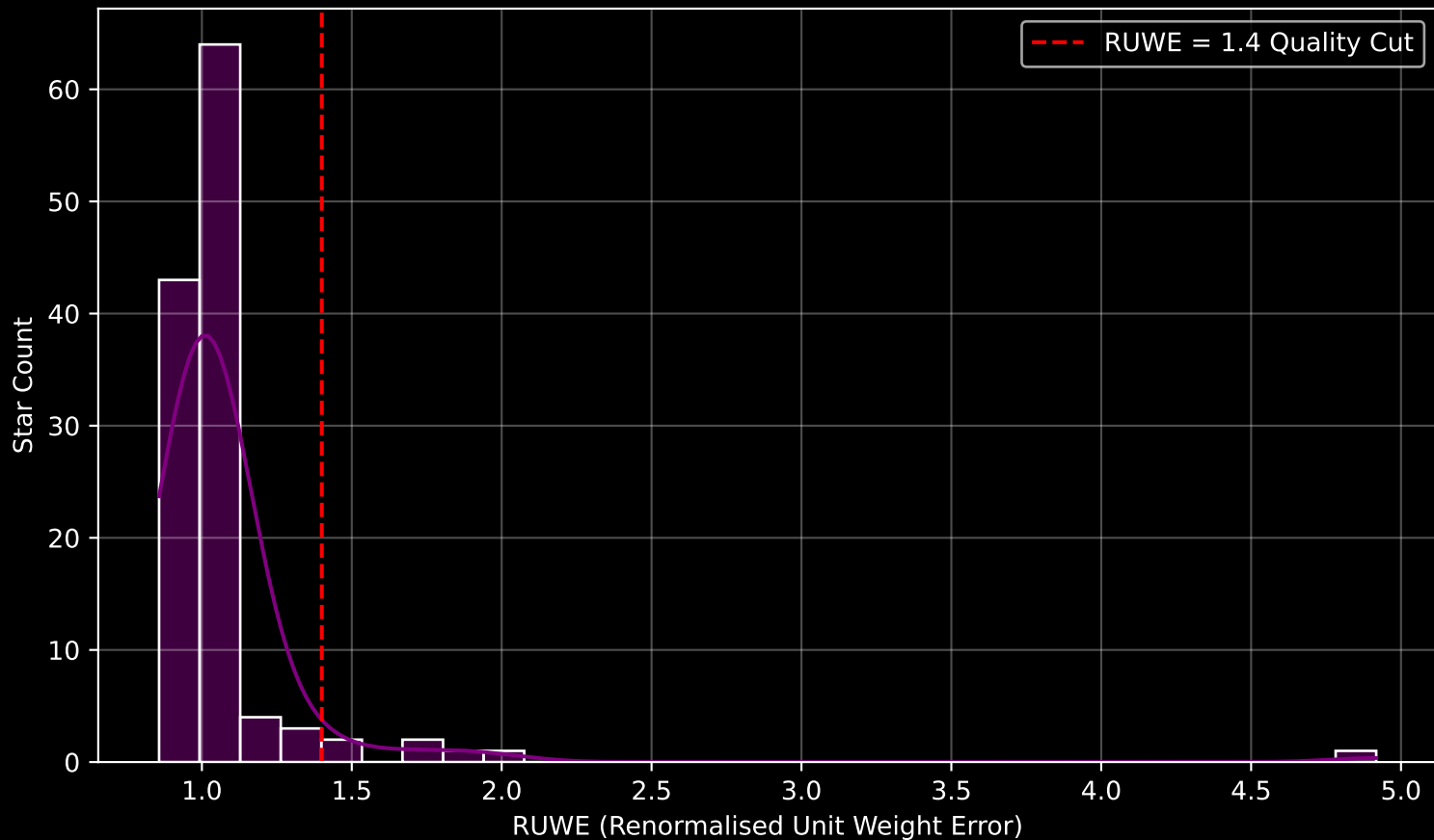
Gaia Cluster: [NGC_5593] RUWE Distribution (n= 121)
