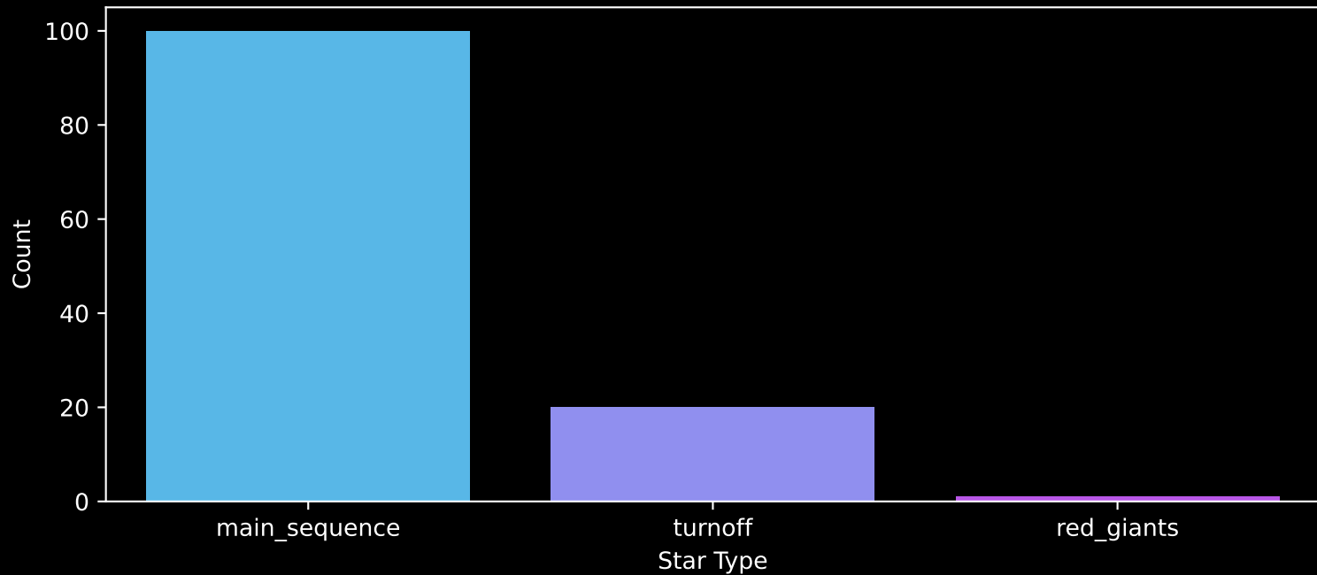
Gaia Cluster: [NGC_5593] Count plot of Star Type
