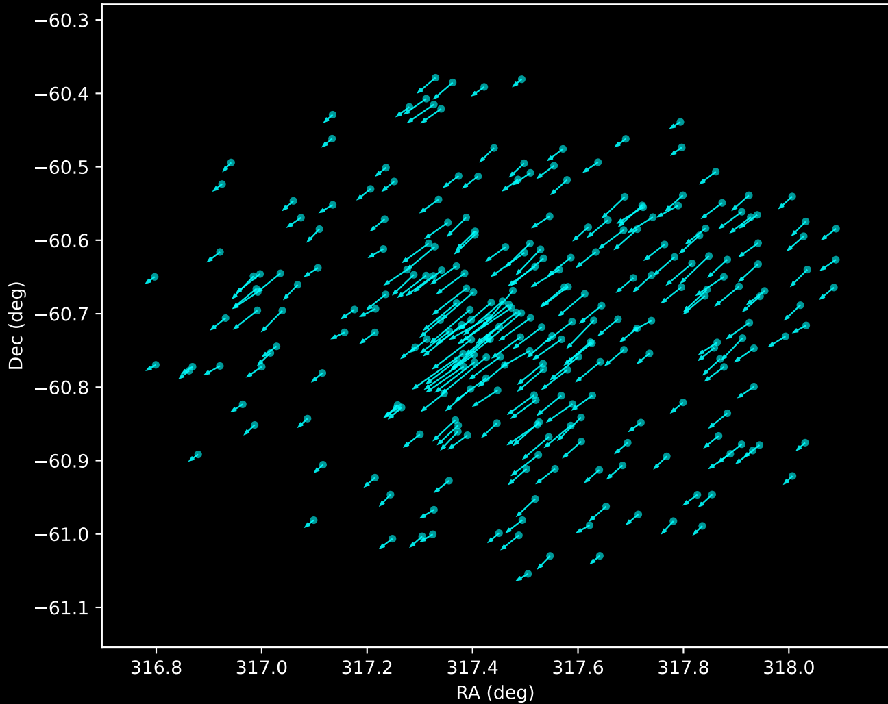
Gaia DR3 Noise Stream Proper Motion Vectors (n=257)
