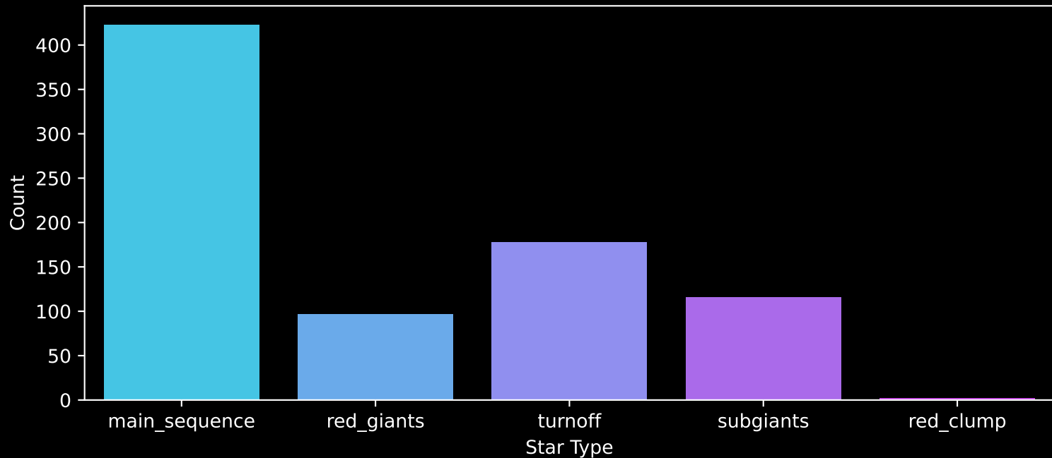
Gaia Cluster: [NGC_5617] Count plot of Star Type
