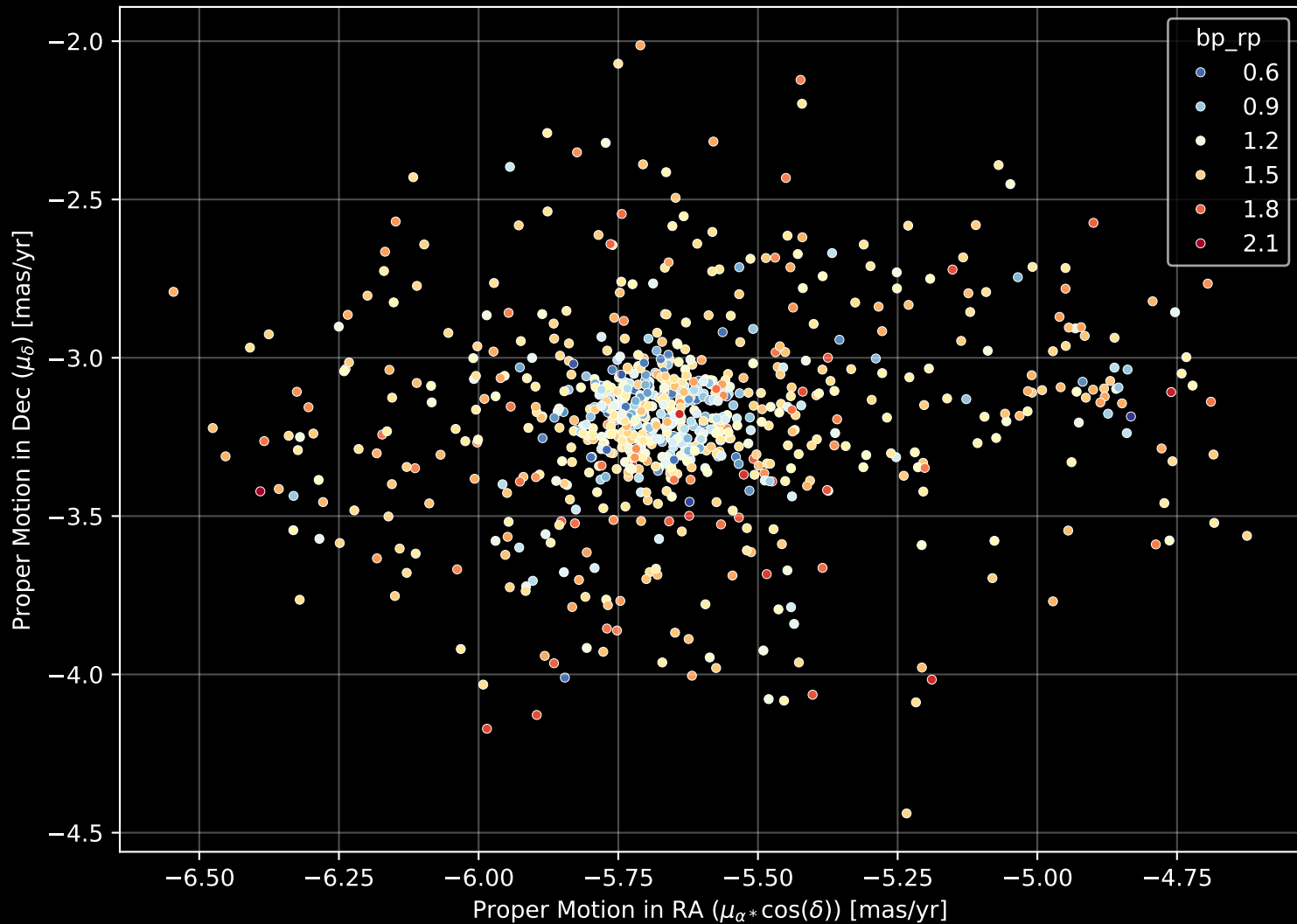
Gaia Cluster: [NGC_5617] Proper Motion Diagram (n= 816)
