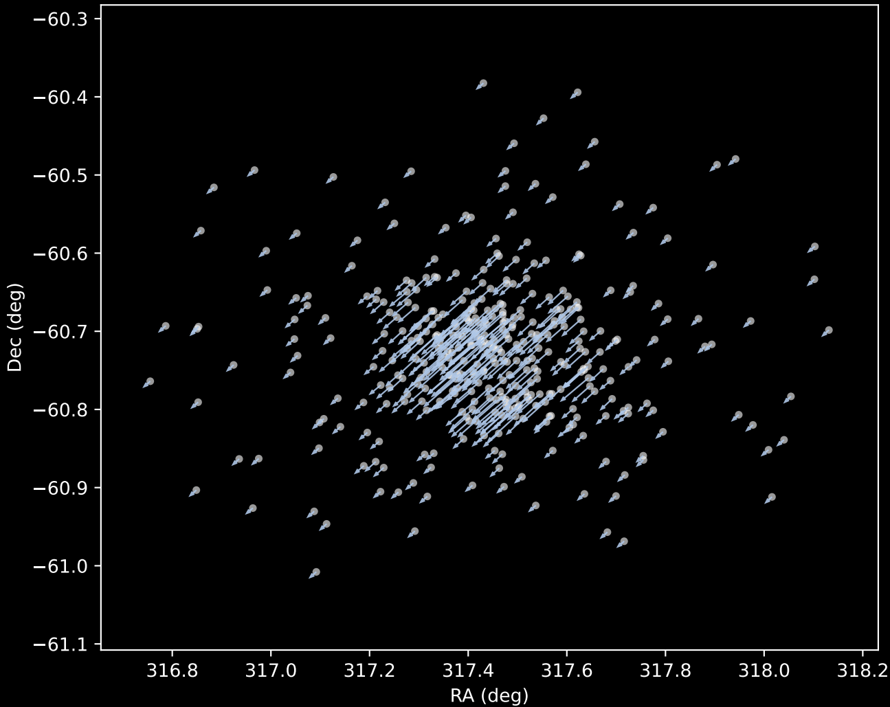
Gaia DR3 Cluster 21 Proper Motion Vectors (n=372)
