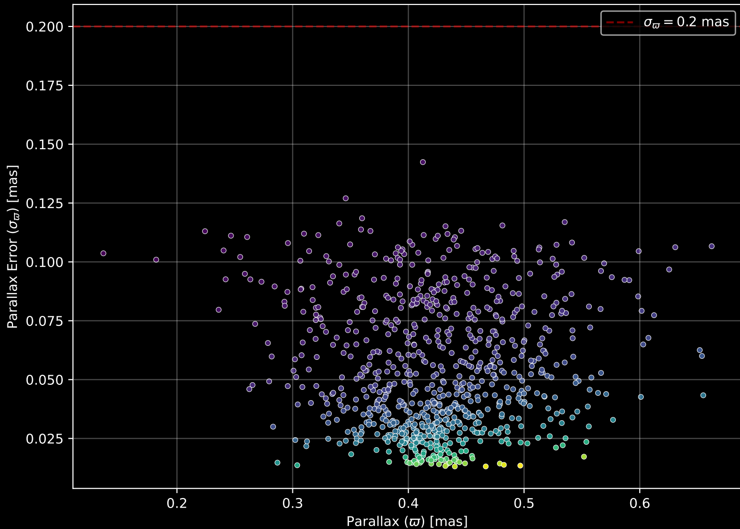
Gaia Cluster: [NGC_5617] Parallax Quality (n= 816)
