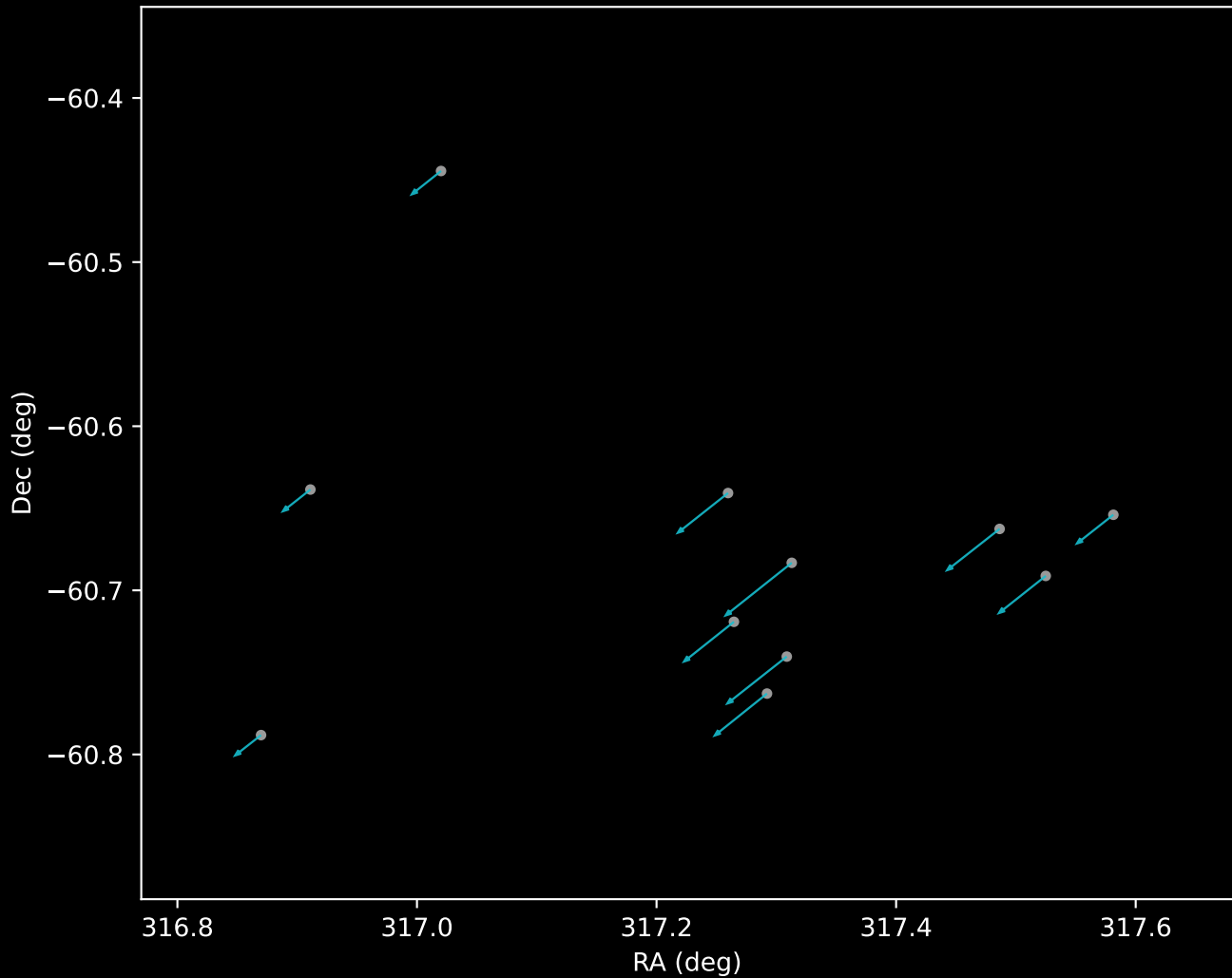
Gaia DR3 Cluster 18 Proper Motion Vectors (n=11)
