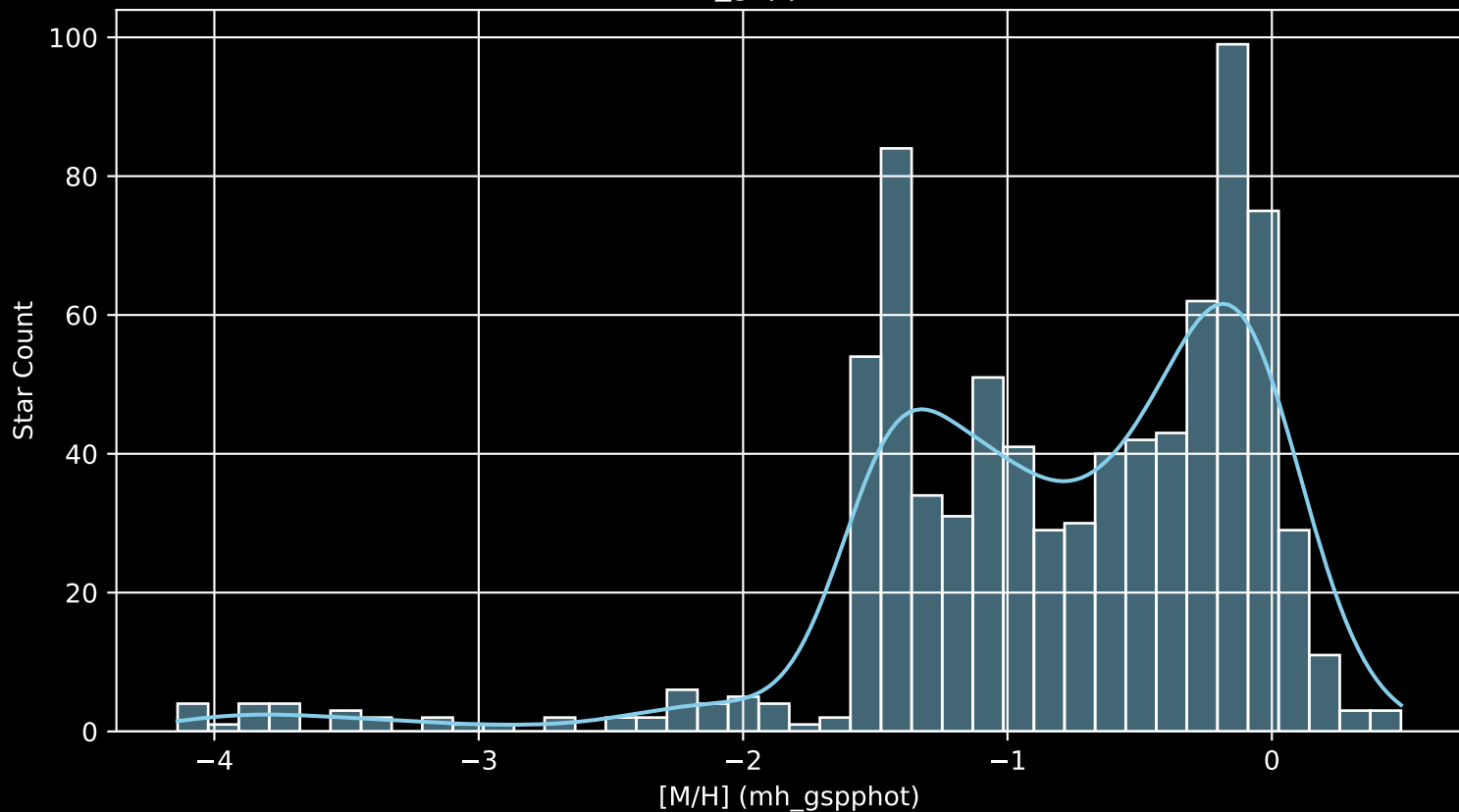
Gaia Cluster: [NGC_5617 [M/H] (mh_gspphot) (n= 811)
