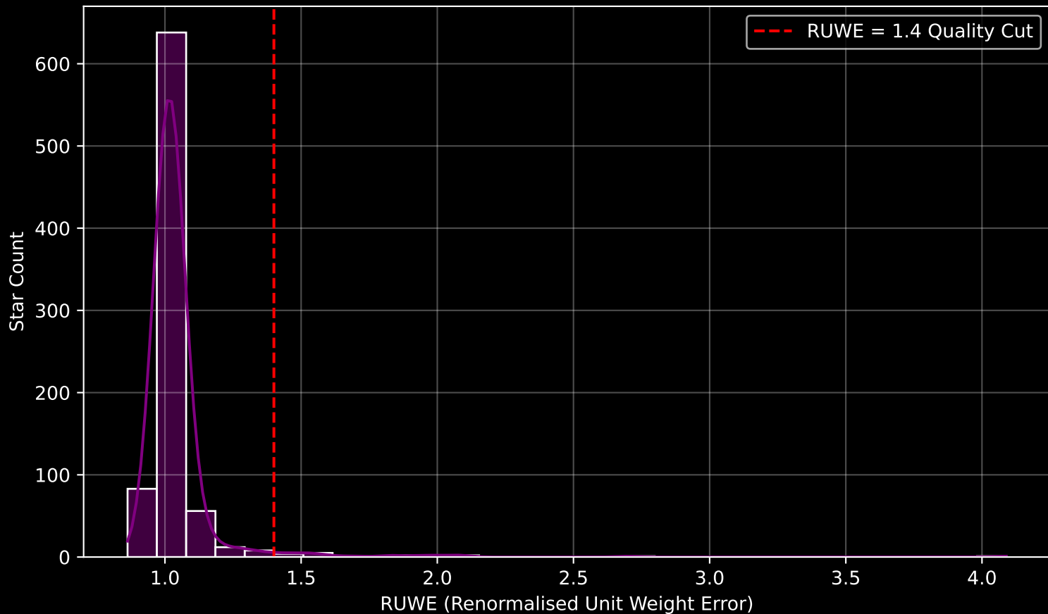
Gaia Cluster: [NGC_5617] RUWE Distribution (n= 816)
