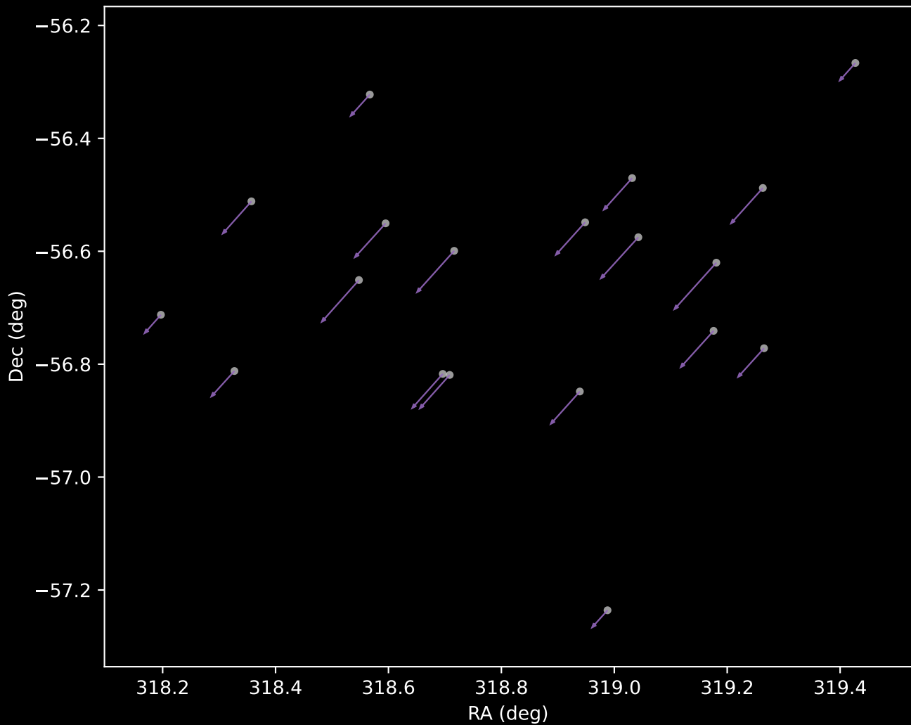
Gaia DR3 Cluster 8 Proper Motion Vectors (n=19)
