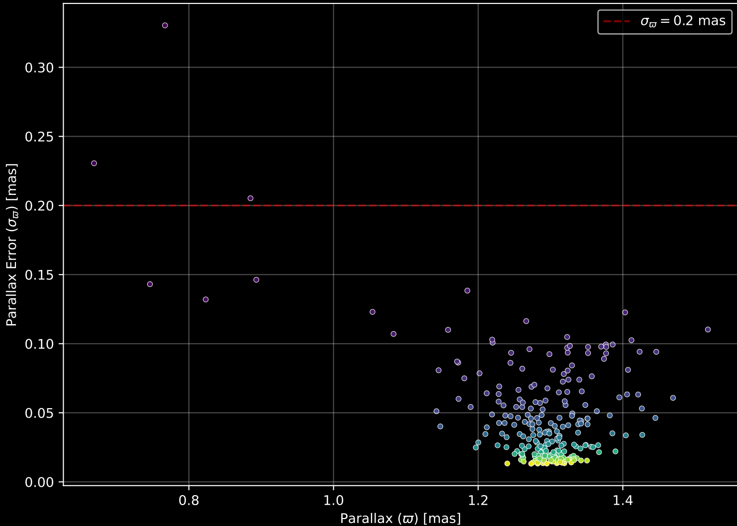
Gaia Cluster: [NGC_5662] Parallax Quality (n= 245)
