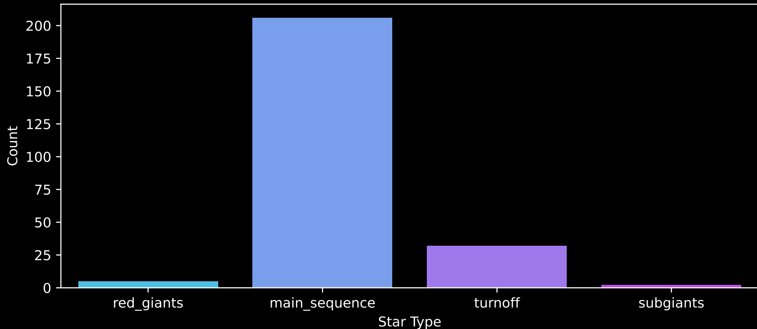
Gaia Cluster: [NGC_5662] Count plot of Star Type
