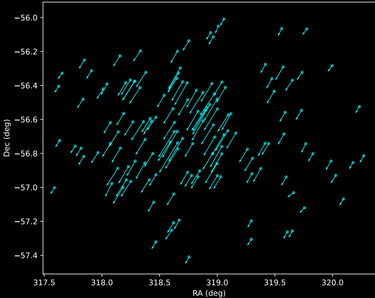
Gaia DR3 Noise Stream Proper Motion Vectors (n=135)
