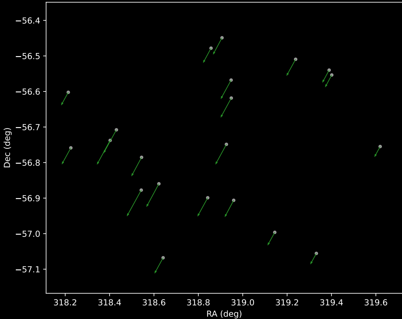
Gaia DR3 Cluster 4 Proper Motion Vectors (n=21)
