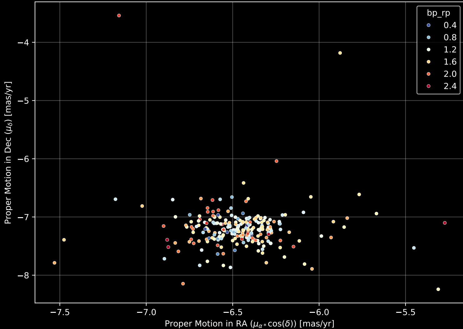
Gaia Cluster: [NGC_5662] Proper Motion Diagram (n= 245)
