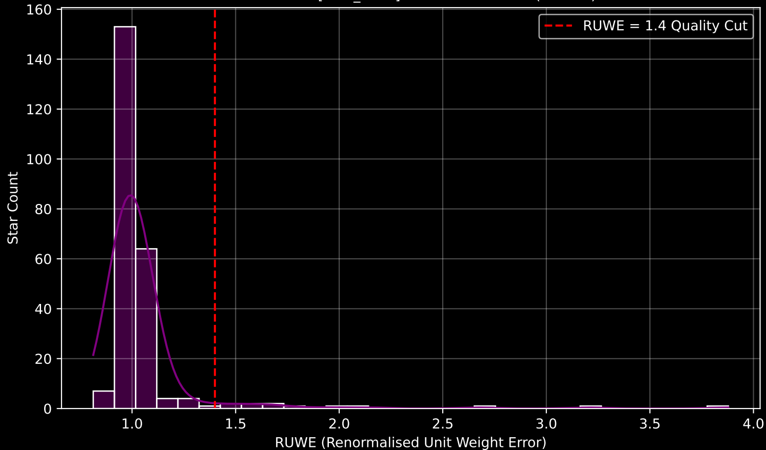
Gaia Cluster: [NGC_5662] RUWE Distribution (n= 245)
