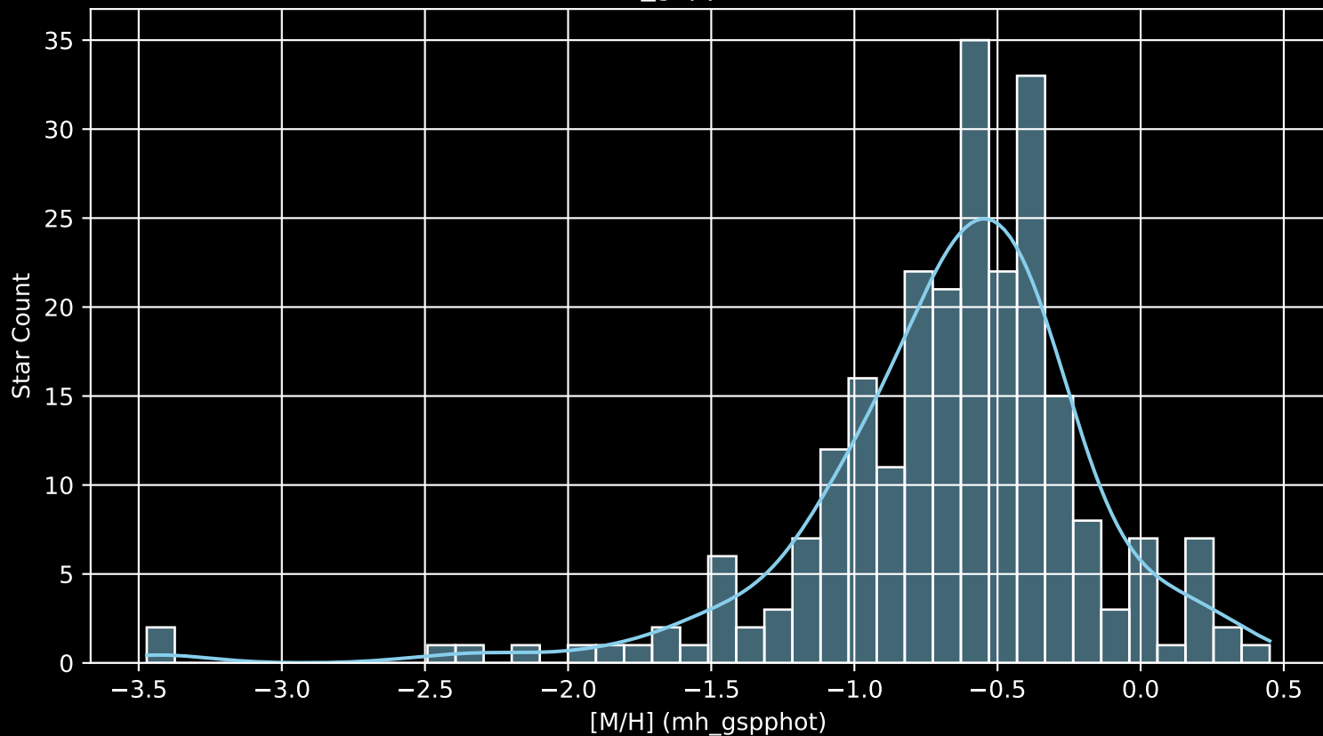
Gaia Cluster: [NGC_5662 [M/H] (mh_gspphot) (n= 245)
