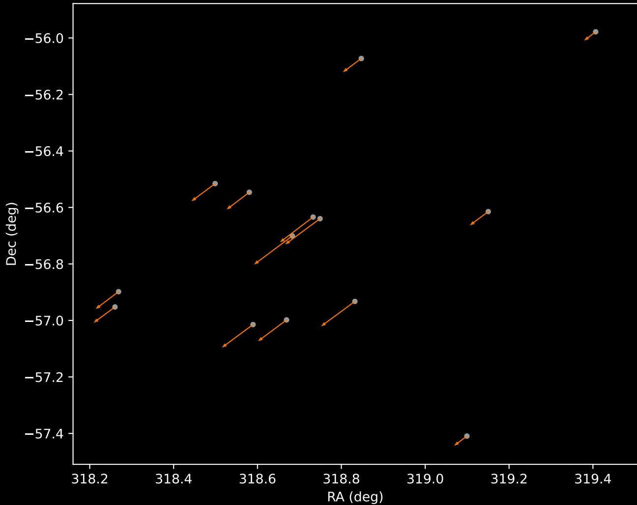
Gaia DR3 Cluster 2 Proper Motion Vectors (n=14)
