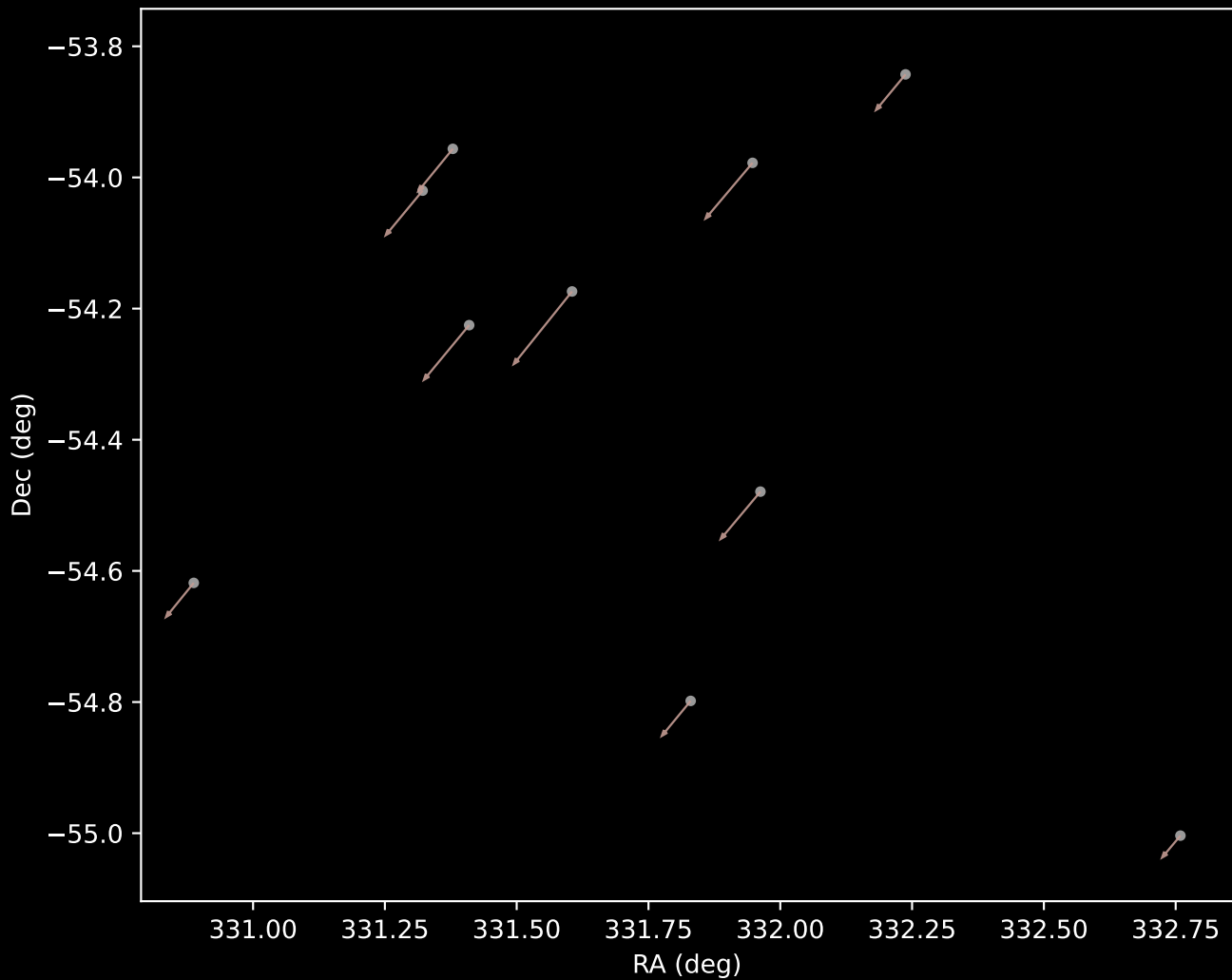
Gaia DR3 Cluster 11 Proper Motion Vectors (n=10)
