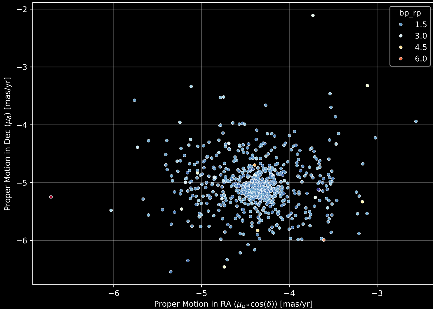
Gaia Cluster: [NGC_5925] Proper Motion Diagram (n= 769)
