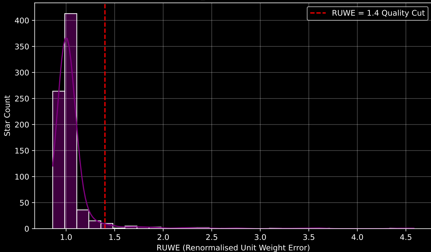
Gaia Cluster: [NGC_5925] RUWE Distribution (n= 763)
