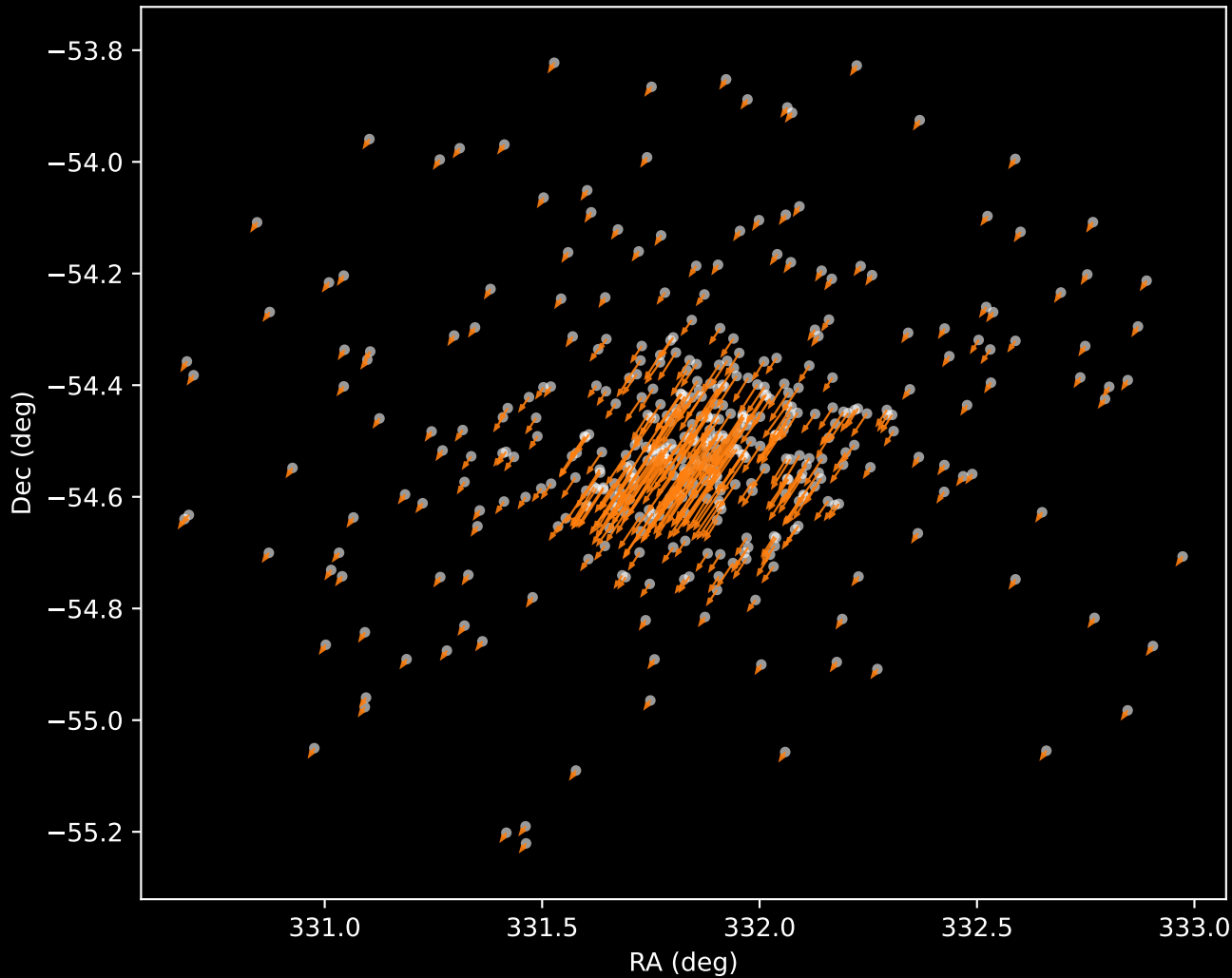
Gaia DR3 Cluster 22 Proper Motion Vectors (n=414)
