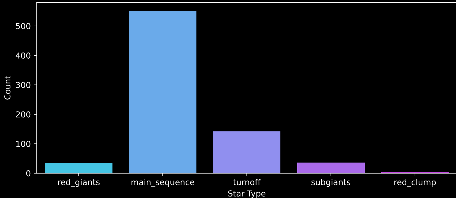
Gaia Cluster: [NGC_5925] Count plot of Star Type
