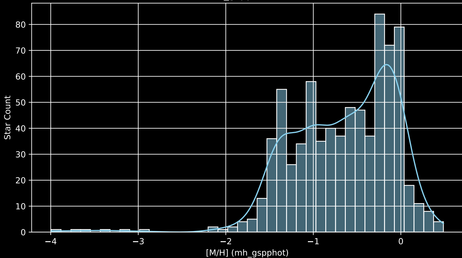
Gaia Cluster: [NGC_5925 [M/H] (mh_gspphot) (n= 762)
