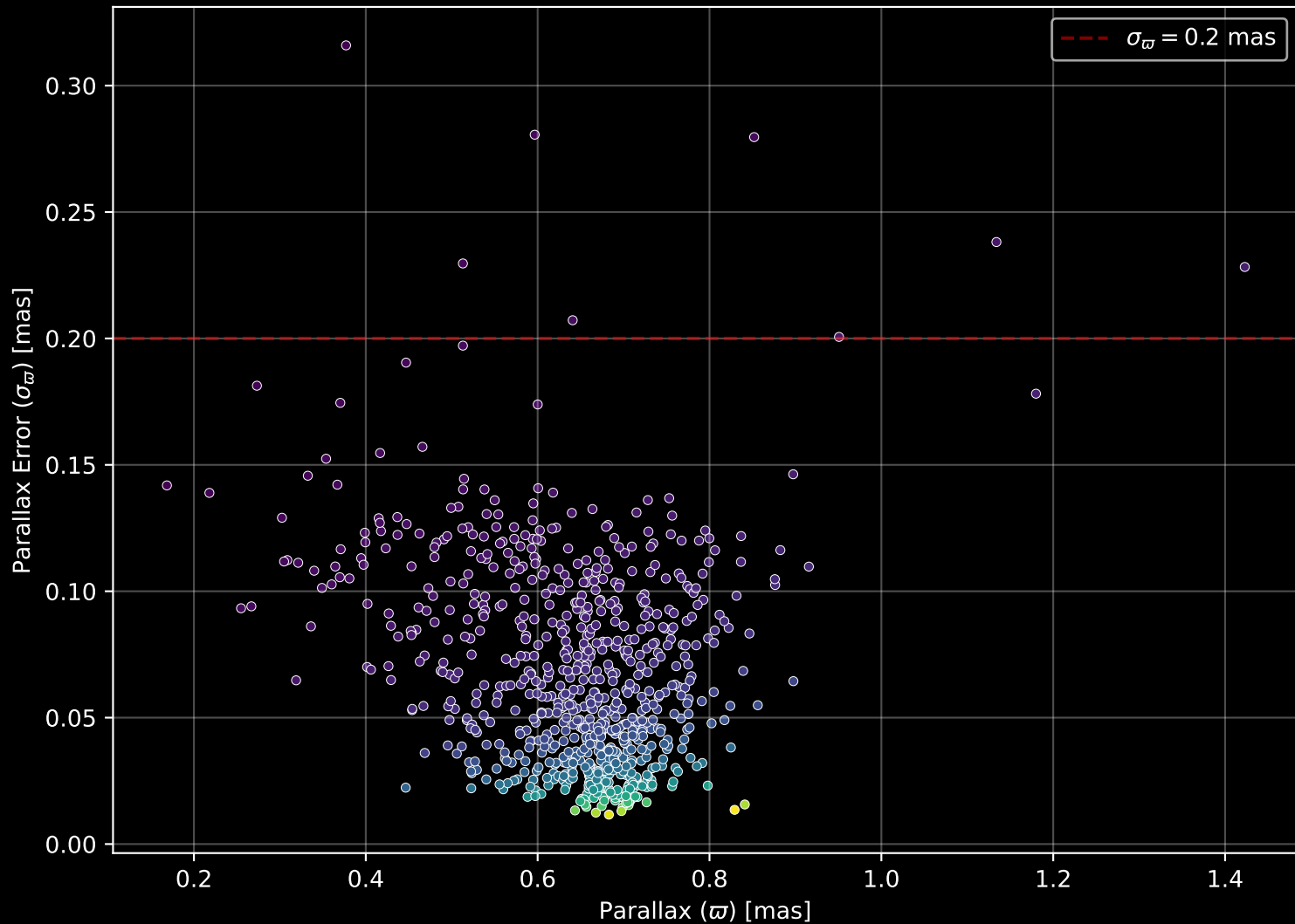
Gaia Cluster: [NGC_5925] Parallax Quality (n= 769)
