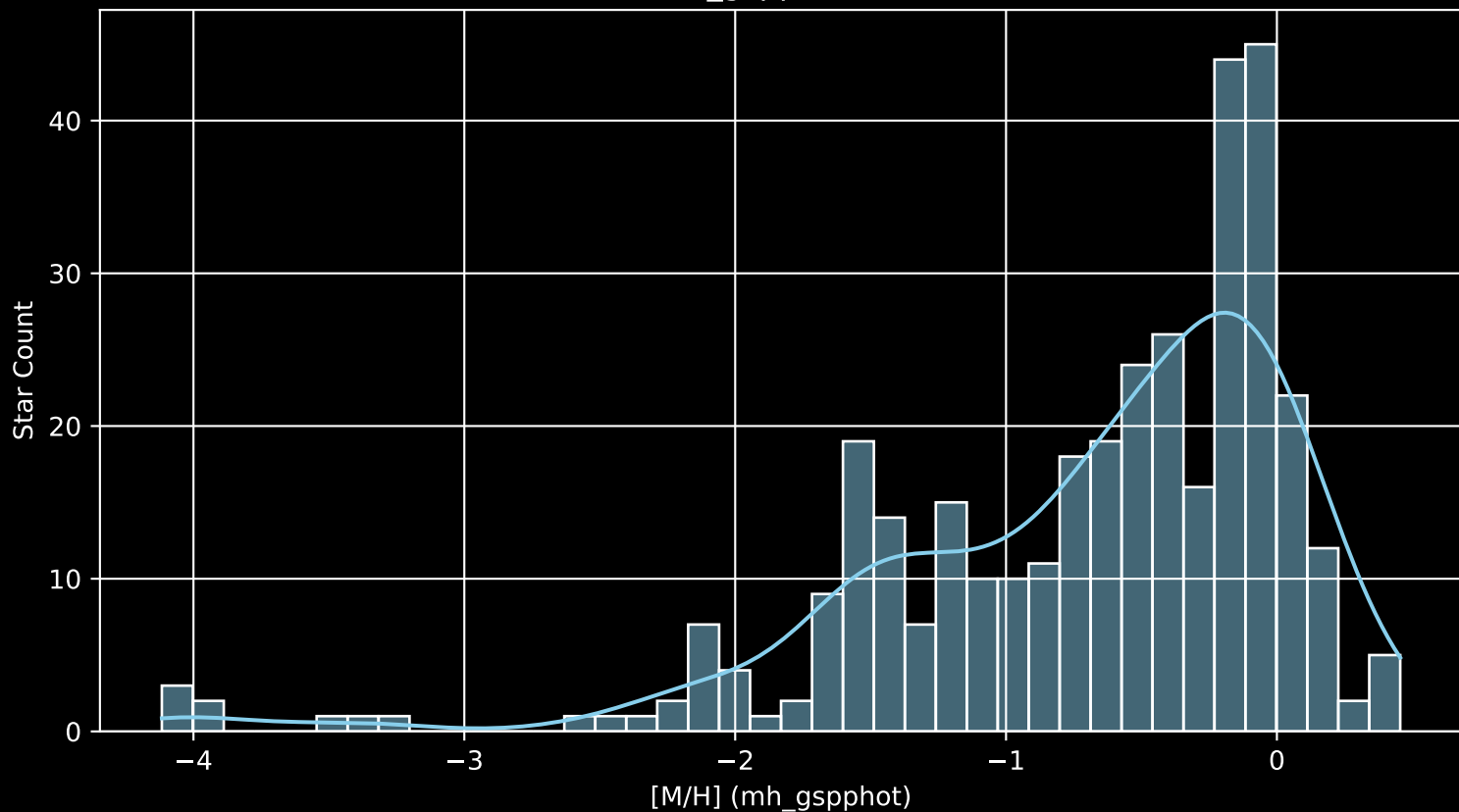
Gaia Cluster: [NGC_5999 [M/H] (mh_gspphot) (n= 355)
