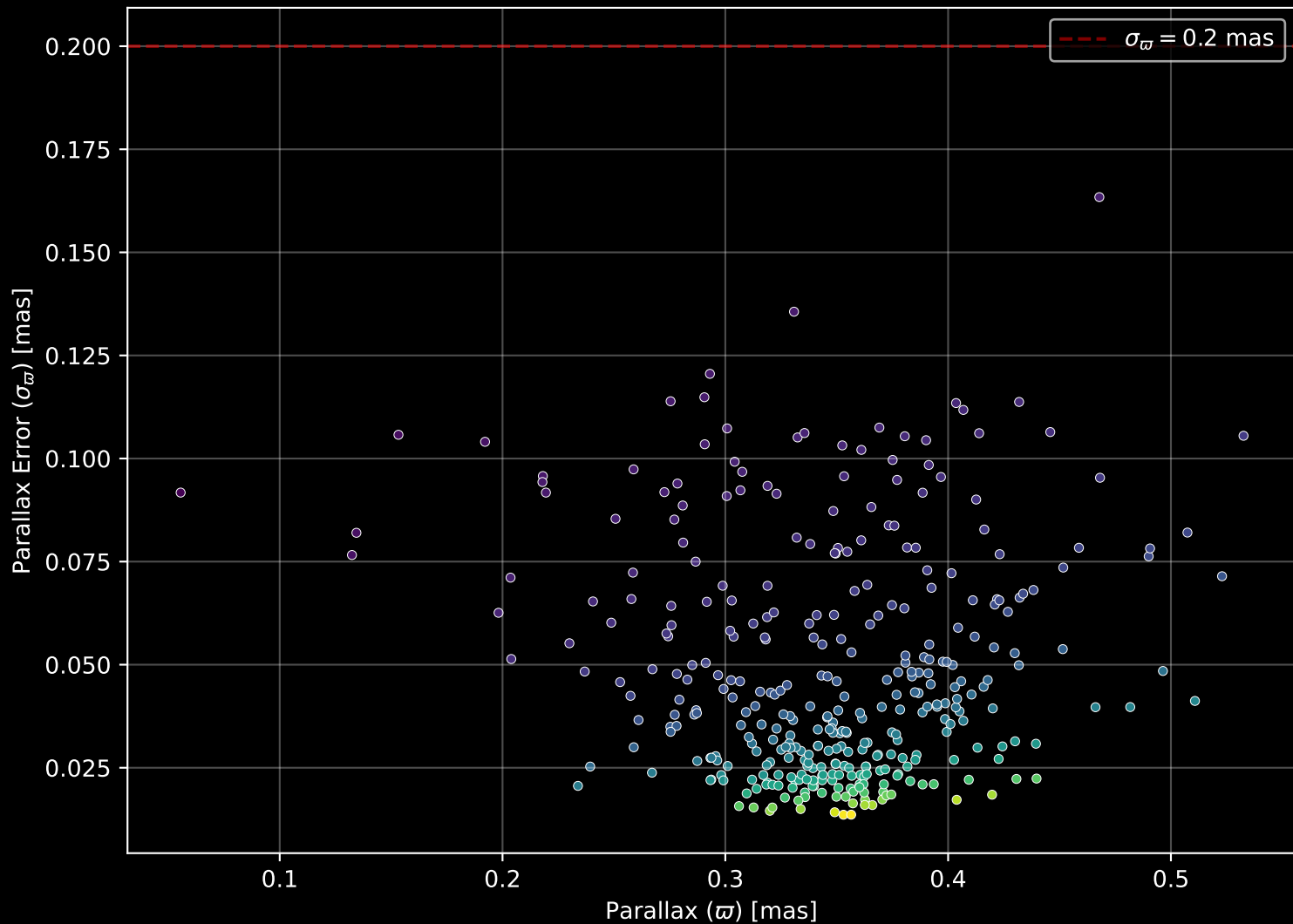
Gaia Cluster: [NGC_5999] Parallax Quality (n= 358)
