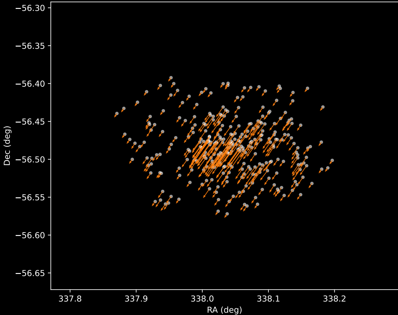
Gaia DR3 Cluster 2 Proper Motion Vectors (n=287)
