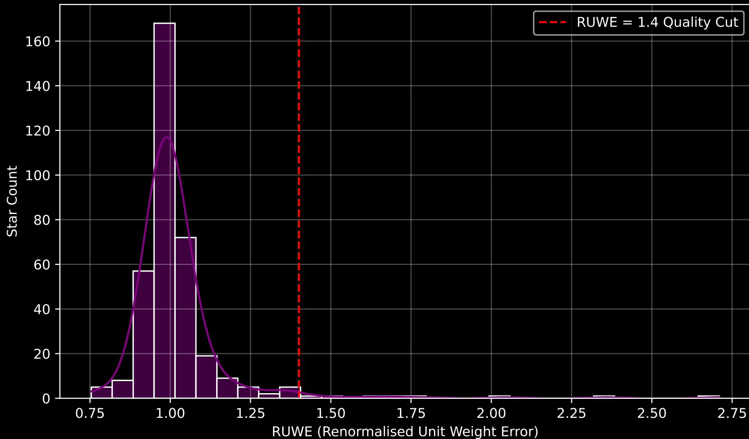
Gaia Cluster: [NGC_5999] RUWE Distribution (n= 358)
