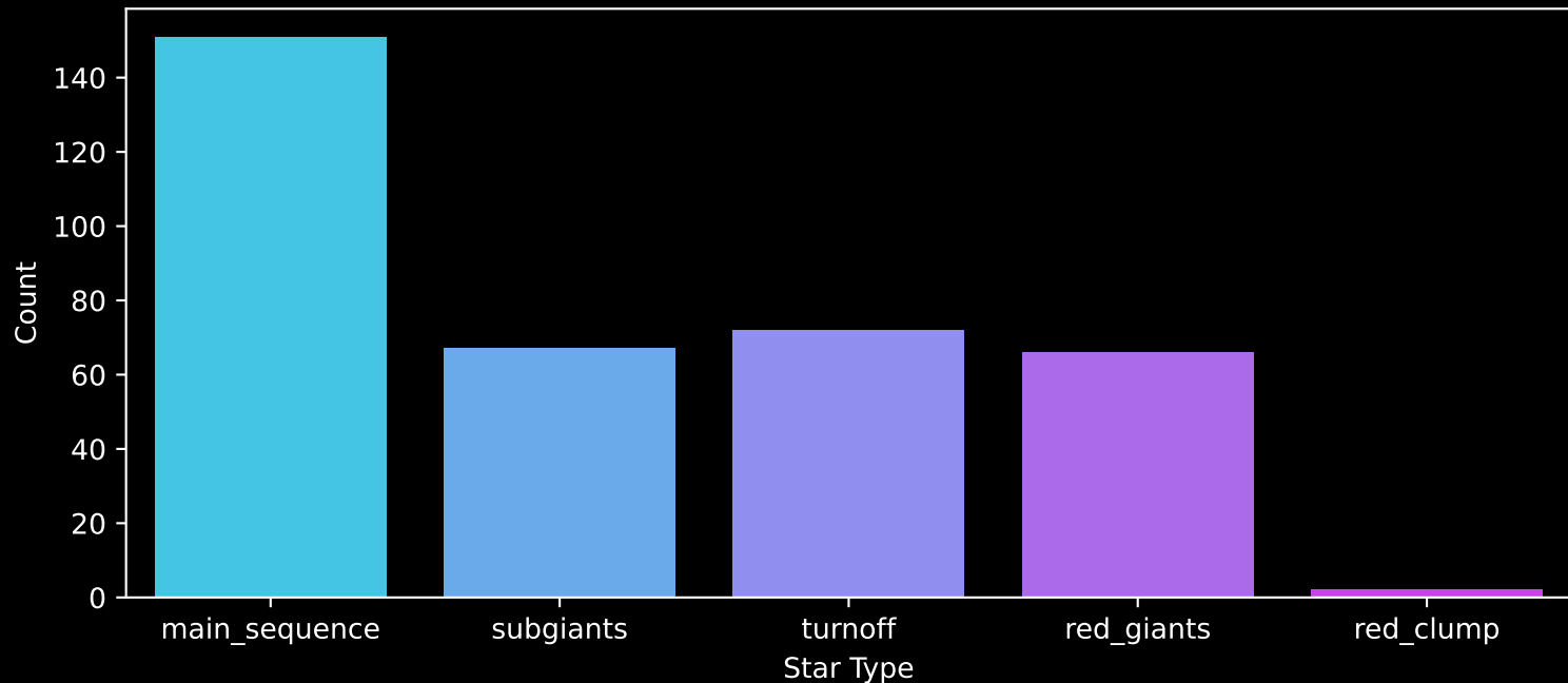
Gaia Cluster: [NGC_5999] Count plot of Star Type
