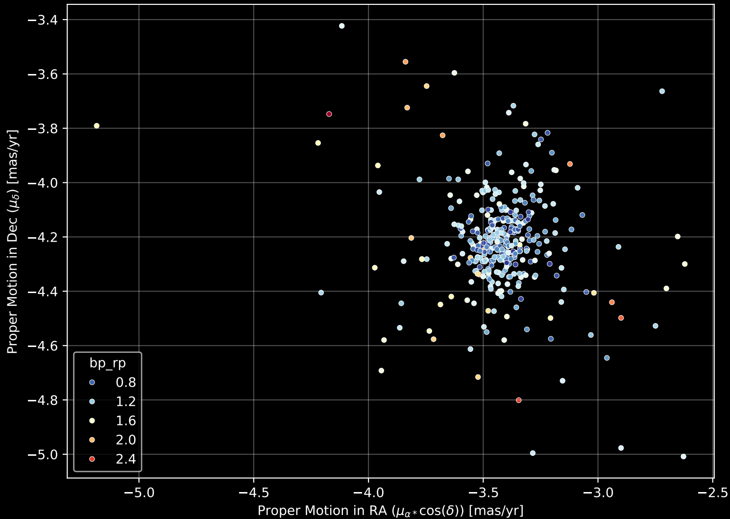
Gaia Cluster: [NGC_5999] Proper Motion Diagram (n= 358)
