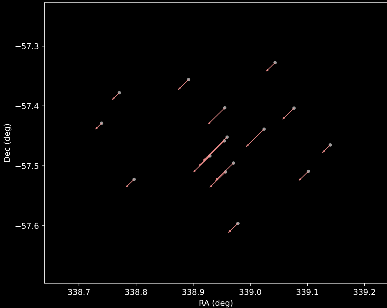
Gaia DR3 Cluster 27 Proper Motion Vectors (n=16)
