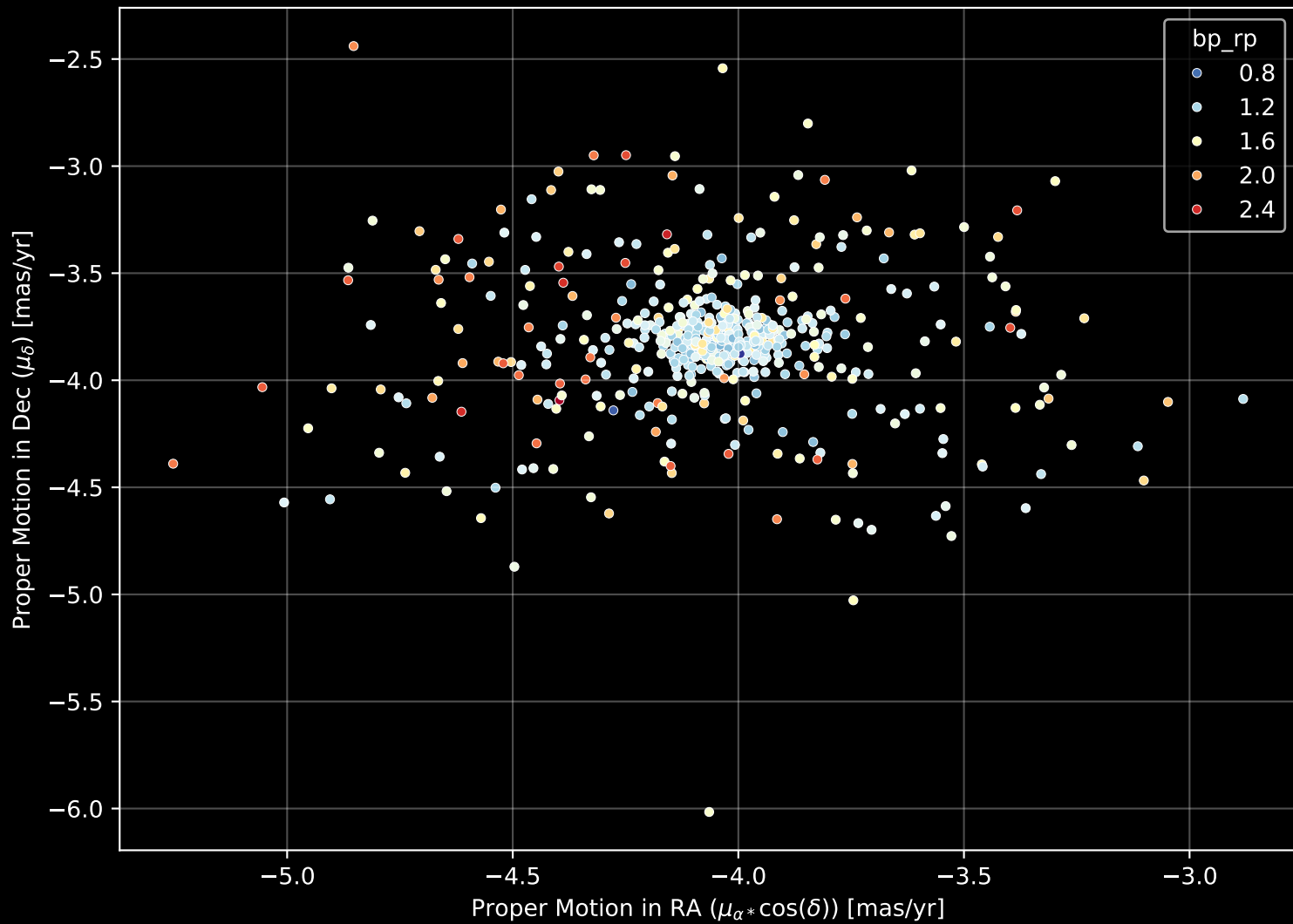
Gaia Cluster: [NGC_6005] Proper Motion Diagram (n= 542)
