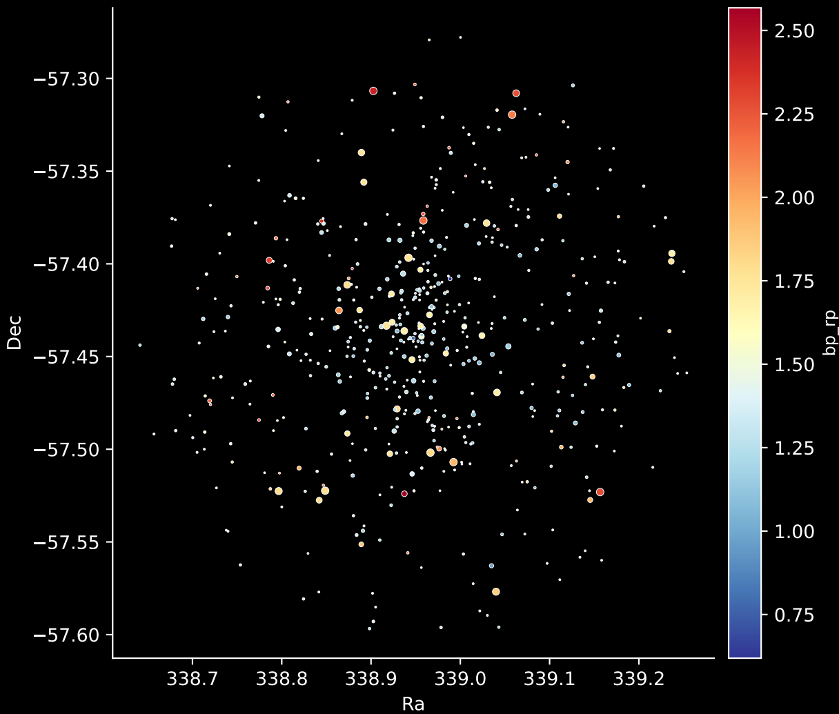
Gaia Cluster: [NGC_6005] Stars: 542
