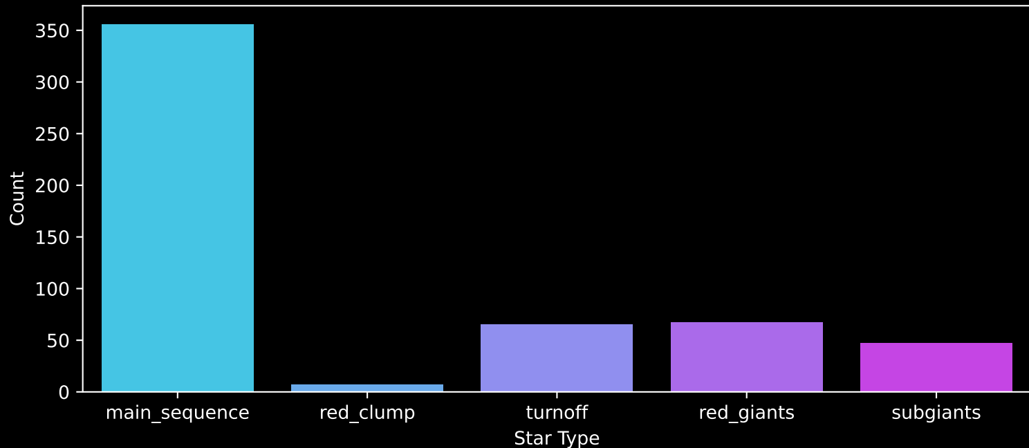
Gaia Cluster: [NGC_6005] Count plot of Star Type
