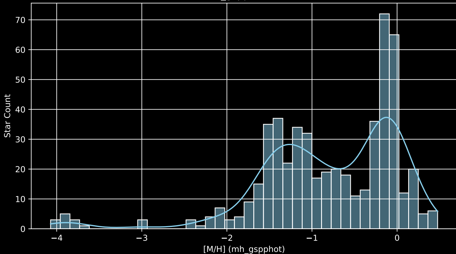
Gaia Cluster: [NGC_6005 [M/H] (mh_gspphot) (n= 535)
