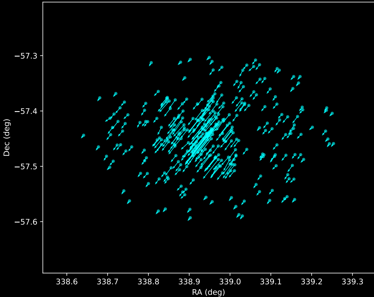
Gaia DR3 Noise Stream Proper Motion Vectors (n=295)
