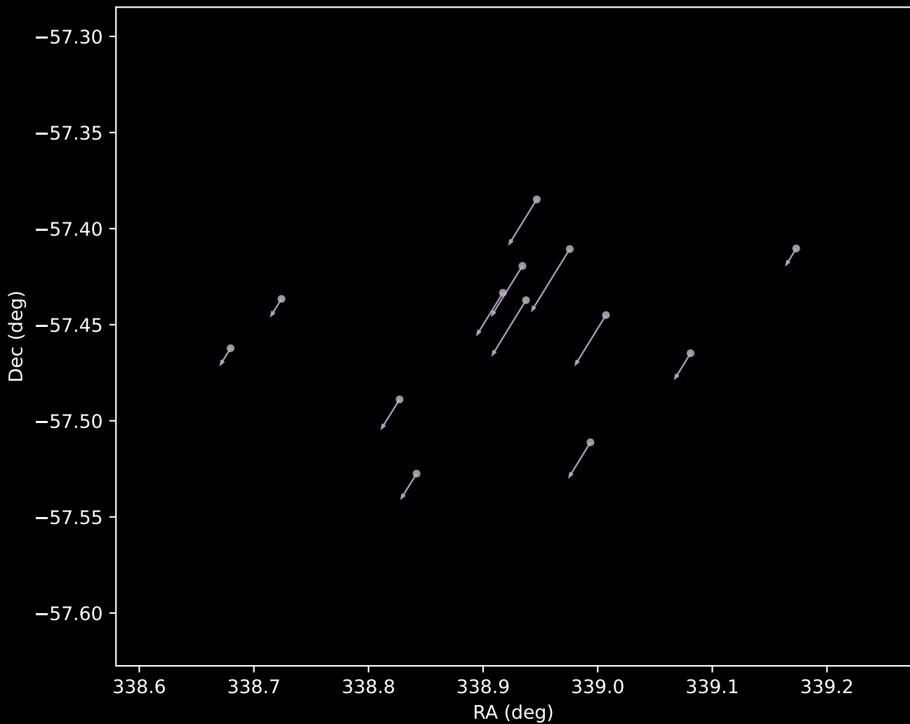
Gaia DR3 Cluster 29 Proper Motion Vectors (n=13)
