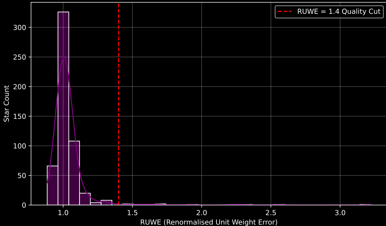
Gaia Cluster: [NGC_6005] RUWE Distribution (n= 542)
