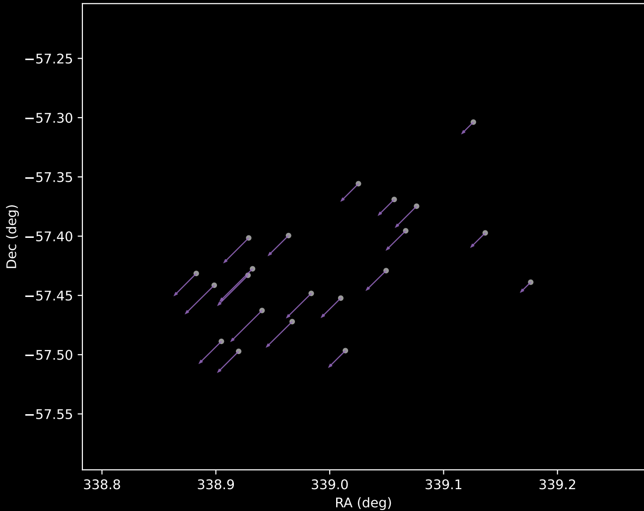
Gaia DR3 Cluster 28 Proper Motion Vectors (n=21)
