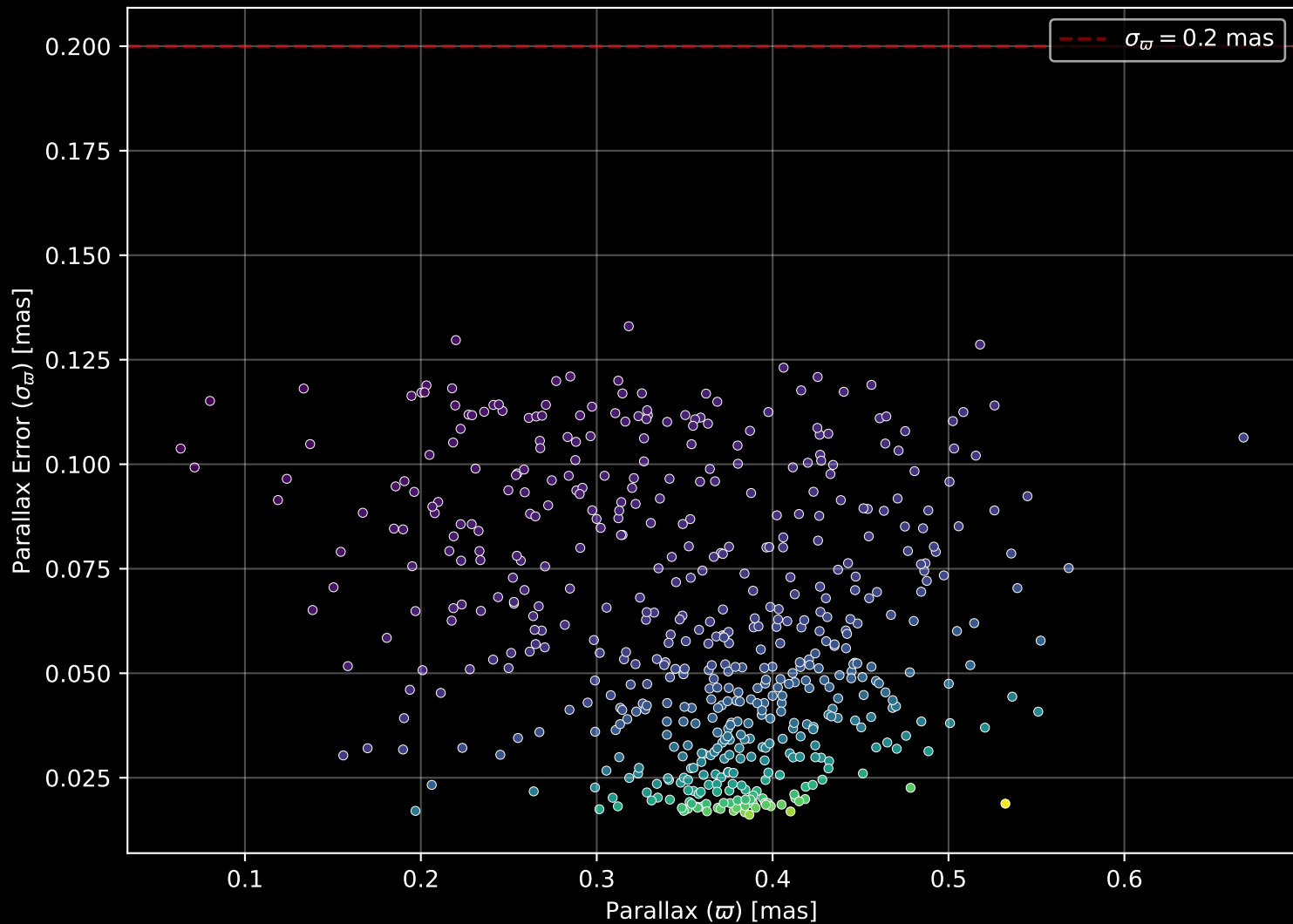
Gaia Cluster: [NGC_6005] Parallax Quality (n= 542)
