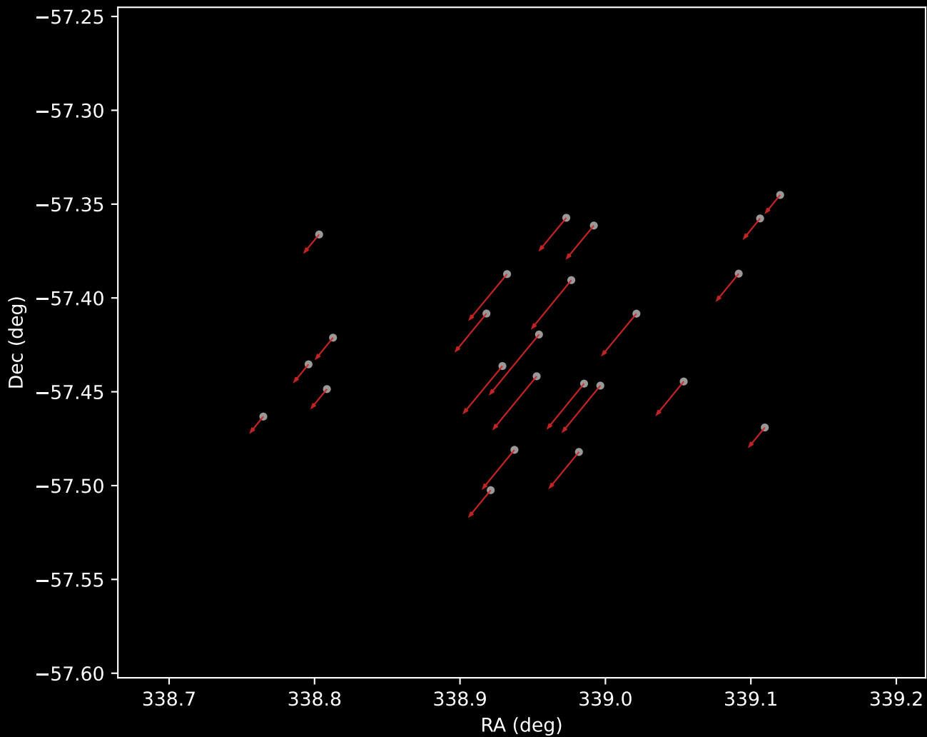
Gaia DR3 Cluster 26 Proper Motion Vectors (n=24)
