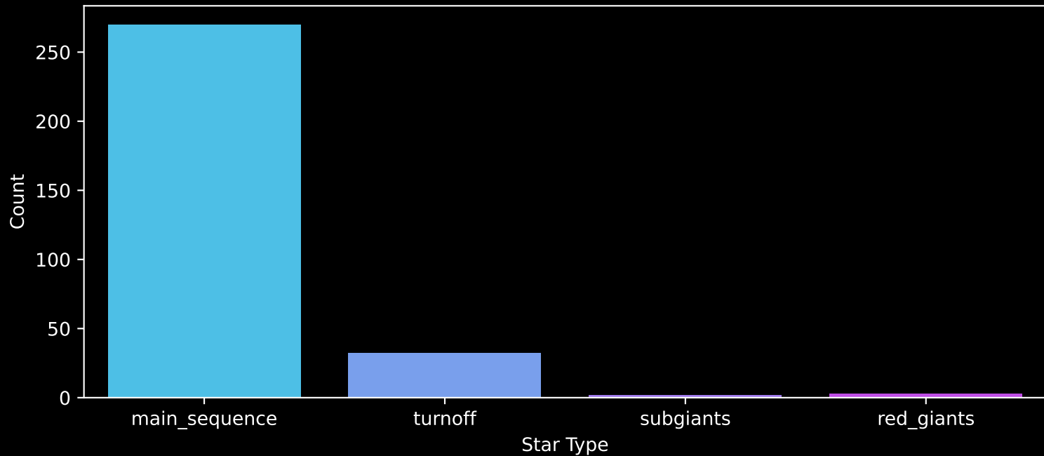
Gaia Cluster: [NGC_6025] Count plot of Star Type
