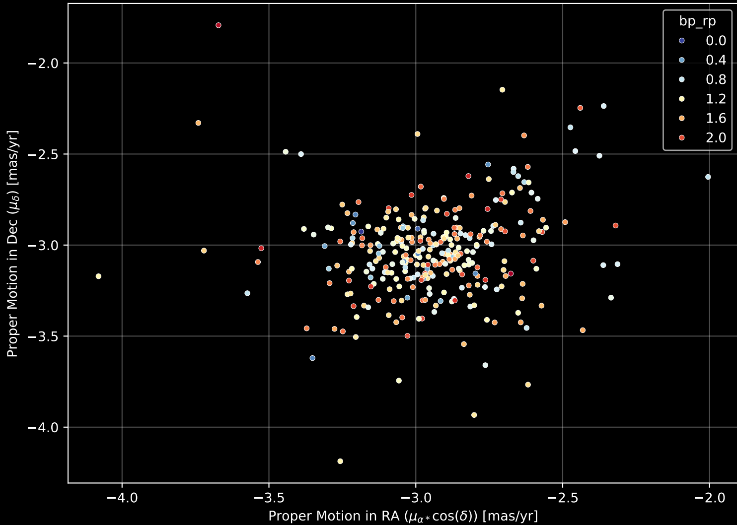
Gaia Cluster: [NGC_6025] Proper Motion Diagram (n= 307)
