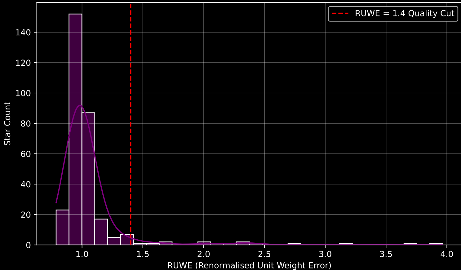
Gaia Cluster: [NGC_6025] RUWE Distribution (n= 305)
