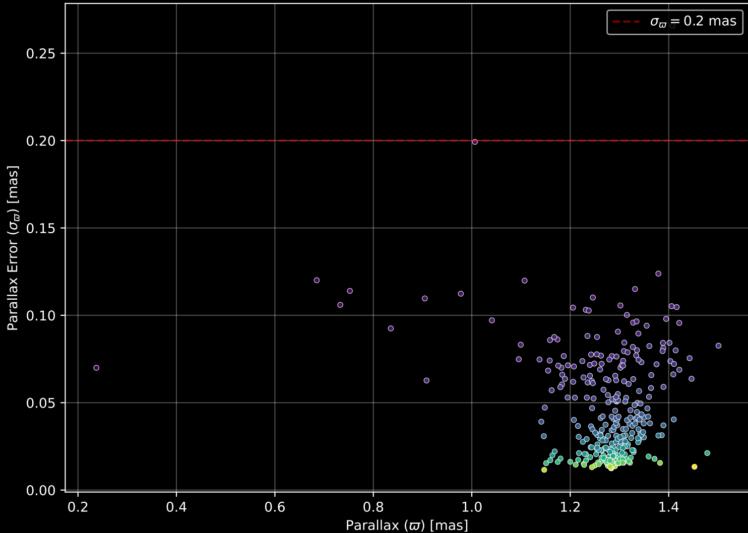
Gaia Cluster: [NGC_6025] Parallax Quality (n= 307)
