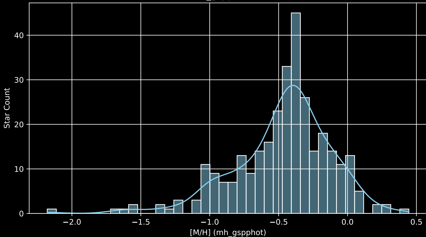
Gaia Cluster: [NGC_6025 [M/H] (mh_gspphot) (n= 307)
