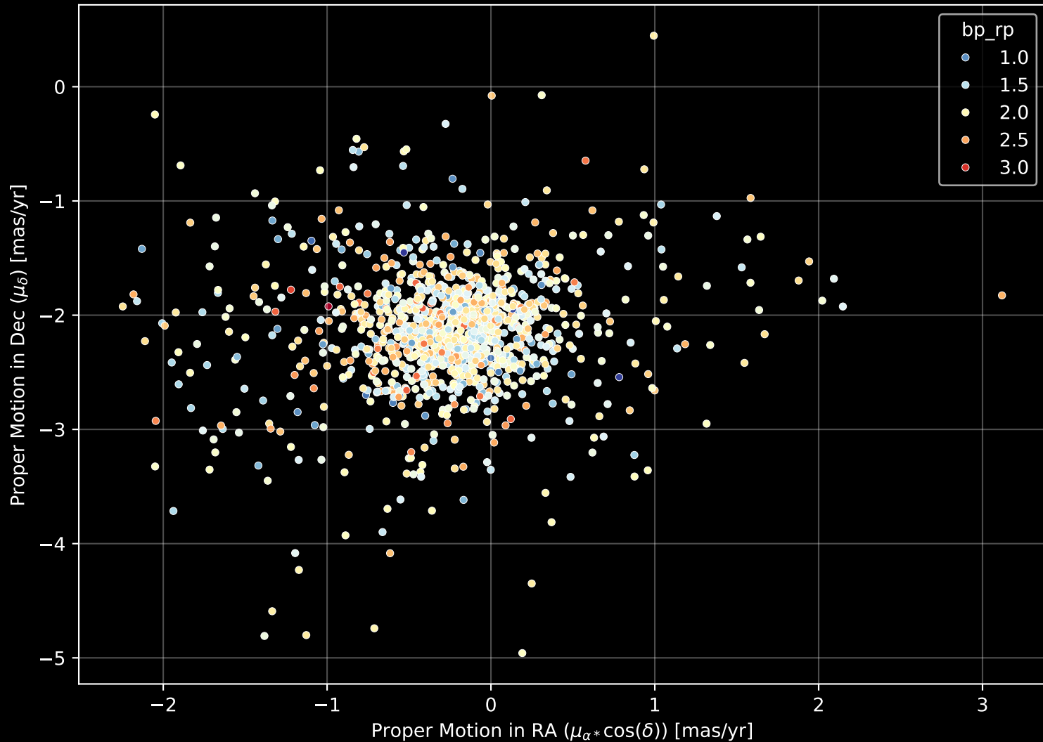
Gaia Cluster: [NGC_6124] Proper Motion Diagram (n= 1259)
