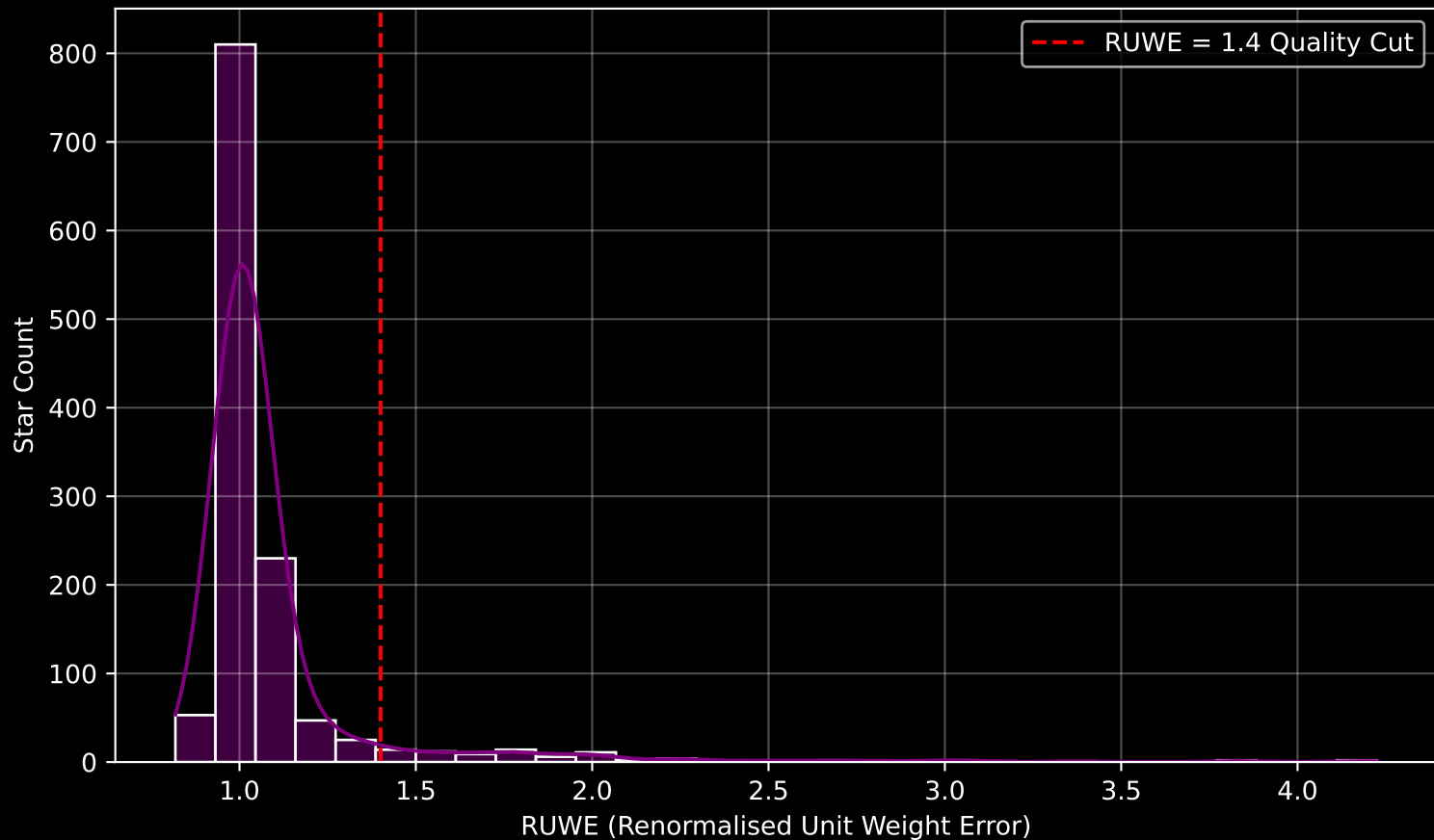
Gaia Cluster: [NGC_6124] RUWE Distribution (n= 1254)
