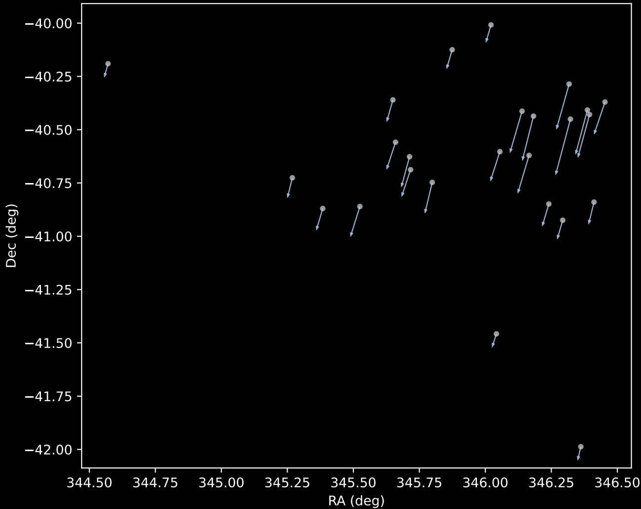
Gaia DR3 Cluster 41 Proper Motion Vectors (n=25)
