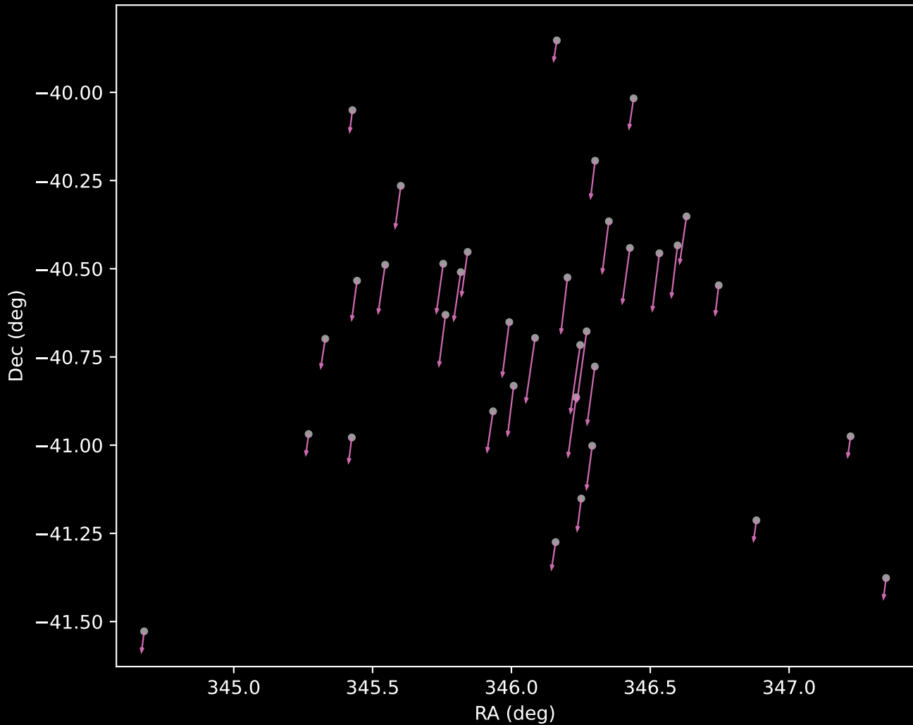
Gaia DR3 Cluster 52 Proper Motion Vectors (n=36)
