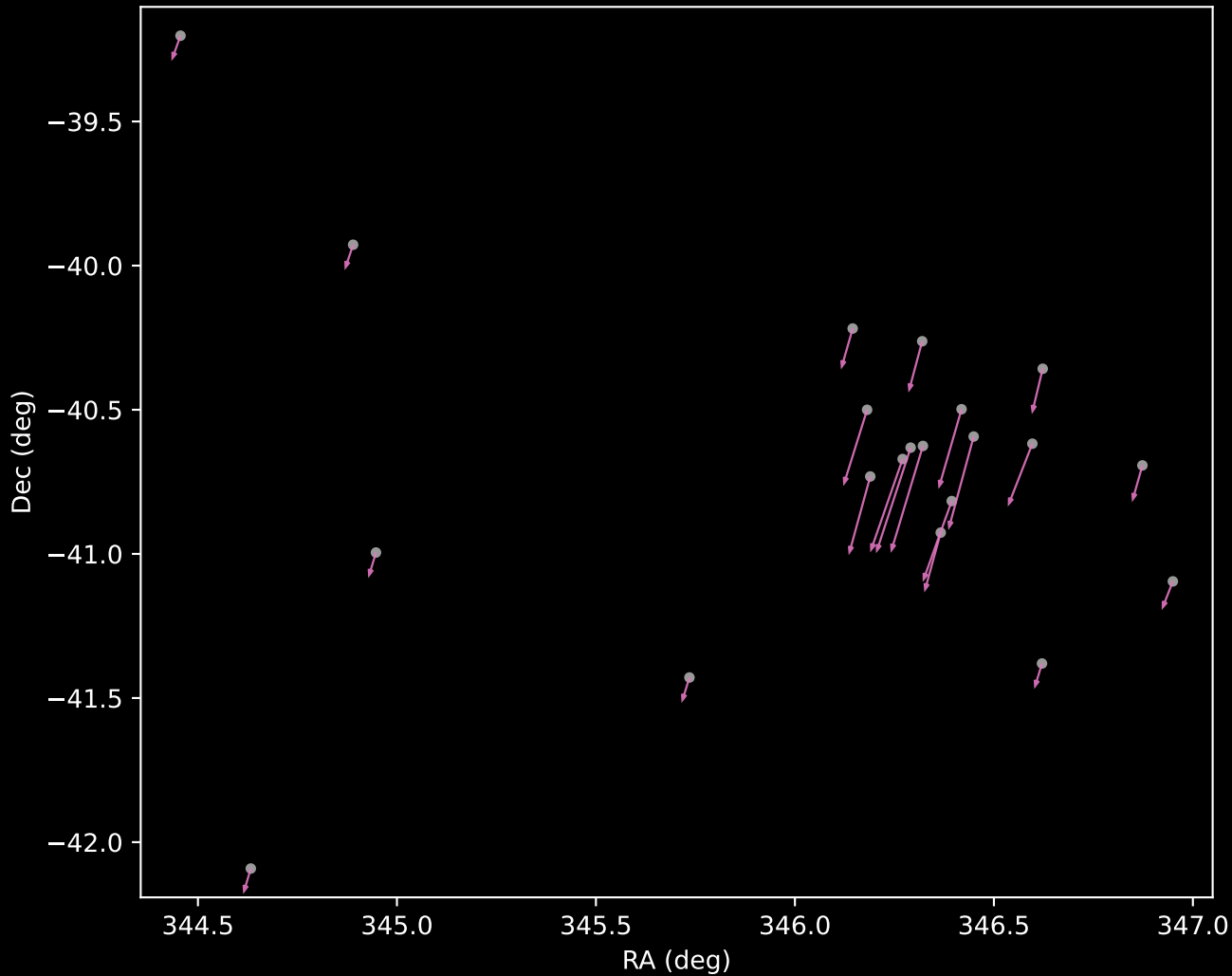
Gaia DR3 Cluster 12 Proper Motion Vectors (n=21)
