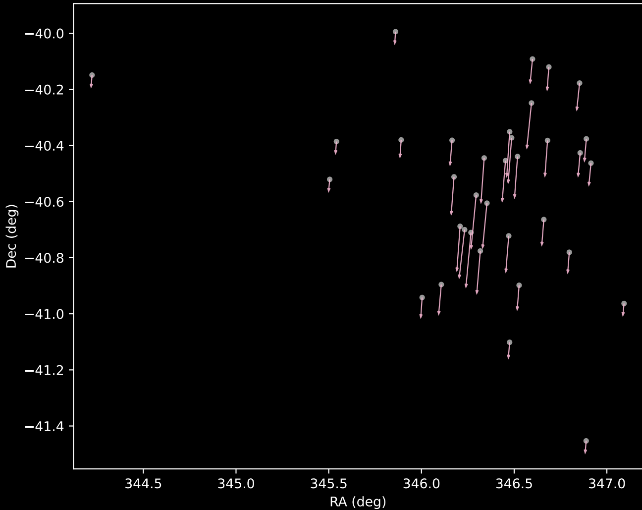
Gaia DR3 Cluster 53 Proper Motion Vectors (n=35)
