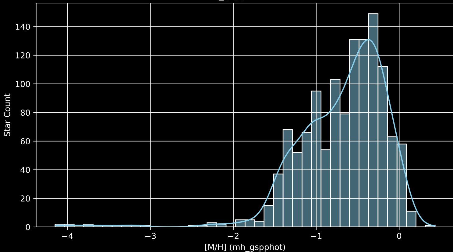
Gaia Cluster: [NGC_6124 [M/H] (mh_gspphot) (n= 1258)
