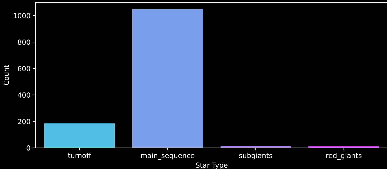
Gaia Cluster: [NGC_6124] Count plot of Star Type
