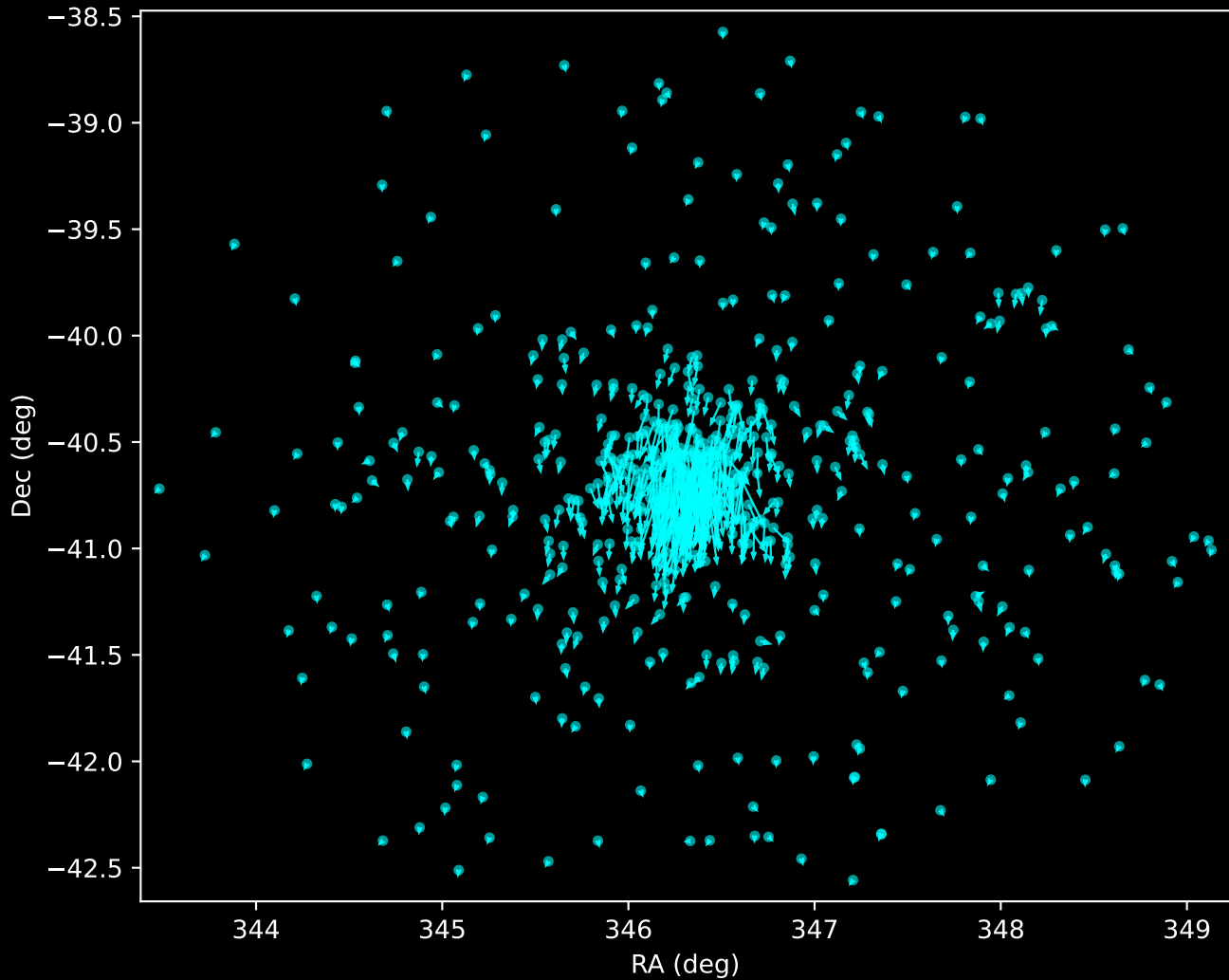
Gaia DR3 Noise Stream Proper Motion Vectors (n=586)
