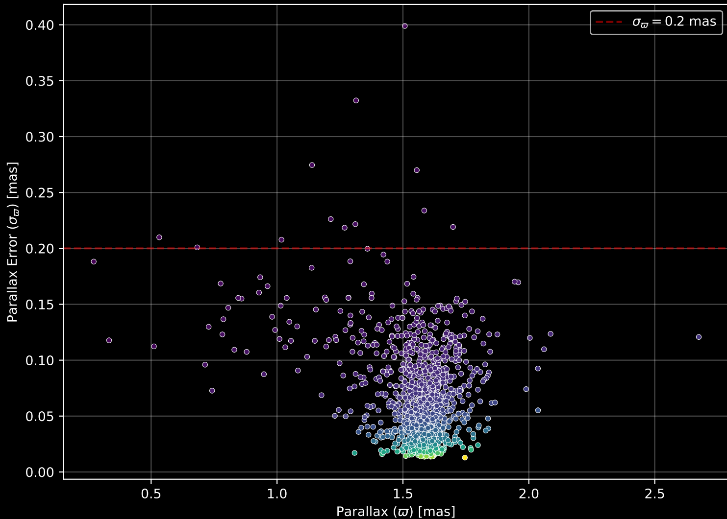
Gaia Cluster: [NGC_6124] Parallax Quality (n= 1259)
