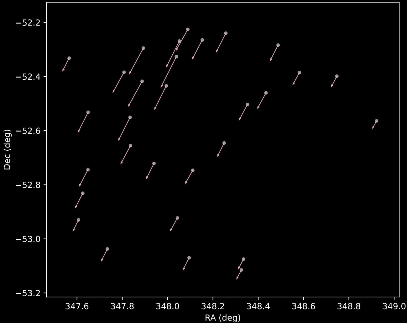
Gaia DR3 Cluster 13 Proper Motion Vectors (n=30)
