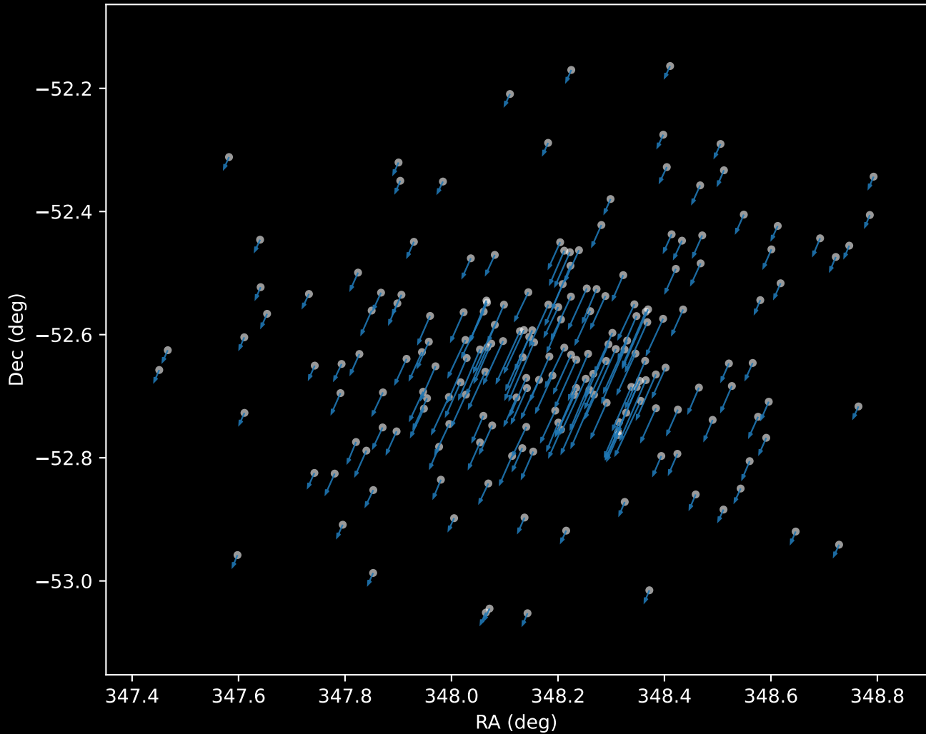
Gaia DR3 Cluster 20 Proper Motion Vectors (n=191)
