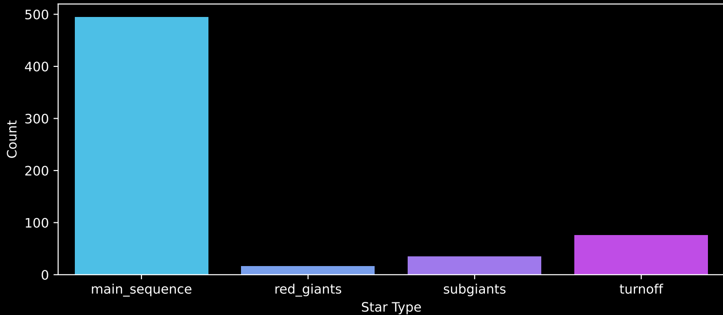
Gaia Cluster: [NGC_6152] Count plot of Star Type
