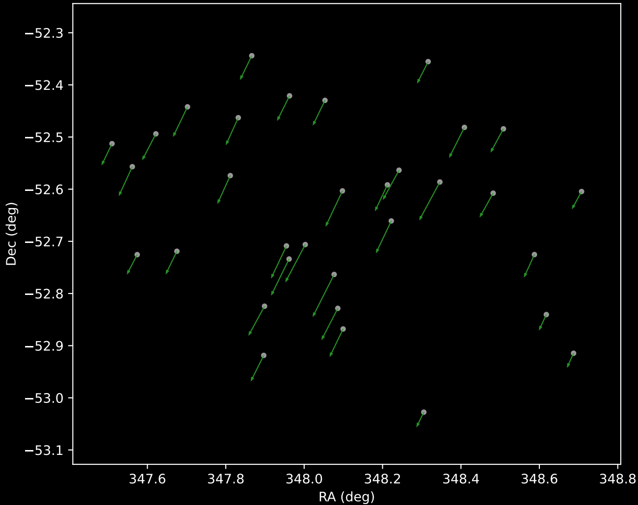
Gaia DR3 Cluster 4 Proper Motion Vectors (n=33)
