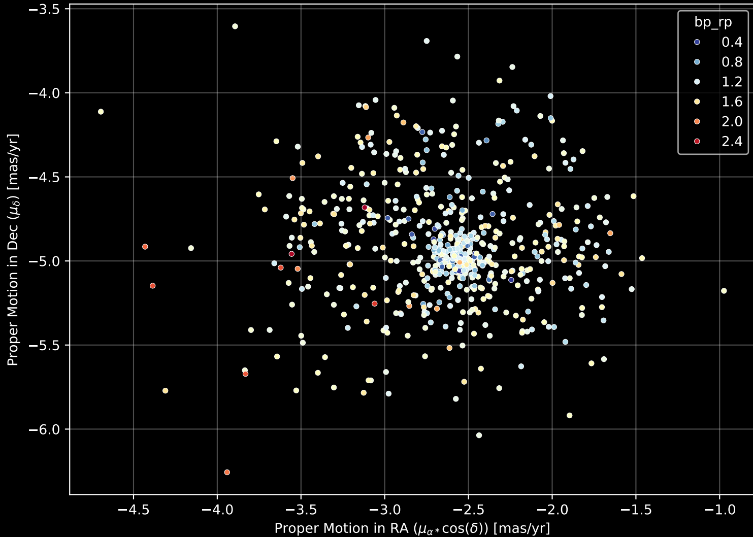
Gaia Cluster: [NGC_6152] Proper Motion Diagram (n= 622)
