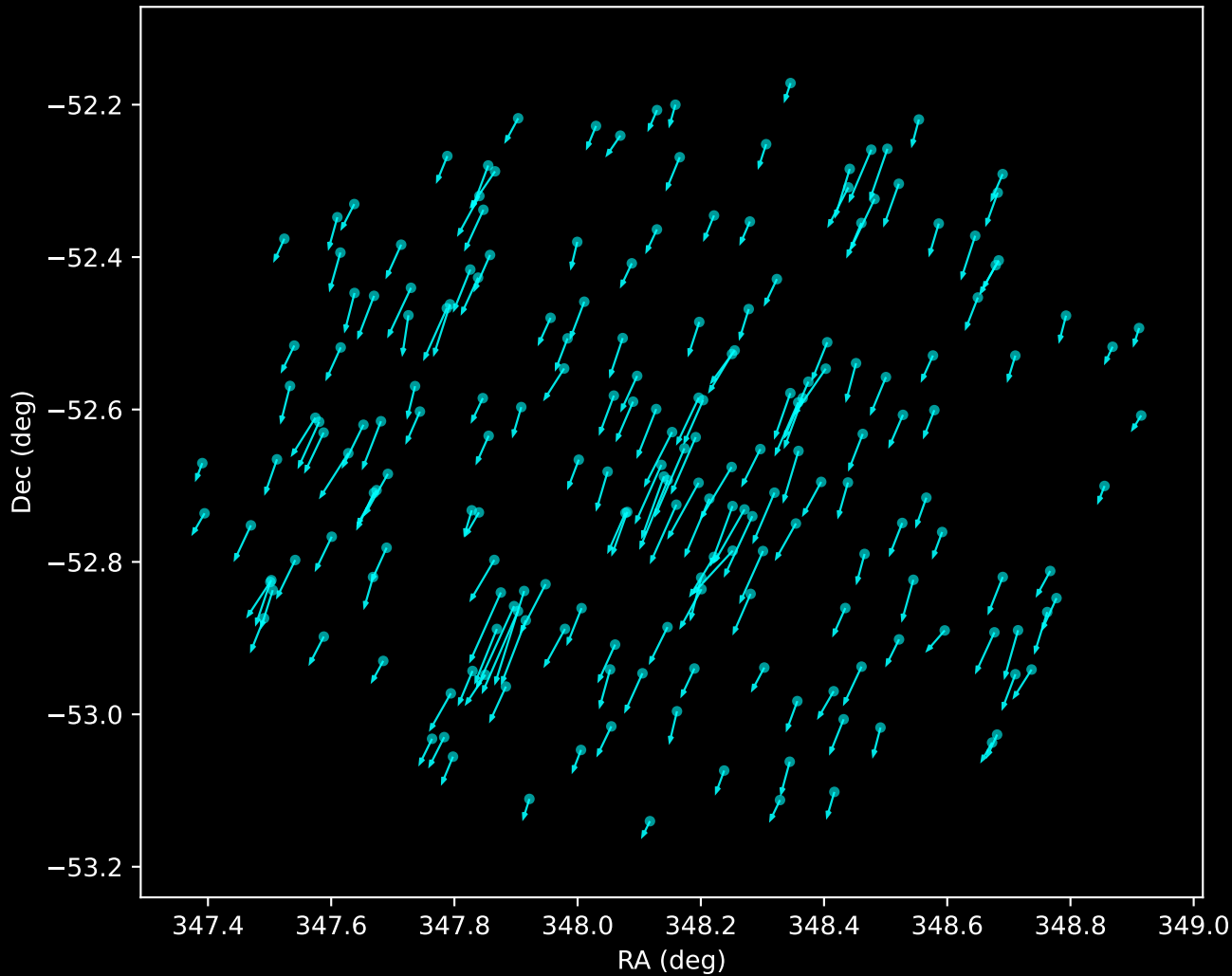
Gaia DR3 Noise Stream Proper Motion Vectors (n=198)
