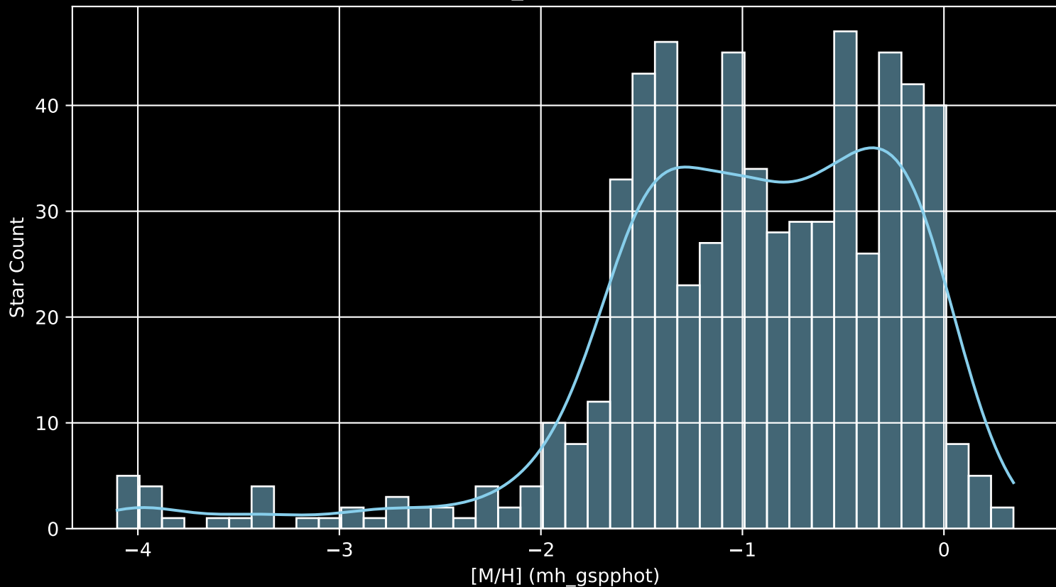
Gaia Cluster: [NGC_6152 [M/H] (mh_gspphot) (n= 621)
