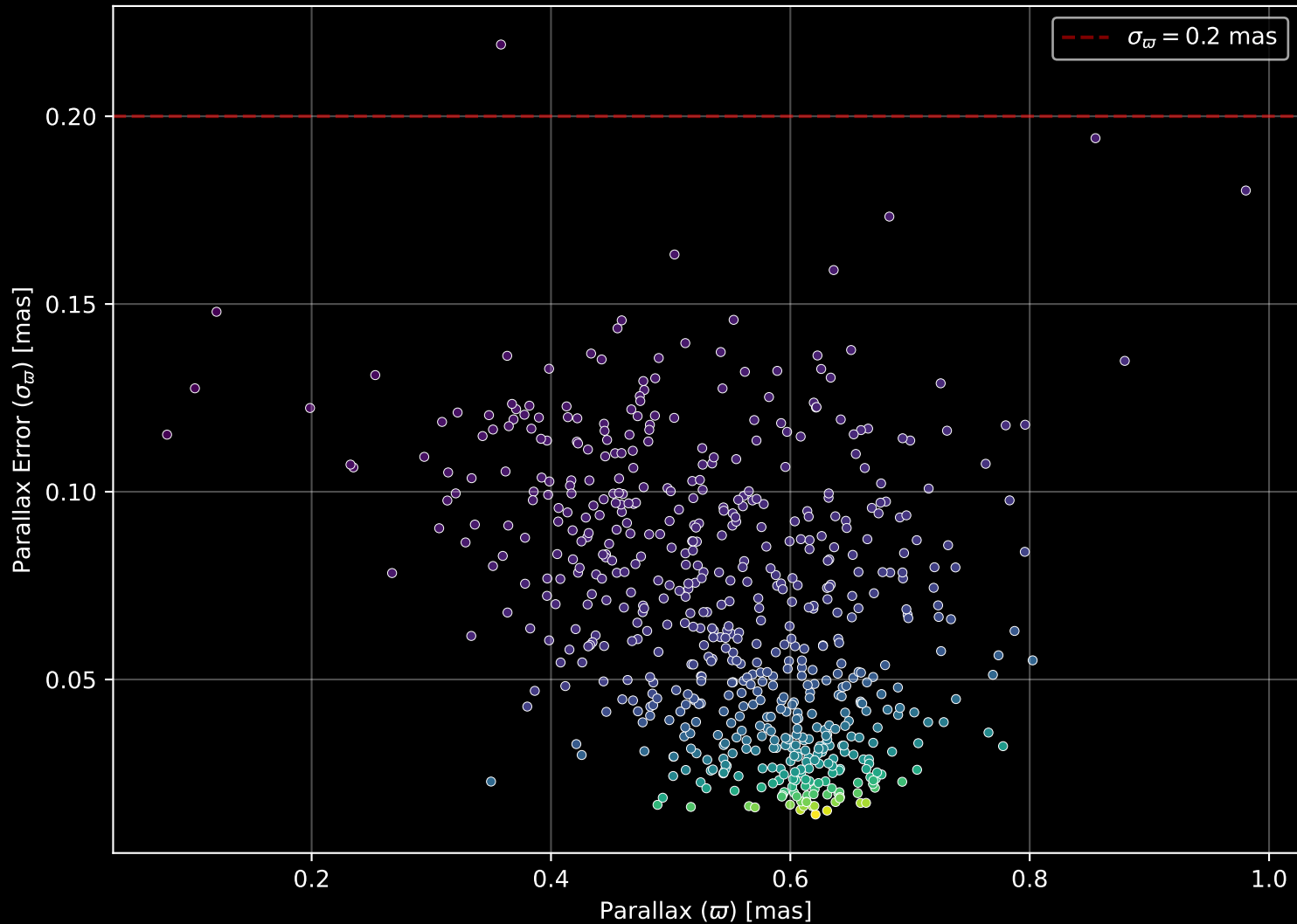
Gaia Cluster: [NGC_6152] Parallax Quality (n= 622)
