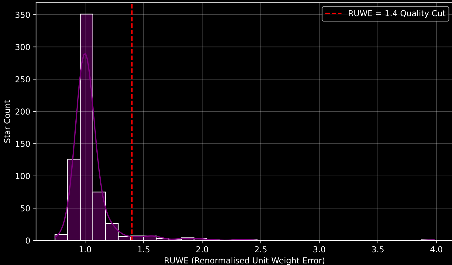
Gaia Cluster: [NGC_6152] RUWE Distribution (n= 622)
