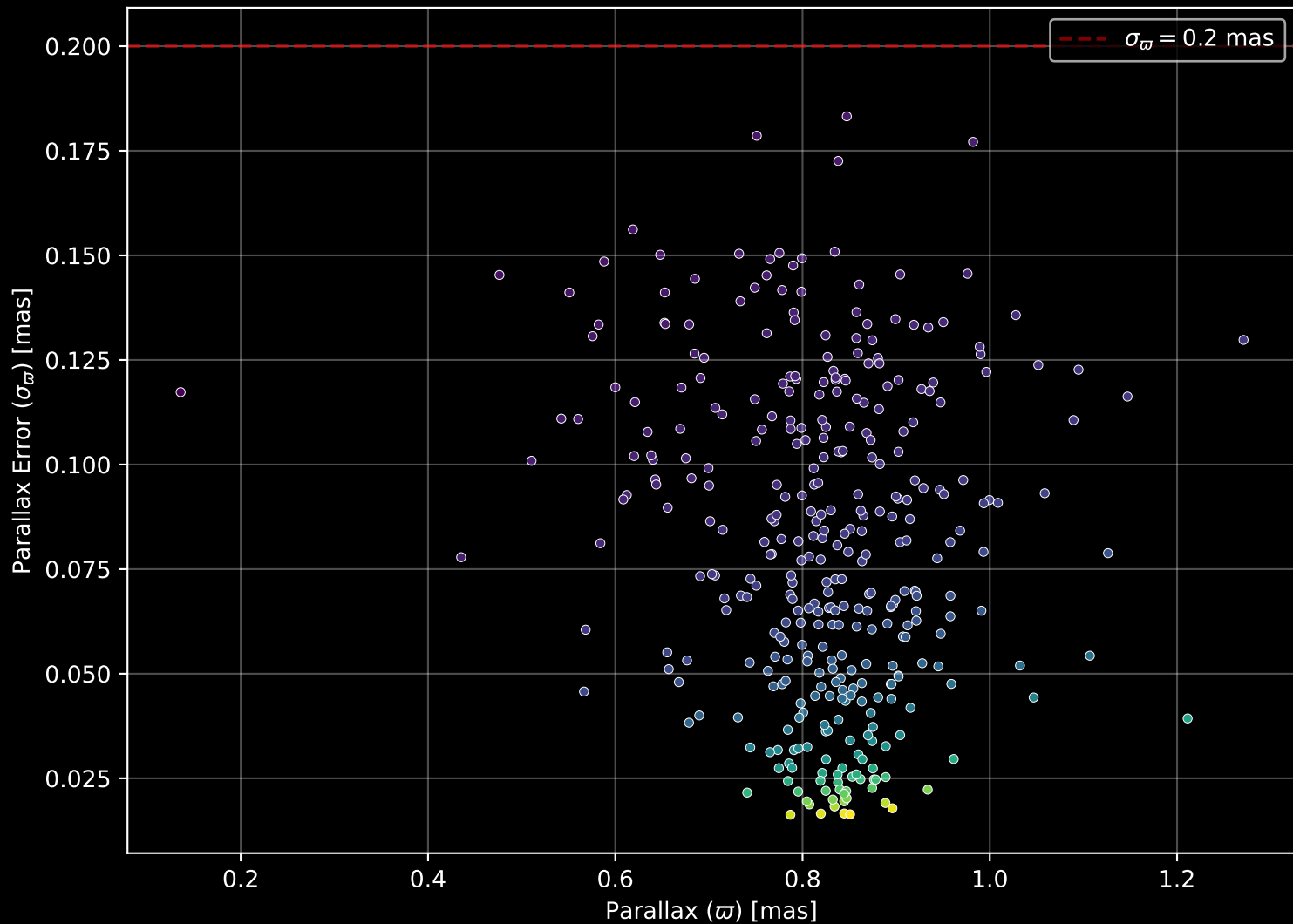
Gaia Cluster: [NGC_6193] Parallax Quality (n= 359)
