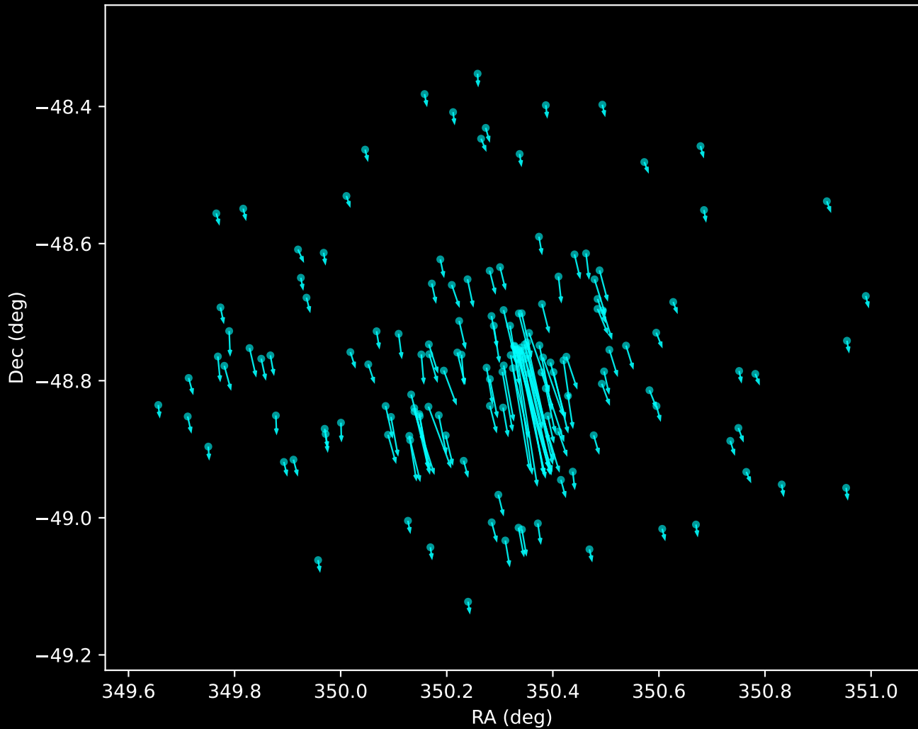
Gaia DR3 Noise Stream Proper Motion Vectors (n=151)
