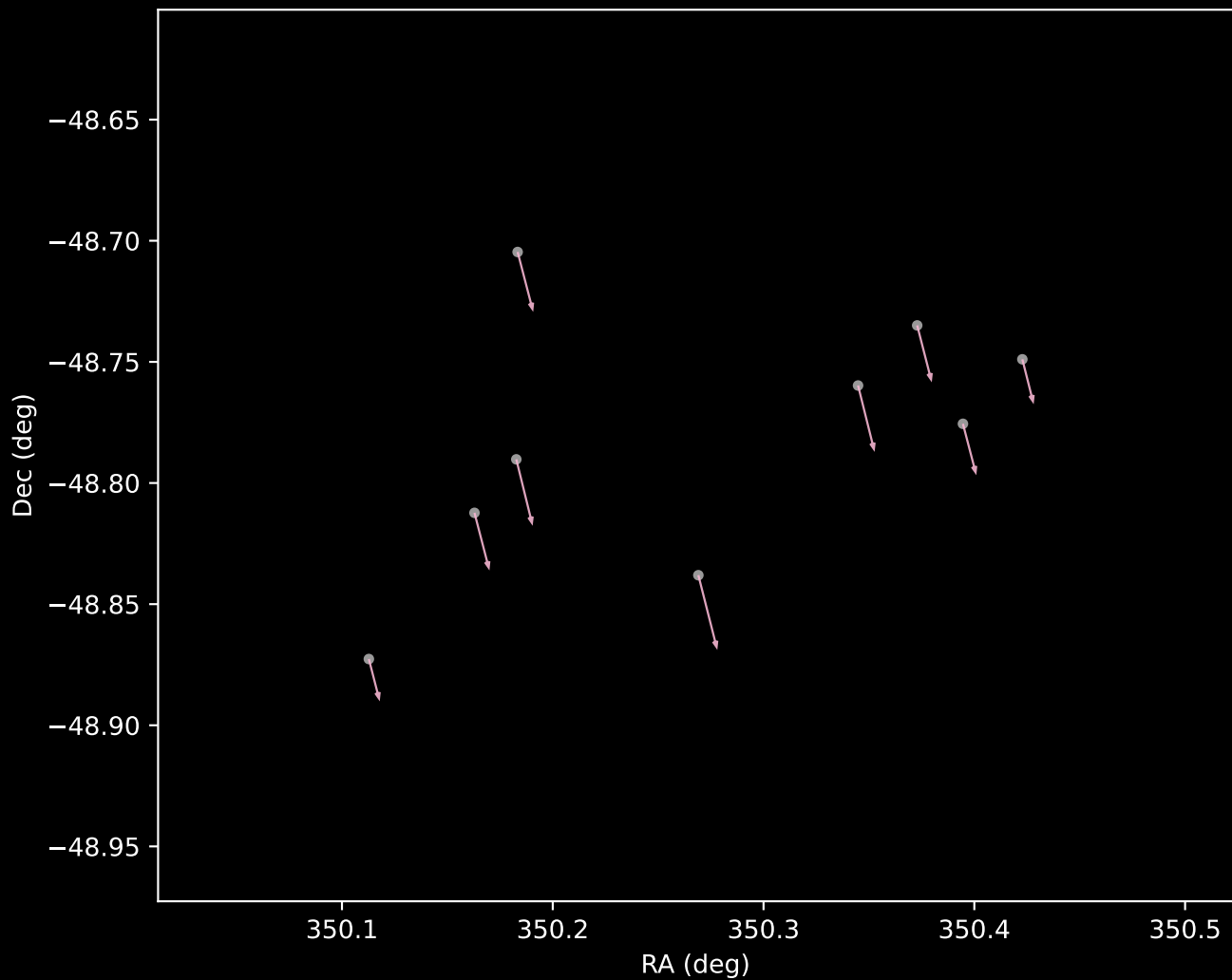
Gaia DR3 Cluster 13 Proper Motion Vectors (n=9)
