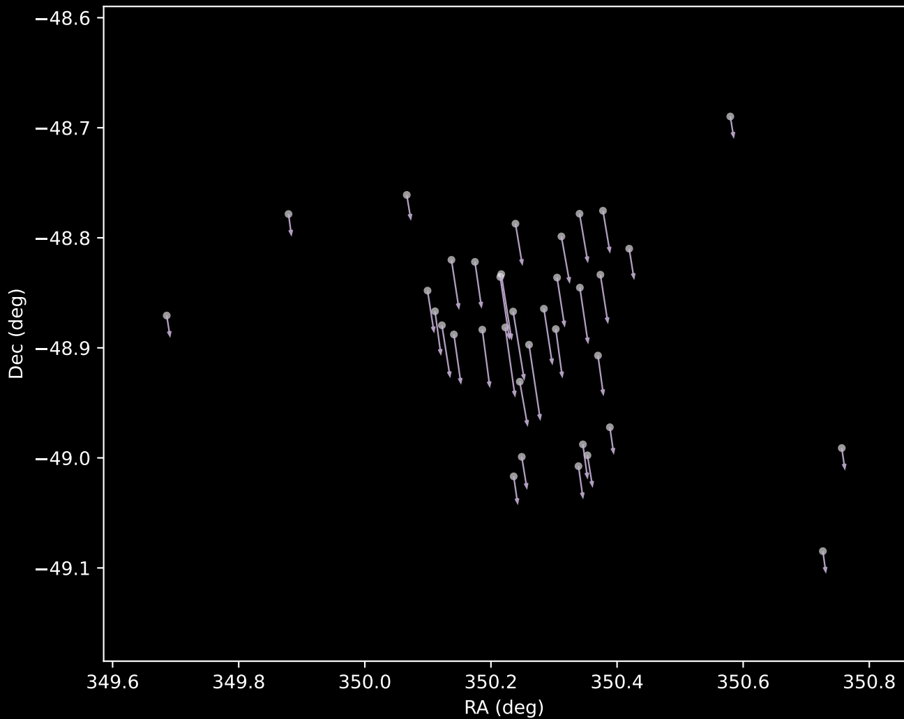
Gaia DR3 Cluster 9 Proper Motion Vectors (n=36)
