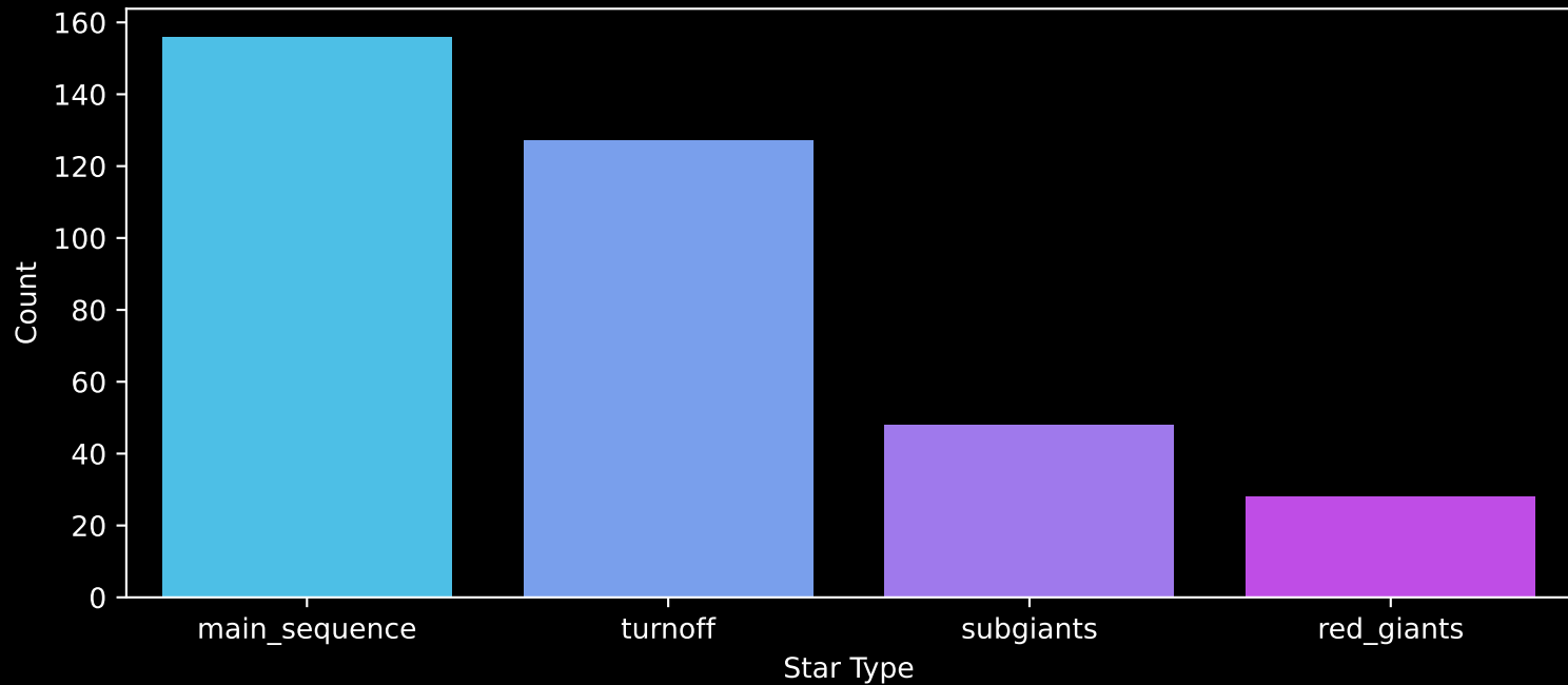
Gaia Cluster: [NGC_6193] Count plot of Star Type
