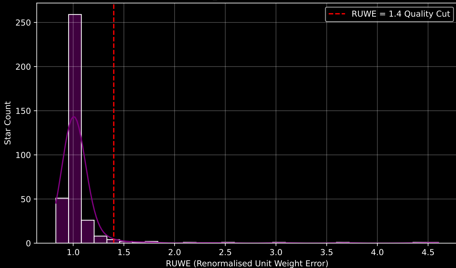
Gaia Cluster: [NGC_6193] RUWE Distribution (n= 359)
