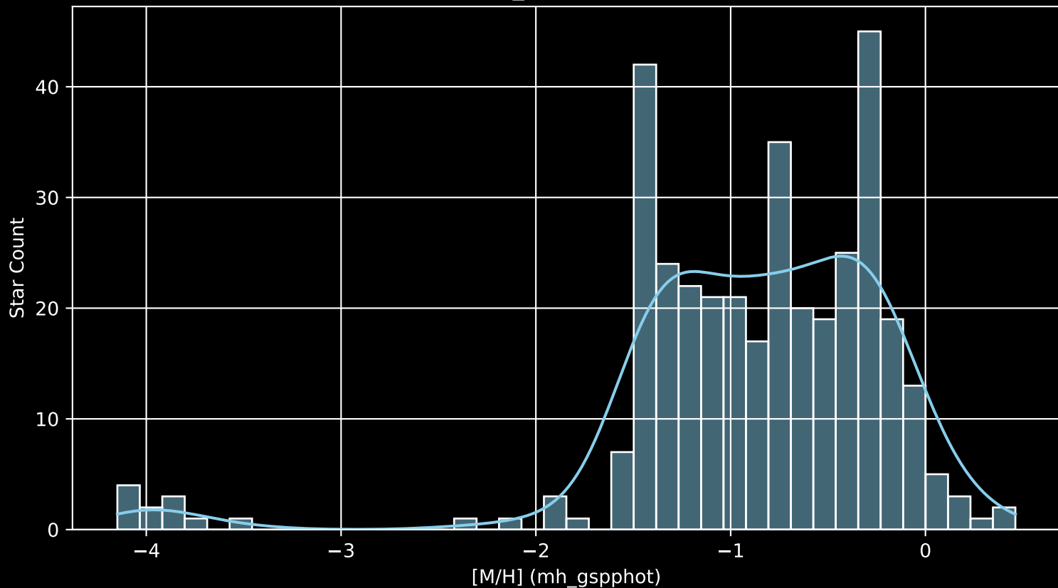
Gaia Cluster: [NGC_6193 [M/H] (mh_gspphot) (n= 358)
