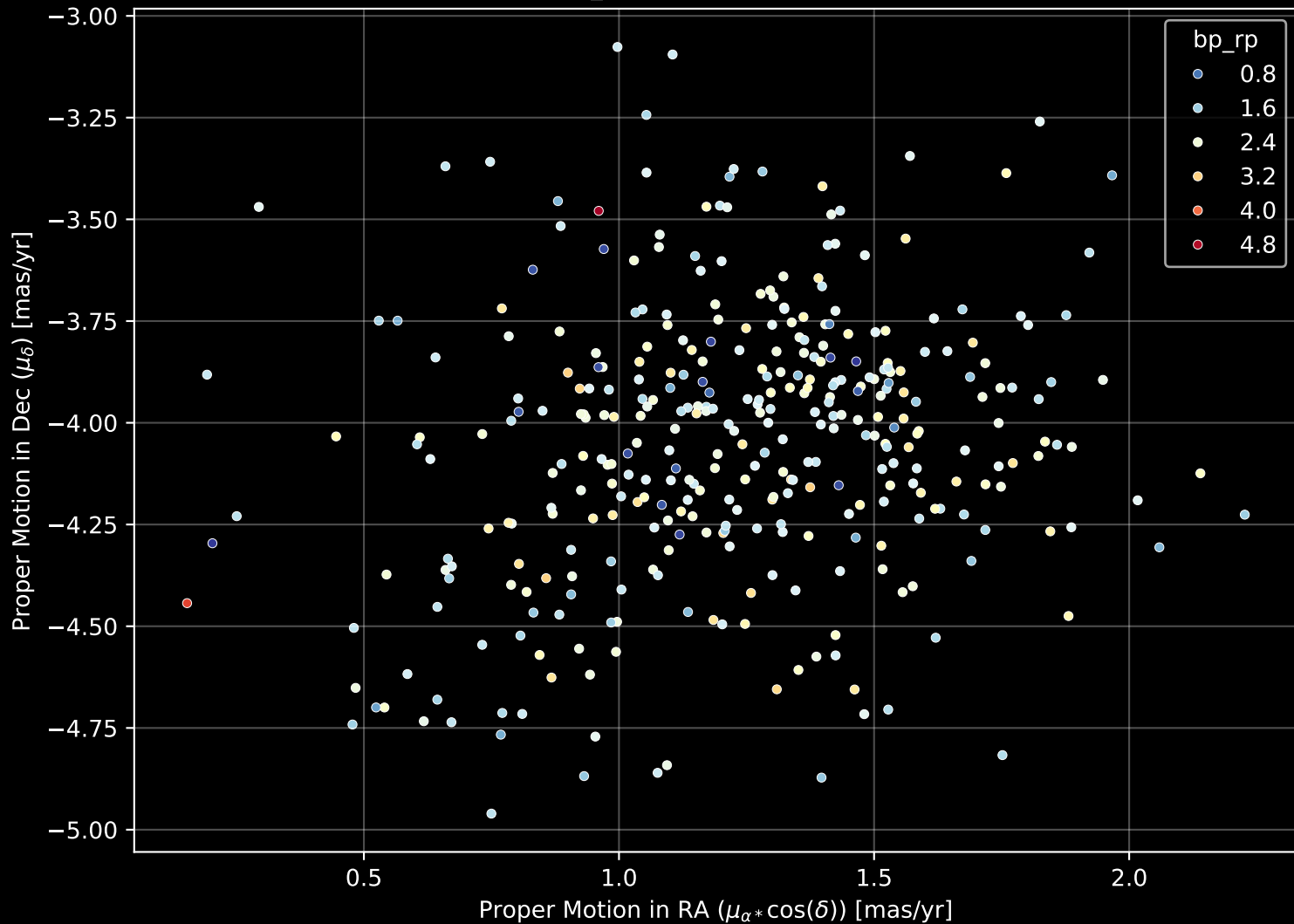
Gaia Cluster: [NGC_6193] Proper Motion Diagram (n= 359)
