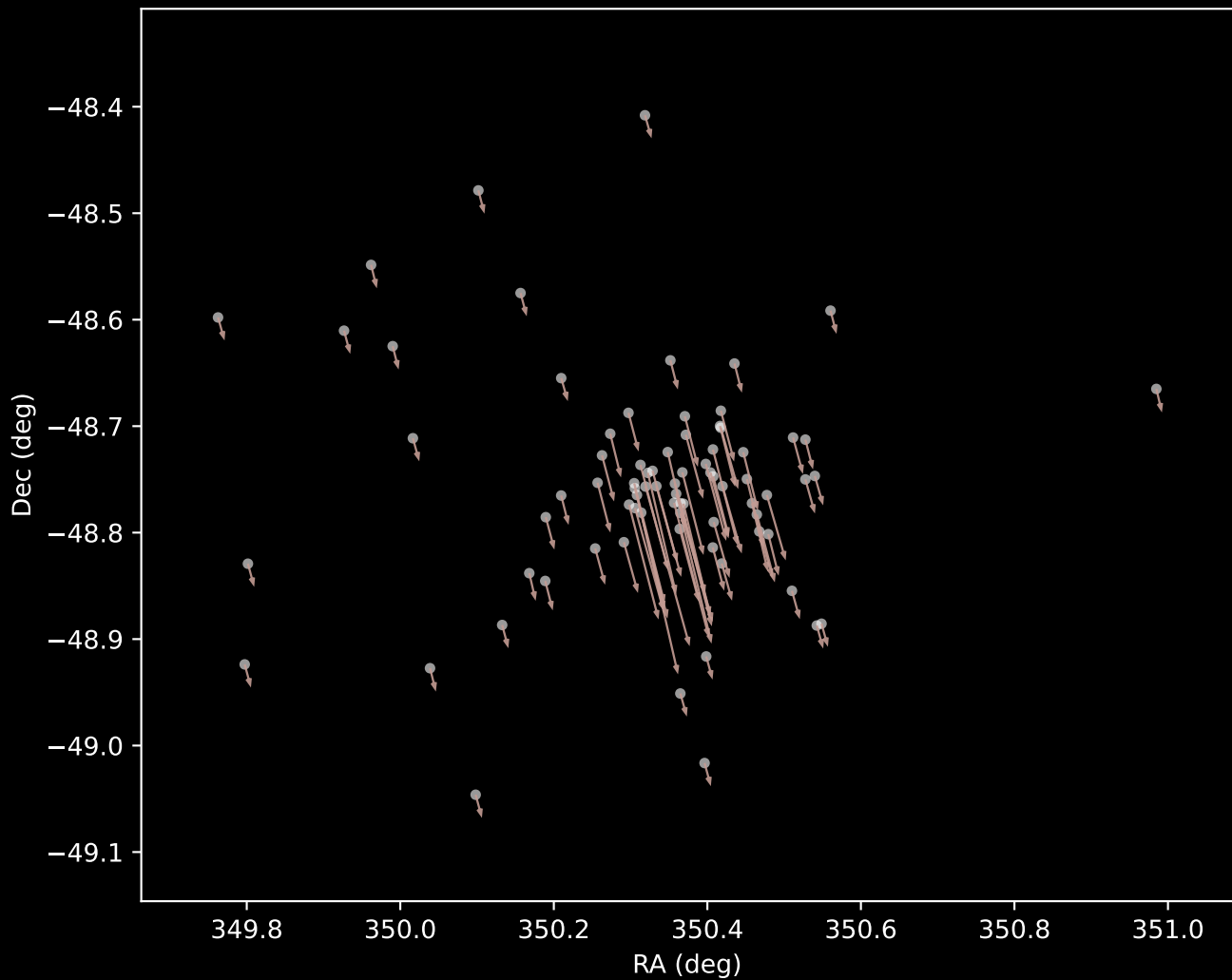
Gaia DR3 Cluster 11 Proper Motion Vectors (n=78)
