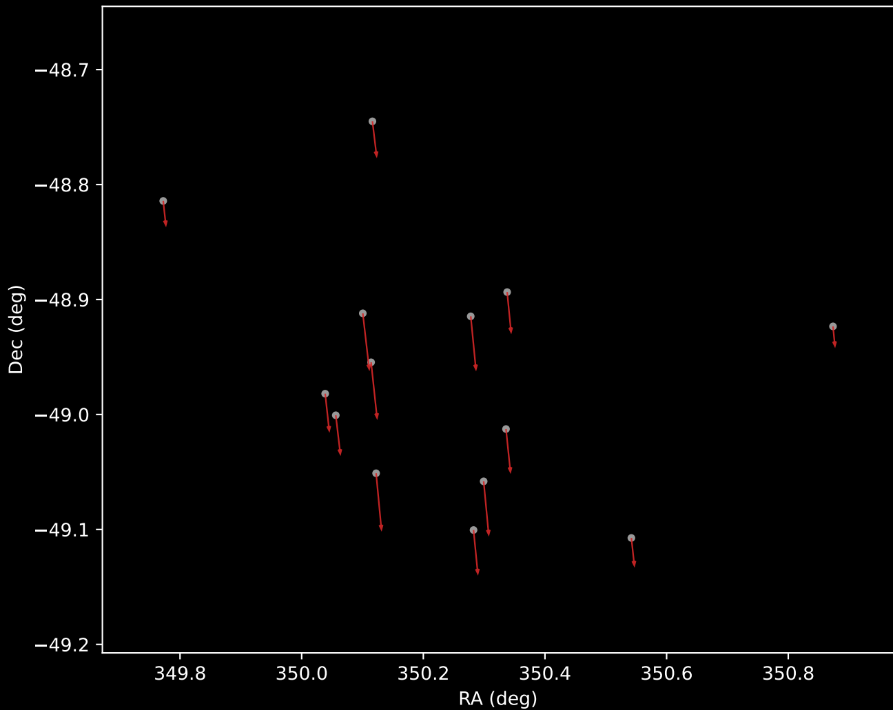
Gaia DR3 Cluster 6 Proper Motion Vectors (n=14)
