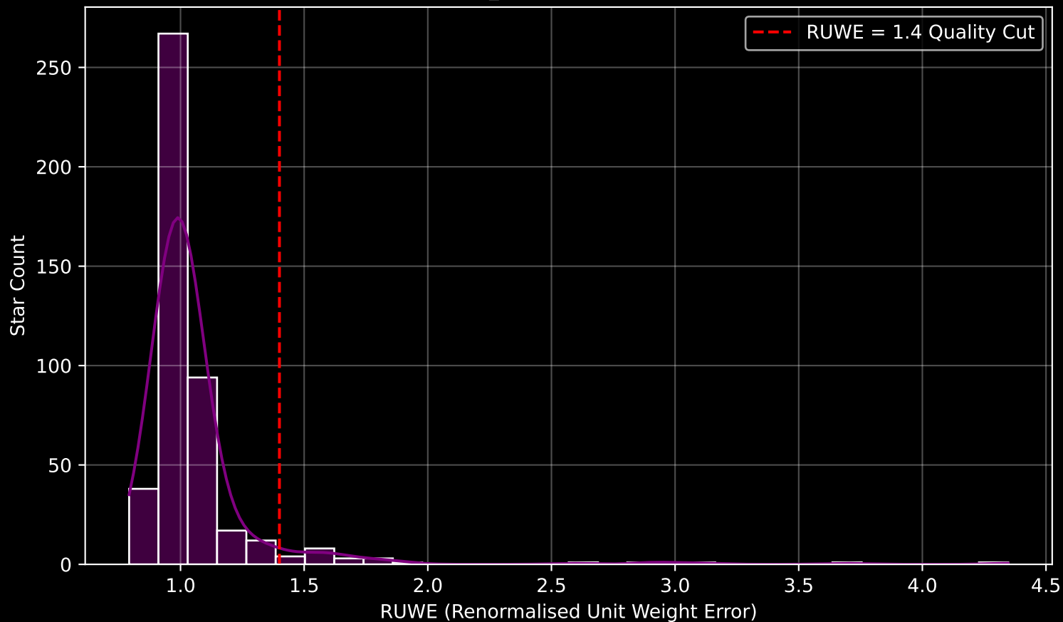
Gaia Cluster: [NGC_6208] RUWE Distribution (n= 453)
