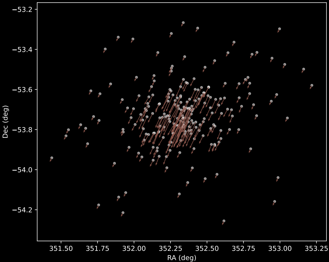
Gaia DR3 Cluster 10 Proper Motion Vectors (n=222)
