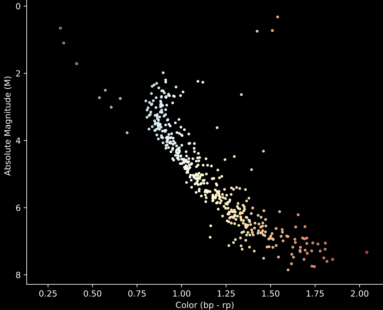
Gaia Cluster: [NGC 6208] Stars (n= 455) Hertzprung-Russel Diagram
