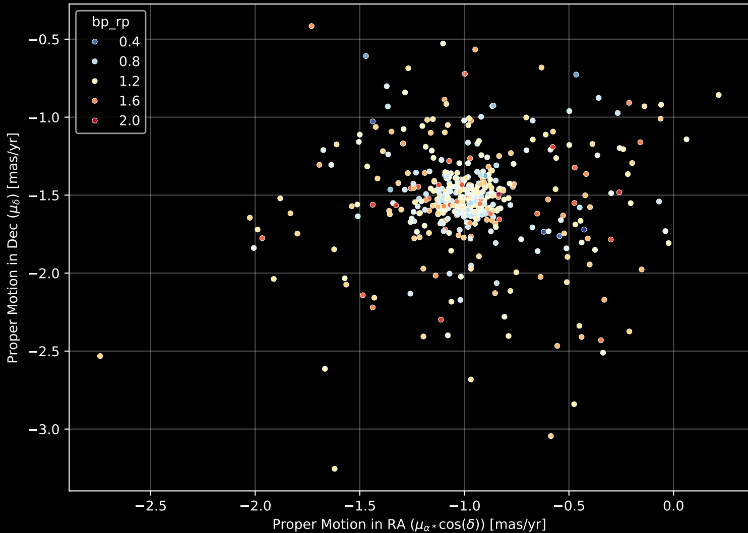
Gaia Cluster: [NGC_6208] Proper Motion Diagram (n= 455)
