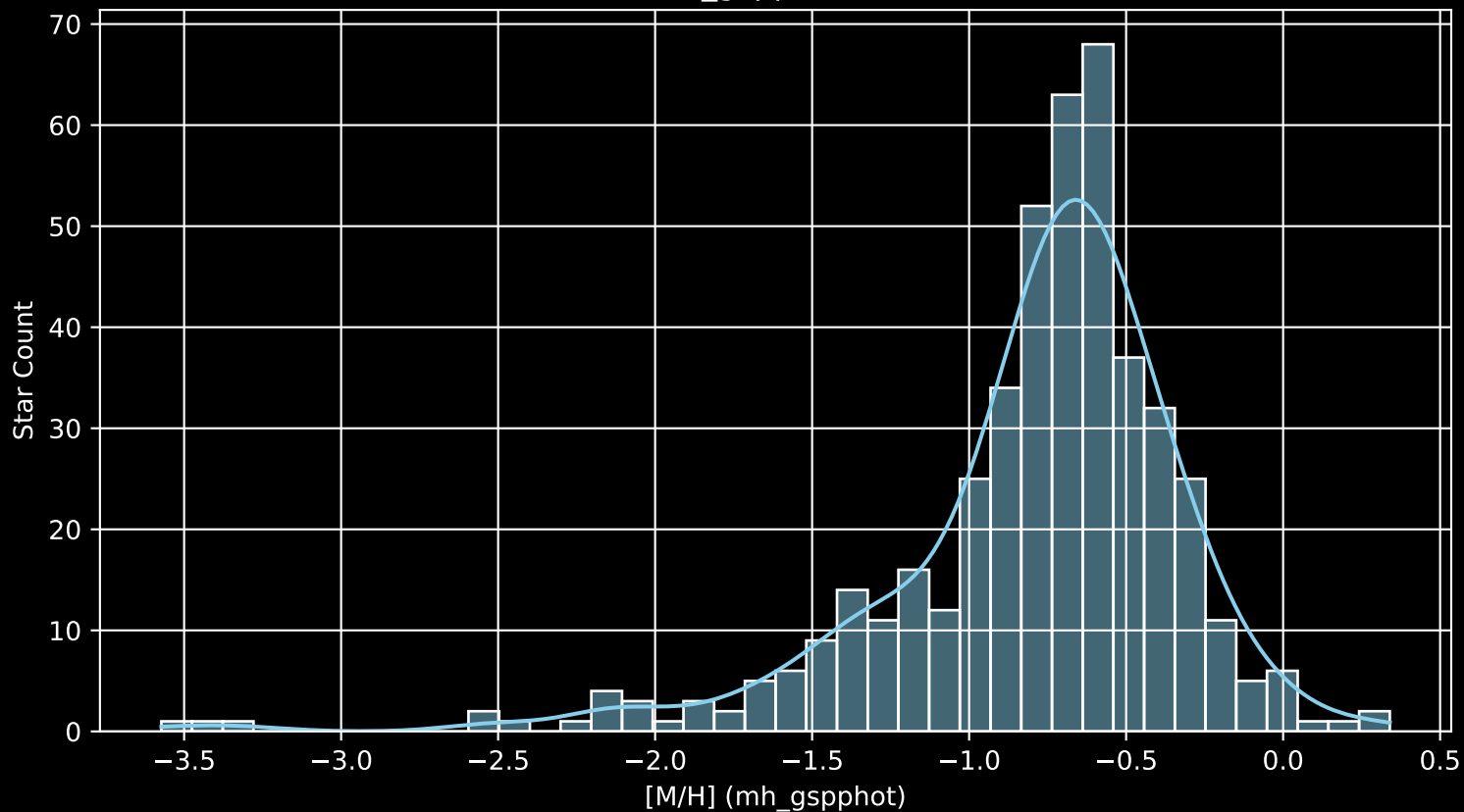
Gaia Cluster: [NGC_6208 [M/H] (mh_gspphot) (n= 455)
