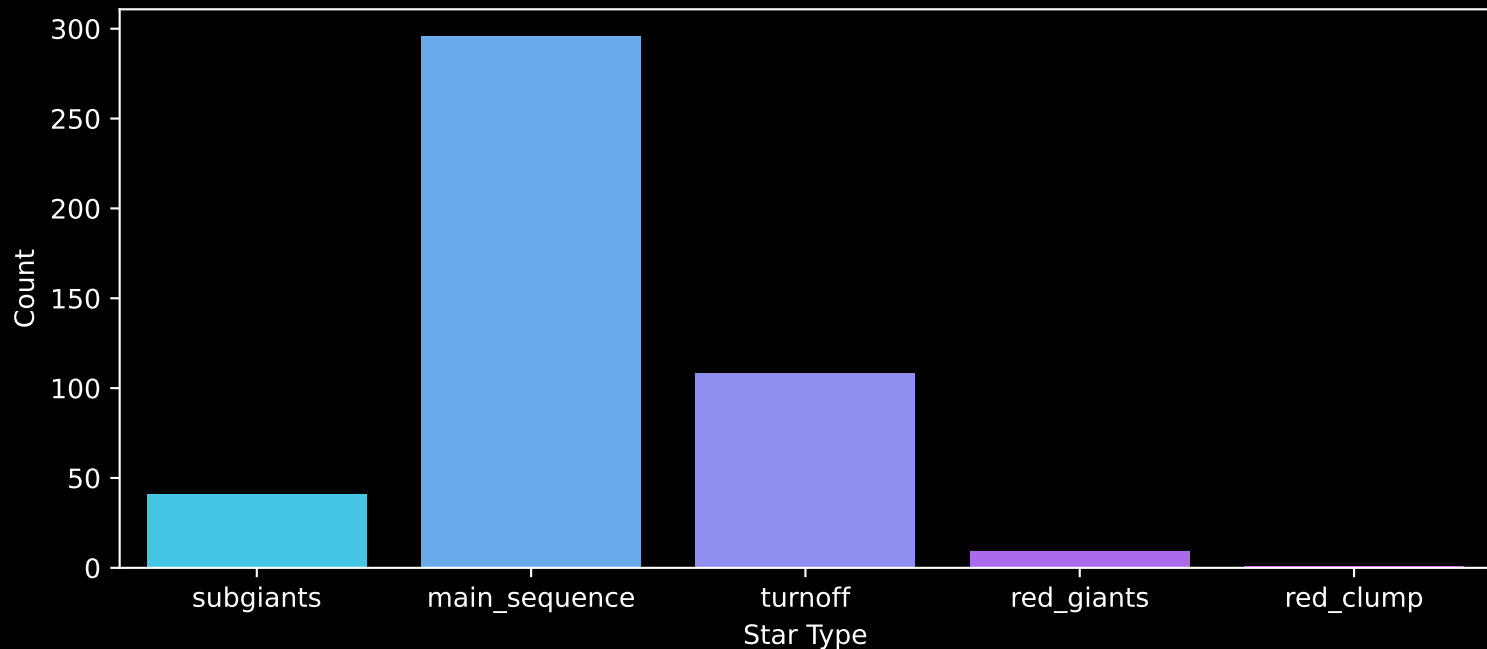
Gaia Cluster: [NGC_6208] Count plot of Star Type
