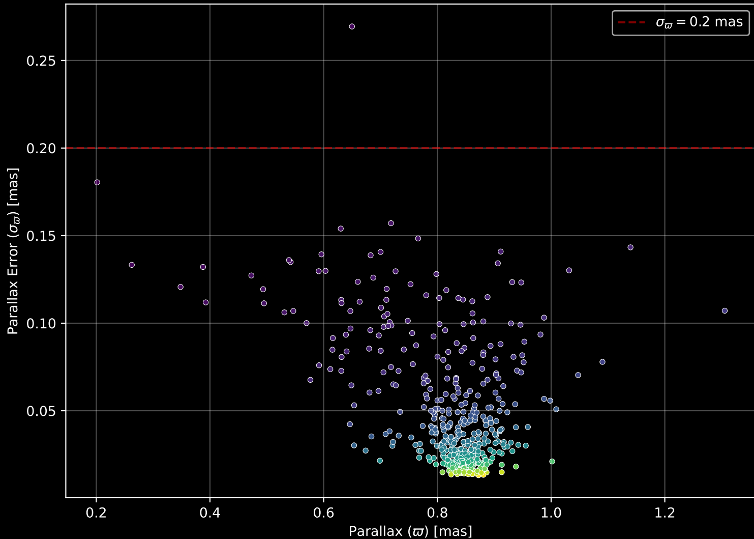
Gaia Cluster: [NGC_6208] Parallax Quality (n= 455)
