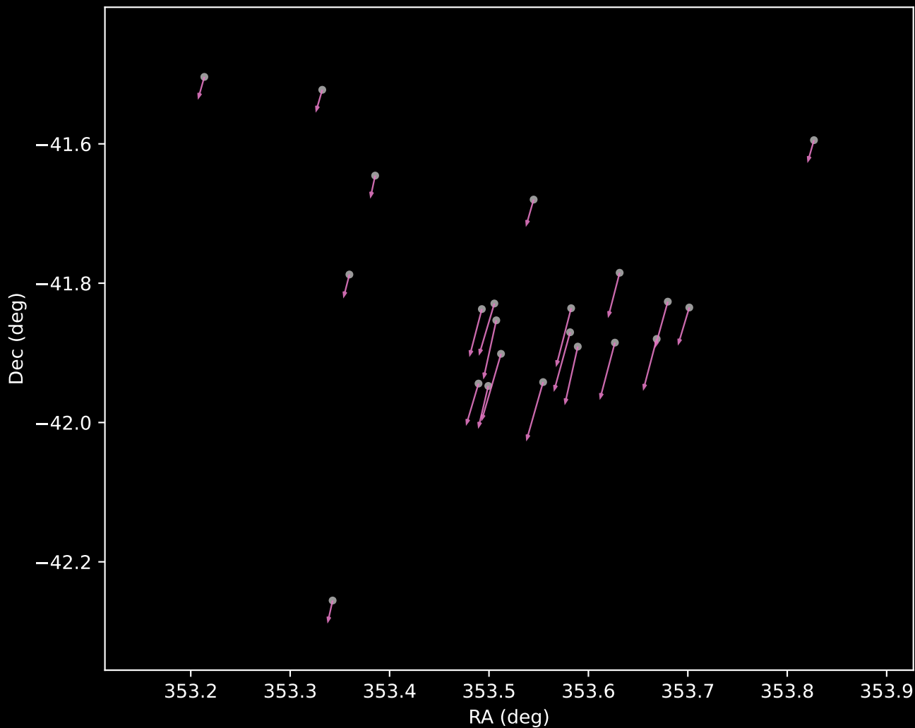
Gaia DR3 Cluster 32 Proper Motion Vectors (n=22)
