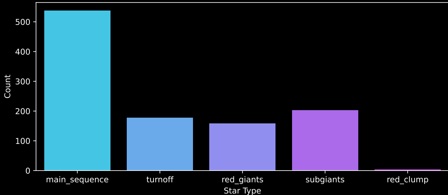
Gaia Cluster: [NGC_6231] Count plot of Star Type
