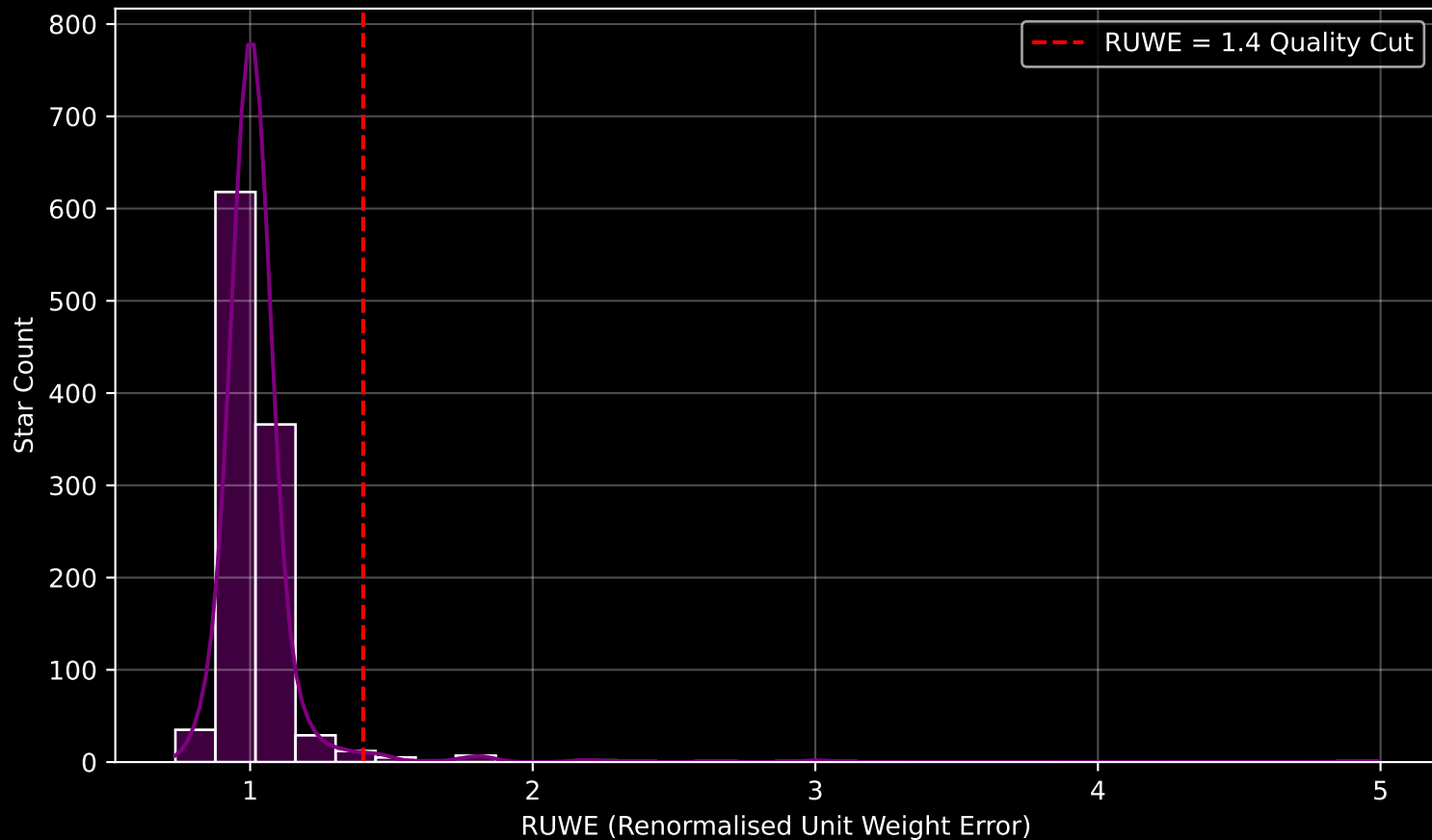
Gaia Cluster: [NGC_6231] RUWE Distribution (n= 1080)
