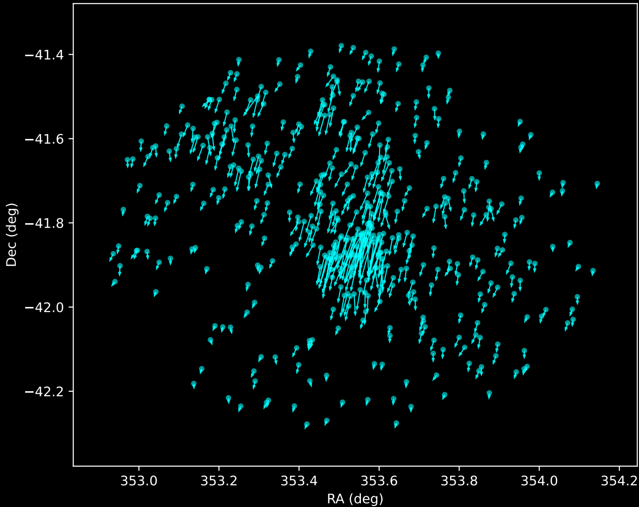
Gaia DR3 Noise Stream Proper Motion Vectors (n=450)
