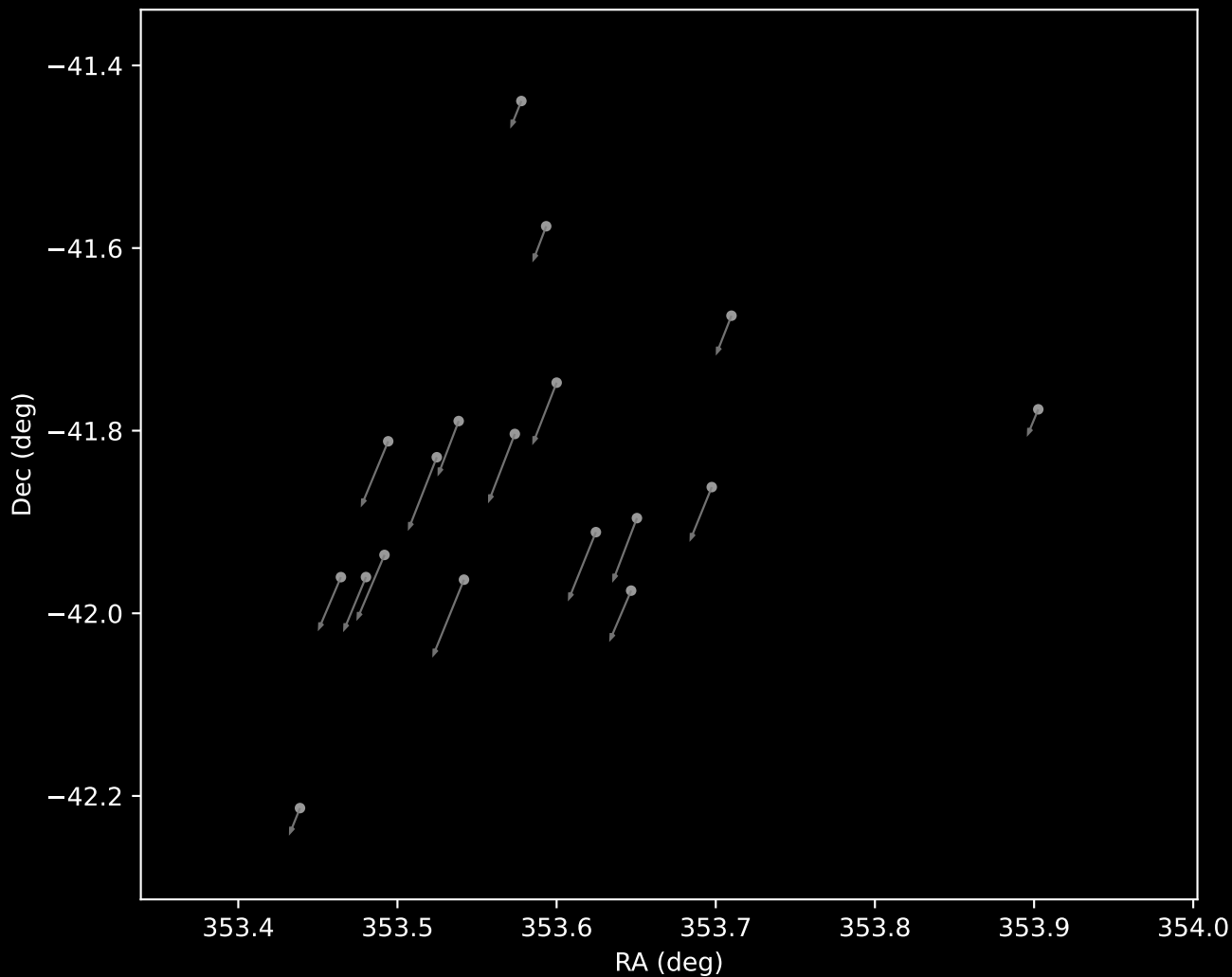
Gaia DR3 Cluster 54 Proper Motion Vectors (n=18)
