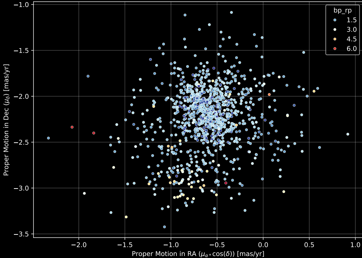
Gaia Cluster: [NGC_6231] Proper Motion Diagram (n= 1080)
