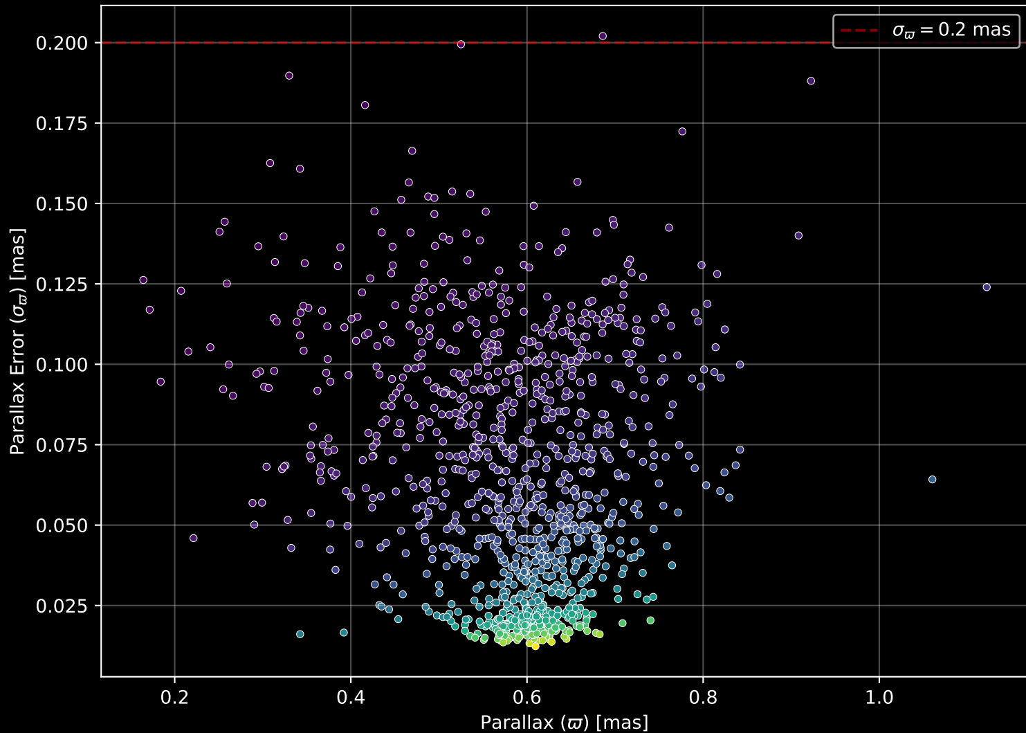
Gaia Cluster: [NGC_6231] Parallax Quality (n= 1080)
