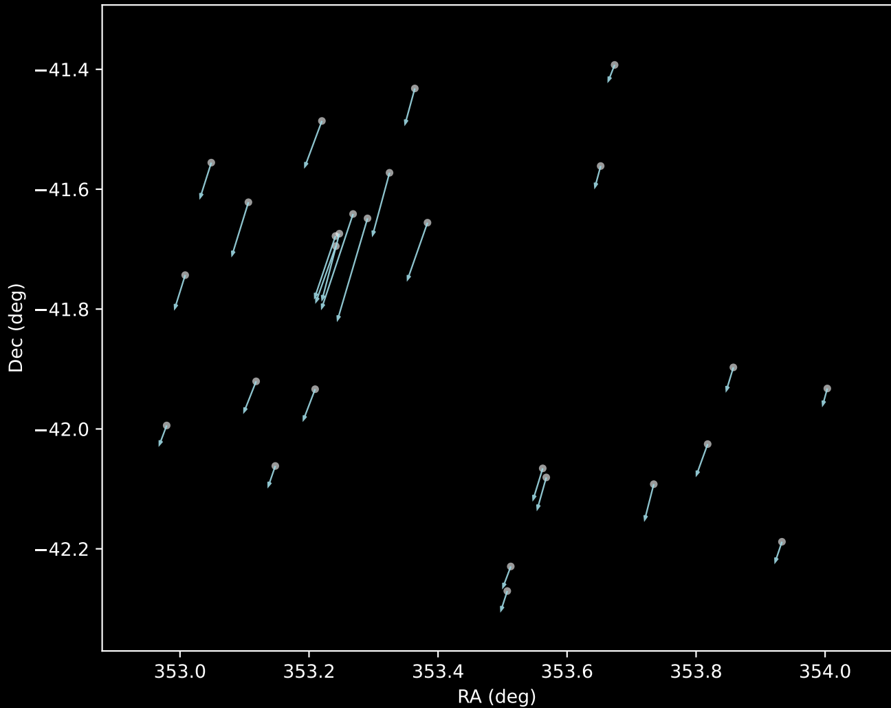
Gaia DR3 Cluster 19 Proper Motion Vectors (n=27)
