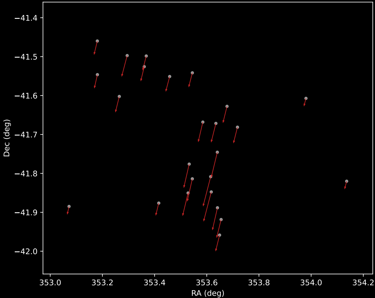
Gaia DR3 Cluster 46 Proper Motion Vectors (n=25)
