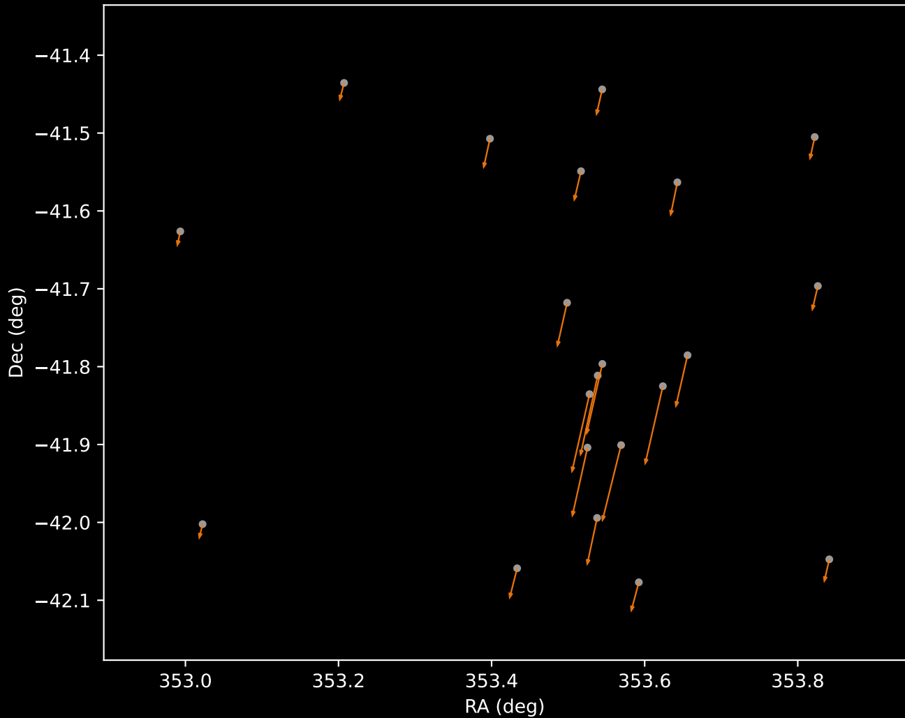
Gaia DR3 Cluster 42 Proper Motion Vectors (n=21)
