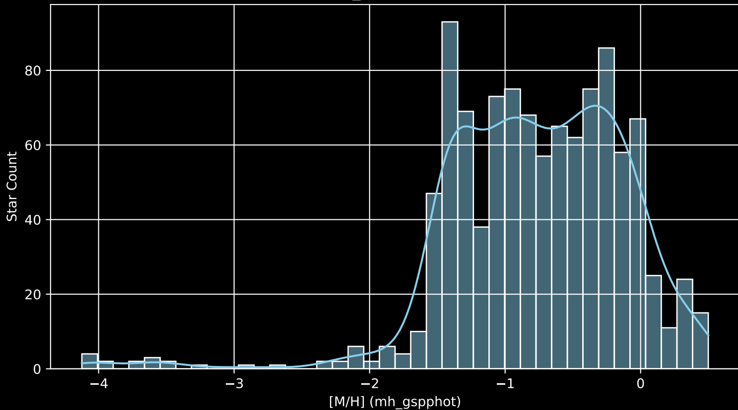
Gaia Cluster: [NGC_6231 [M/H] (mh_gspphot) (n= 1056)
